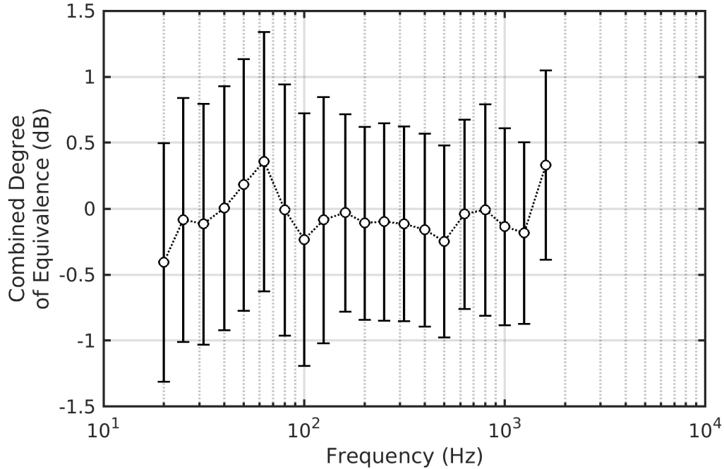
Figure D-23. Comparison BC-6 – Degree of Equivalence – LEFAC
