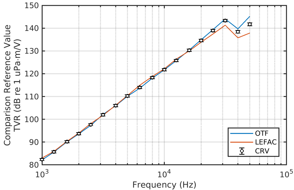
Figure D-16. Comparison BC-5 – F37 SN A117 – Transmitting Voltage Response
