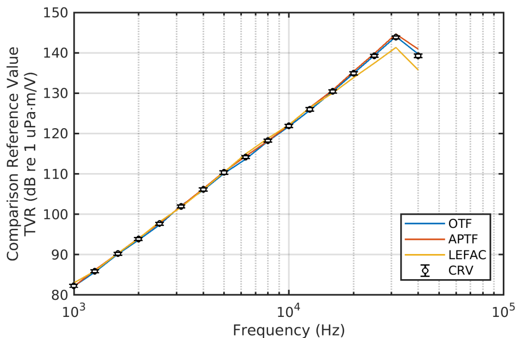
Figure D-28. Comparison MC-2 – Type F37 SN A117 – Transmitting Voltage Response
