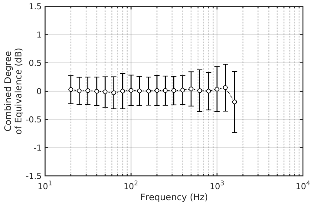
Figure D-22. Comparison BC-6 – Degree of Equivalence – LOFAC
