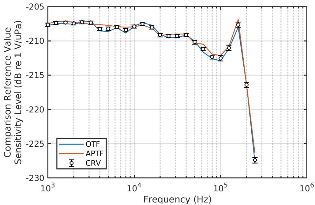
Figure D-2. Comparison BC-1 – Type F42D SN 145 – Receive Voltage Response
