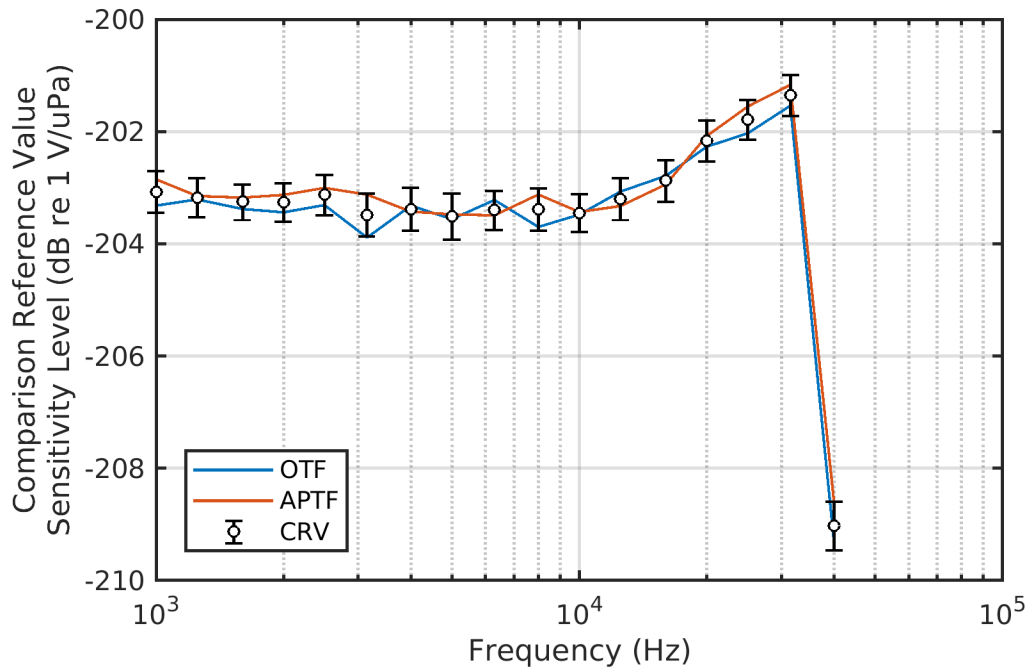
Figure D-5. Comparison BC-2 – Type F37 SN A117 – Receive Voltage Response
