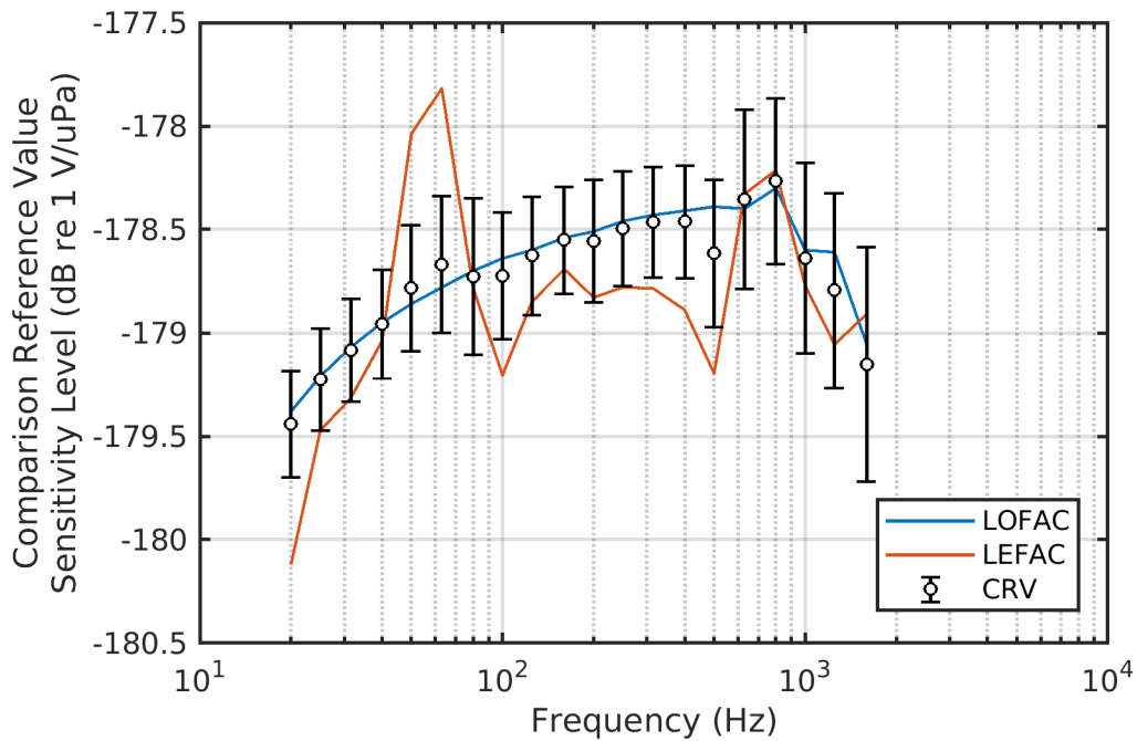
Figure D-19. Comparison BC-6 – Type H52 SN 84 – RVS
