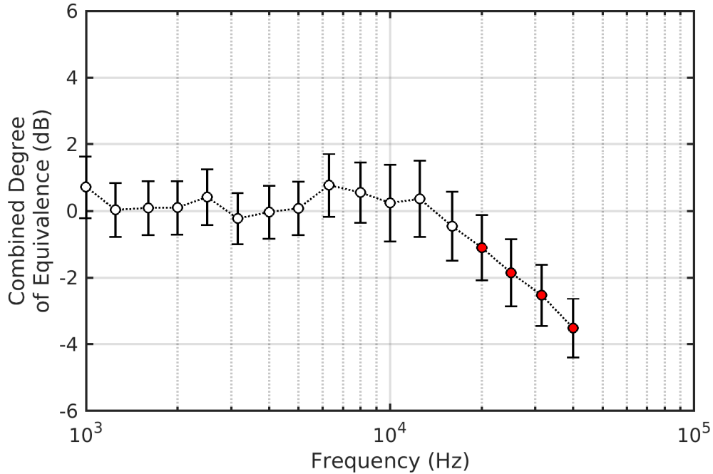
Figure D-31. Comparison MC-2 – Degree of Equivalence – LEFAC
