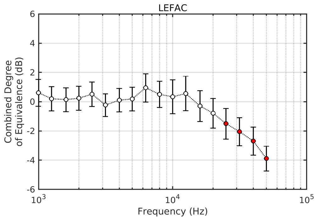
Figure D-18. Comparison BC-5 – Degree of Equivalence – LEFAC
