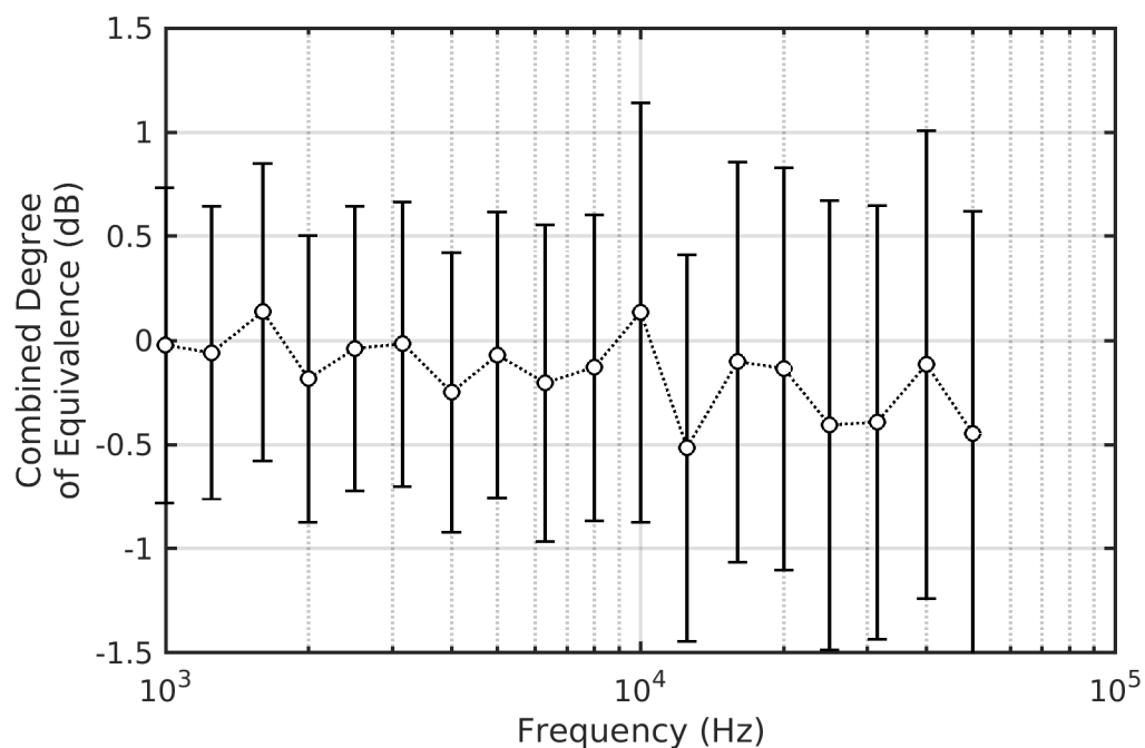
Figure D-15. Comparison BC-4 – Degree of Equivalence – LEFAC
