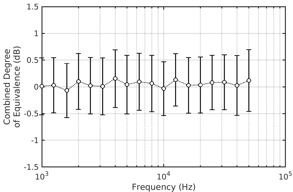
Figure D-14. Comparison BC-4 – Degree of Equivalence – OTF
