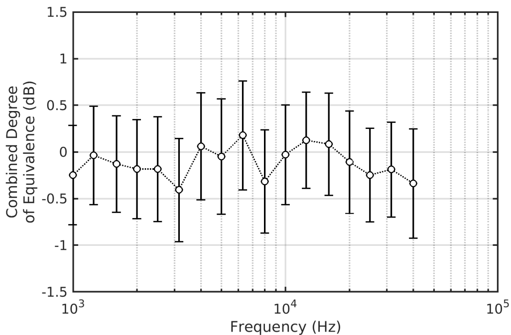
Figure D-6. Comparison BC-2 – Degree of Equivalence – OTF
