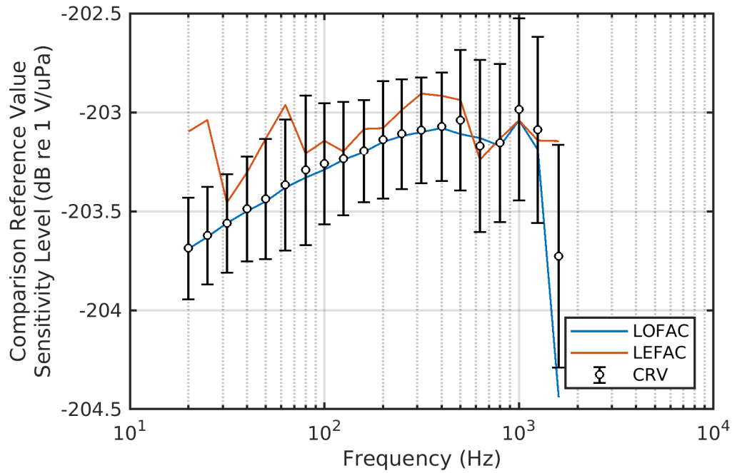
Figure D-21. Comparison BC-6 – Type F37 SN A117 – RVS
