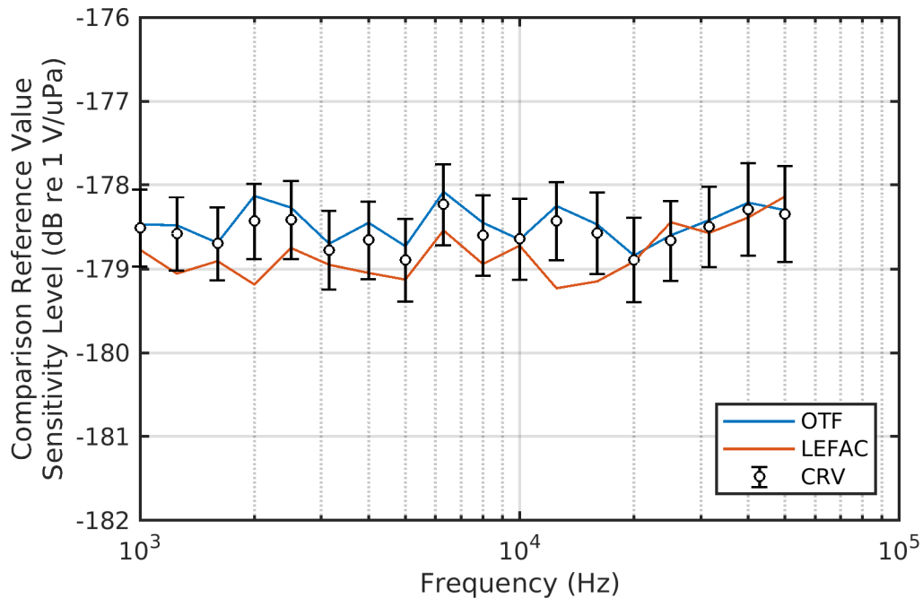
Figure D-11. Comparison BC-4 – Type H52 SN 84 – Receive Voltage Response
