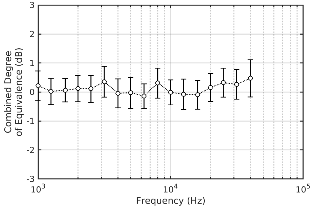
Figure D-26. Comparison MC-1 – Degree of Equivalence – APTF
