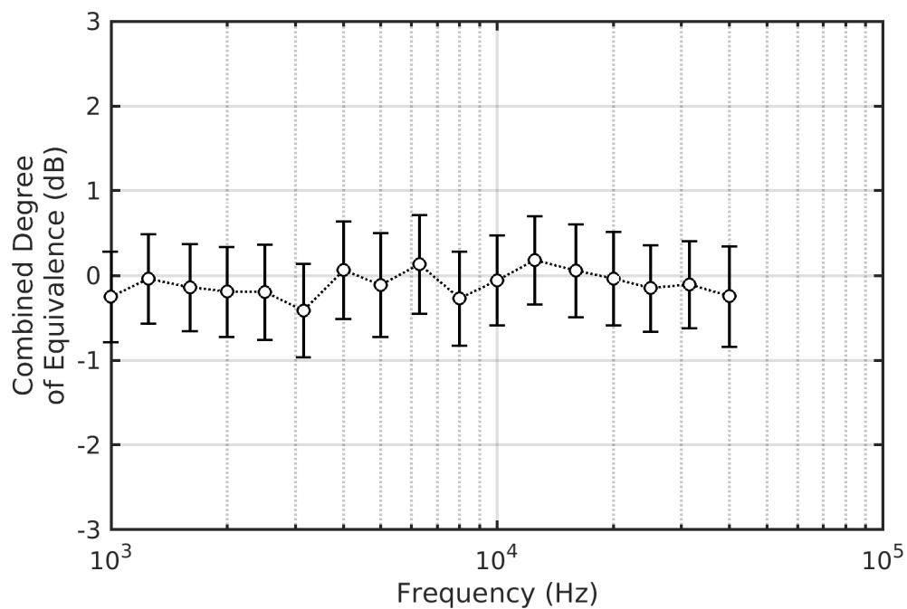
Figure D-25. Comparison MC-1 – Degree of Equivalence – OTF
