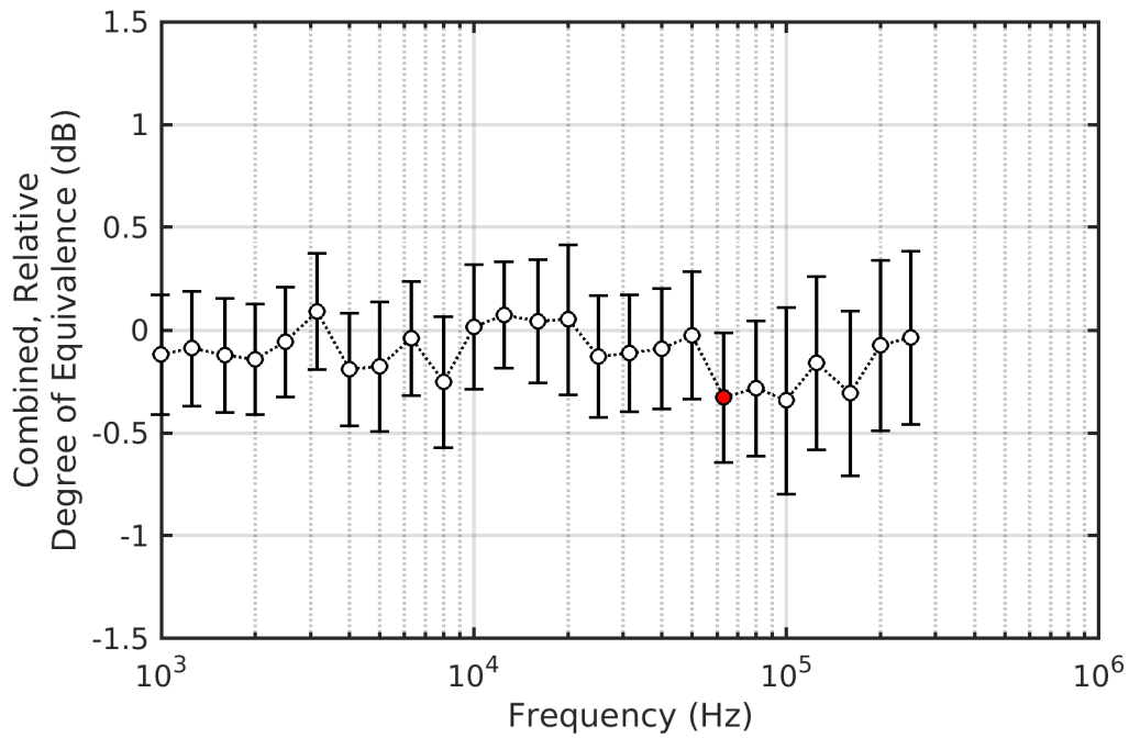
Figure D-3. Comparison BC-1 – Degree of Equivalence – OTF
