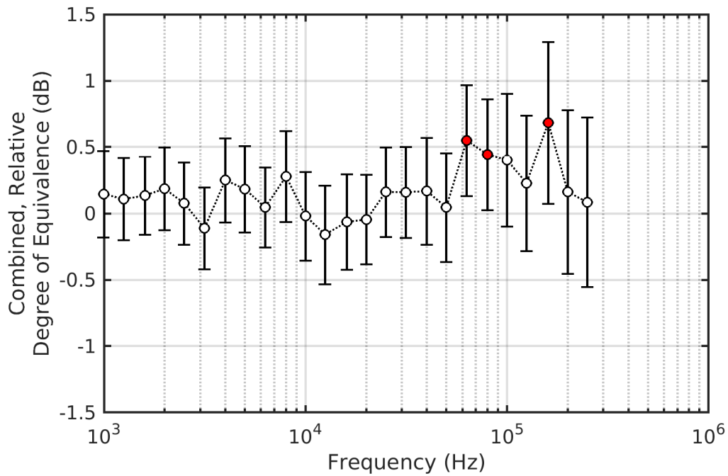
Figure D-4. Comparison BC-1 – Degree of Equivalence – APTF
