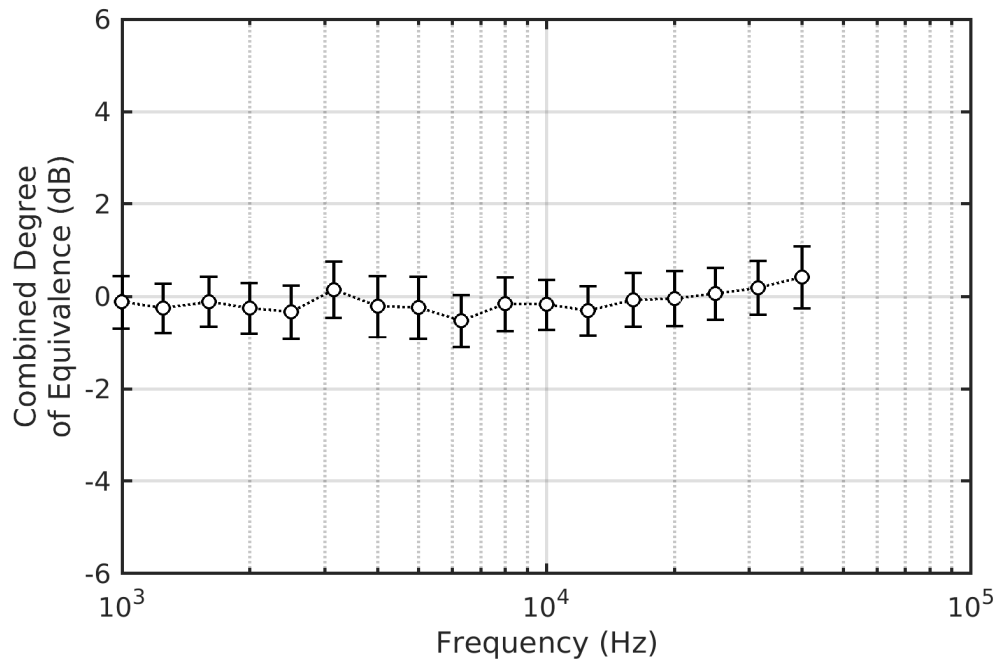
Figure D-29. Comparison MC-2 – Degree of Equivalence – OTF
