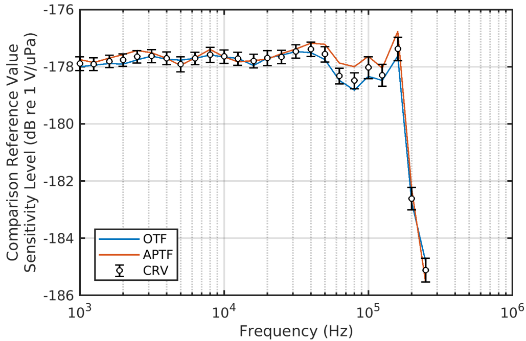
Figure D-1. Comparison BC-1 – Type H52 SN 80 – Receive Voltage Response
