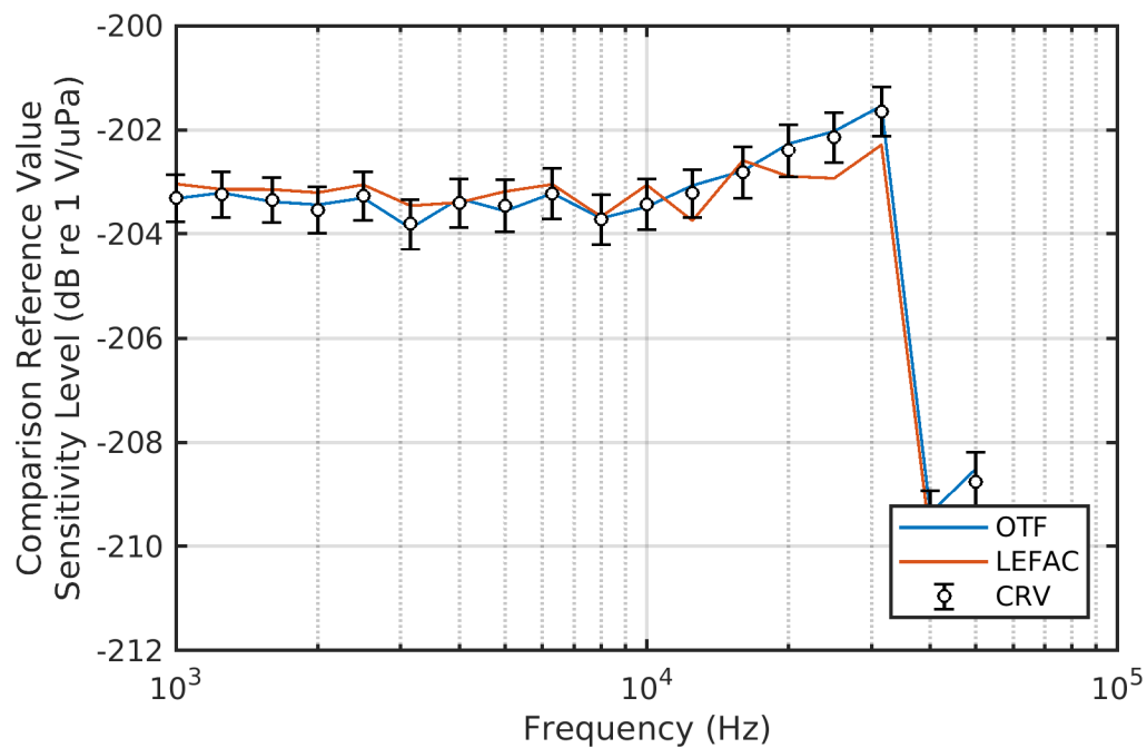
Figure D-13. Comparison BC-4 – Type F37 SN 117 – Receive Voltage Response
