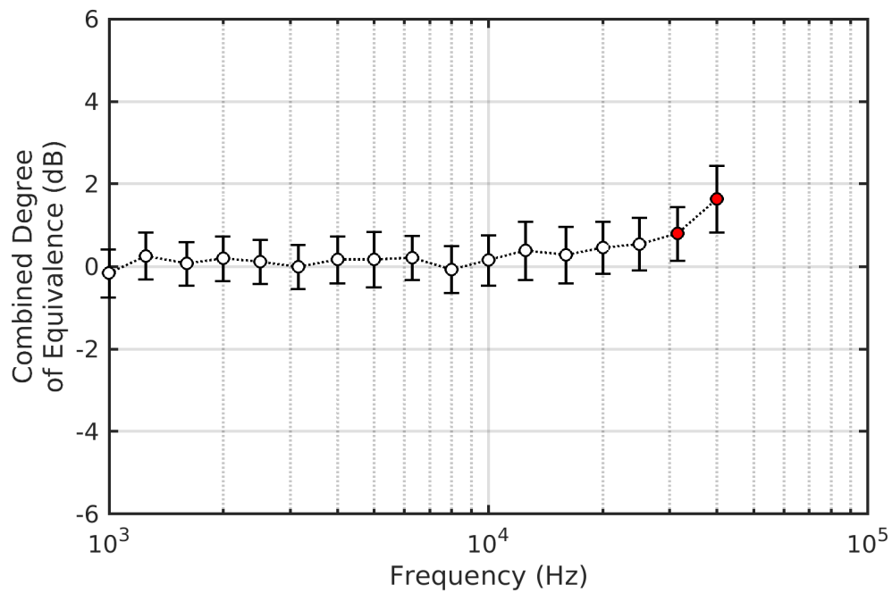
Figure D-30. Comparison MC-2 – Degree of Equivalence – APTF
