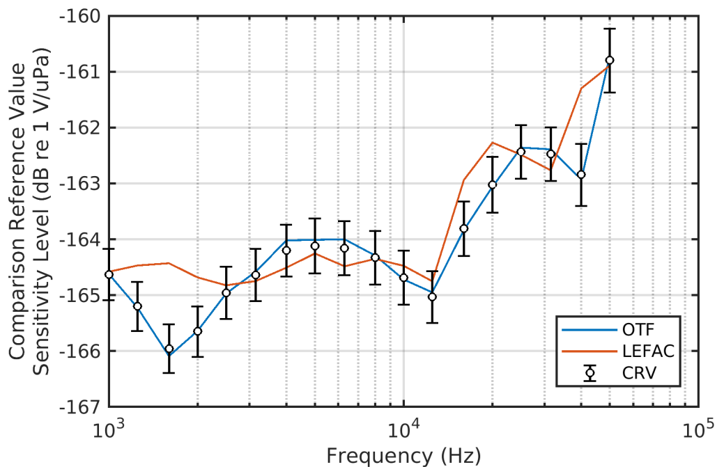
Figure D-12. Comparison BC-4 – Type H56 SN 125 – Receive Voltage Response
