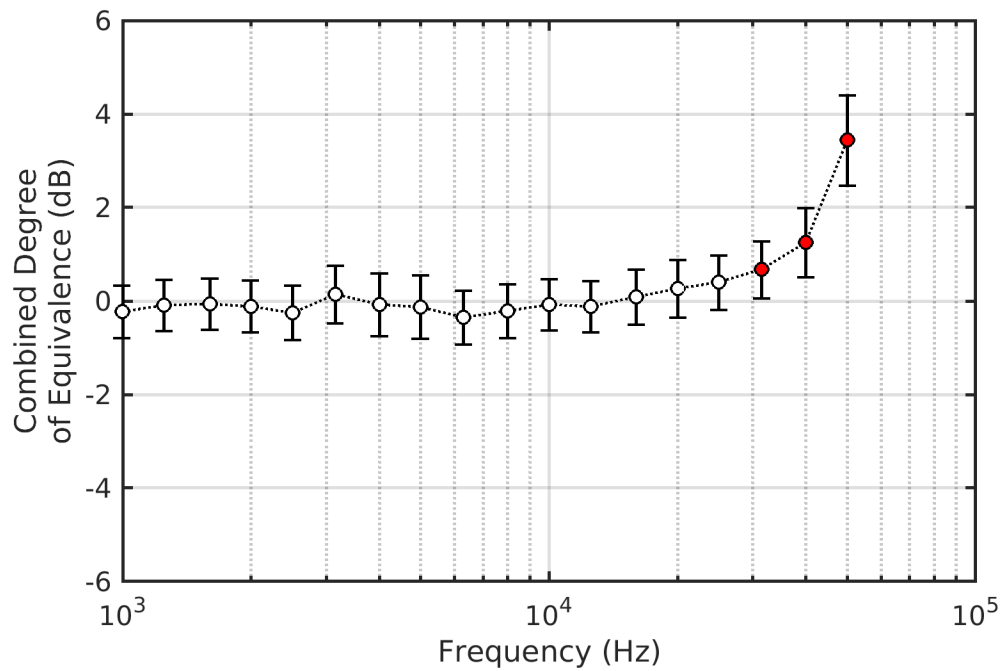
Figure D-17. Comparison BC-5 – Degree of Equivalence – OTF
