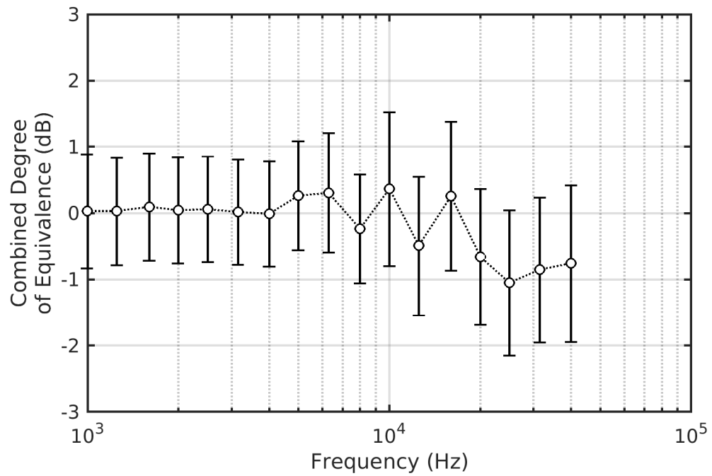
Figure D-27. Comparison MC-1 – Degree of Equivalence – LEFAC
