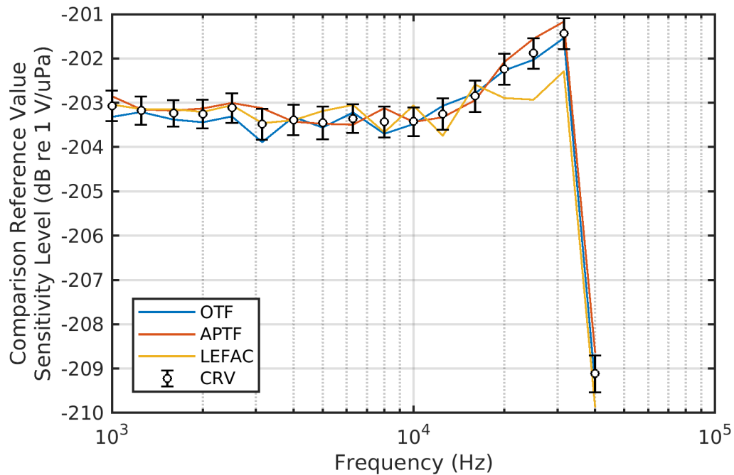
Figure D-24. Comparison MC-1 – Type F37 SN A117 – RVS
