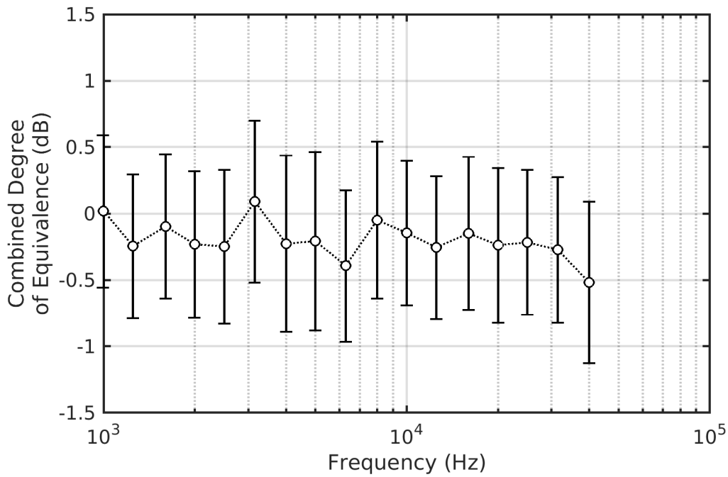
Figure D-9. Comparison BC-3 – Degree of Equivalence – OTF
