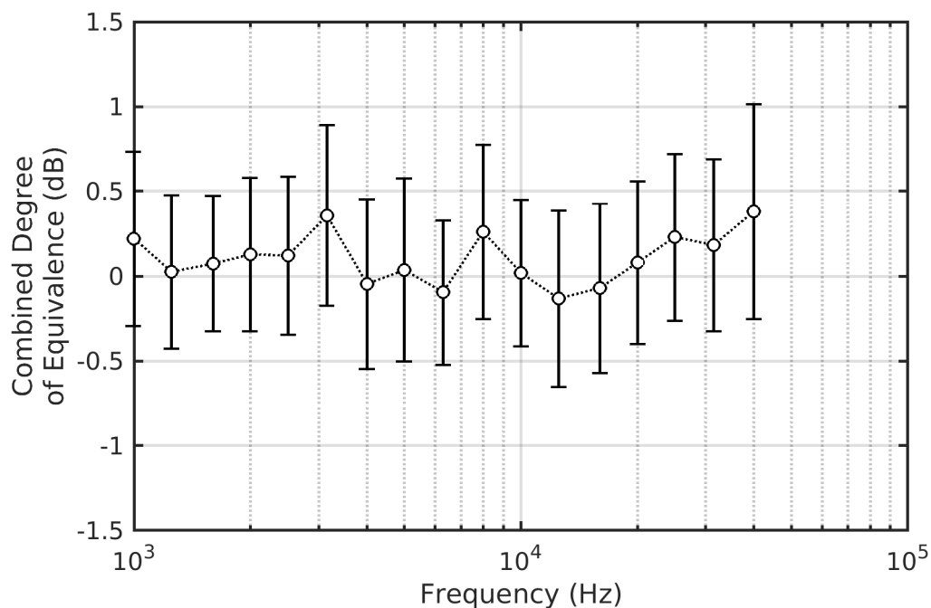
Figure D-7. Comparison BC-2 – Degree of Equivalence – APTF
