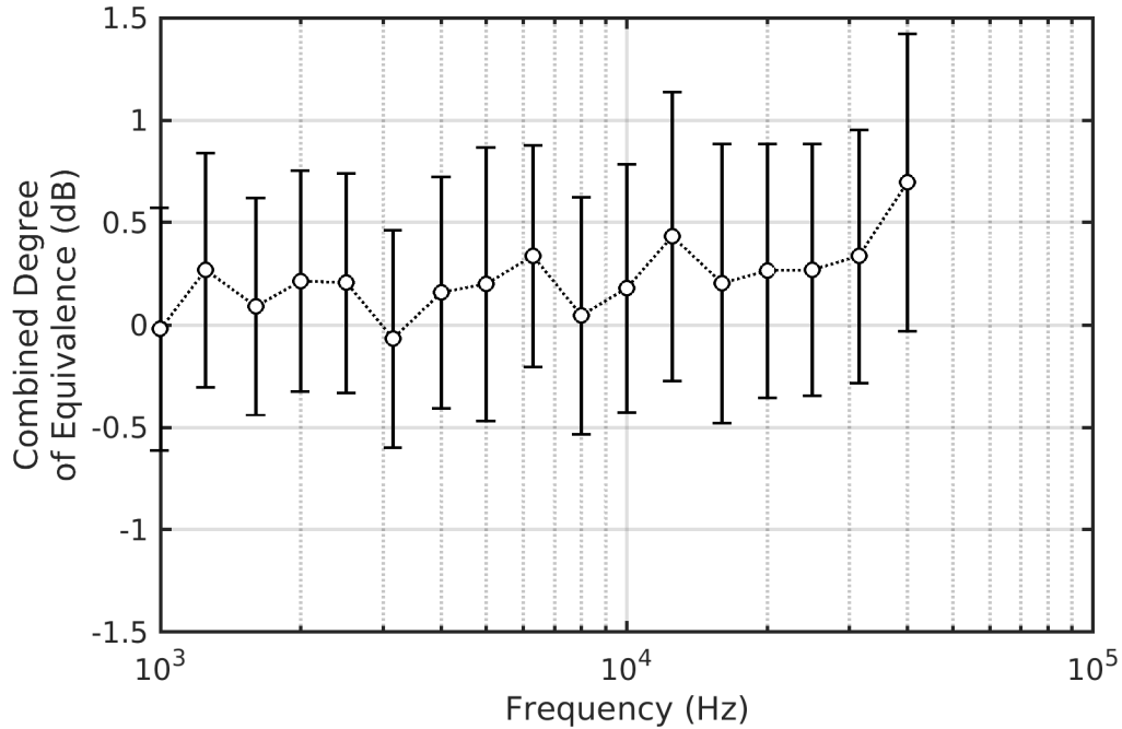
Figure D-10. Comparison BC-3 – Degree of Equivalence – APTF
