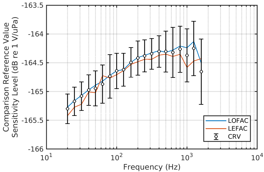
Figure D-20. Comparison BC-6 – Type H56 SN 125 – RVS
