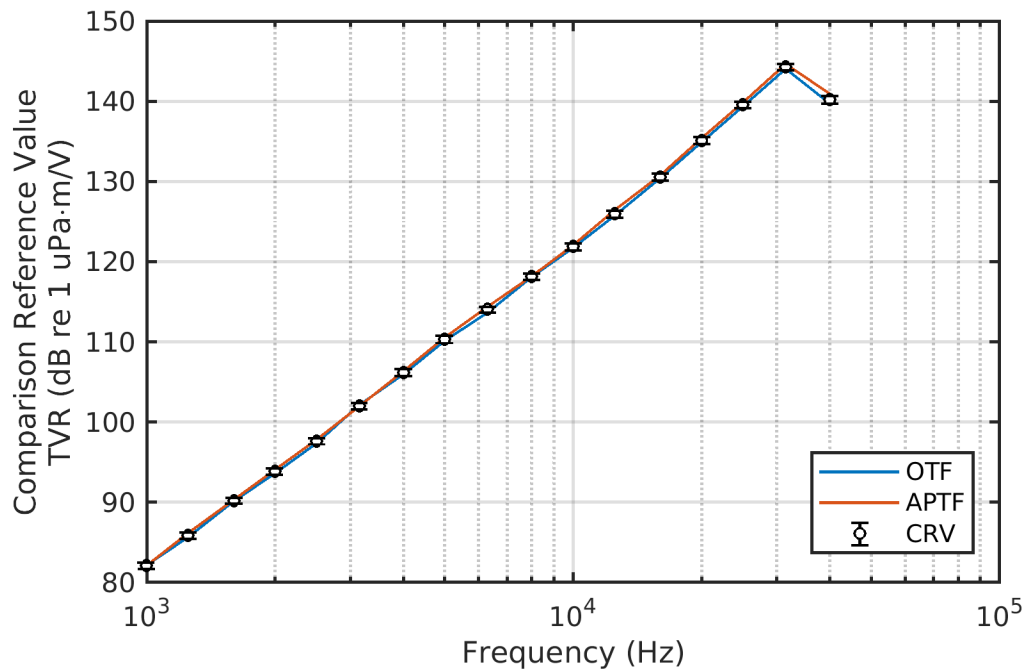
Figure D-8. Comparison BC-3 –Type F37 SN A117 – Transmitting Voltage Response
