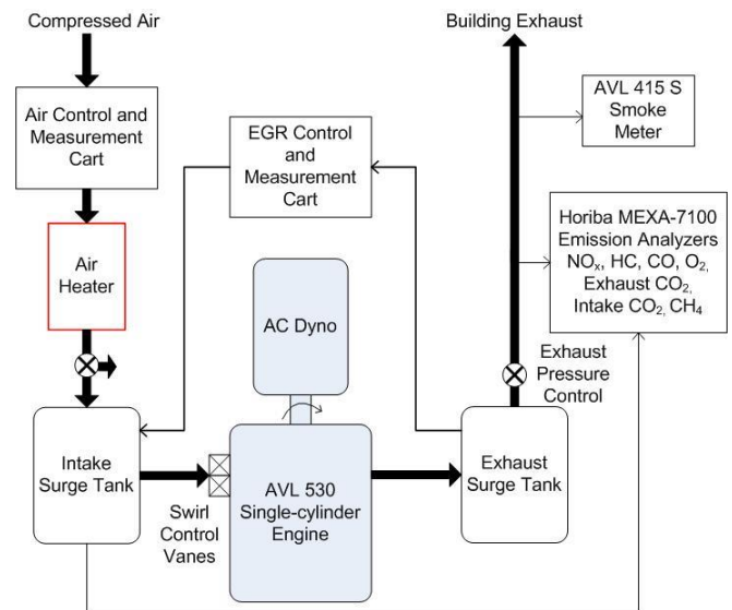
Figure 1: Laboratory setup.
