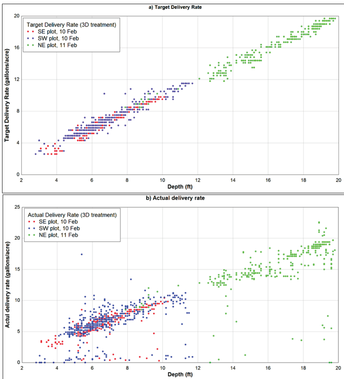
Figure 13. Target (a) and actual (b) delivery rate versus depth for 3-D delivery mode of dye for all 3-D treatments in Lake Underhill, FL, February 2016.
