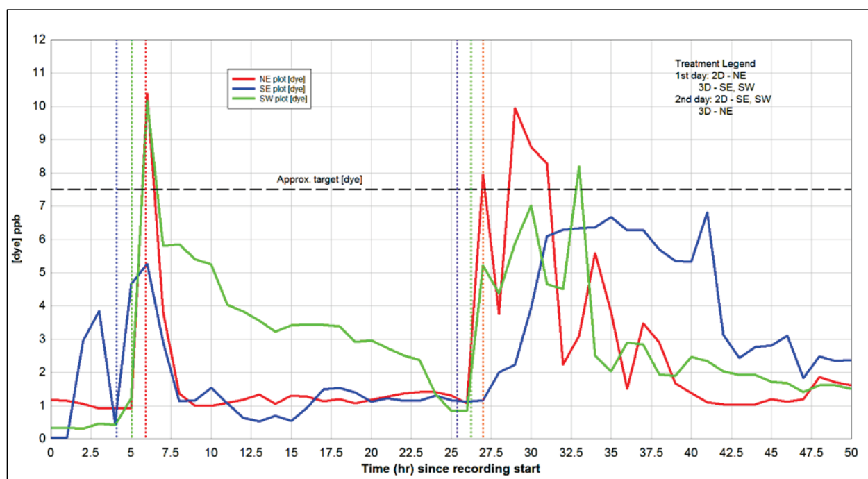
Figure 14. Hydrolab dye concentration measurements in treated plots in Lake Underhill, FL. Vertical dotted lines indicate time treatment was completed by plot.
