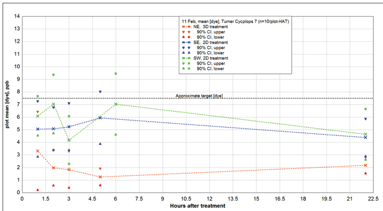
Figure 16. Mean of dye concentration measurements (Turner Cyclops 7) in treated plots in Lake Underhill, FL, 11 February 2016.
