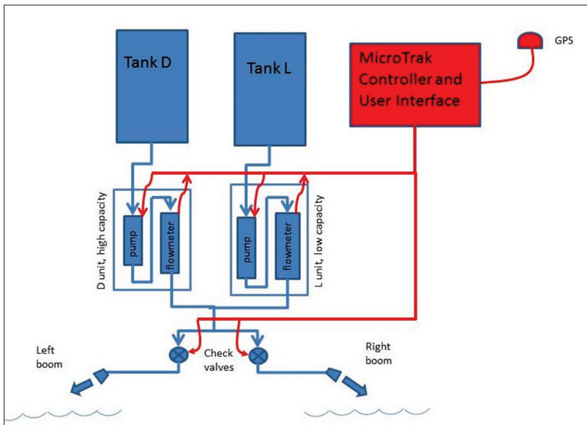
Figure 2. Mechanical and electronic control of existing MT system. Blue indicates mechanical components and red indicates electronic components and control.
