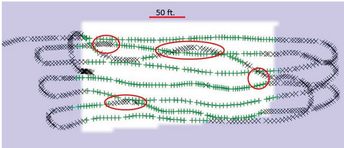
Figure 9. Position and dye flow (discharge) status for SE plot in Lake Underhill, FL, 10 February 2016, superimposed on treatment mask (white is within plot, purple is outside plot). Green crosses indicate dye flow, while black X's indicate no dye flow. Red circled areas indicate treatment boat path overlap.
