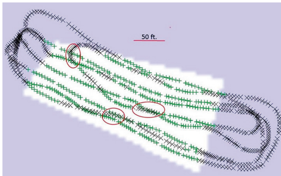
Figure 10. Position and dye flow (discharge) status for SW plot in Lake Underhill, FL, 10 February 2016, superimposed on treatment mask (white is within plot, purple is outside plot). Green crosses indicate dye flow, while black X's indicate no dye flow. Red circled areas indicate treatment boat path overlap.
