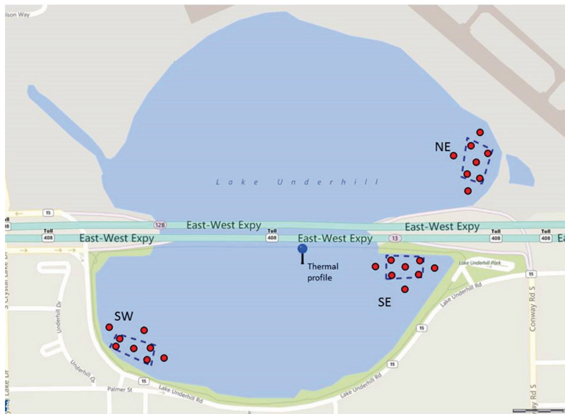
Figure 7. Sampling locations for dye measurements on Lake Underhill, FL, consisting of a combination of sites sampled by hand-held instrumentation and automated instrumentation fixed at the center of each plot.
