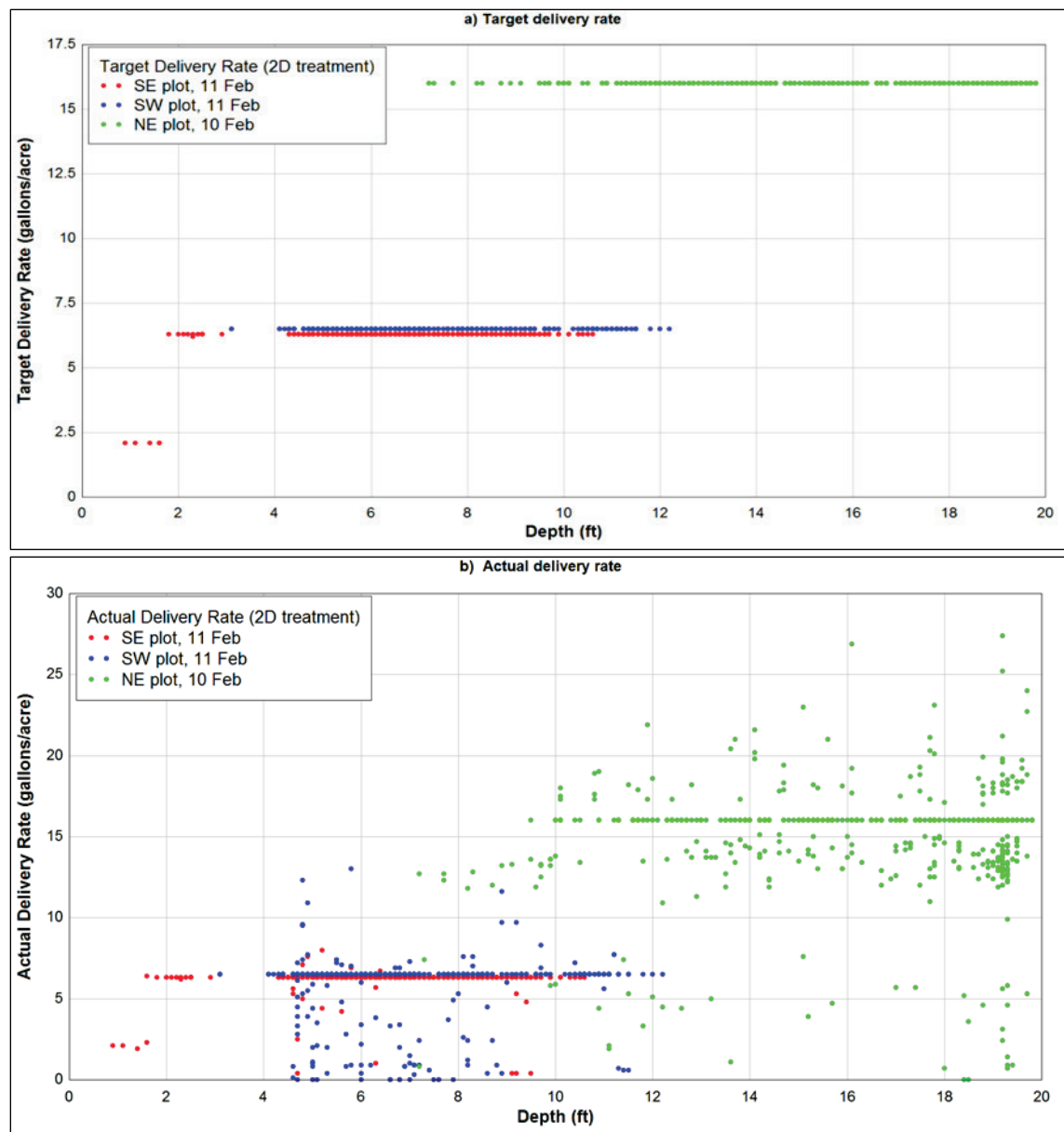
Figure 12. Target (a) and actual (b) delivery rate versus depth for 2-D delivery mode of dye for all 2-D treatments in Lake Underhill, FL, February 2016.
