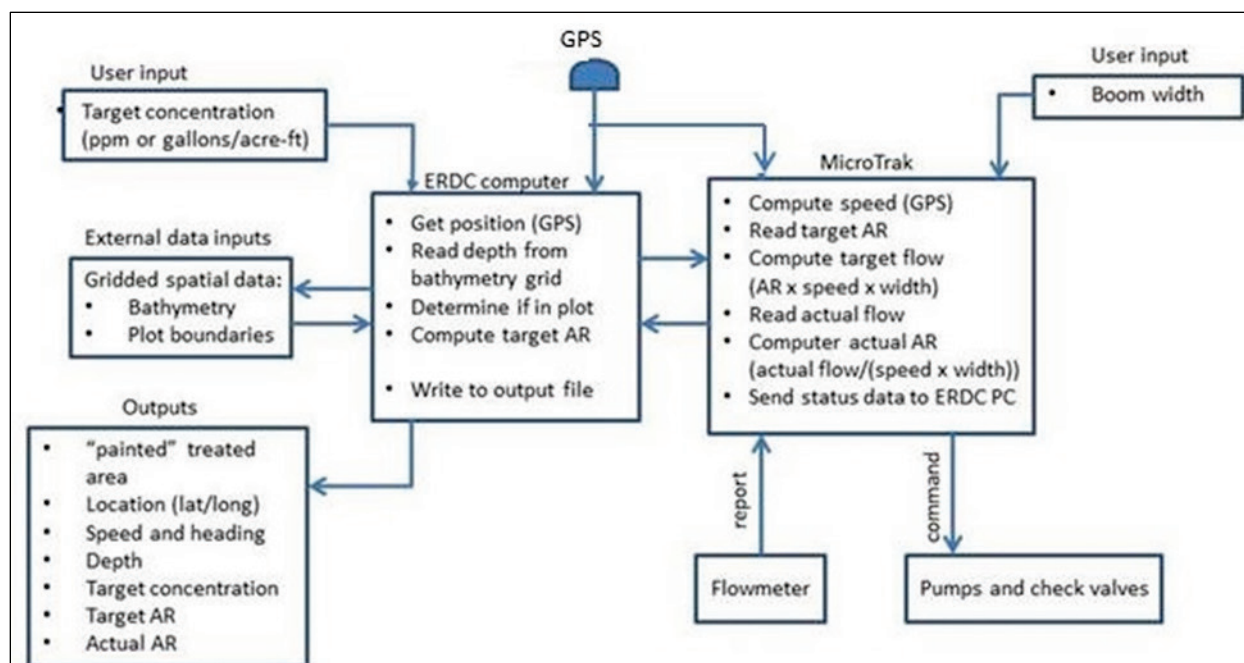
Figure 3. Electronic control, computations, and data management of entire 3-D system with PC enhancements.
