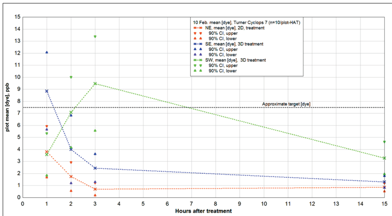
Figure 15. Mean of dye concentration measurements (Turner Cyclops 7) in treated plots in Lake Underhill, FL, 10 February 2016.
