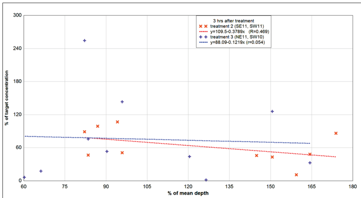
Figure 19. Plot of normalized depth vs. normalized dye concentration for treatments in Lake Underhill, FL, three hours after releasing dye.
