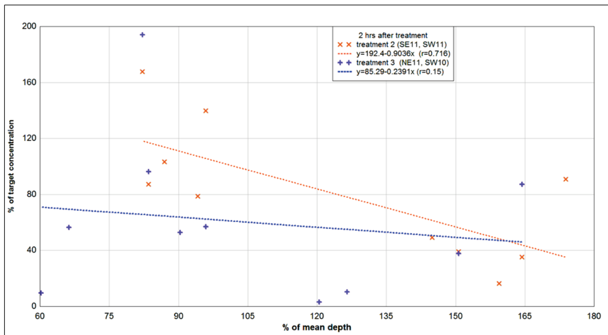
Figure 18. Plot of normalized depth vs. normalized dye concentration for treatments in Lake Underhill, FL, two hours after releasing dye.
