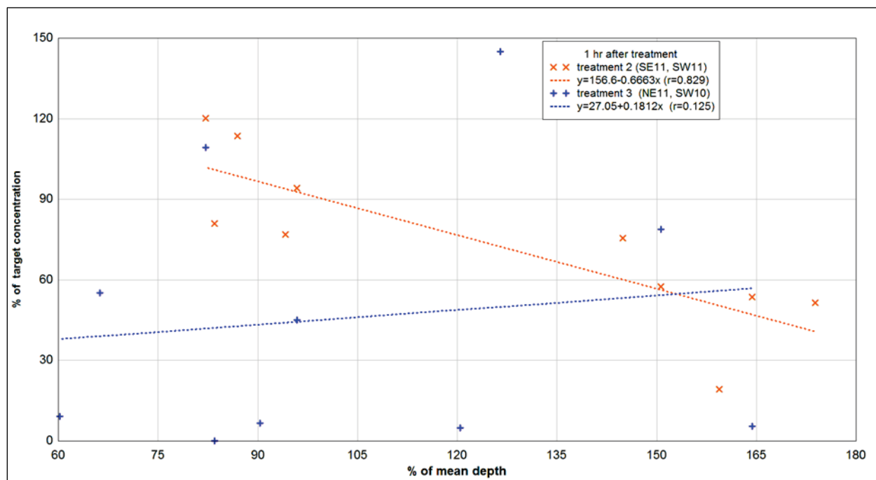
Figure 17. Plot of normalized depth vs. normalized dye concentration for treatments in Lake Underhill, FL, one hour after releasing dye.
