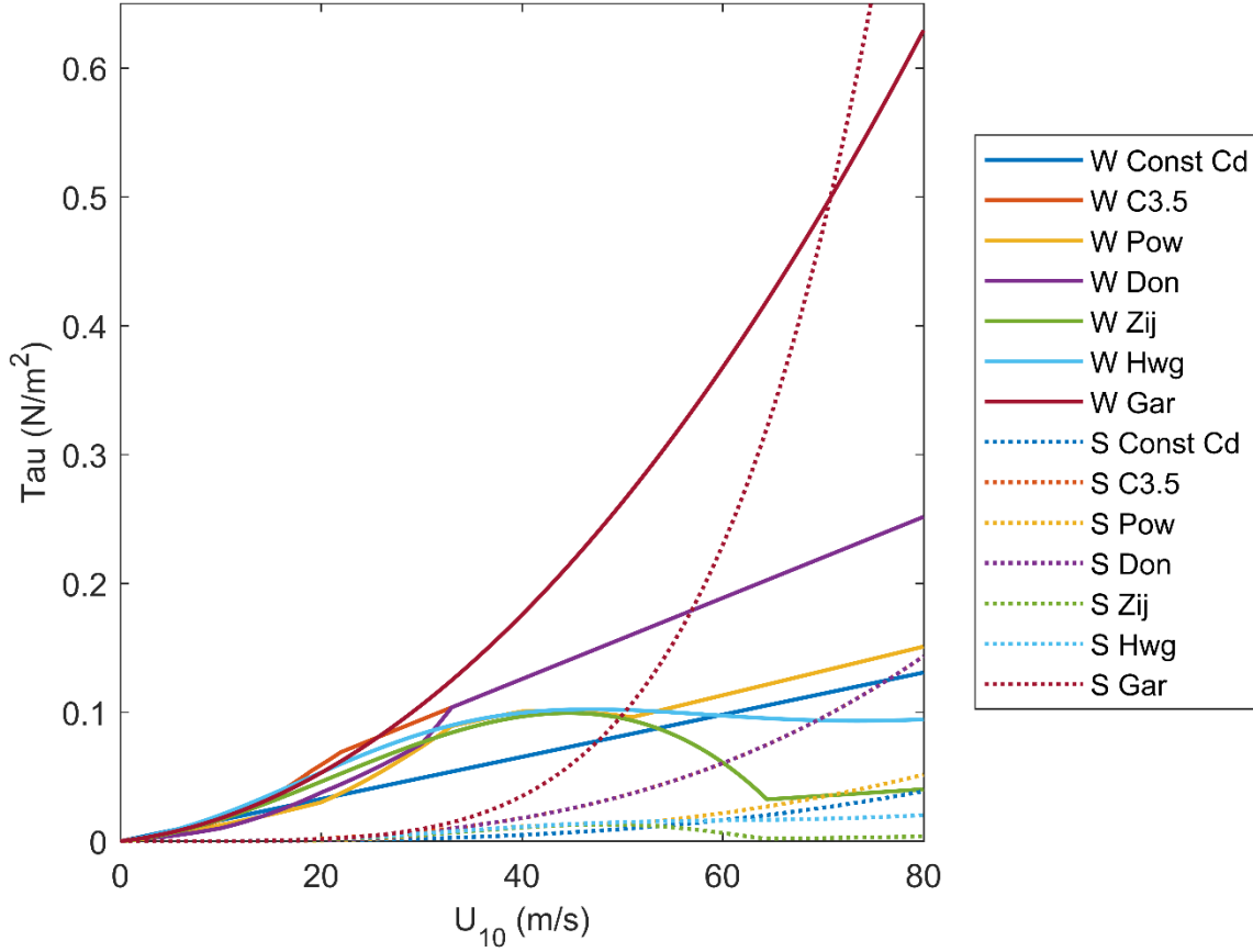
Figure 3-1: Separated wind ( \tau_w ) and spray stresses ( \tau_{sp} ) [ \text{N/m}^2 ] vs. wind speed ( U_{10} ) [ \text{m/s} ] for all C_D parameterizations discussed in Section 2.2 and used in this study. Solid and dotted lines represent modeled output with wind-only (“W”) ( \tau_w ) and spray-only (“S”) \tau_{sp} forcing respectively.
