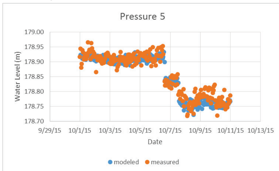
Figure 32. Validation plot pressure sensor 5 (S/N 9858765).
