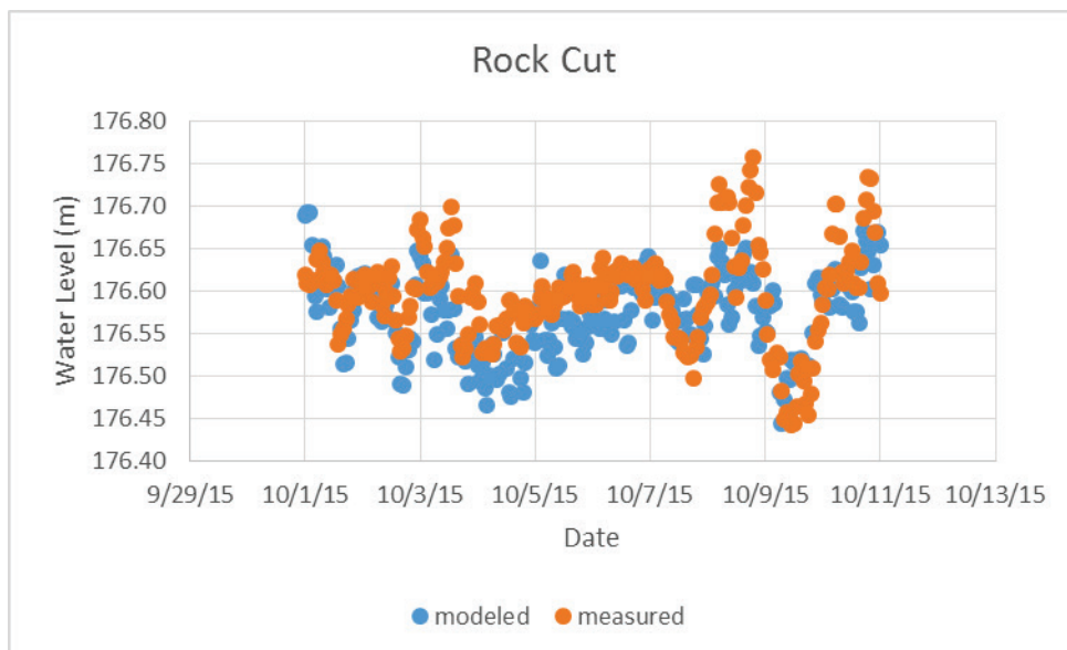
Figure A- 33. Calibration plot for Rock Cut NOAA.
