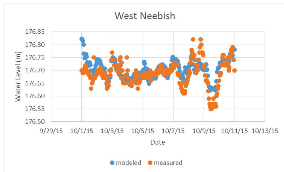
Figure A- 31. Calibration plot for West Neebish NOAA.
