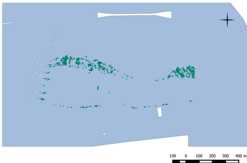
Lake Sturgeon - Habitat Suitable for egg survival in 2015 Deviation scenario
