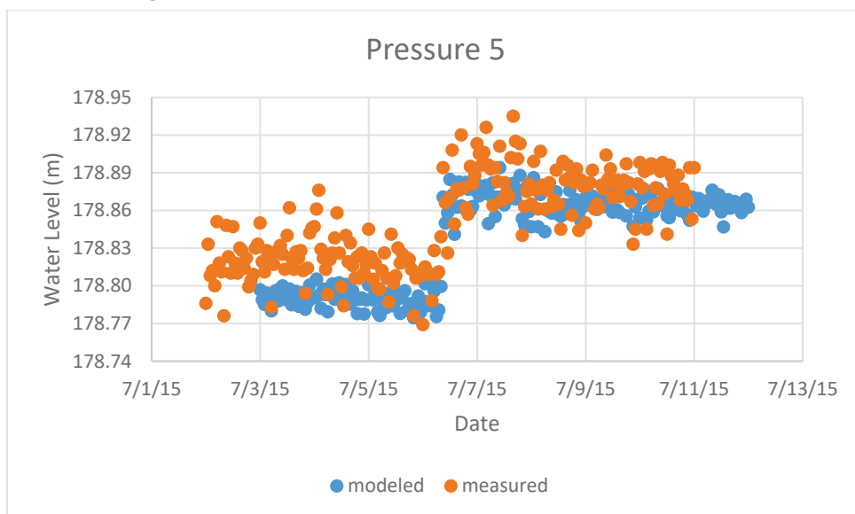
Figure 20. Calibration plot pressure sensor 5 (S/N 9858765).
