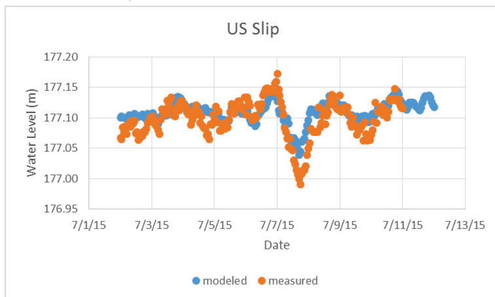
Figure A- 12. Calibration plot for U.S. Slip NOAA.
