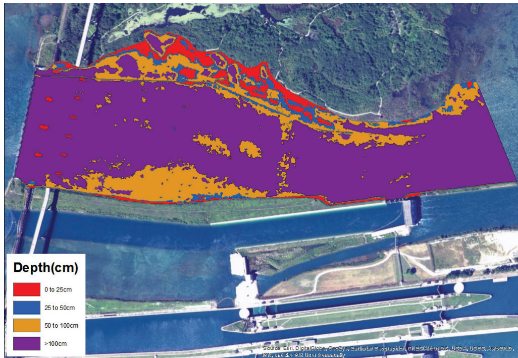
Figure 56. Depth map, Run 15-18.
