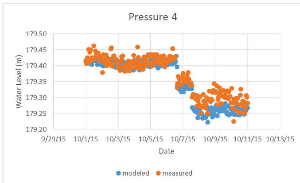
Figure 31. Validation plot pressure sensor 4 (S/N 10662591).
