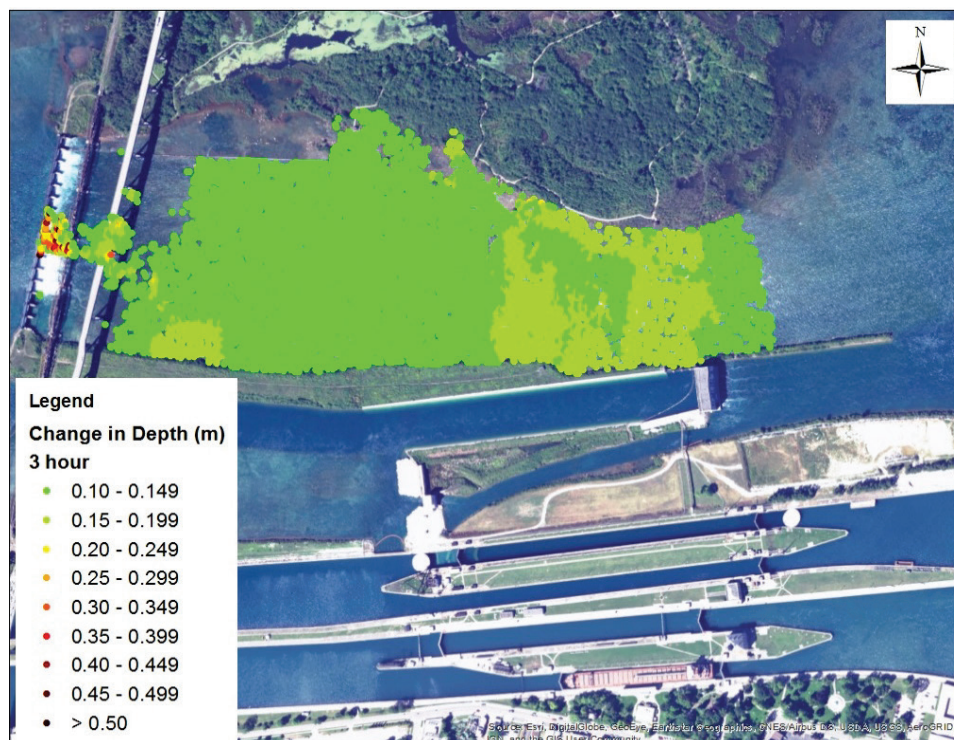
Figure 39. Water level rate of change from one-half gate setting to an approximate three gate setting for a gate opening occurring over a 3-hour period on 1 May 2015.
