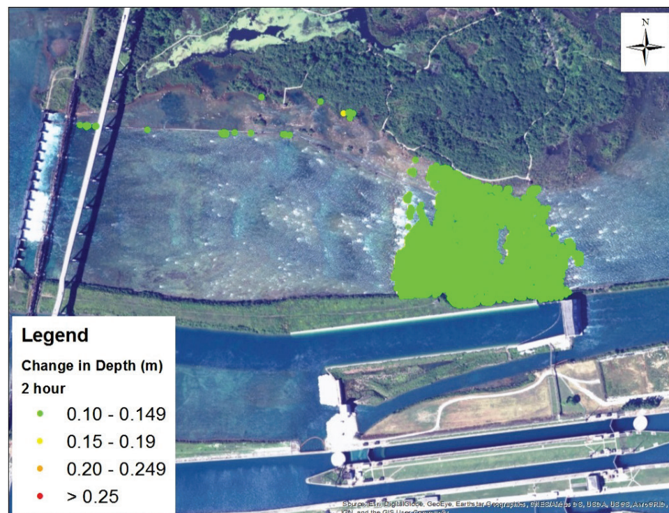
Figure 43. Water level rate of change from a 71 cm setting to an 89 cm gate opening occurring over a two hour period on 14 July 2015.
