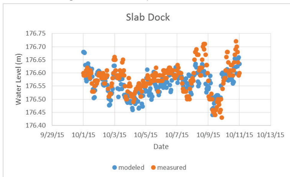
Figure A- 32. Calibration plot for Slab Dock USACE.
