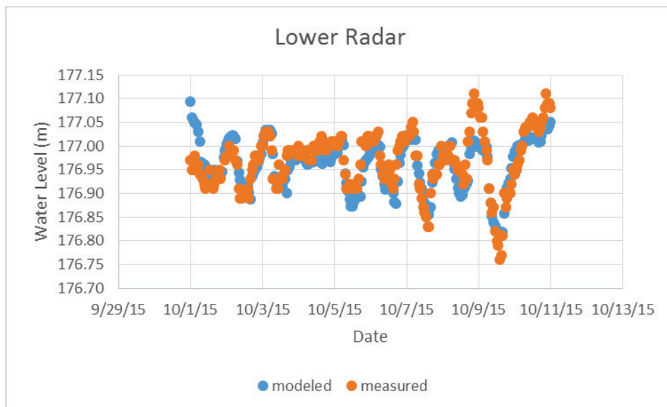
Figure A- 27. Calibration plot for Lower Radar USACE.
