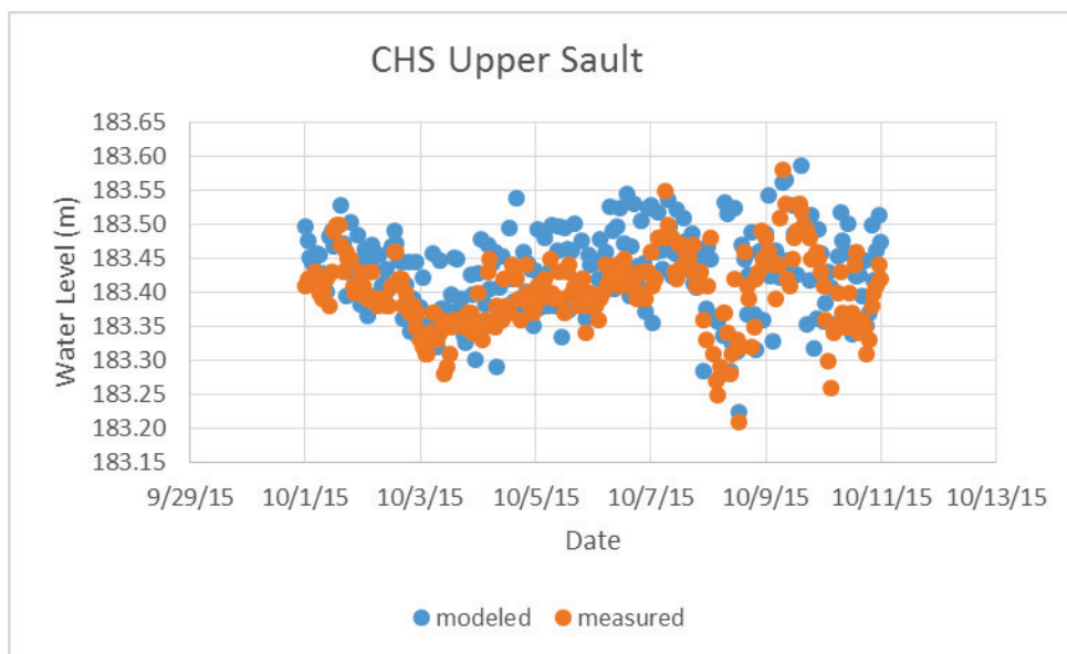
Figure 27. Validation plot, above the locks CHS (10980).
