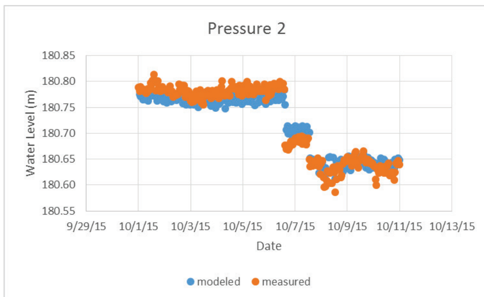
Figure 29. Validation plot pressure sensor 2 (S/N 10351961).
