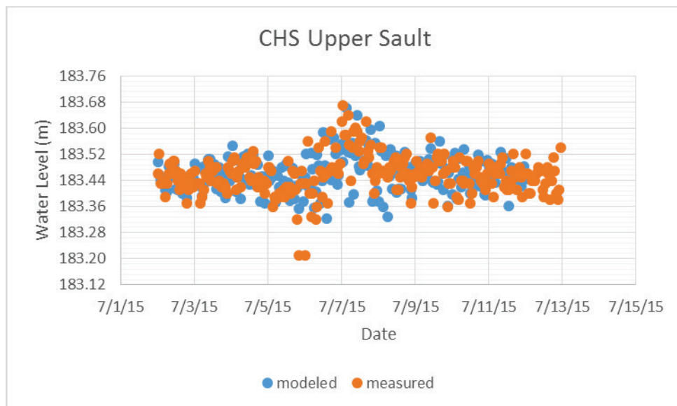
Figure A- 3. Calibration plot for Upper Sault CHS.
