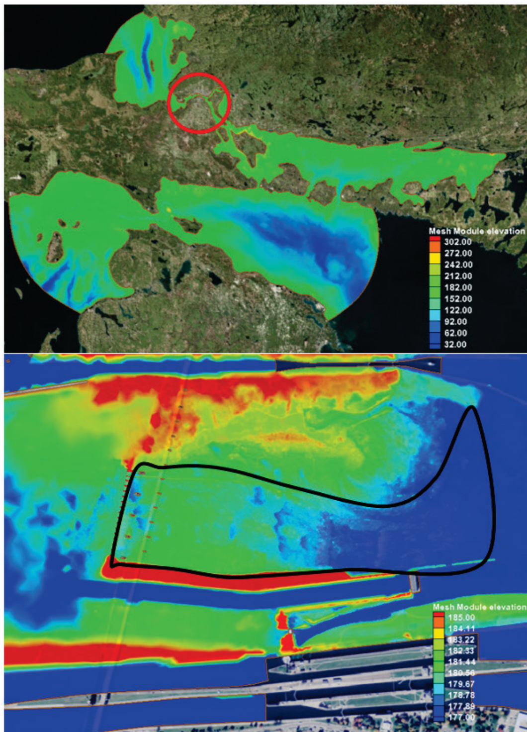
Figure 13. The Adaptive Hydraulics model domain for the St. Marys River with colored bathymetry (top; project area circled) and the rapids outlined (bottom; black line).
