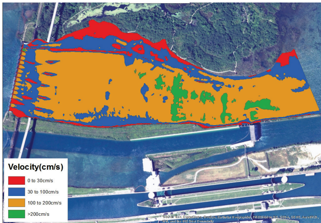
Figure 57. Velocity map, Run15-18.
