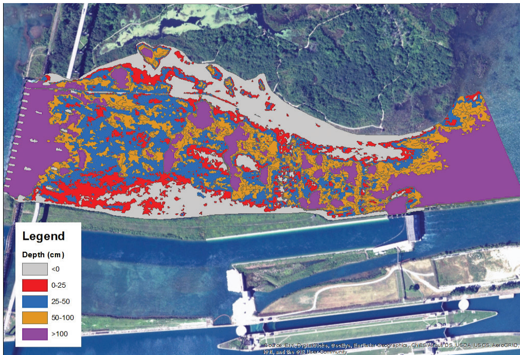
Figure 44. Depth map, Run 15-1.
