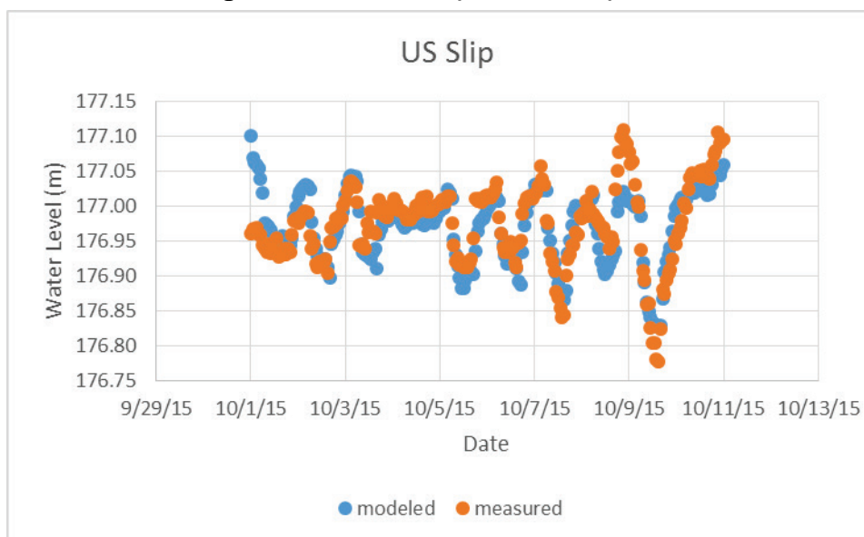
Figure A- 28. Calibration plot for U.S. Slip NOAA.
