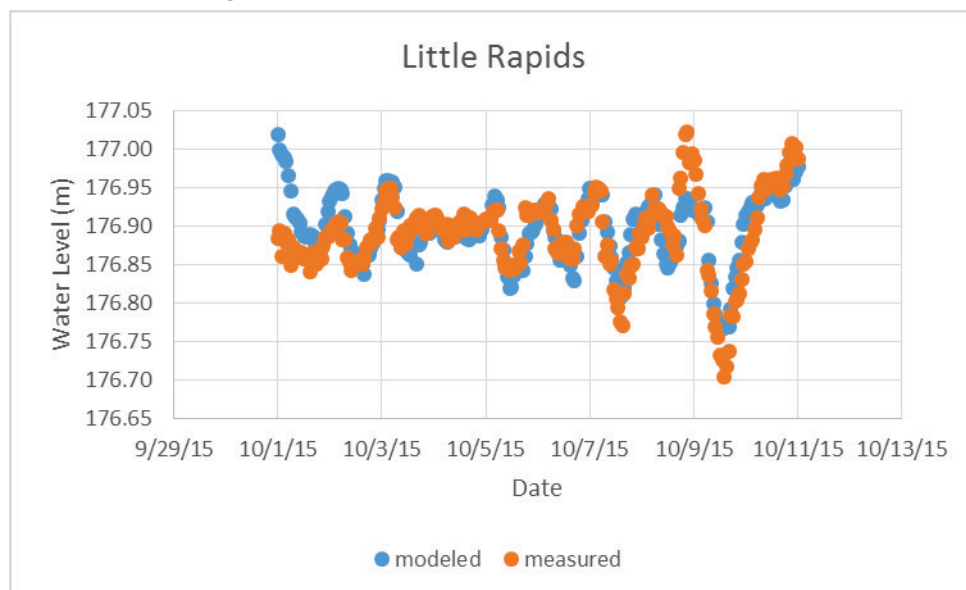
Figure A- 29. Calibration plot for Little Rapids NOAA.
