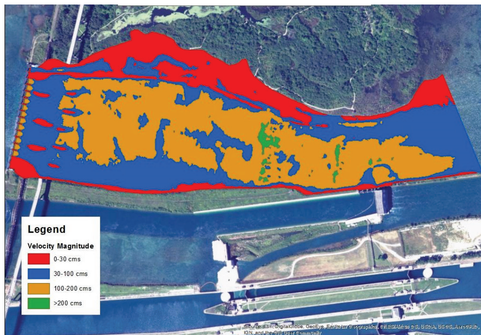
Figure 48. Velocity map, Run 15-2.
