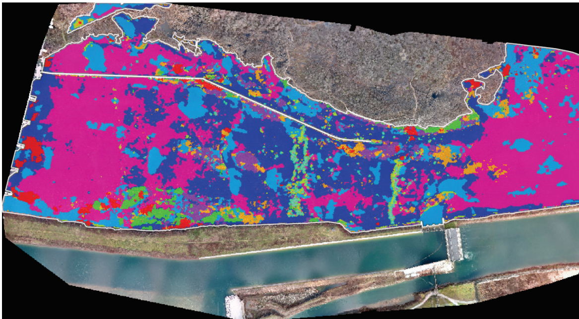
Figure 12. Map of the k-means clustering obtained from the texture descriptors developed in this study. Least squares were calculated on the basis the Mahalanobis distance. The nine groups are shown with different colors. Zones with the same color are similar in surface roughness.
