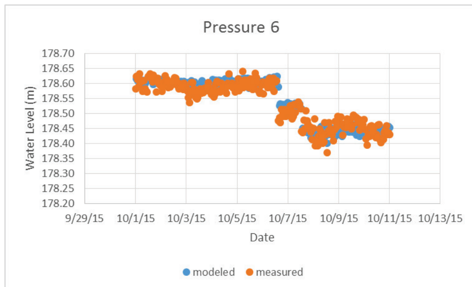
Figure A- 25. Calibration plot for Pressure Sensor 6 USACE.
