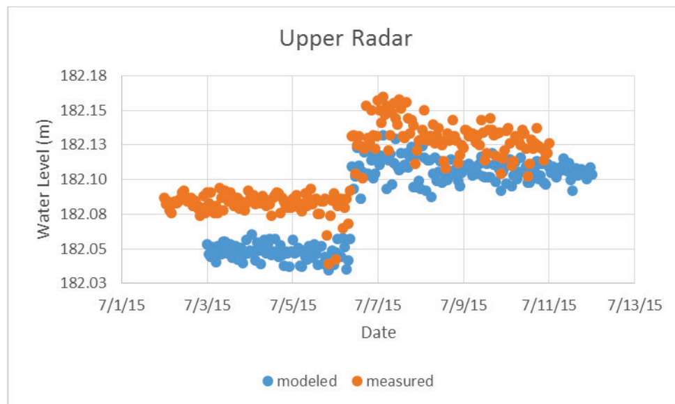
Figure 16. Calibration plot upper rapids radar.
