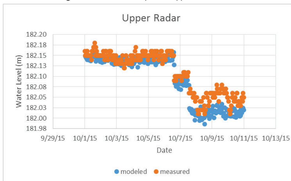
Figure A- 22. Calibration plot for Upper Radar USACE.
