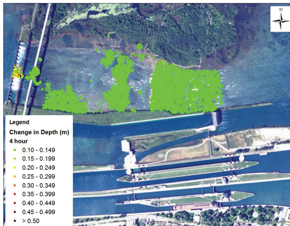
Figure 40. Water level rate of change from one-half gate setting to an approximate three gate setting for a gate opening occurring over a 4-hour period on 1 May 2015.
