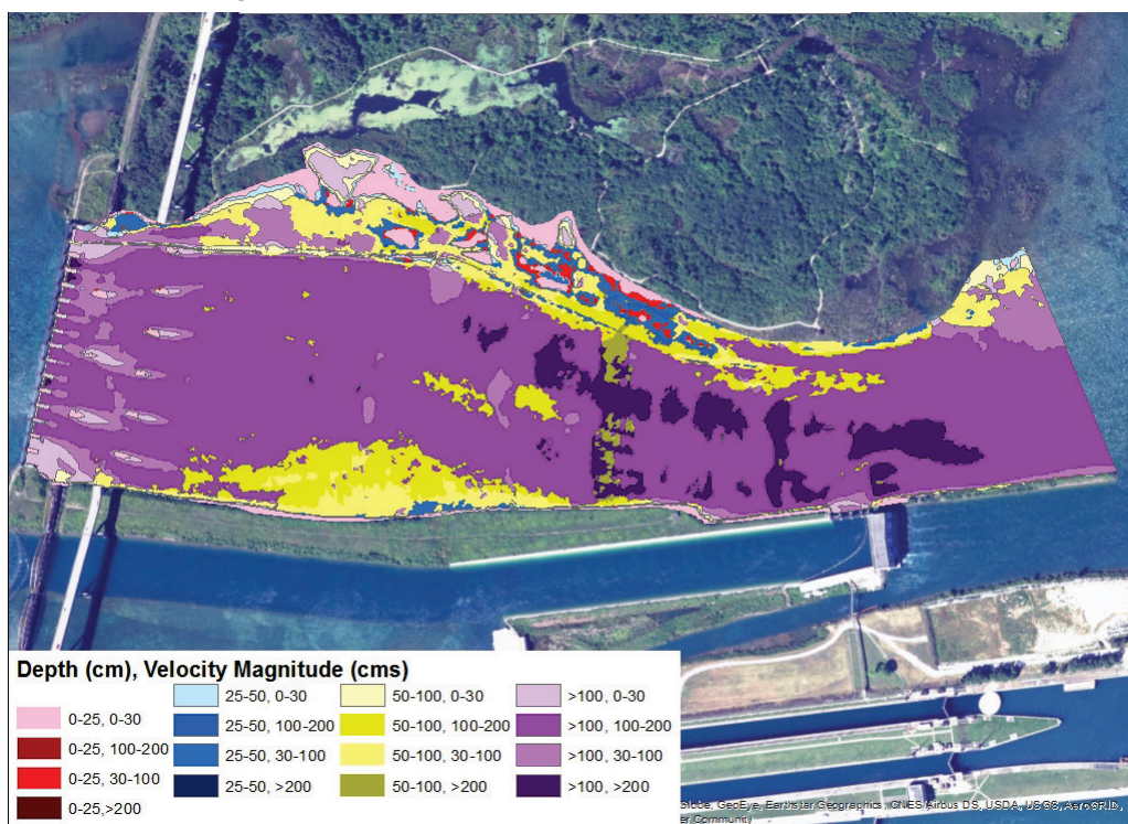
Figure 52. Depth and velocity intersection map, Run 15-5.
