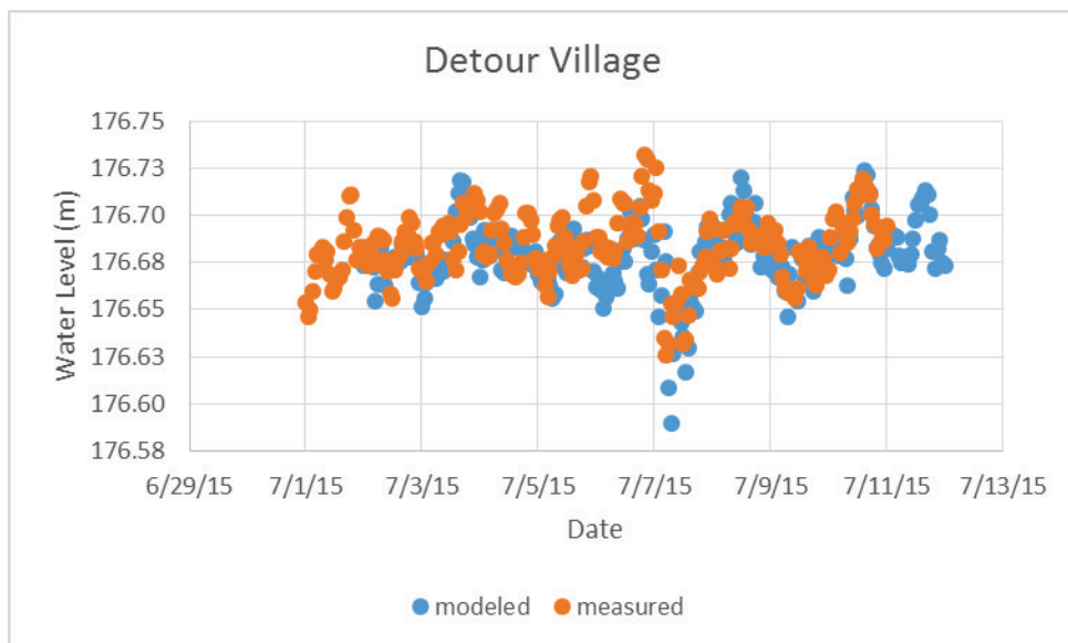
Figure A- 18. Calibration plot for Detour Village NOAA.
