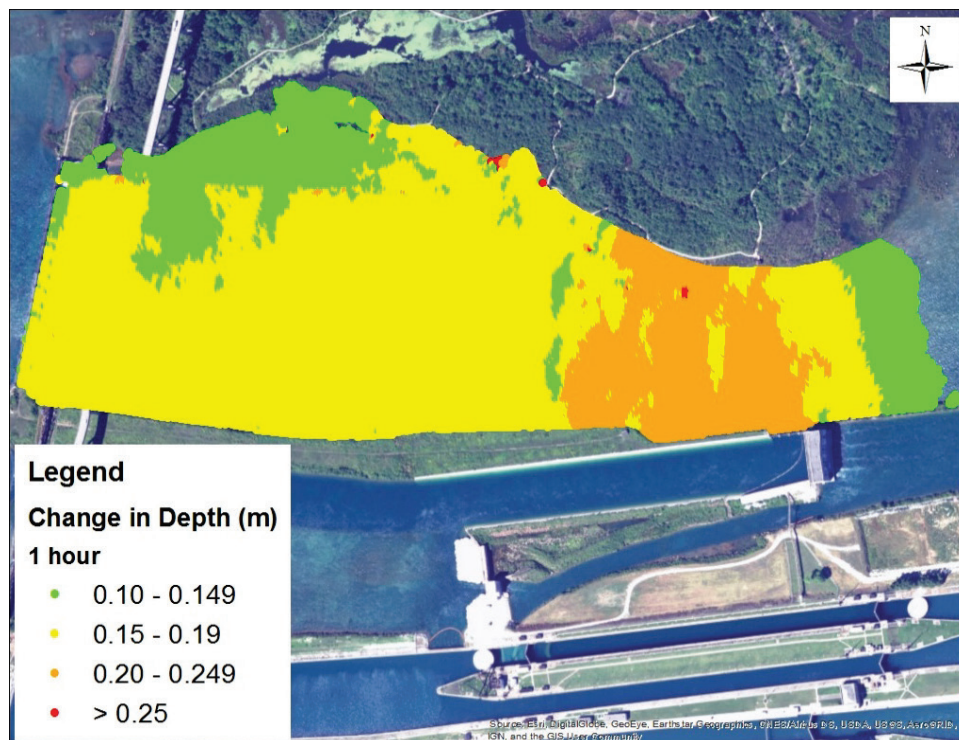
Figure 42. Water level rate of change from 71 cm setting to an 89 cm gate opening occurring over a one hour period on 14 July 2015.
