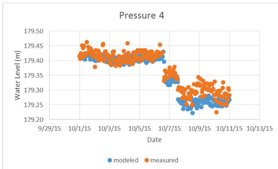
Figure A- 24. Calibration plot for Pressure Sensor 4 USACE.
