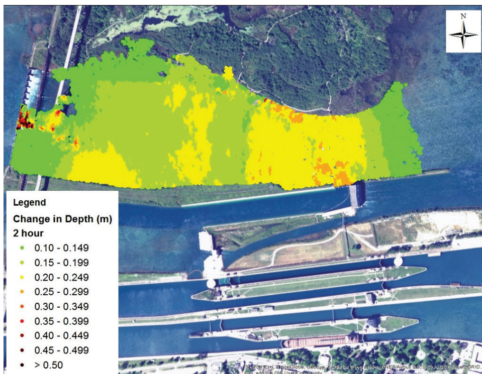
Figure 38. Water level rate of change from one-half gate setting to an approximate three gate setting for a gate opening occurring over a 2-hour period on 1 May 2015.
