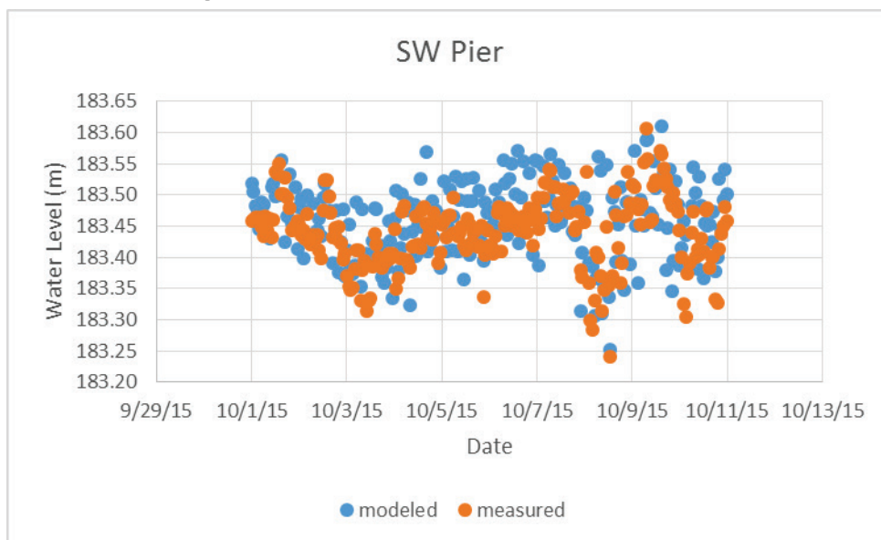
Figure 26. SW Pier validation plot NOAA (9076070).
