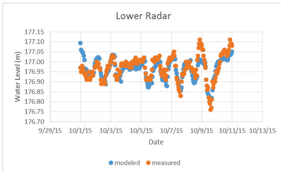
Figure 35. Validation plot lower rapids radar.
