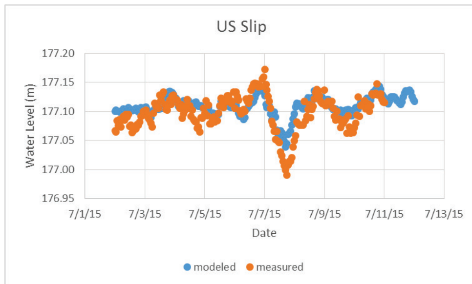
Figure 24. Calibration plot U.S. Slip NOAA (9076060).
