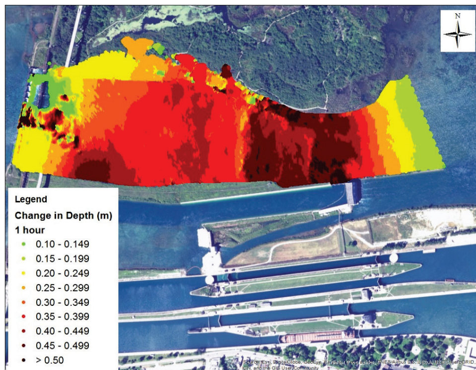
Figure 37. Water level rate of change from one-half gate setting to an approximate three gate setting over a 1-hour period on 1 May 2015.
