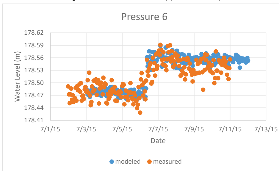
Figure 21. Pressure Sensor 6 (S/N 10662592).
