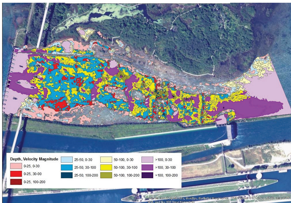
Figure 46. Depth and velocity intersection map, Run 15-1.
