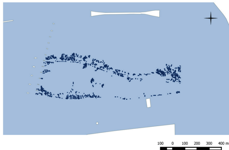
Lake Sturgeon - Habitat Suitable for spawning in 2015 Deviation scenario
