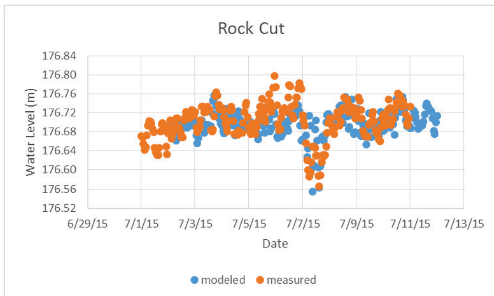
Figure A- 17. Calibration plot for Rock Cut NOAA.
