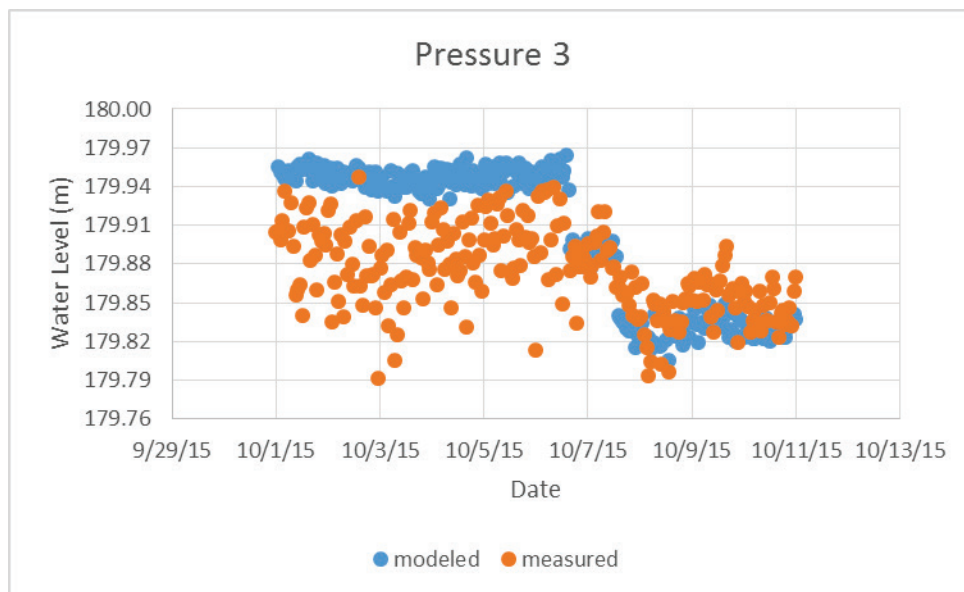
Figure 30. Validation plot pressure sensor 3 (S/N 9870920).
