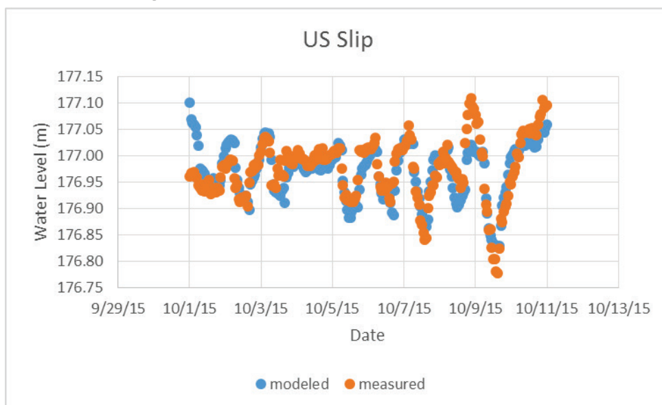
Figure 36. Validation plot U.S. slip NOAA (9076060).
