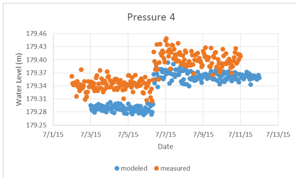
Figure 19. Calibration plot press sensor 4 (S/N 10662591).
