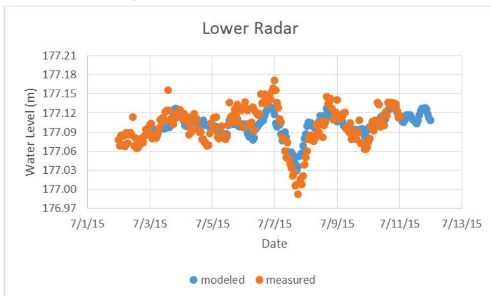
Figure 23. Calibration plot lower rapids radar.
