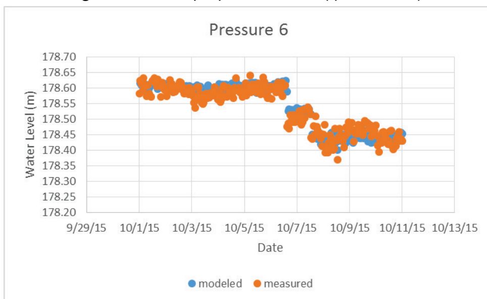
Figure 33. Validation plot pressure sensor 6 (S/N 10662592).
