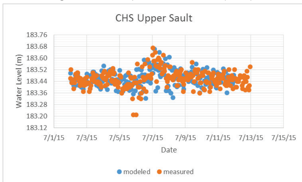
Figure 15. Calibration plot Above the Locks CHS (10980).
