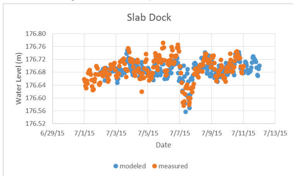
Figure A- 16. Calibration plot for Slab Dock USACE
