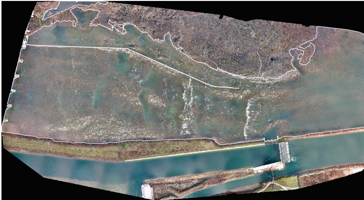
Figure 10. Compound image obtained from multiple aerial pictures taken from an UAS flying over a trans-border stretch of the St. Marys River, located north of Edison Sault Hydroelectric Plant (Michigan, USA; +45.5062,-84.3493). Dimensions (x × y): 1197 m × 659 m.
