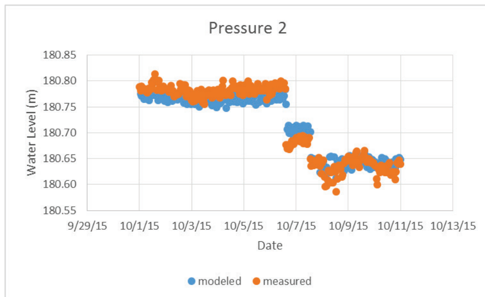
Figure A- 24. Calibration plot for Pressure Sensor 2 USACE.
