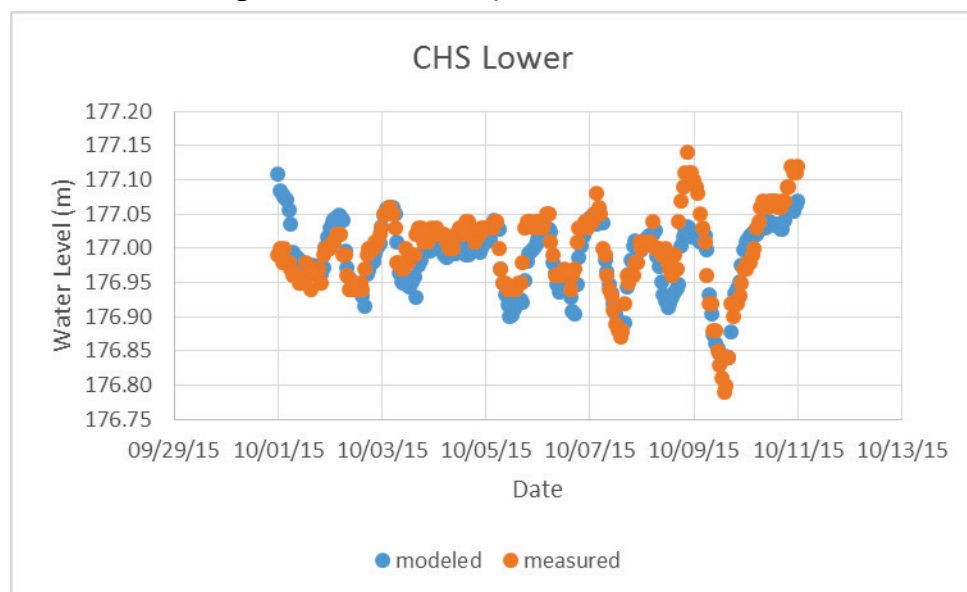
Figure A- 26. Calibration plot for Lower Sault CHS.
