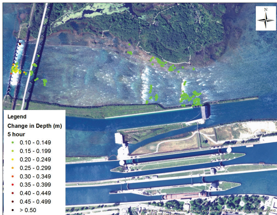
Figure 41. Water level rate of change from one-half gate setting to an approximate three gate setting for a gate opening occurring over a 5-hour period on 1 May 2015.
