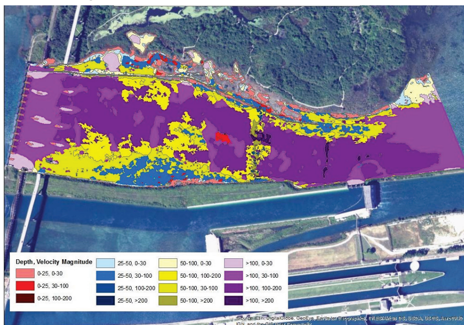
Figure 49. Depth and velocity intersection map, Run 15-2.
