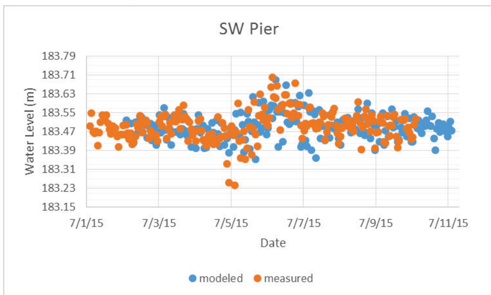
Figure A- 2. Calibration plot for SW Pier NOAA.
