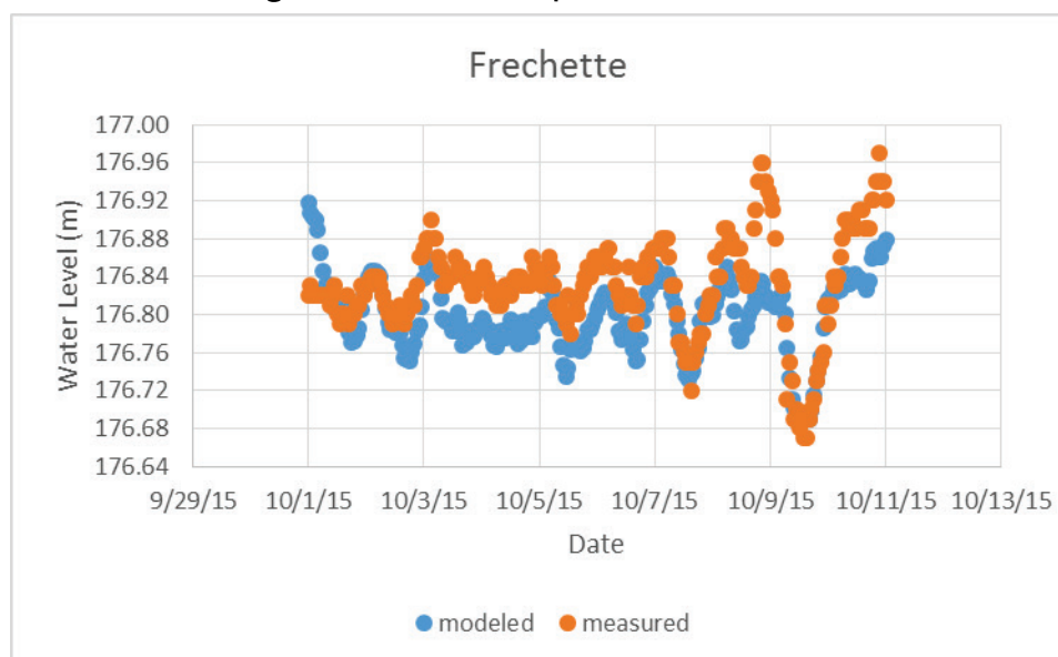
Figure A- 30. Calibration plot for Frechette NOAA.
