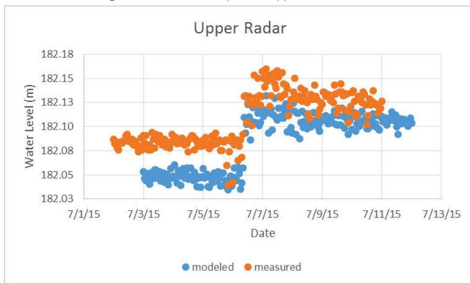
Figure A- 4. Calibration plot for Upper Radar USACE.
