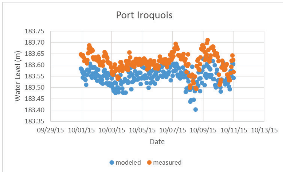
Figure A- 20. Validation plot for Point Iroquois NOAA.
