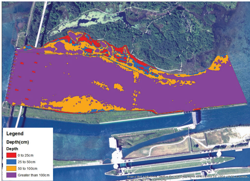
Figure 50. Depth map, Run 15-5.
