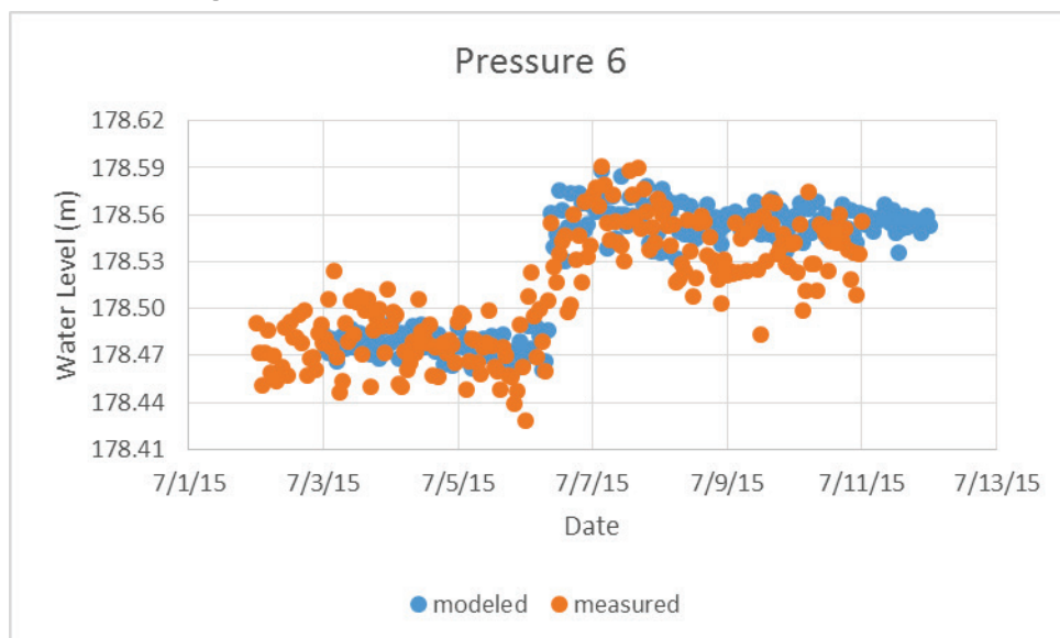
Figure A- 9. Calibration plot for Pressure Sensor 6 USACE.
