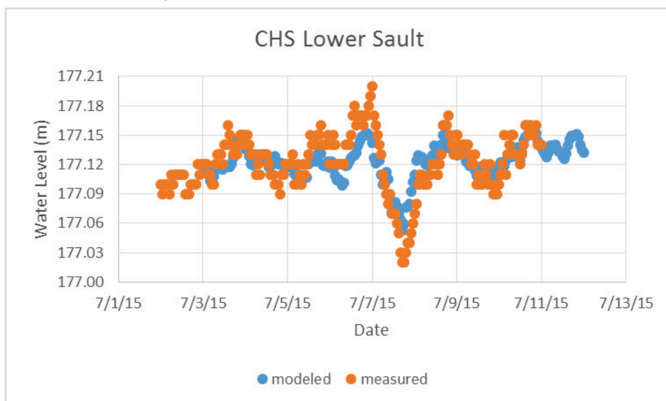
Figure A- 10. Calibration plot for Lower Sault CHS.
