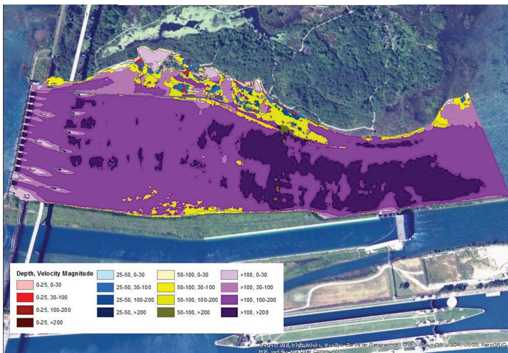
Figure 55. Depth and velocity intersection map, Run 15-12.
