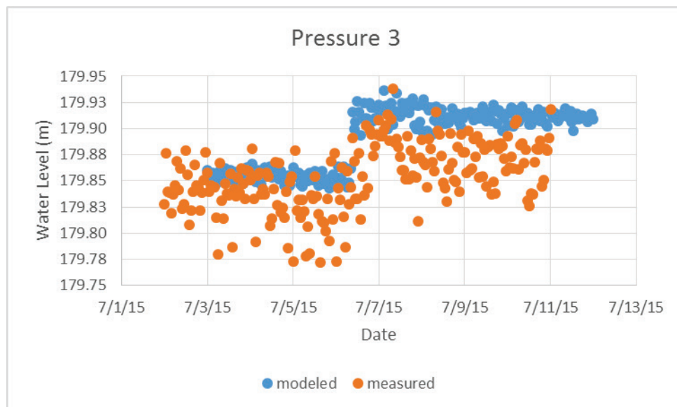
Figure 18. Calibration plot pressure sensor 3 (S/N 9870920).
