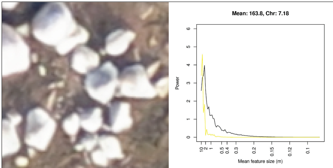
Figure 11. Left- Image of rough substrate (metric boulders). Right - Power spectrum of pixel intensity (black line). Right - Chromatic variability (yellow line) calculated using a window with N=112 (resolution: 0.04455 m, window width: 4.990 m).
