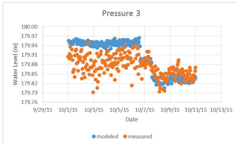
Figure A- 23. Calibration plot for Pressure Sensor 3 USACE.
