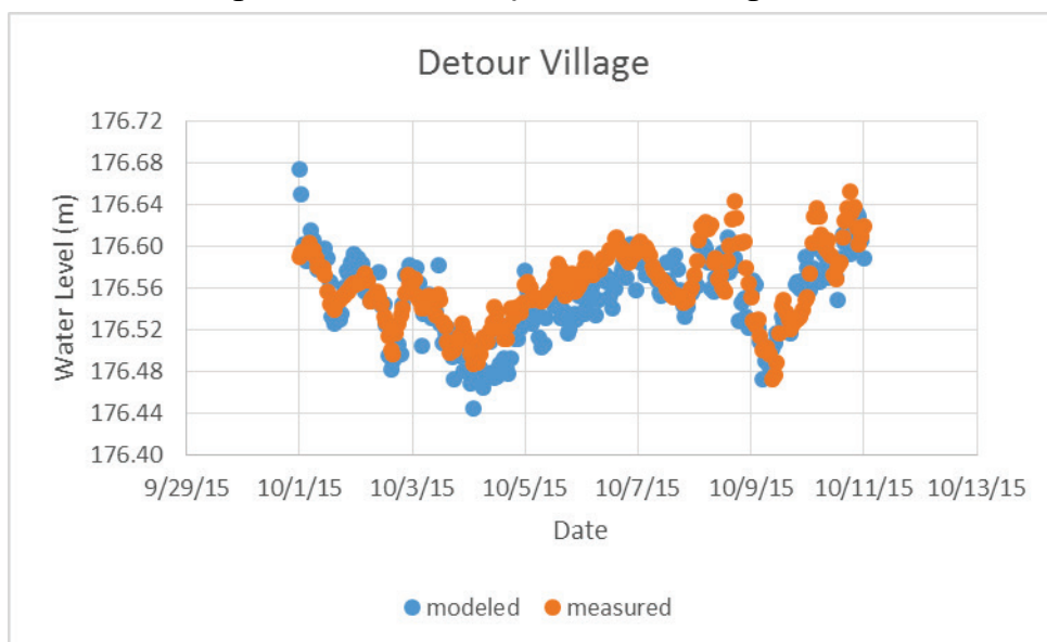
Figure A- 37. Calibration plot for Detour Village NOAA.
