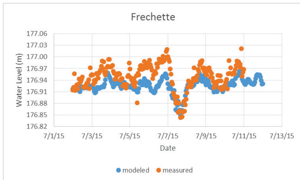
Figure A- 14. Calibration plot for Frechette NOAA.
