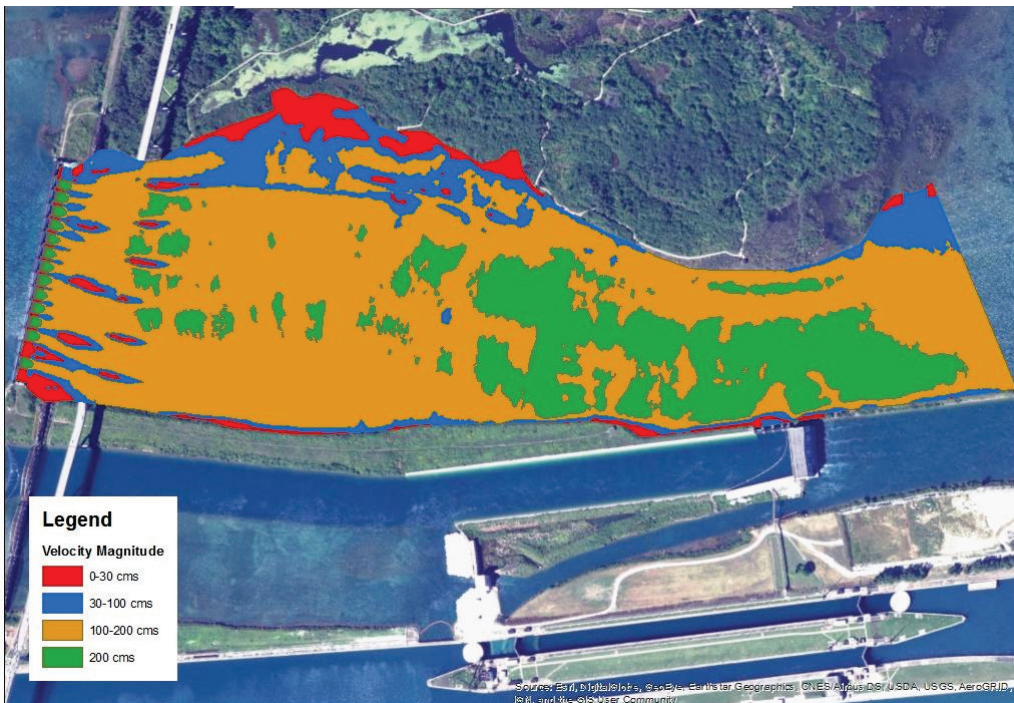
Figure 54. Velocity map, Run 15-12.
