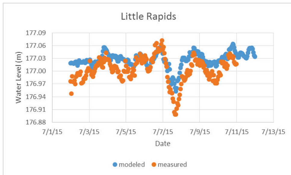
Figure A- 13. Calibration plot for Little Rapids.
