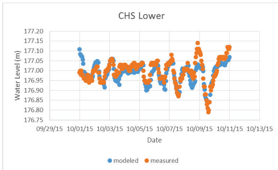
Figure 34. Validation graph CHS gauge below the locks (11010).
