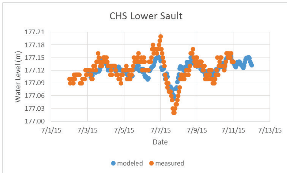
Figure 22. CHS gauge below the locks (11010).
