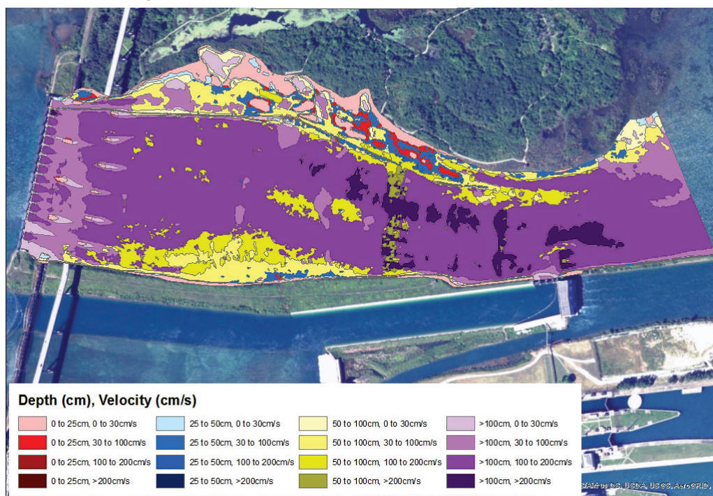
Figure 58. Depth and velocity intersection map, Run 15-18.
