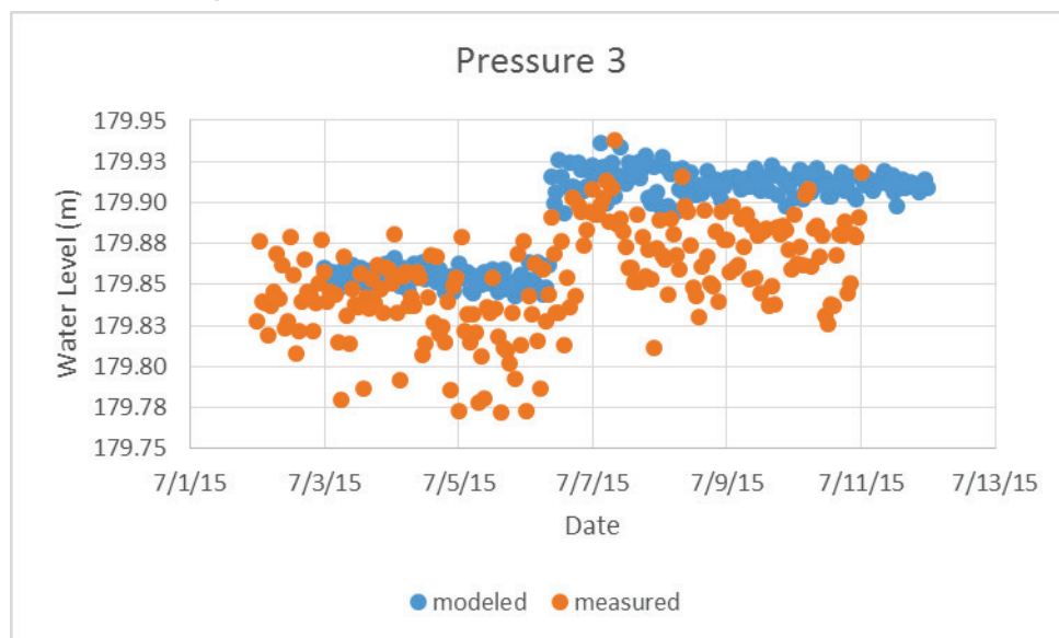
Figure A- 6. Calibration plot for Pressure Sensor 3 USACE.
