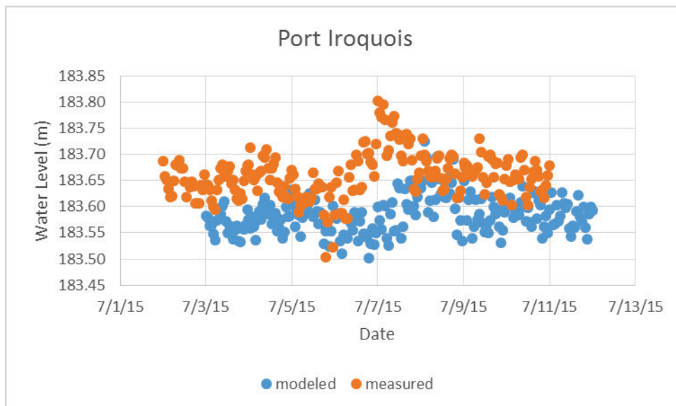
Figure A- 1. Calibration plot for Point Iroquois NOAA.
