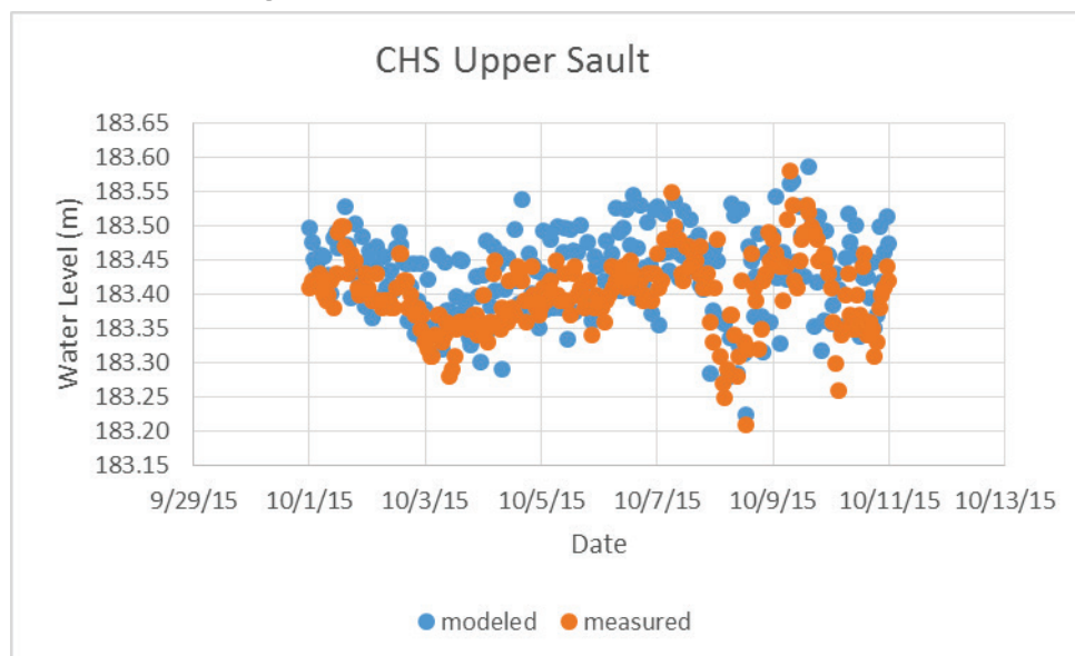
Figure A- 21. Calibration plot for Upper Sault CHS.
