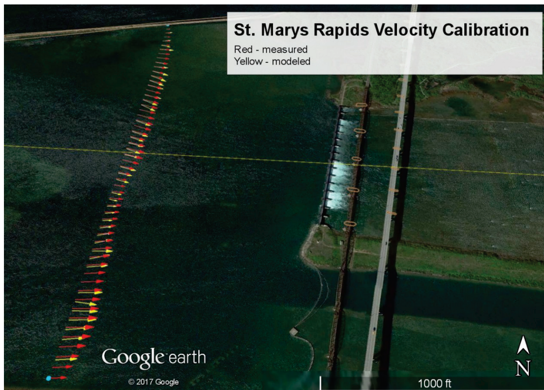
Figure 25. Velocity comparison 13 July 2017 at 1700 hours upstream of the St. Marys River Comp Works.
