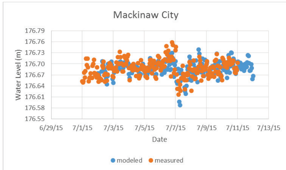
Figure A- 19. Calibration plot for Mackinaw City NOAA.
