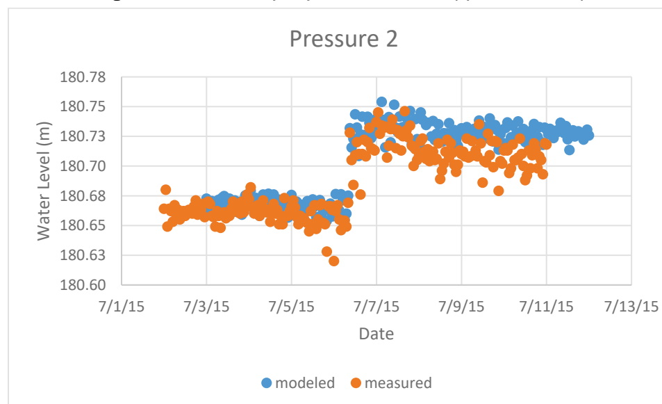
Figure 17. Calibration plot pressure sensor 2 (S/N 10351961).
