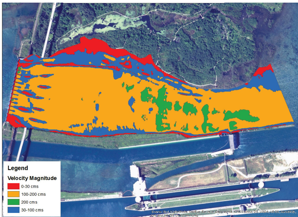
Figure 51. Velocity map, Run 15-5.
