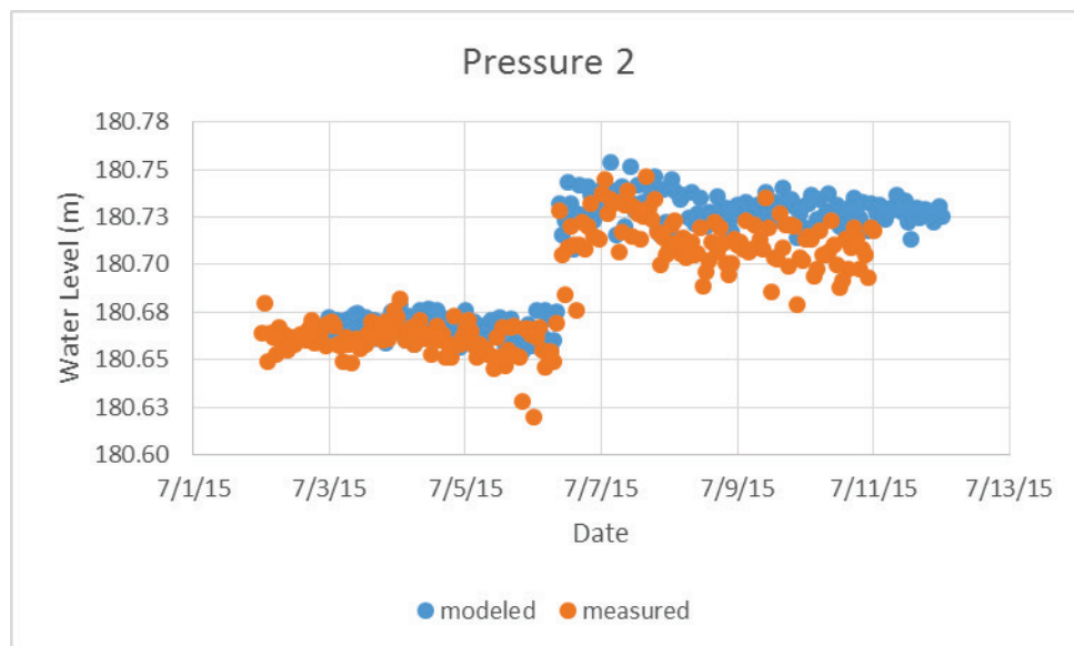
Figure A- 5. Calibration plot for Pressure Sensor 2 USACE.
