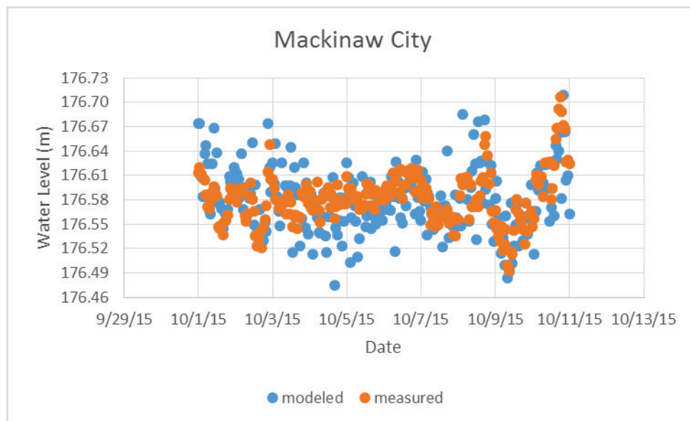
Figure A- 34. Calibration plot for Mackinaw City NOAA.
