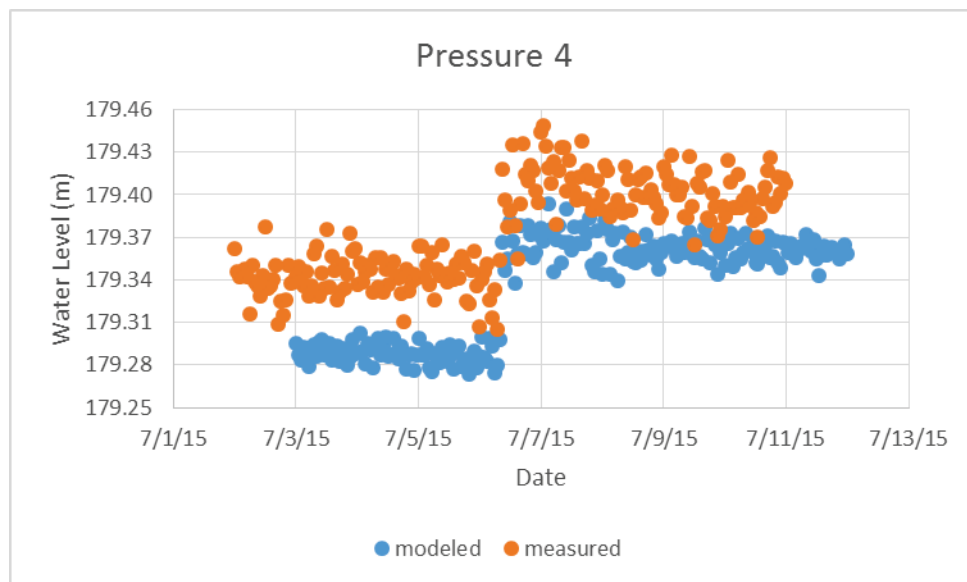
Figure A- 7. Calibration plot for Pressure Sensor 4 USACE.
