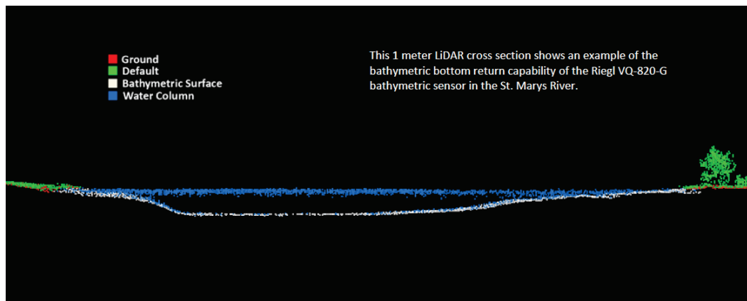
Figure 8. Typical cross section showing column surface (blue), channel bottom (white) and vegetation (green) high resolution bathymetry results obtained during the LiDAR survey.
