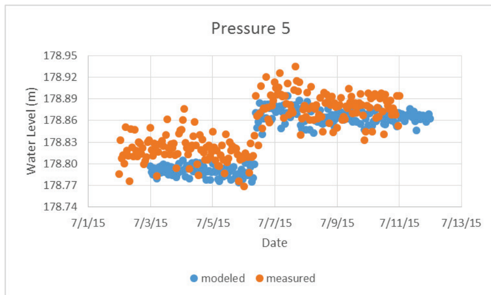
Figure A- 8. Calibration plot for Pressure Sensor 5 USACE.
