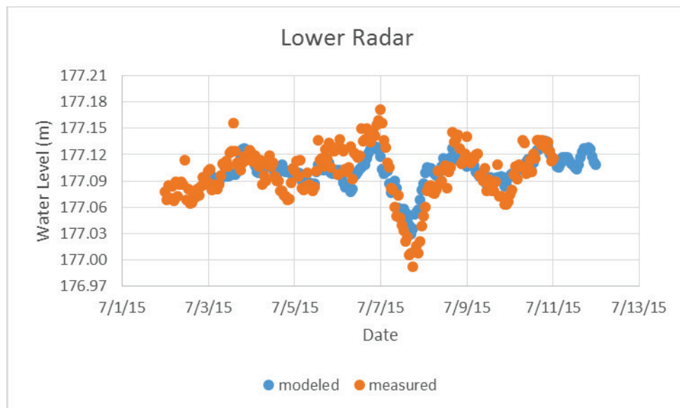
Figure A- 11. Calibration plot for Lower Radar USACE.
