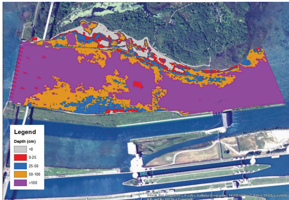
Figure 47. Depth map, Run 15-2.
