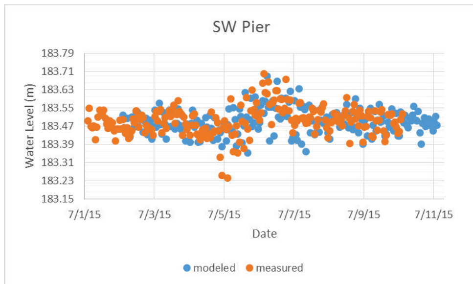
Figure 14. Calibration plot for SW Pier NOAA (9076070).
