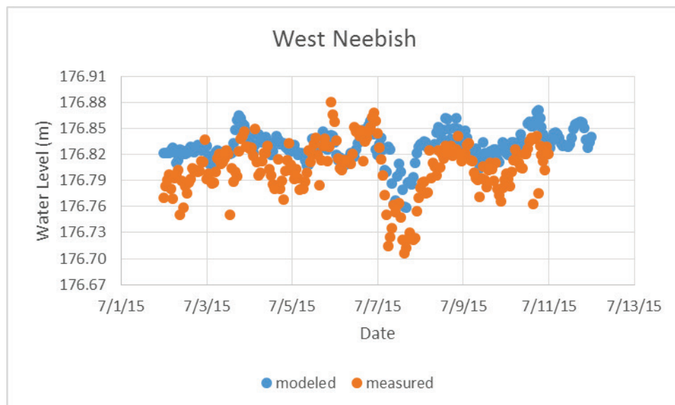
Figure A- 15. Calibration plot for West Neebish NOAA.
