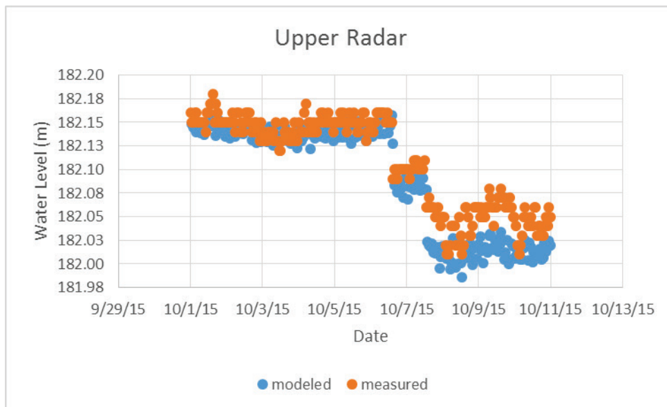
Figure 28. Validation plot upper rapids radar.
