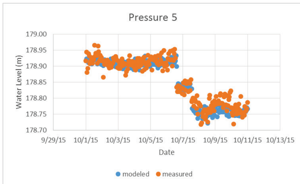
Figure A- 27. Calibration plot for Pressure Sensor 5 USACE.
