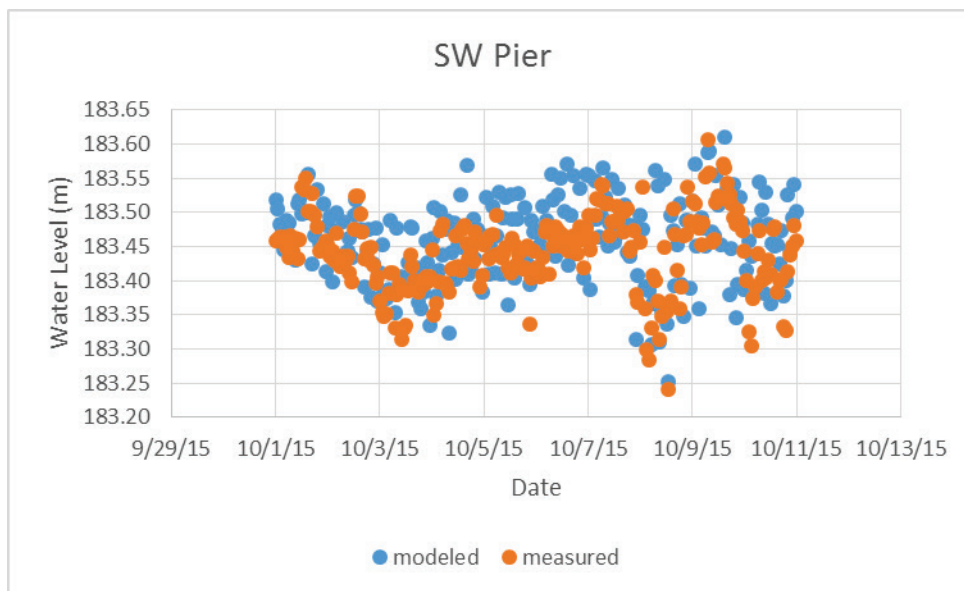
Figure A- 21. Calibration plot for SW Pier NOAA.
