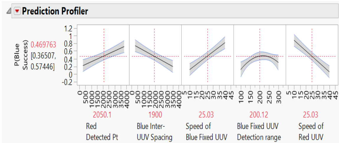
Figure 47 Prediction Profiler for Fixed Shooters
