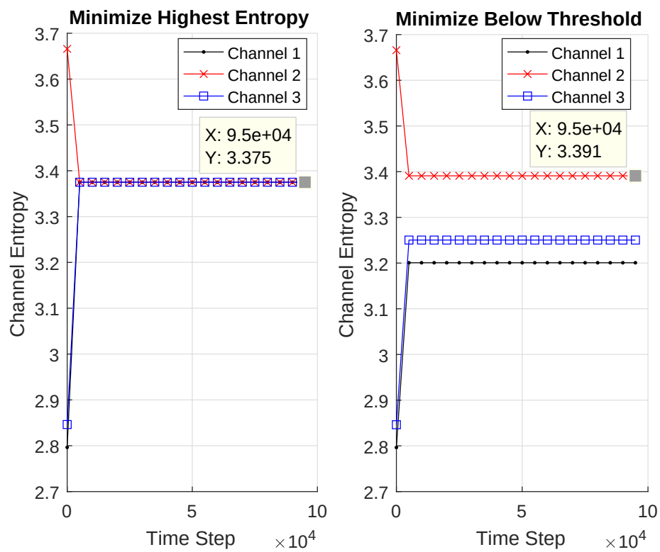
Figure 4.5: Highest entropy minimization for three channels.
