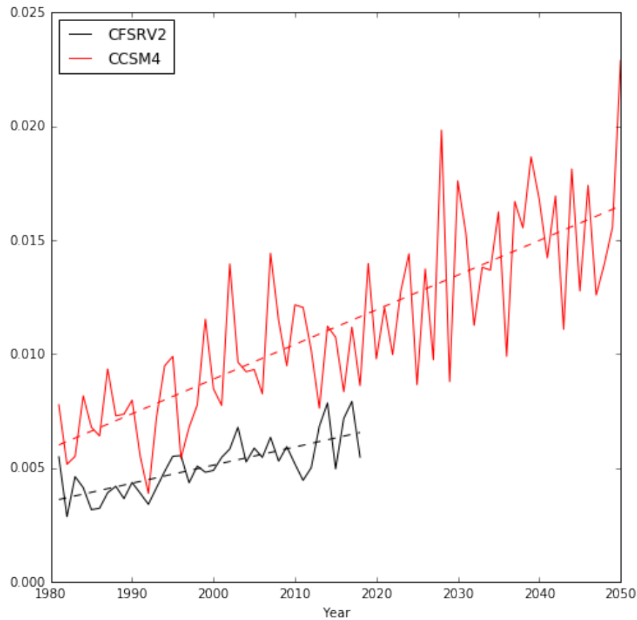
Figure 35. TC formation probabilities for the CFR for JASO 1981–2050 based on historical and projected information from CFSRV2 (black) and CCSM4 (red) with best fit trend lines (dashed).
