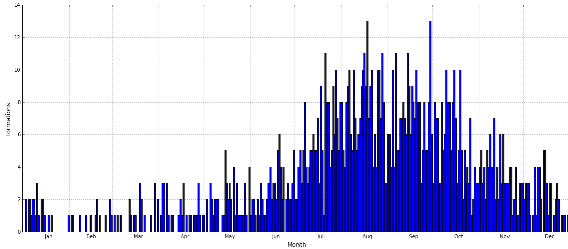
Figure 11. Number of TC formations (y-axis) for the WNP region by month (x-axis) during 1981–2018 for the WNP (100°E–180°E, 0°N–50°N). TC formation numbers from JTWC best track data for 1981–2017 and from NRL TC Page (NRL Monterey 2019) for 2018.
