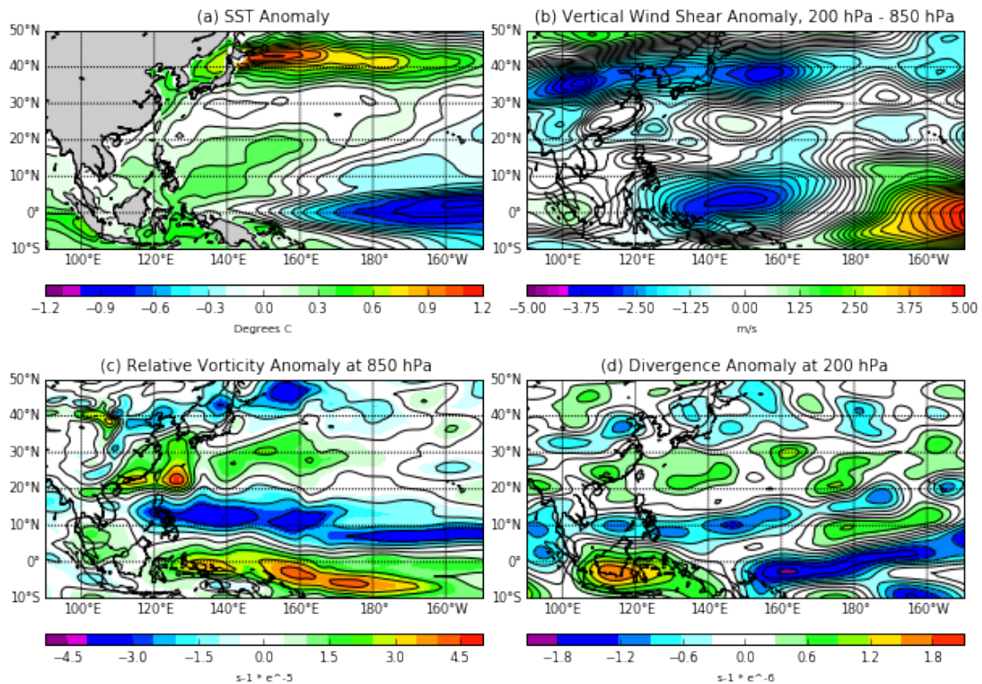
Figure 23. LN LSEF anomalies for JASO of 1981–2005 based on CCSM4 historical results. (a) SST (°C); (b) vertical wind shear ( \text{m s}^{-1} ); (c) relative vorticity ( \text{s}^{-1} ); (d) divergence ( \text{s}^{-1} ).
