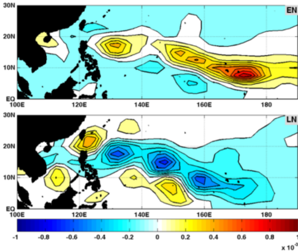
Figure 4. EN (top panel) and LN (bottom panel) TC formation probability anomalies (color shading) for JASO 1981–2010. Source: Johnson (2011).
