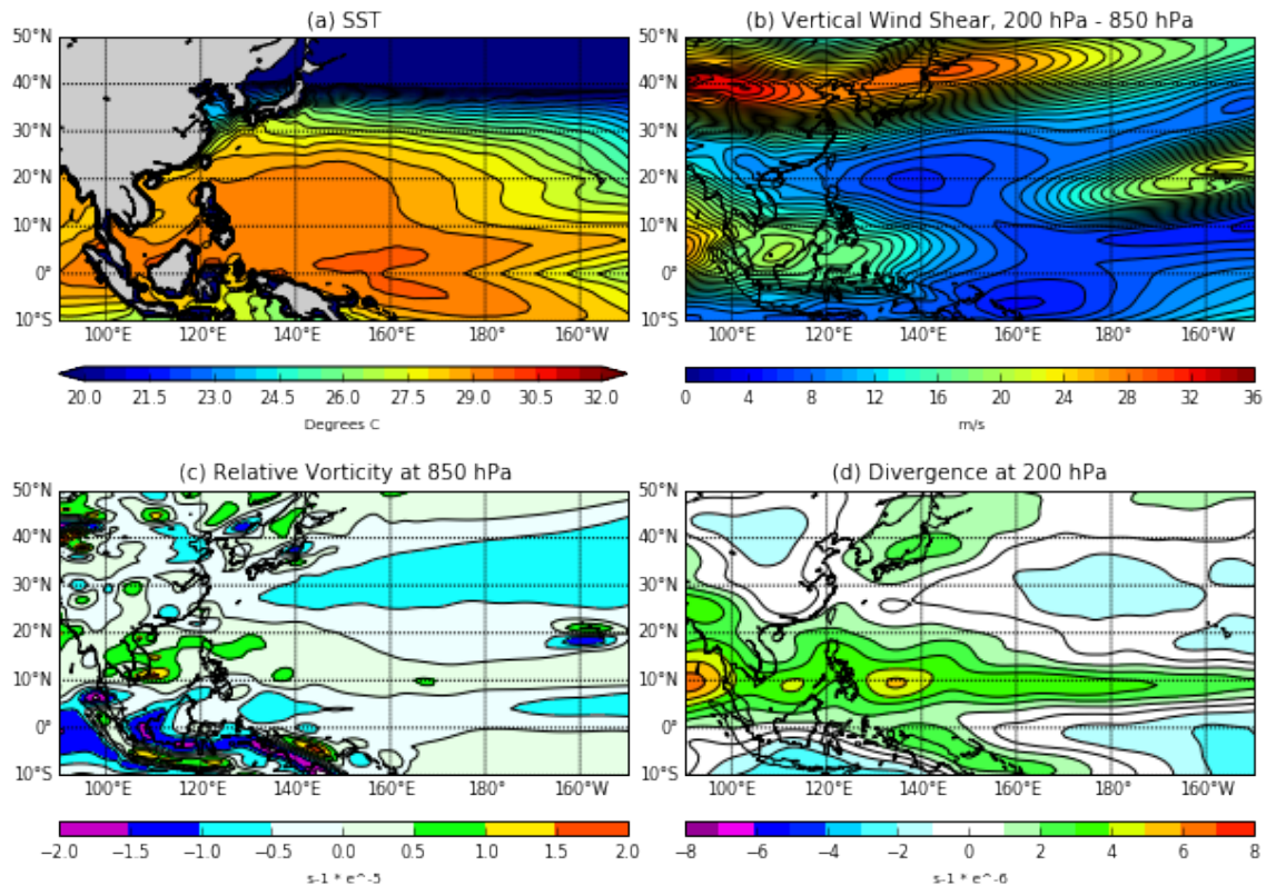
Figure 28. LSEFs for JASO 1981–2018 based on CFSRV2 results. (a) SST (°C); (b) vertical wind shear ( m s^{-1} ); (c) relative vorticity ( s^{-1} ); (d) divergence ( s^{-1} ).
