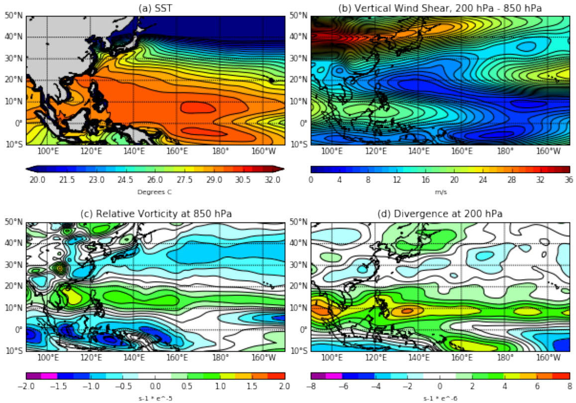
Figure 17. LSEFs for JASO of EN years (1982, 1986, 1987, 1991, 1997, 2002) based on CCSM4 historical results. (a) SST (°C); (b) vertical wind shear (m s -1 ); (c) relative vorticity (s -1 ); (d) divergence (s -1 ).
