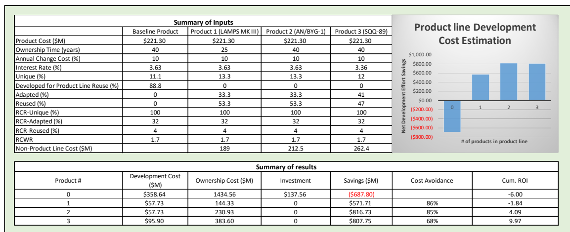
Figure 18. Best Case Scenario System COPLIMO
