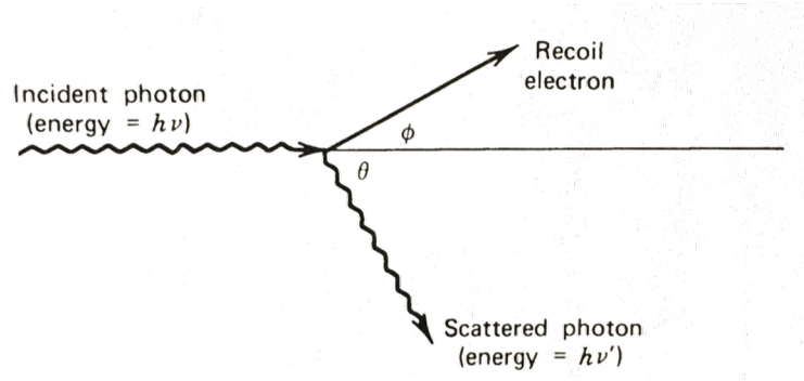
Figure 5. Depiction of Compton Scattering. Source: [14].
