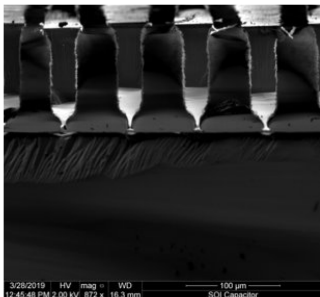
Figure 28. Side-View SEM Image of Capacitor Chip
