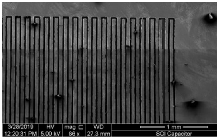
Figure 27. Top-Down SEM Image of Capacitor Chip
