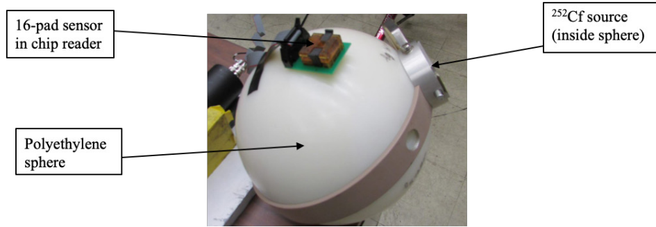
Figure 40. 16-pad Resistive Sensor Exposed to Moderated Californium-252
