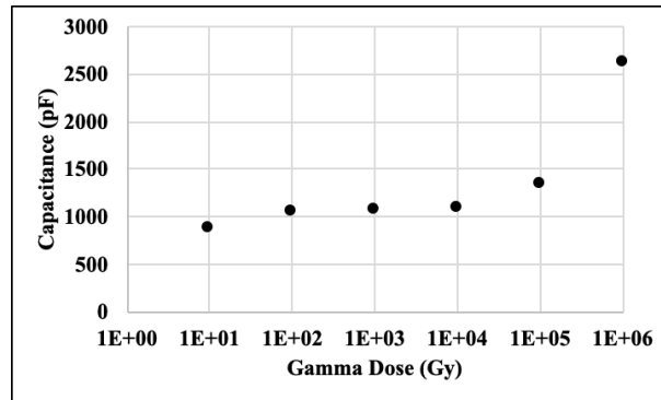
Figure 55. Theoretical Capacitance Values for Future Sensor
