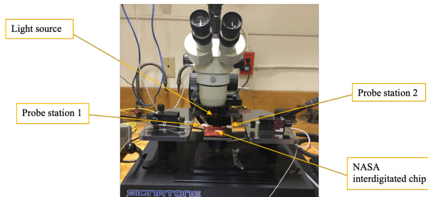
Figure 46. Probe Station Set Up for Light Interaction Experiment
