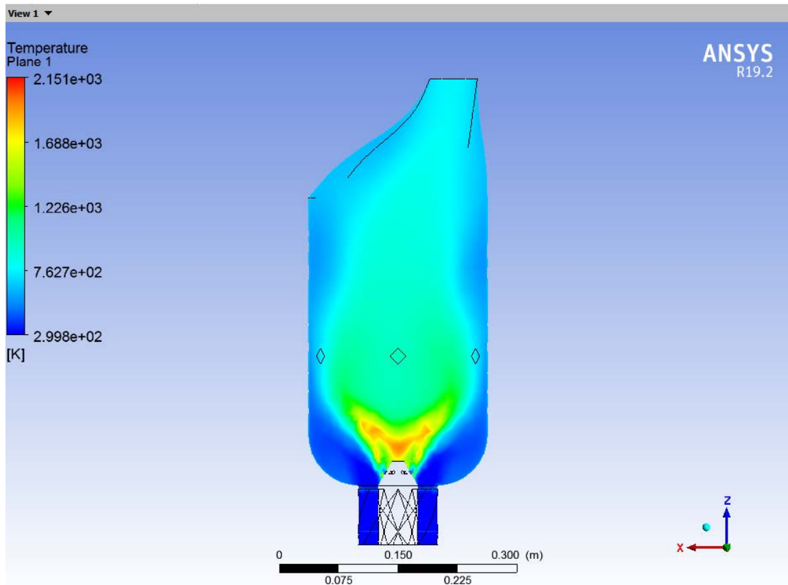
Temperature inside the combustion chamber ( \text{H}_2 -air reaction, inlet velocity 40 m/s)
