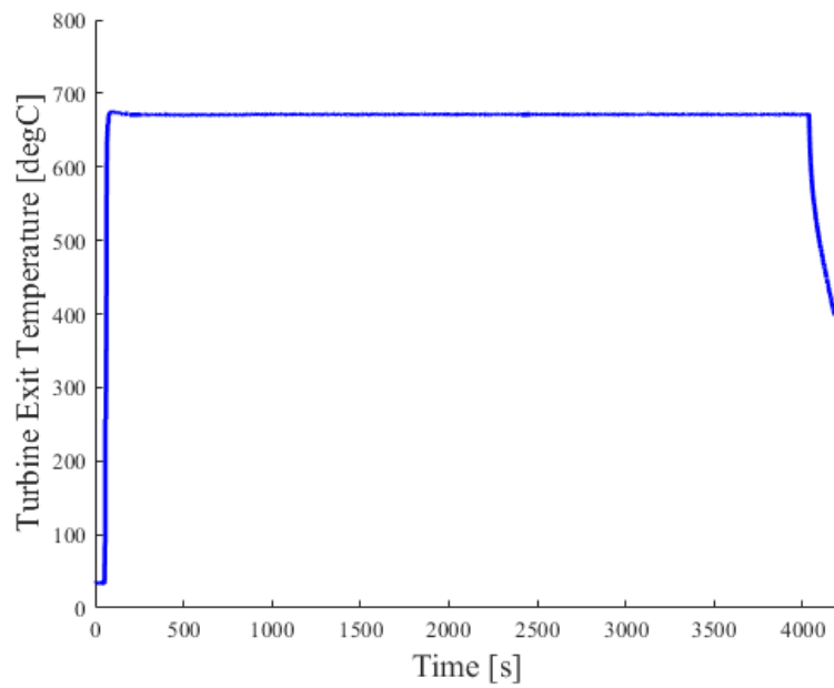
Figure 21. Total runtime vs. turbine exit temperature ( \text{C}_3\text{H}_8 -fueled operation with high-pressure C30)
