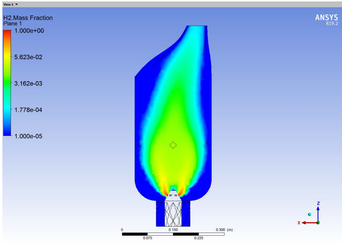
Figure 9. Fuel mass fraction inside the combustion chamber ( \text{H}_2 -air reaction, 165 m/s)
