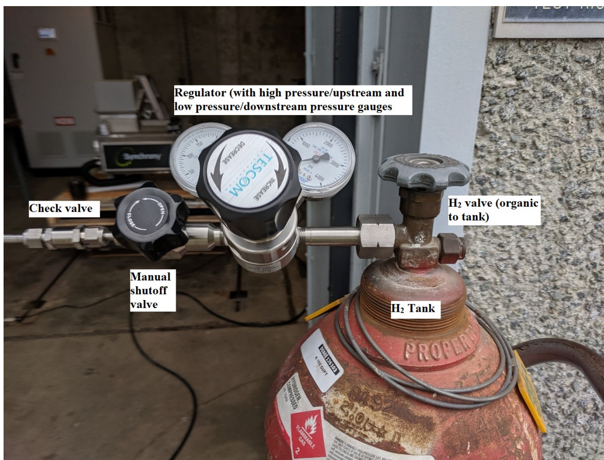
Figure 17. H 2 regulator assembly, including the regulator, pressure gauges, manual shutoff valve, and check valve
