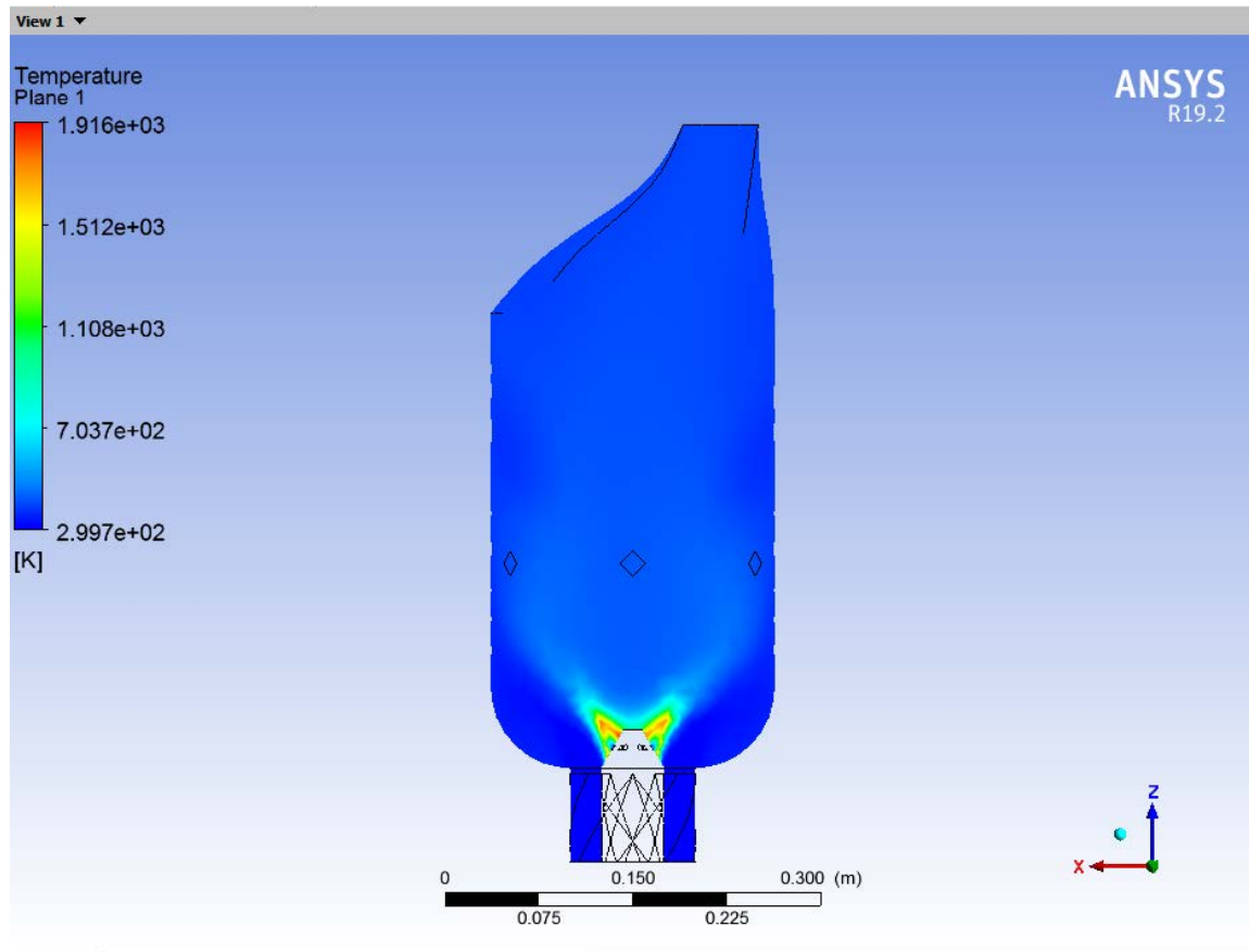
Temperature inside the combustion chamber ( \text{H}_2 -air reaction, inlet velocity 10 m/s)
