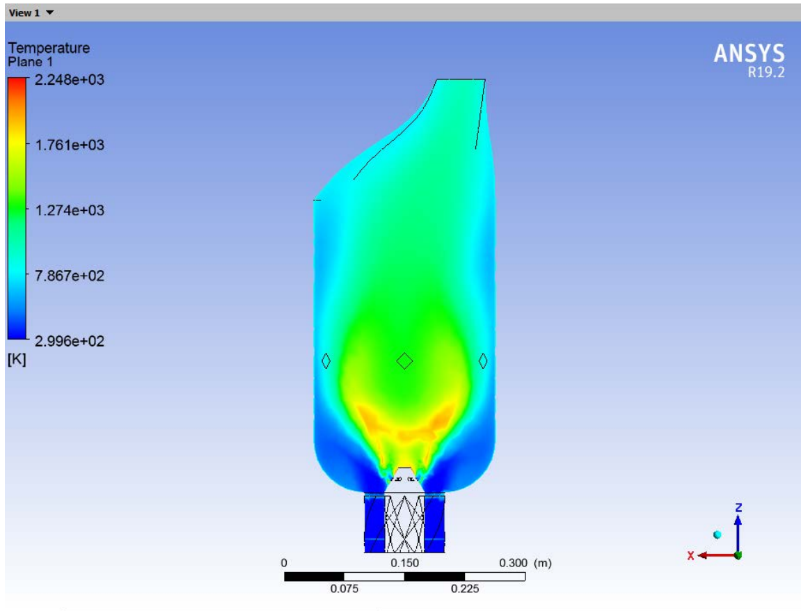
Temperature inside the combustion chamber ( \text{H}_2 -air reaction, inlet velocity 60 m/s)
