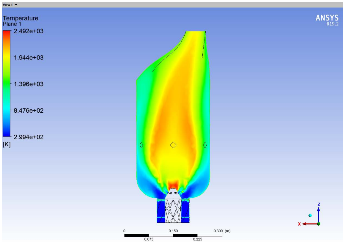
Temperature inside the combustion chamber ( \text{H}_2 -air reaction, inlet velocity 165 m/s)
