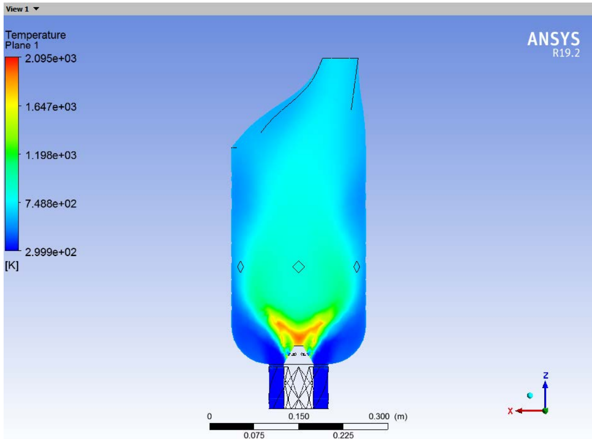
Temperature inside the combustion chamber ( \text{H}_2 -air reaction, inlet velocity 35 m/s)
