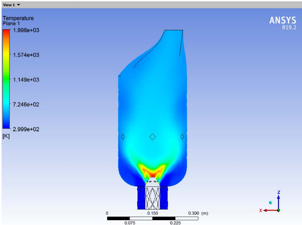
Temperature inside the combustion chamber ( \text{H}_2 -air reaction, inlet velocity 25 m/s)
