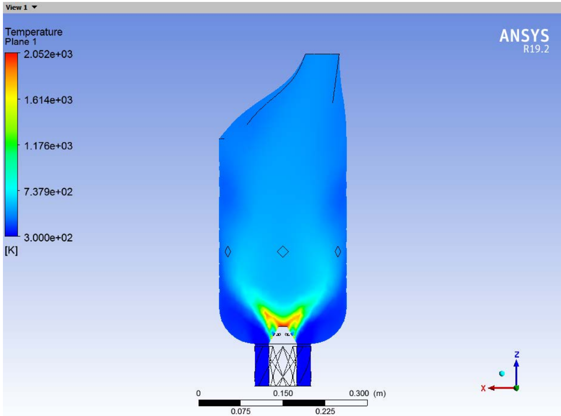
Temperature inside the combustion chamber ( \text{H}_2 -air reaction, inlet velocity 20 m/s)
