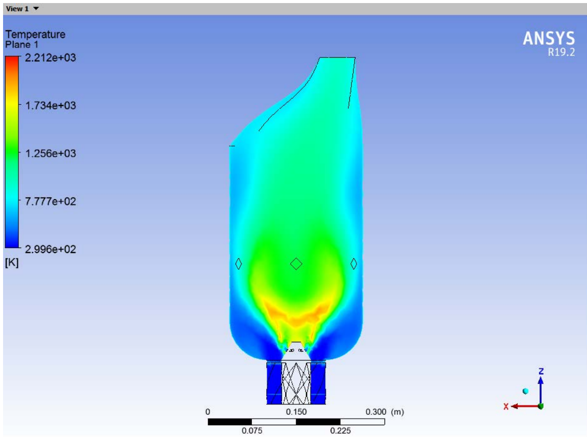
Temperature inside the combustion chamber ( \text{H}_2 -air reaction, inlet velocity 55 m/s)
