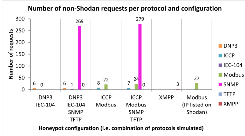
Figure 4. Results from Cloud-Based Industrial Honeypot Deployment. Source: [19].
