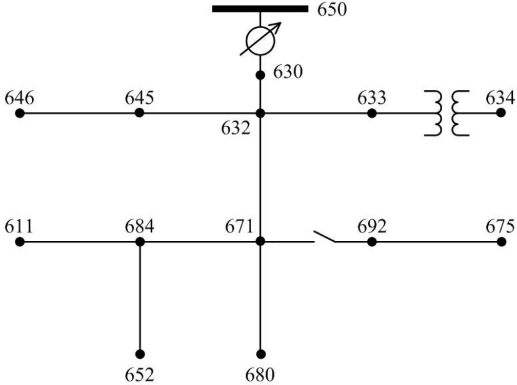
The switch is located between nodes 671 and 692. The transformer is located between nodes 633 and 634. The regulator is located between nodes 630 and 650.
