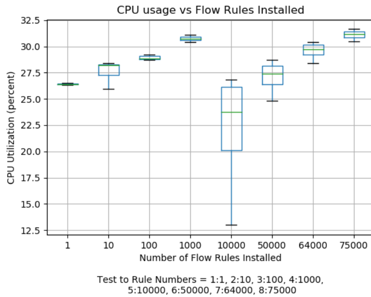
Figure 4.8. CPU Utilization per Test Comparison. Notice that for 10,000 rules the range of values is large.
