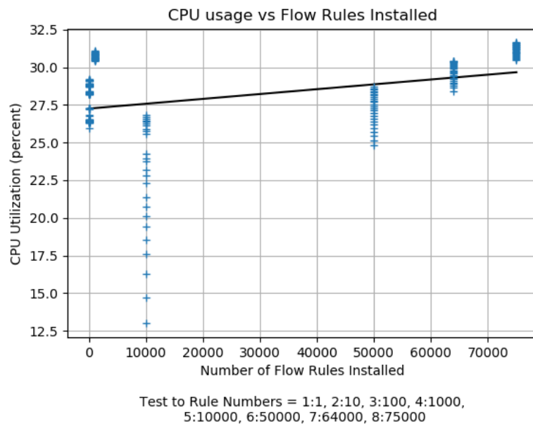
Figure 4.9. CPU Utilization with Linear Regression. r^2 for this fit was low at 0.061892
