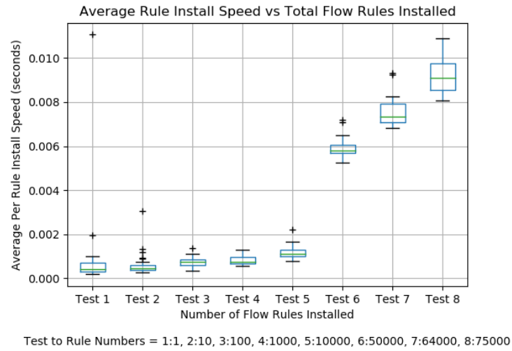
Figure 4.2. Average Per Rule Installation Time Comparisons. The depicted bars are standard box plots showing the inter-quartile range, min, max, median and outliers of each test.
