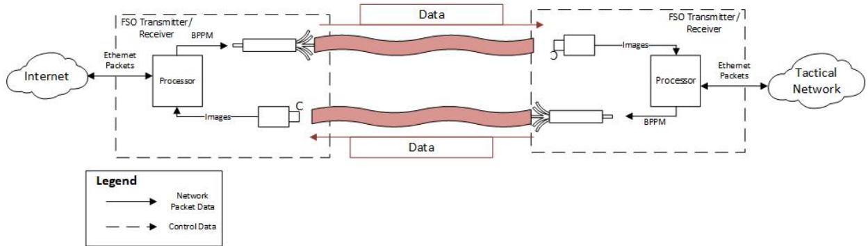
Figure 9. Transmission Overview
