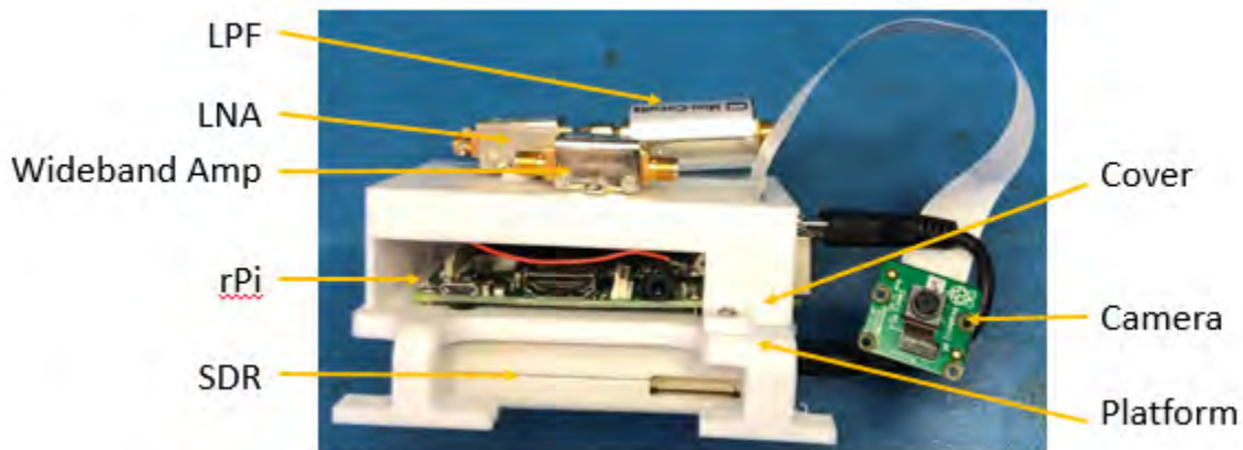
Figure 40. Payload Mount
