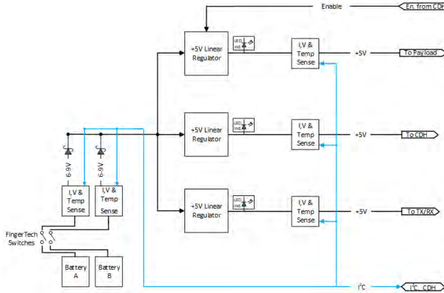
Figure 29. RDCS EPS Block Diagram. Adapted from [57].
