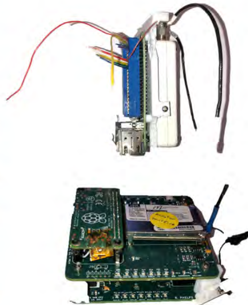
From top left to right: Mini-Circuits Components, Payload Deck, electrical harness, and EPS and C&DH Board.
