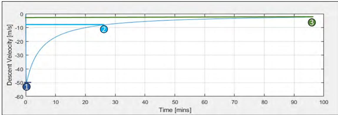
Figure 38. Predicted Descent Velocity as a Function of Time
