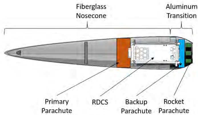
Figure 53. Payload Bay Integration. Adapted from [32].
