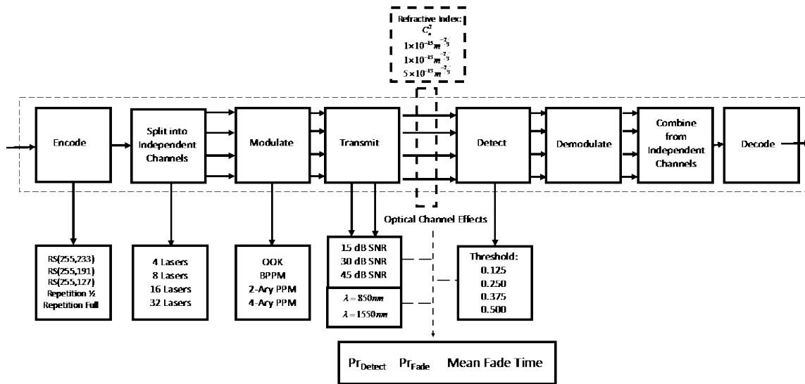
Figure 17. Architecture Design Decisions
