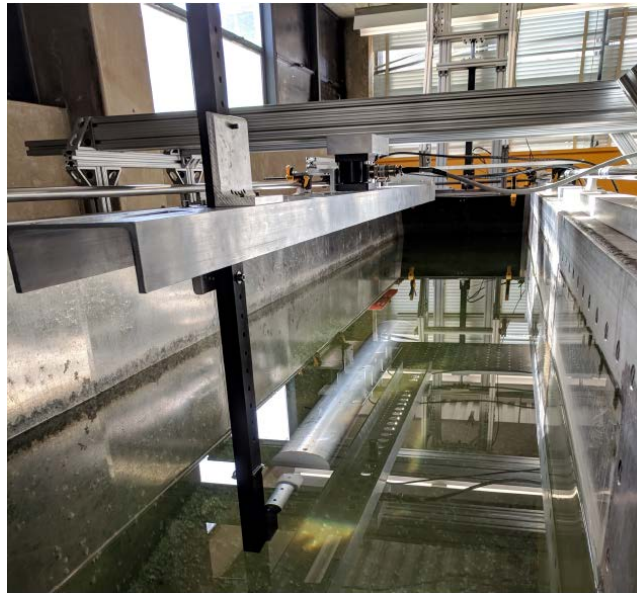
Figure 10. Sting style test fixture with model attached. Source: [5].
