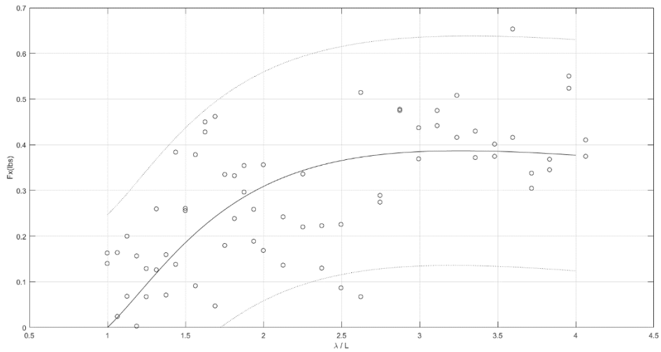
Figure 73. Drag force results for a model with flat face end caps at a nondimensional depth of 2.0 at 0.762 m/sec (2.5 ft./sec)
