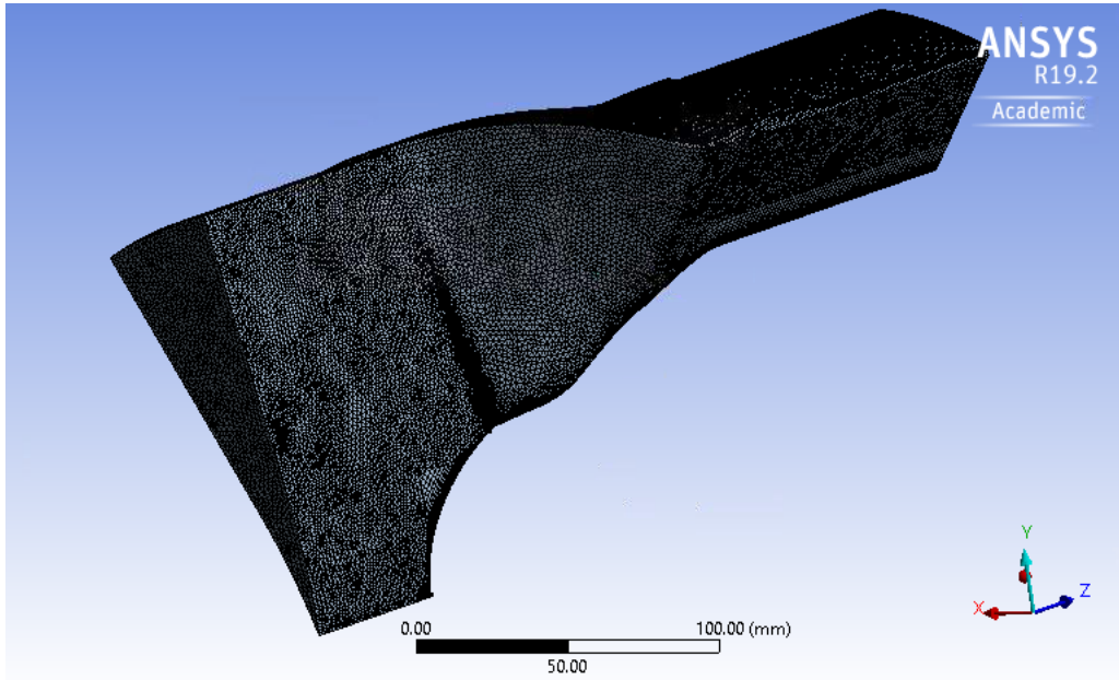
Figure 17. Gas-path mesh for flow-feature identification, 1.41% tip-gap
