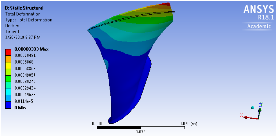
Figure 6. Total deformation due to 90% speed operation
