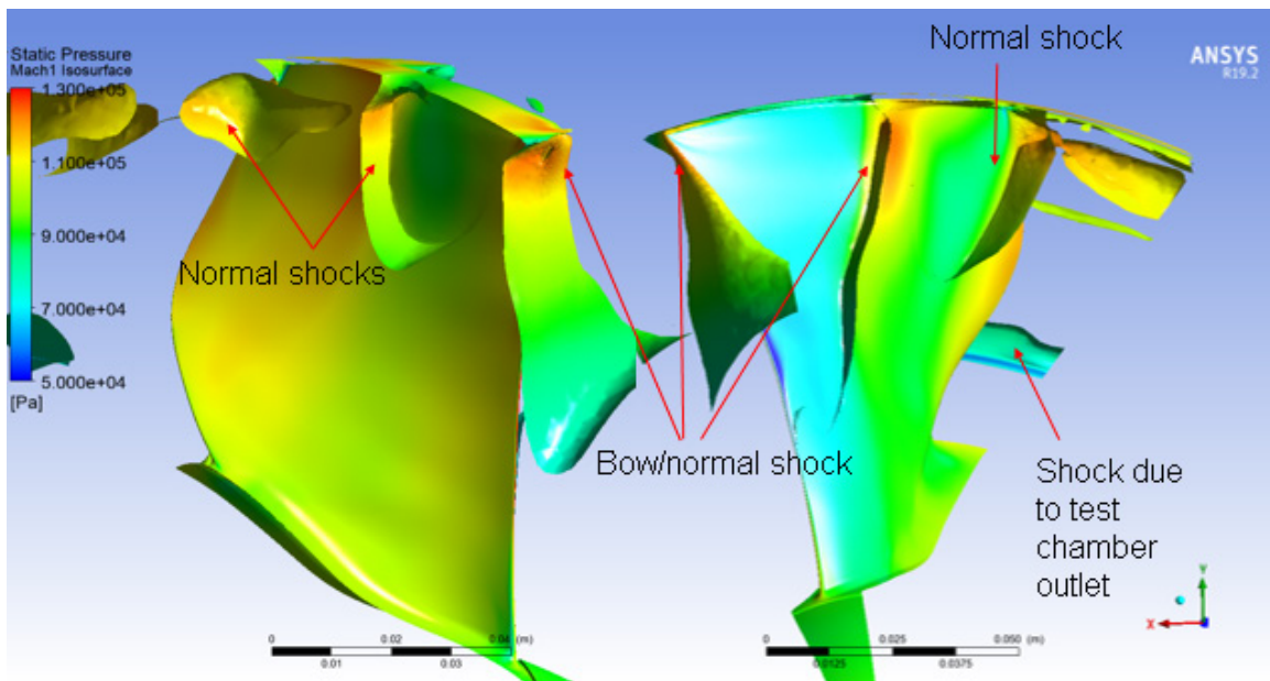
Figure 20. Mach 1 isosurface, pressure contours for hot shape, 1.41% tip-gap
