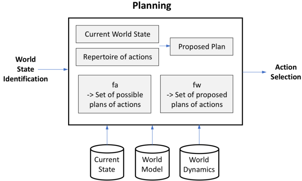
Fig. 11 Planning component
