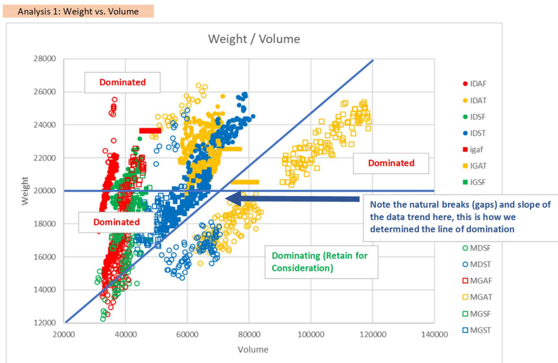
Figure 17: Set Based Design analysis comparing variants of a medium-surface combatant [65]
