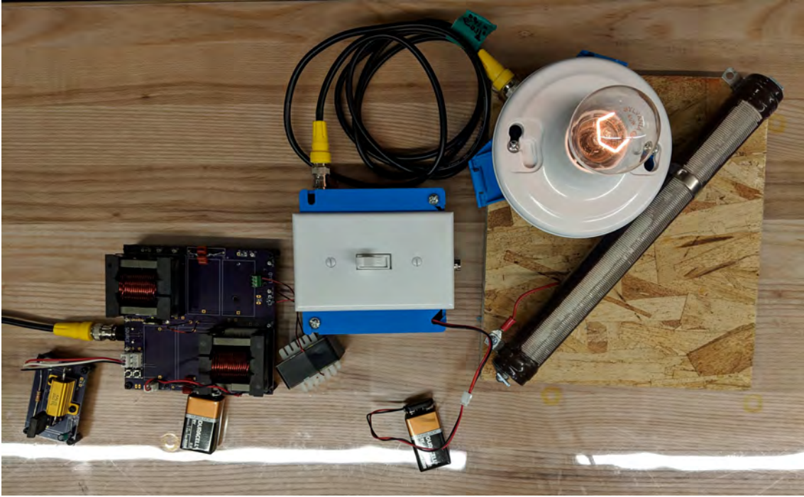
Figure 4-1. The model-scale power system used in the experiments.
