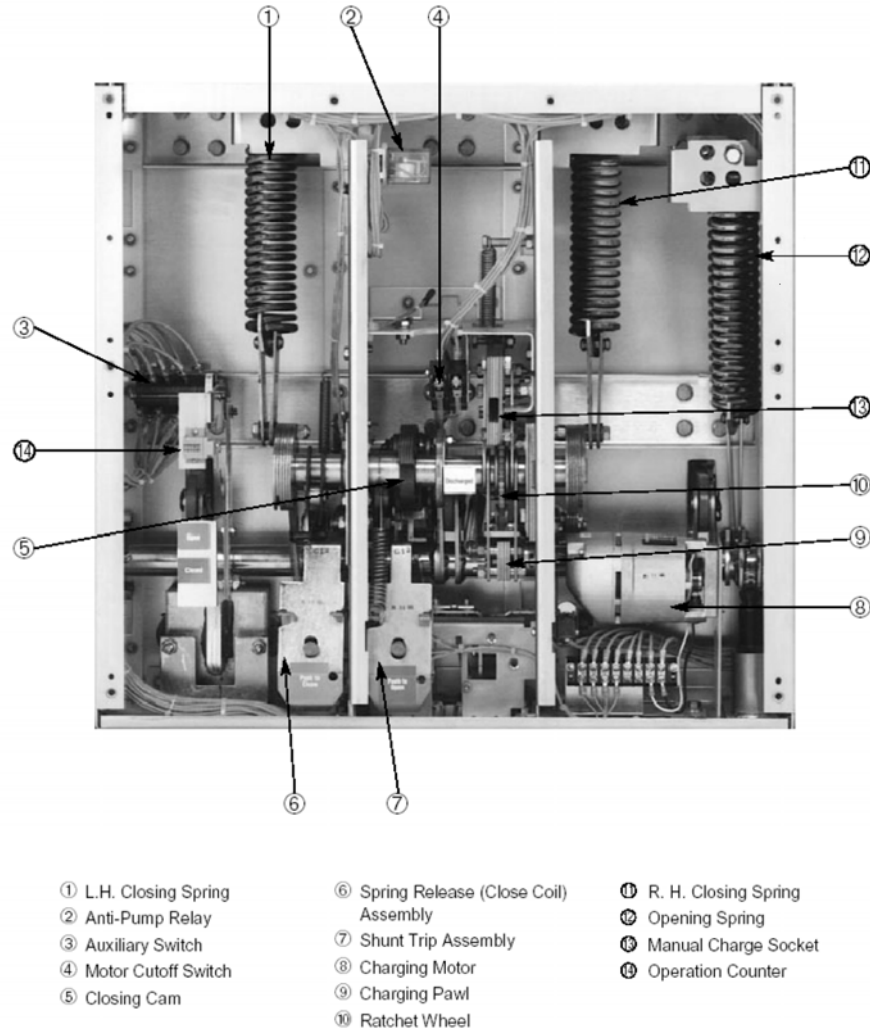
Figure 5-2. A picture of Eaton VCP-W Vacuum Circuit Breaker showing internal components, including opening springs. Source: Eaton, used with permission [15].
