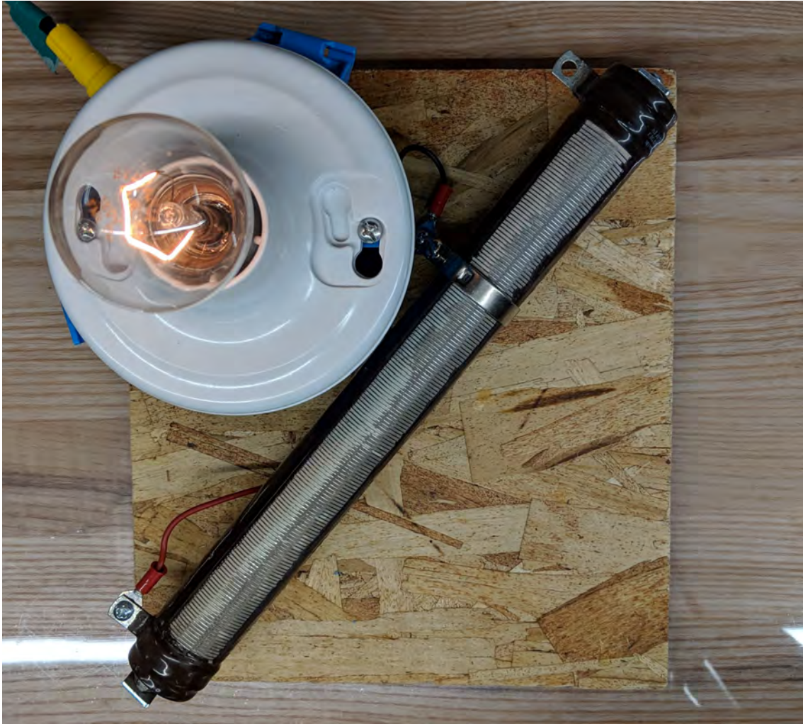
Figure D-3. A photograph of the load connected to the model-scale system.
