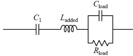
Figure 4-5. The RLC oscillator responsible for the first ringing transient shown in Figure 4-4.
