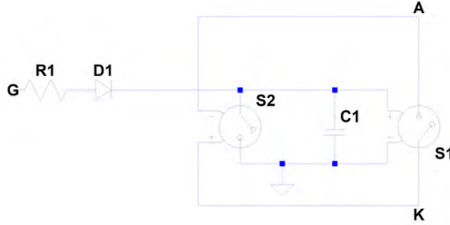
Figure B-1. LTSpice circuit model of a thyristor.
