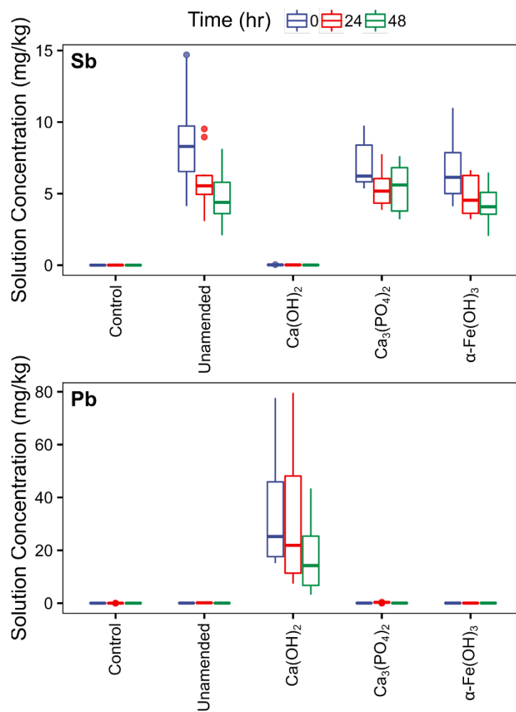
Figure 3. Box and whisker plots of Sb and Pb concentrations in batch-reactor solutions over the 48-hour experiment.
