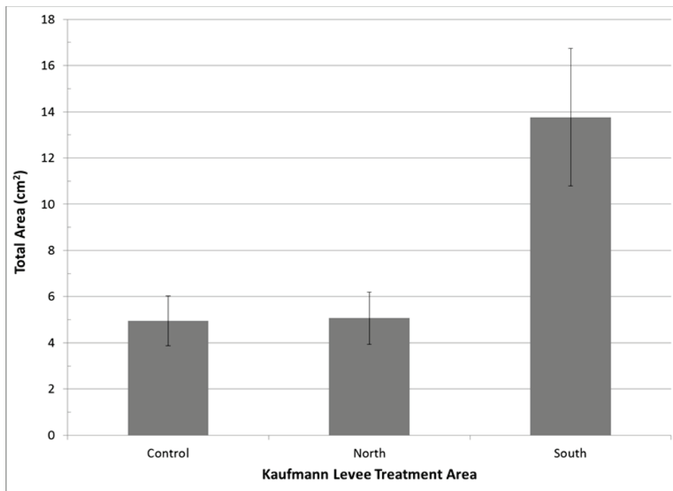
Figure 24. Comparison of total root area (cm 2 ) between plants grown with no biopolymer to those grown in biopolymer-treated soil (North and South Treatment Areas).
