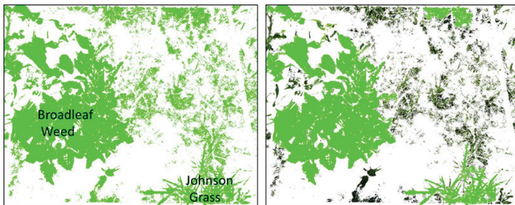
Figure 17. Easy Leaf Area digital image of the sample plot shown in Figure 16, with filters applied, allowing separation of plants from background and selection of specific plants. Black in the image on the right indicates Bermuda grass.
