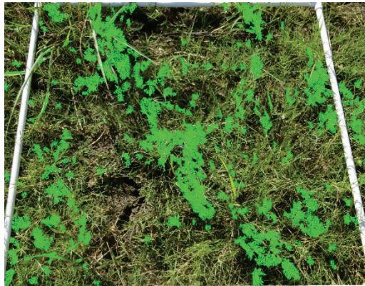
Figure A51. Middle Treatment Area, sample 5 (Non-Bermuda grass leaf area).
