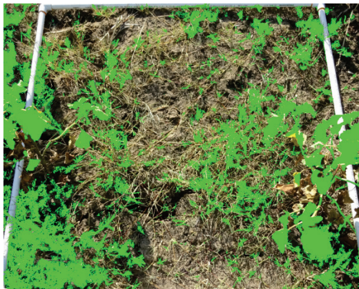
Figure A23. North Treatment Area, sample 2 (total leaf area).
