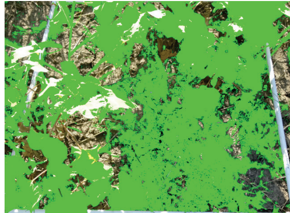
Figure A17. Control Area, sample 6 (total leaf area).
