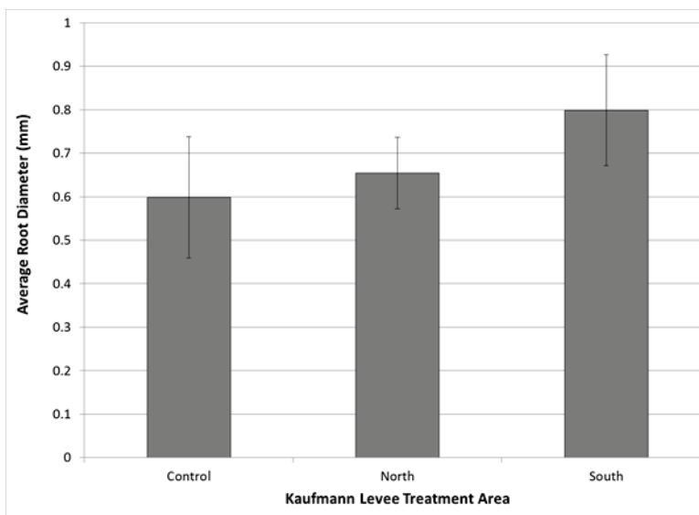
Figure 21. Comparison of average root diameter between plants grown with no biopolymer to those grown in biopolymer-treated soil (North and South Treatment Areas).
