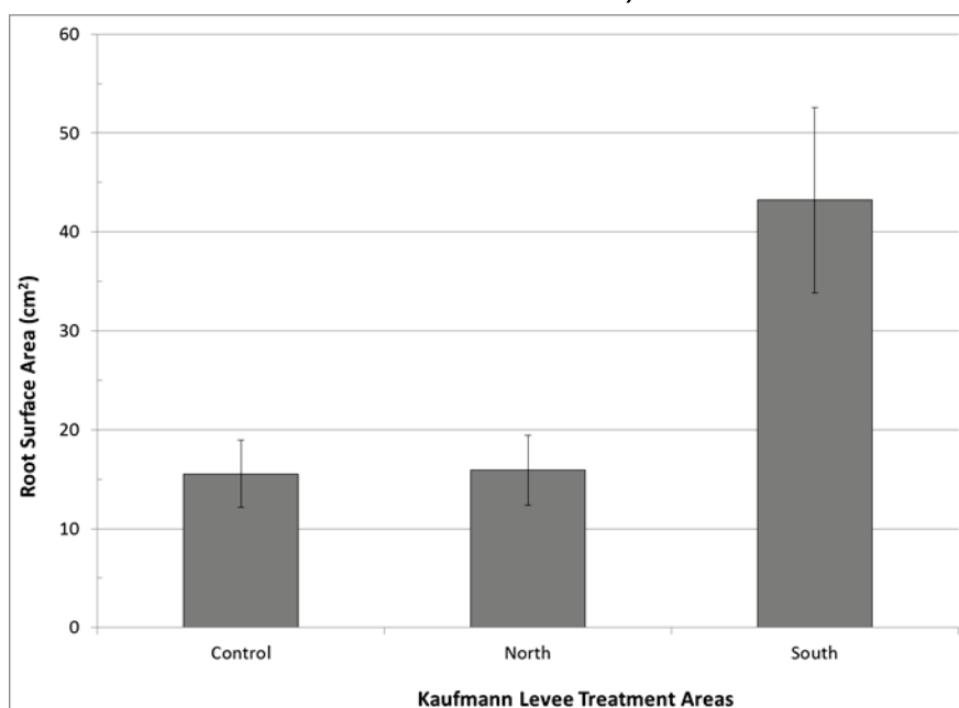
Figure 23. Comparison of root surface area ( \text{cm}^2 ) between plants grown with no biopolymer to those grown in biopolymer-treated soil (North and South Treatment Areas).
