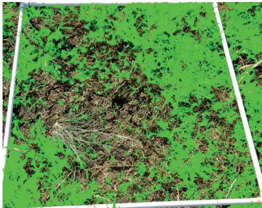
Figure A53. Middle Treatment Area, sample 6 (total leaf area).
