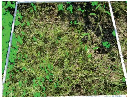
Figure A42. Middle Treatment Area, sample 2 (non-Bermuda grass leaf area).
