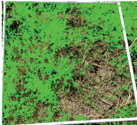
Figure A67. South Treatment Area, sample 5 (total leaf area).
