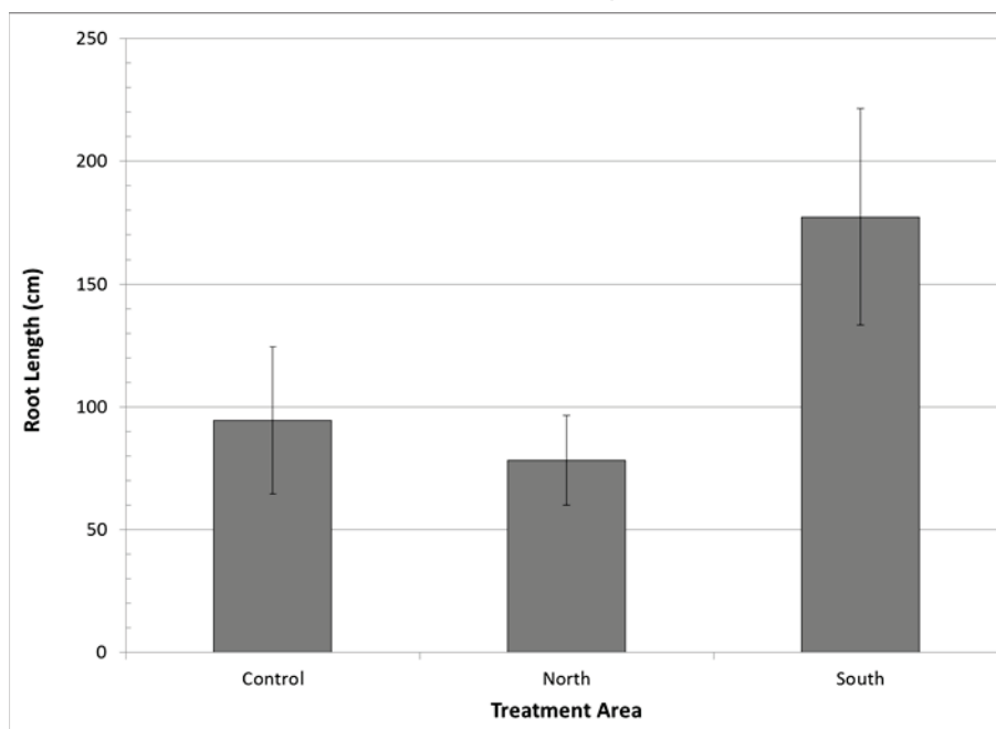
Figure 20. Comparison of average root length between plants grown with no biopolymer to those grown in biopolymer-treated soil (North and South Treatment Areas).
