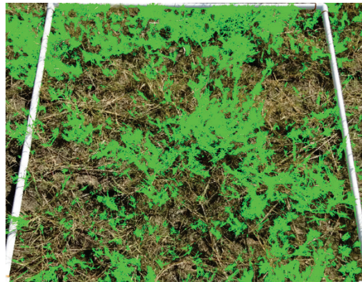
Figure A64. South Treatment Area, sample 4 (total leaf area).
