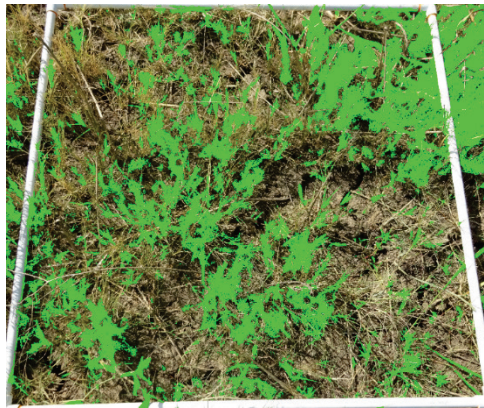
Figure A61. South Treatment Area, sample 3 (total leaf area).
