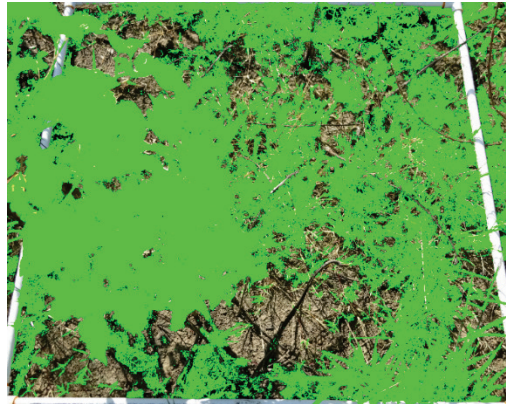
Figure A47. Middle Treatment Area, sample 4 (total leaf area).
