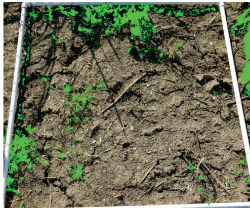
Figure A32. North Treatment Area, sample 5 (total leaf area).
