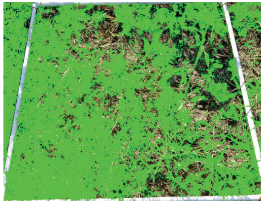
Figure A41. Middle Treatment Area, sample 2 (total leaf area).
