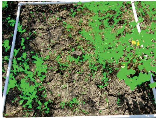
Figure A29. North Treatment Area, sample 4 (total leaf area).
