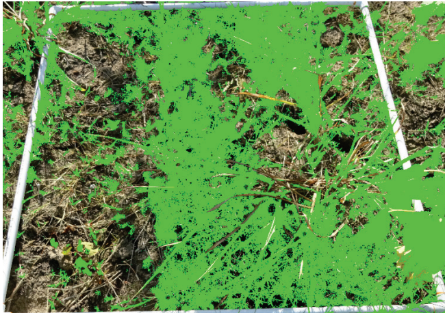
Figure A11. Control Area, sample 4 (total leaf area).
