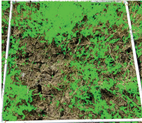
Figure A58. South Treatment Area, sample 2 (total leaf area).
