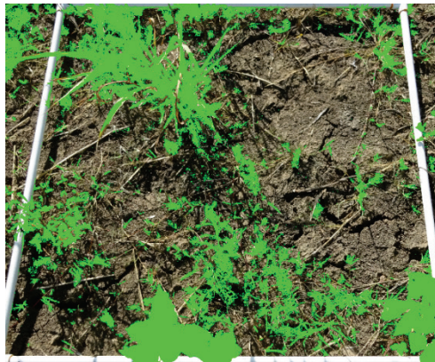
Figure A44. Middle Treatment Area, sample 3 (total leaf area).
