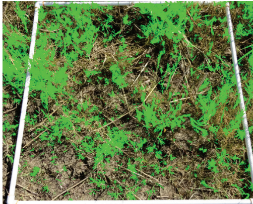
Figure A70. South Treatment Area, sample 6 (total leaf area).
