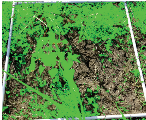
Figure A38. Middle Treatment Area, sample 1 (total leaf area).
