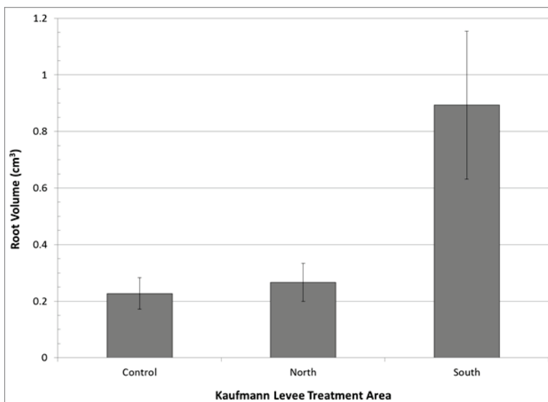
Figure 22. Comparison of root volume ( \text{cm}^3 ) between plants grown with no biopolymer to those grown in biopolymer-treated soil (North and South Treatment Areas).
