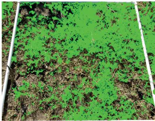
Figure A26. North Treatment Area, sample 3 (total leaf area).
