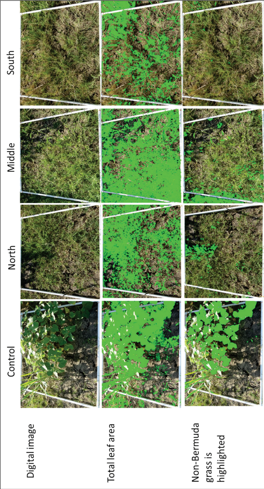
Figure 18. Set of photographic data from all biopolymer treatment areas and the control area of the Kaufman levee.
