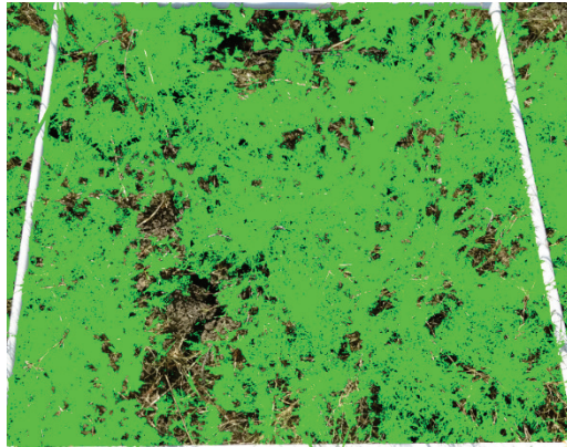
Figure A50. Middle Treatment Area, sample 5 (total leaf area).
