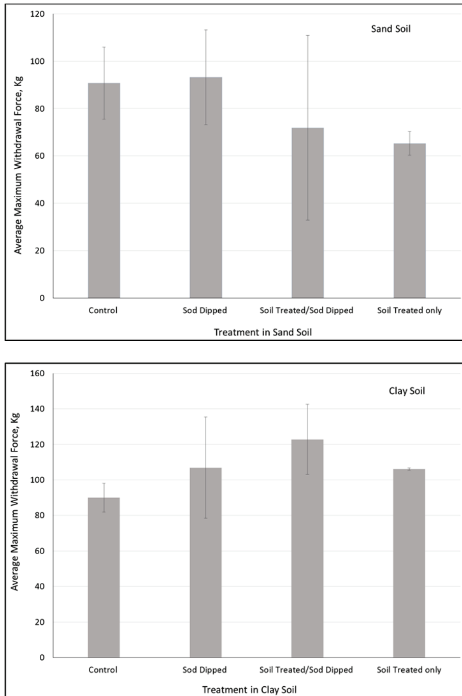
Figure 11. Average maximum withdrawal force (kg) required to remove sod section from the surrounding soil in control and biopolymer-treated experimental plots after 10 weeks. Top. Sand-soil type. Bottom. Clay-soil type.
