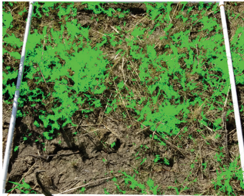
Figure A56. South Treatment Area, sample 1 (total leaf area).
