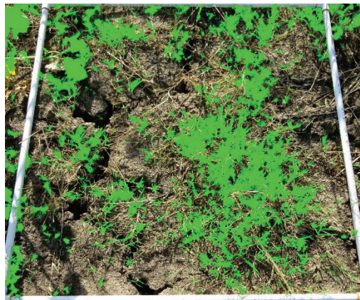
Figure A20. North Treatment Area, sample 1 (total leaf area).
