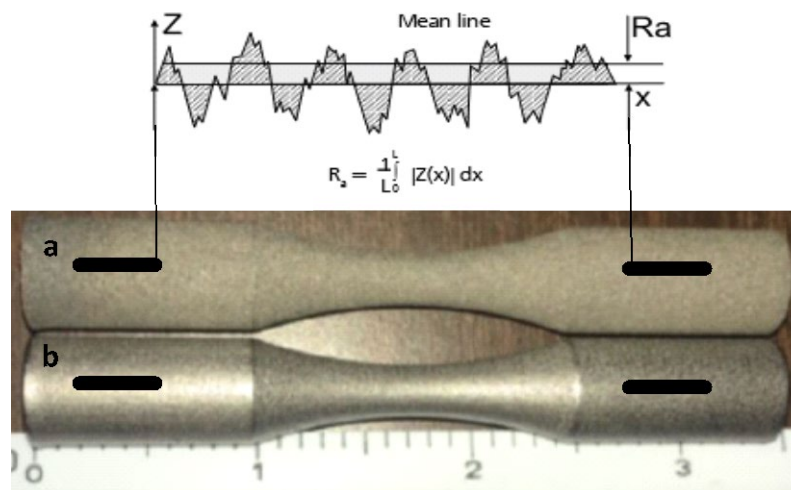
Figure 8. Fatigue Specimen: a) fatigue specimen in the as printed built condition with an average surface roughness Ra = 25.0 μm; b) fatigue specimen after 30 minutes of processing with the TT 45 with Ra = 5.4 μm
