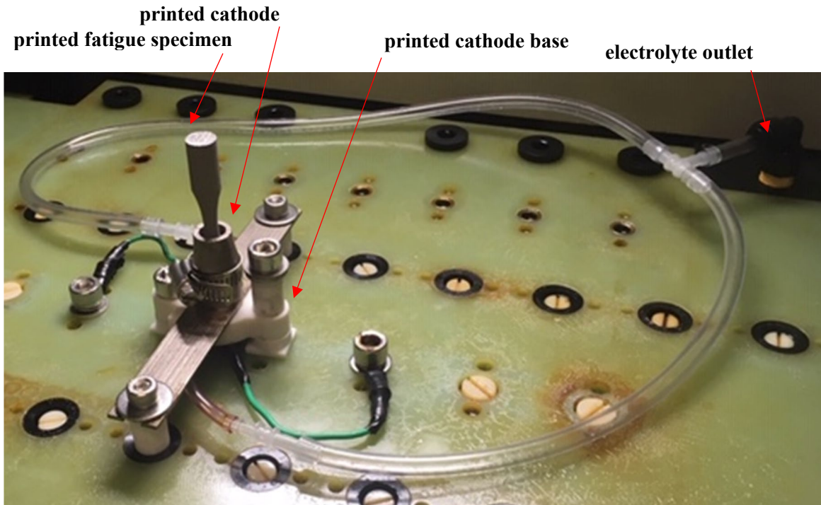
Figure 9. Cool Pulse 1000 Set UP for Machining a Fatigue Specimen
