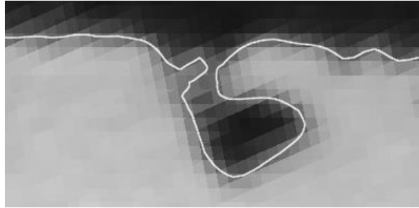
Figure 10. CAT Scan of the Surface of a Ti 6 Al 4 Part that was printed using Laser Powder Bed Fusion, Hot-Isostatic Pressed, and Superfinished with the Image showing a Smooth Surface ( R_a < 0.2 \mu\text{m} ) and a Surface Interconnected Porosity Defect; Courtesy of CIMP 3D
