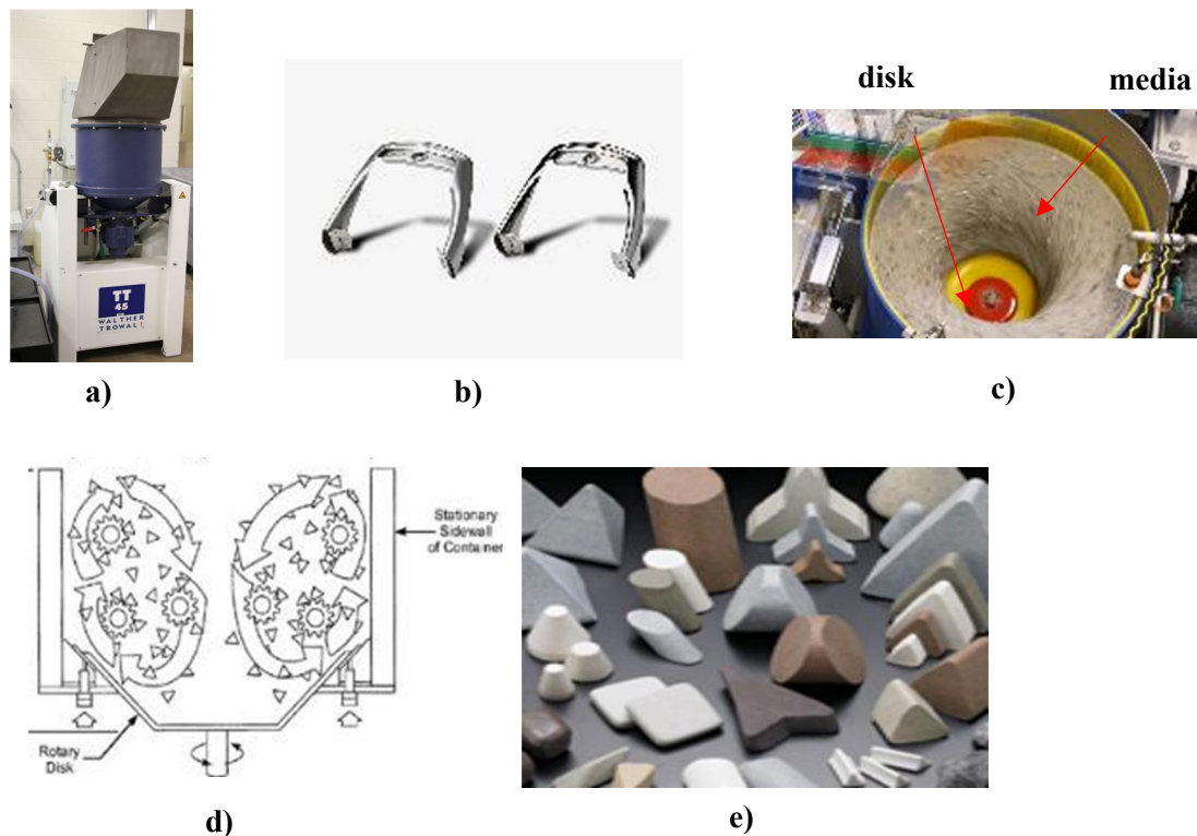
Figure 1. TT 45 Centrifugal Disk Finisher: a) TT 45 in Penn State Lab; b) open surfaced parts typically machined*; c) disk and media in motion*; d) part and media tumbling action; e) rigid media; *courtesy of Walther Trowal
