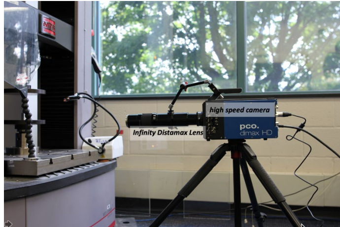
Figure 6. High Speed Camera System
