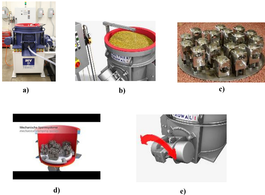
Figure 2. MV 21 Multi-Vibe Bowl Finisher: a) MV 21 in Penn State Lab; b) tumbling media in bowl*; c) parts typically machined*; d) parts fixtured to bowl bottom*; e) motor with adjustable orientation* ; * courtesy of Walther Trowal
