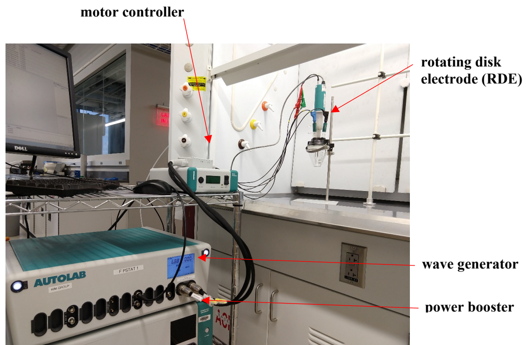
Figure 7. Mini-ECM Equipment
