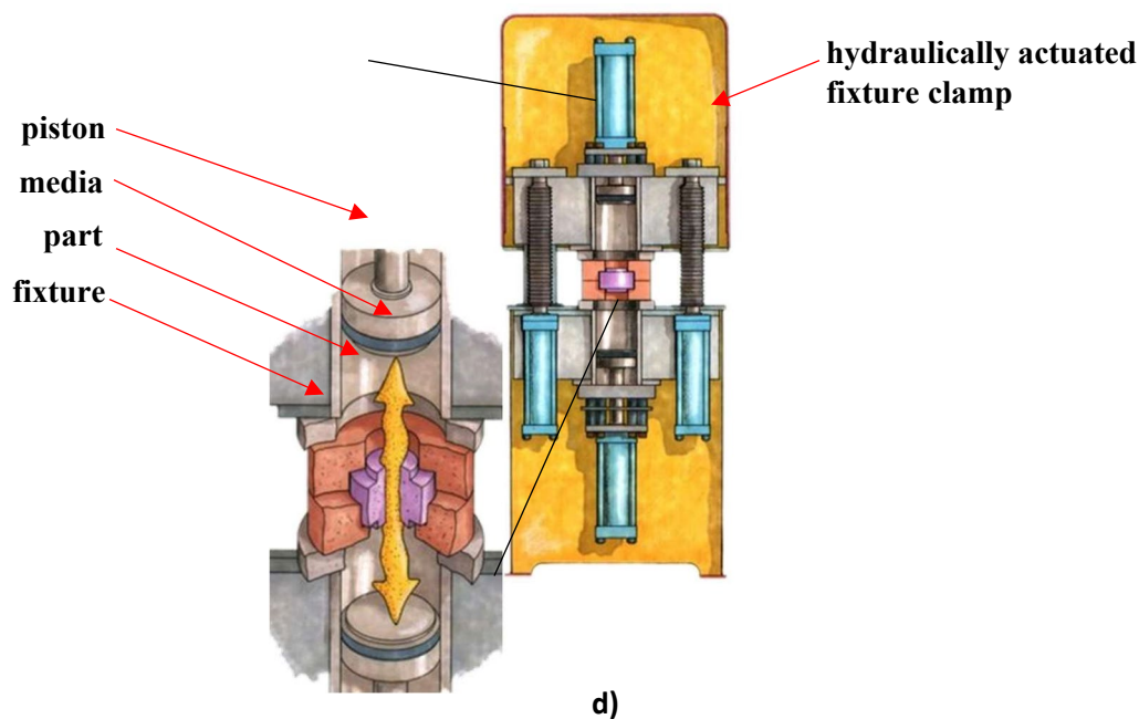
Figure 3. Vector 150 Abrasive Flow Machine: a) Vector 150 in Penn State Lab; b); viscous abrasive media*; c) parts typically machined*; d) fixture, part, reciprocating pistons and media in motion*; *courtesy of Extrude Hone
