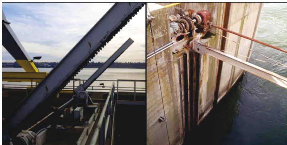
Figure 25. Left - Heavily greased above-water gearing for movement of adjustable fishway weirs at McNary Dam. Right - Greased above water cable system movement of adjustable fishway entrance gates, McNary Dam.
