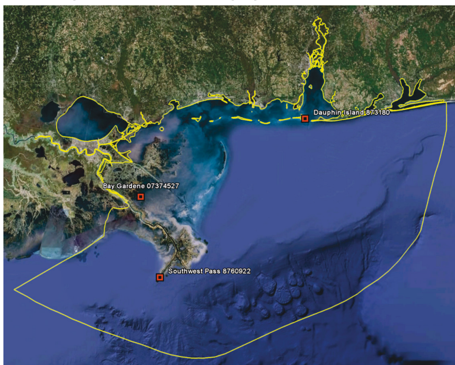
Figure 2-4. Location of tidal gauges and model boundary.
