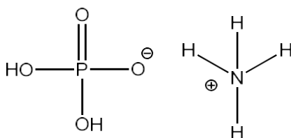
Figure 2. [\text{NH}_4][\text{H}_2\text{PO}_4]
