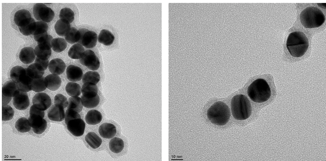
Figure 3. TEM images of \sim 15 nm diameter Au nanoparticles wrapped in \sim 3 nm thick \text{TiO}_2 shells. The “darker” core is Au and the “lighter” shell is \text{TiO}_2 . In a majority of the cases the shells .
