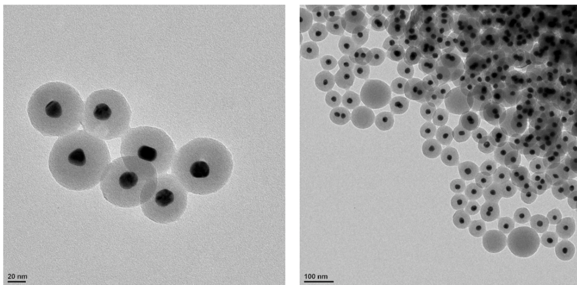
Figure 2. TEM images of ~15 nm diameter Au nanoparticles wrapped in ~ 10 nm thick NiO shells. The “darker” core is Au and the “lighter” shell is NiO. In a majority of the cases the shell only encapsulates a single Au particle.
