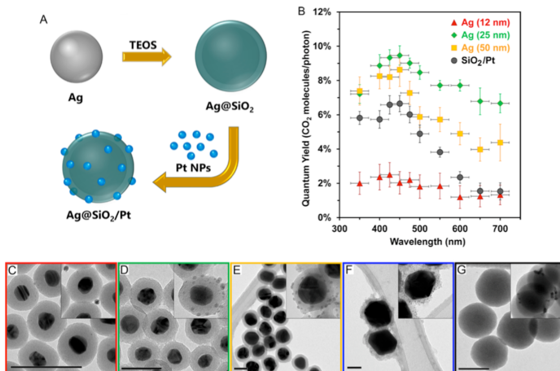
Figure 6. (A) Synthesis scheme for the Pt decorated core-shell Ag@SiO 2 particles. (B) Quantum yield for CO 2 production as a function of wavelength for core-shell structures with varying Ag particle size and constant SiO 2 thickness and Pt particle loading. The results demonstrate the clear ability of Ag localized surface plasmon resonance to promote photocatalysis by nearby Pt particles. (C)-(G) TEM images of Ag@SiO 2 /Pt particles with 12 nm (C), 25 nm (D), 50 nm (E) and 100 nm (F) Ag cores and constant 10 nm thick shells. (G) shows a TEM image of the control sample with Pt deposited on 50 nm SiO 2 particles.
