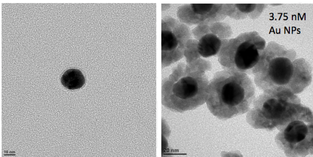
Figure 1. TEM images of ~15 nm diameter Au nanoparticles wrapped in ~ 2 nm thick and ~10 nm thick \text{Cu}_2\text{O} shells. The “darker” core is Au and the “lighter” shell is \text{Cu}_2\text{O} .
