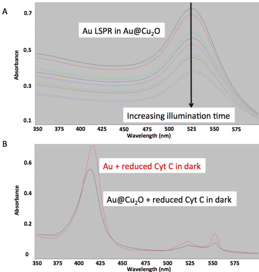
Figure 5. (A) UV-Vis absorbance spectra of Au@Cu 2 O nanoparticles with a 2 nm thick Cu 2 O shell in the solution used for cytochrome C reactivity measurements, but without cytochrome C. The measurements were collected as a function of time during illumination by 10 mW of monochromatic 532 nm light, where it is seen that the Au localized surface plasmon resonance (LSPR) peak decreased in intensity and shifted as a function of time, showing degradation of the particles. (B) UV-Vis absorbance spectra for mixtures of Au or Au@Cu 2 O with reduced cytochrome c (Cyt C) after 15 minutes in the dark, where it is clearly seen from the peaks between 500-600 nm that the Au@Cu 2 O particles can induce oxidation of cytochrome C, even in the dark.
