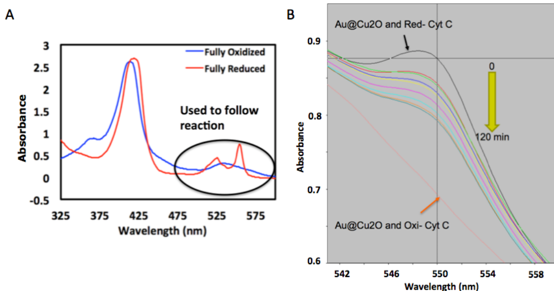
Figure 4. (A) UV-Vis absorbance spectra of fully oxidized and fully reduced cytochrome c. The features at 500-600 nm that are distinct between the two states will be used to follow the oxidation or reduction of this species. (B) UV-Vis absorbance spectra in the 540-560 nm region during an experiment where \text{Au@Cu}_2\text{O} particles shown in Figure 1(A) were mixed with cytochrome c and exposed to monochromatic 532 nm illumination (in resonance with the Au plasmon). The spectra are shown as a function of illumination time where simultaneous decrease in the feature at 550 nm and decrease in the baseline intensity were observed.
