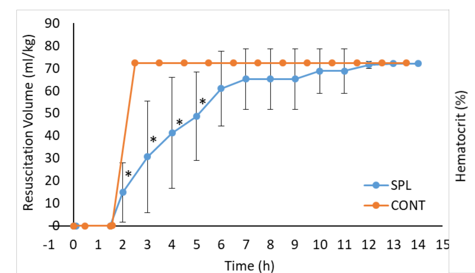
Figure 3 Resuscitation volume (A), hematocrit (B), and cardiac output (C) vs. time. (A) By T = 5 h, only 1/3rd of SPL subjects had reached their maximum resuscitation, compared to all of the CONT subjects within 1 h of starting resuscitation. (B) Hematocrit was higher in SPL than CONT at the start of hemorrhage (likely due to handling of the spleen during removal), but their positions reversed by the end of hemorrhage as the CONT spleen was able to discharge its stored red blood cells. Positions reversed again during at the time points following the start of resuscitation as the CONT group accepted all of its allowed LR in that short span of time. The lack of improvement in pressure suggests the volume was all be likely filled back up rather than resisting the influx). However the cr causing fluid to leak out through capillaries, hence the subsequent ris two groups, except at the time point after the start of resuscitation w decreased plasma viscosity lowering resistance to flow.
