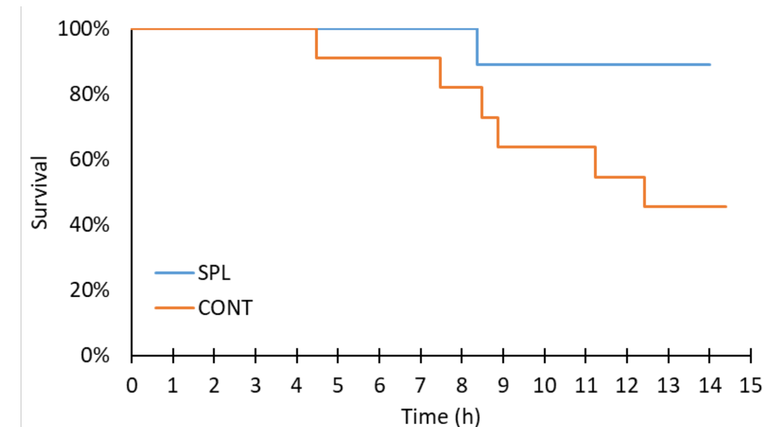
Figure 1 Effects of splenectomy on survival vs. time. Start of shock at T = 0 h. Start of resuscitation at T = 1.5 h. Total blood removal, including blood drained from the excised spleen, was 30 ml/kg in SPL group, compared to 27 ml/kg in the CONT group. Despite this increase, mortality in the SPL group was reduced to 11% (p=0.04 vs CONT) Liver re-bleeding was similar between groups ( 7.9 \pm 3.3 ml/kg in SPL, 8.1 \pm 3.0 ml/kg in CONT; NS).
