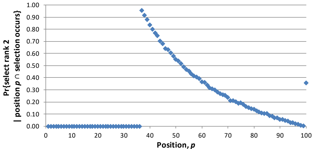
Figure 15b. For SPANS with N = 100 , probability that an applicant of rank r = 2 is selected, given the applicant is in position p and the DM makes a selection. Note that \Pr\{\text{select rank 2} \mid \text{position } p \cap \text{selection occurs}\} \geq \Pr\{\text{select rank 2} \mid \text{last position} \cap \text{selection occurs}\} for p = 37, 38, \dots 61 , and 100.
