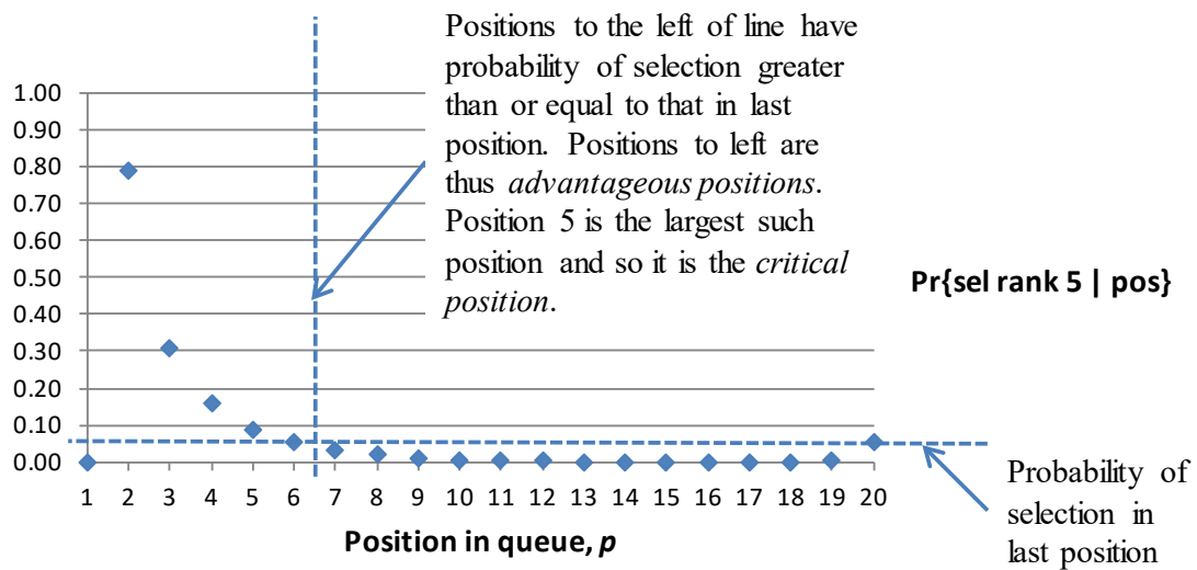
Figure 5. Conditional probability of selecting applicant with rank 5, given applicant is in position p in queue. Probability of selection is higher in positions p = 2, 3, 4 , and 5 than in last position. N = 20 and start position s = 2 .
