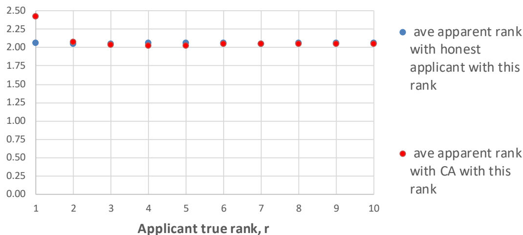
Figure 40b. Average apparent ranks for honest-only queues and CAs with ranks 1 through 10 seeking to evade selection. N = 50 and results are based on 10^6 simulated random runs.
