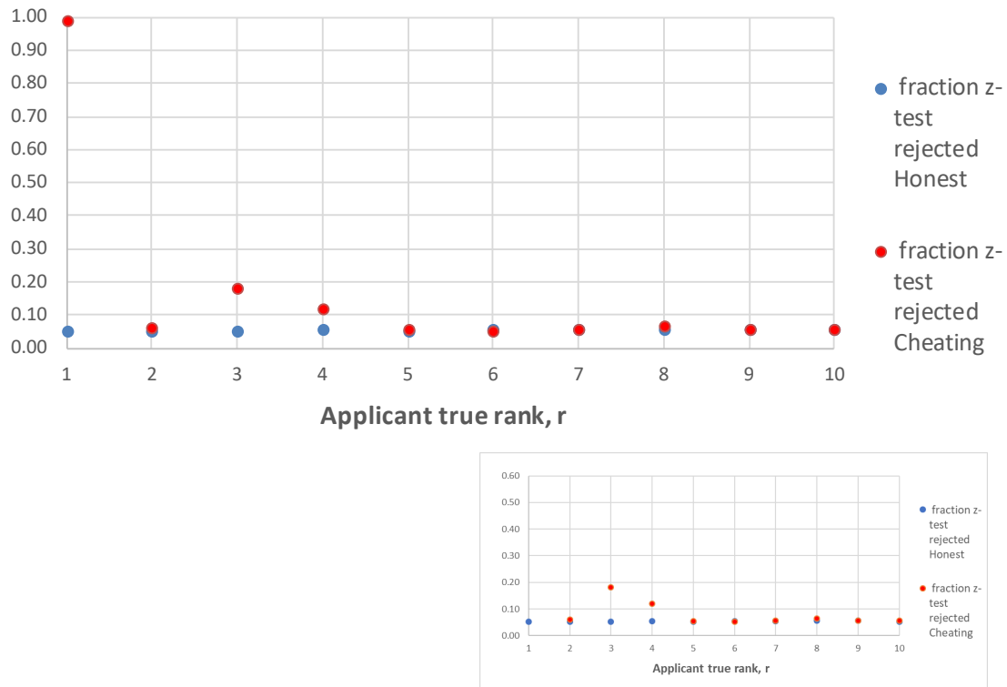
Figure 43d. Summary of reject rates for tests of hypothesis for honest-only queues and queues with CAs with ranks 1 through 10 seeking to evade selection. N = 20 applicants and z -test sample size n = 1,000 . For each CA rank, points are plotted for one set of 10^4 tests of hypothesis. An independent simulation of the honest-only queue was performed with each CA simulation. Inset is scaled to show more detail for CAs 2 through 10.
