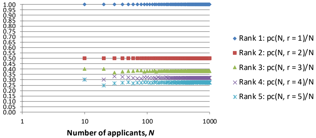
Figure 11. Critical position p_c(N, r) divided by N appears to approach constant value even for small N .
