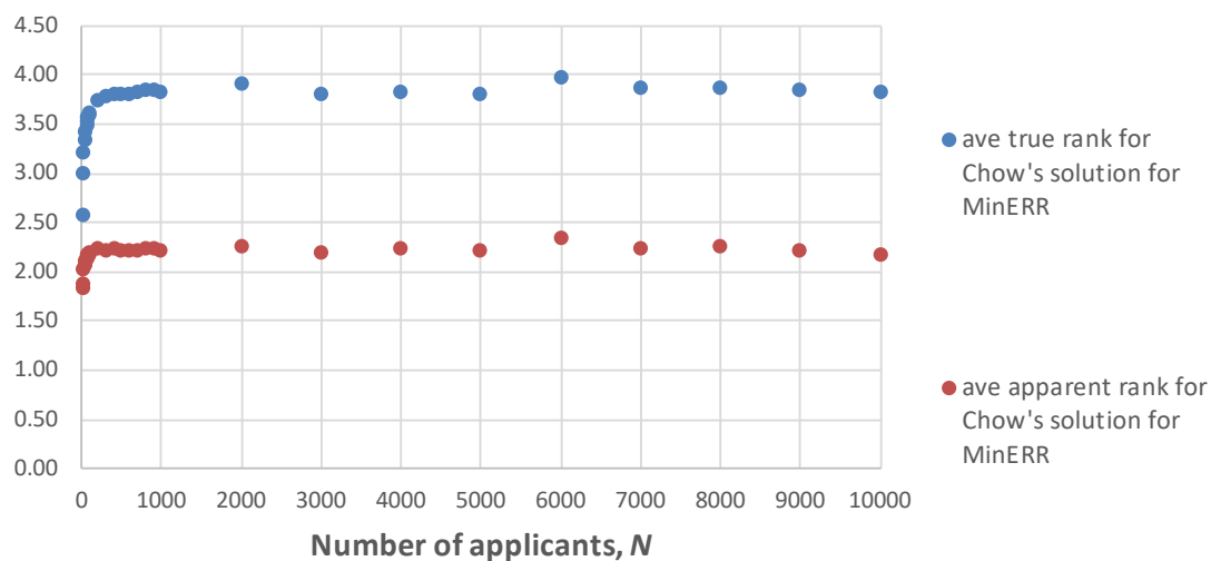
Figure 30. Expected relative true rank and apparent rank for Chow's solution for MinERR.
