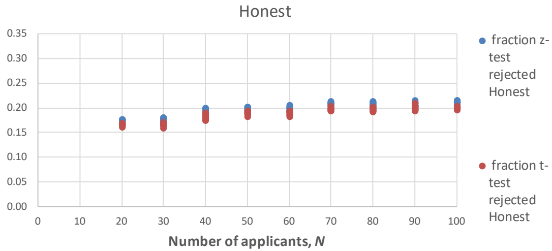
Figure 35a. Test of hypothesis reject rates for a range of N values for honest-only queues. Sample size n = 30 for z -test and t -test. For each value of N , points are plotted for five sets of tests, where each set obtained a reject rate based on 10^4 tests of hypothesis.
