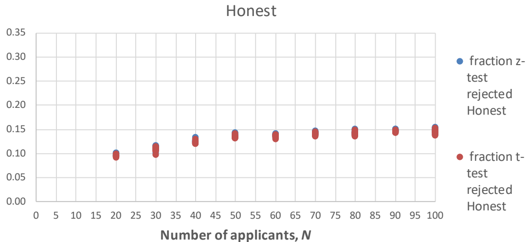
Figure 37. Test of hypothesis reject rates for a range of N values for honest-only queues. Sample size n = 100 for z -test and t -test. For each value of N , points are plotted for five sets of tests, where each set obtained a reject rate based on 10^4 tests of hypothesis.
