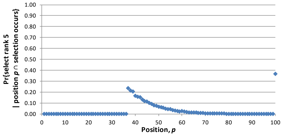
Figure 15d. For SPANS with N = 100 , probability that an applicant of rank r = 5 is selected, given the applicant is in position p and the DM makes a selection. Note that \Pr\{\text{select rank 5} \mid \text{position } p \cap \text{selection occurs}\} < \Pr\{\text{select rank 5} \mid \text{last position} \cap \text{selection occurs}\} for all p < 100 .
