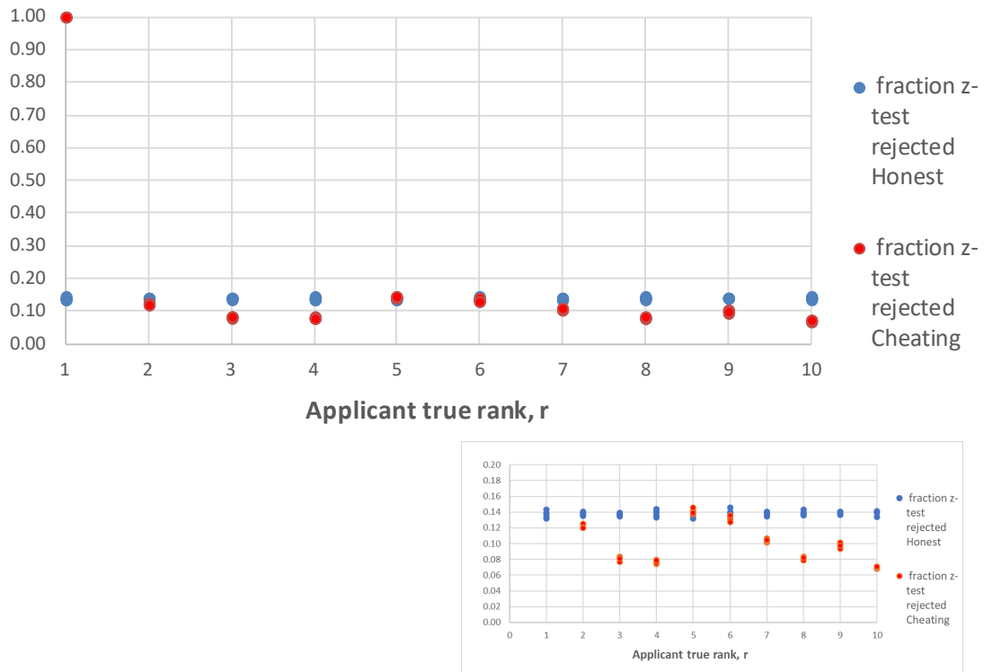
Figure 39b. Summary of reject rates for tests of hypothesis for honest-only queues and queues with CAs with ranks 1 through 10. N = 20 applicants and z-test sample size n = 50 . For each CA rank, points are plotted for five sets of tests, where each set obtained a reject rate based on 10^4 tests of hypothesis. An independent simulation of the honest-only queue was performed with each CA simulation. Inset is scaled to show more detail for CAs 2 through 10.
