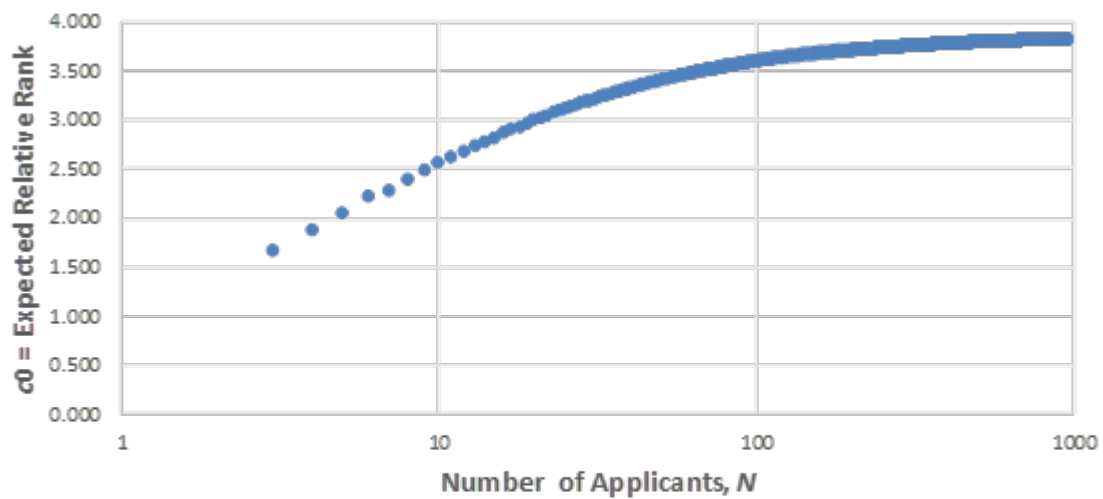
Figure 16a. The value of c_0 , the expected relative rank of the applicant selected using Chow's solution for MinERR payoff, as a function of N . Plot ends at N=955 where c_0 is within 1% of its upper bound of approximately 3.8695.
