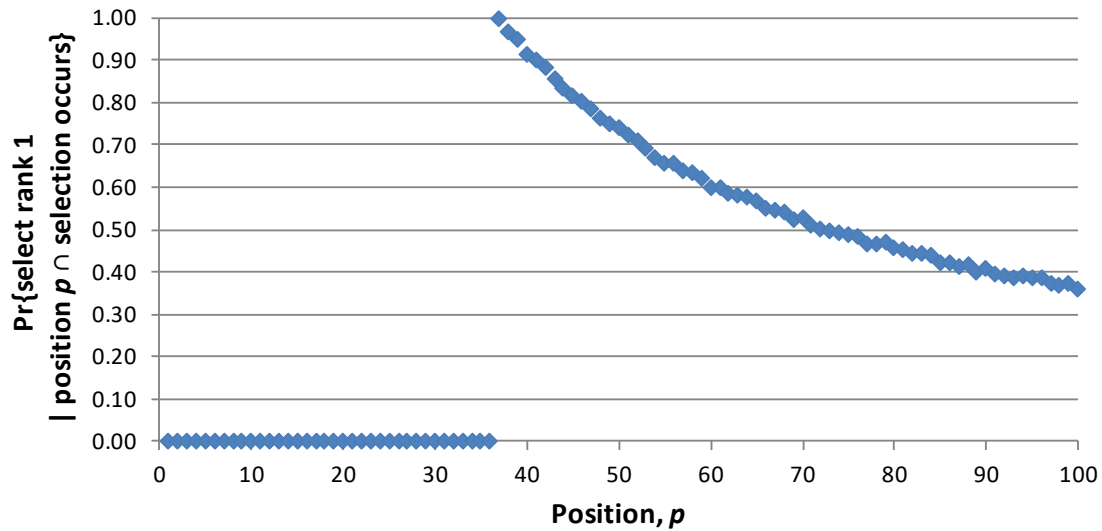
Figure 15a. For SPANS with N = 100 , probability that an applicant of rank r = 1 is selected, given the applicant is in position p and the DM makes a selection. Note that \Pr\{\text{select rank 1} \mid \text{position } p \cap \text{selection occurs}\} \geq \Pr\{\text{select rank 1} \mid \text{last position} \cap \text{selection occurs}\} for p = 37, 38, \dots 100 .
