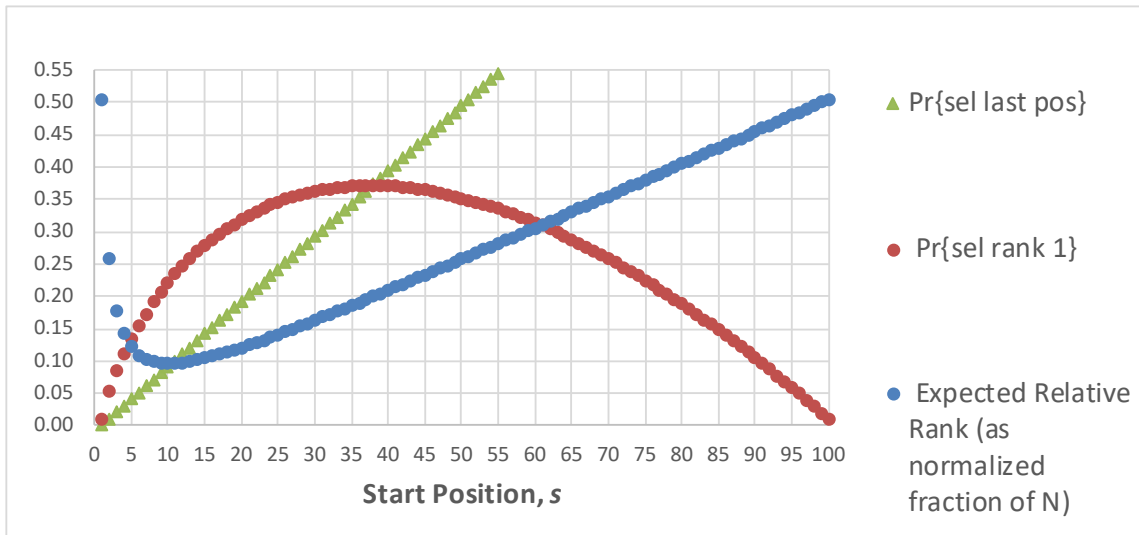
Figure 2. C2PS for MinERR payoff has sharp minimum but NBTB payoff has wider range around maximum. Probability of selecting last applicant increases linearly with start position. N=100 and results are based on 10^6 simulated random runs.
