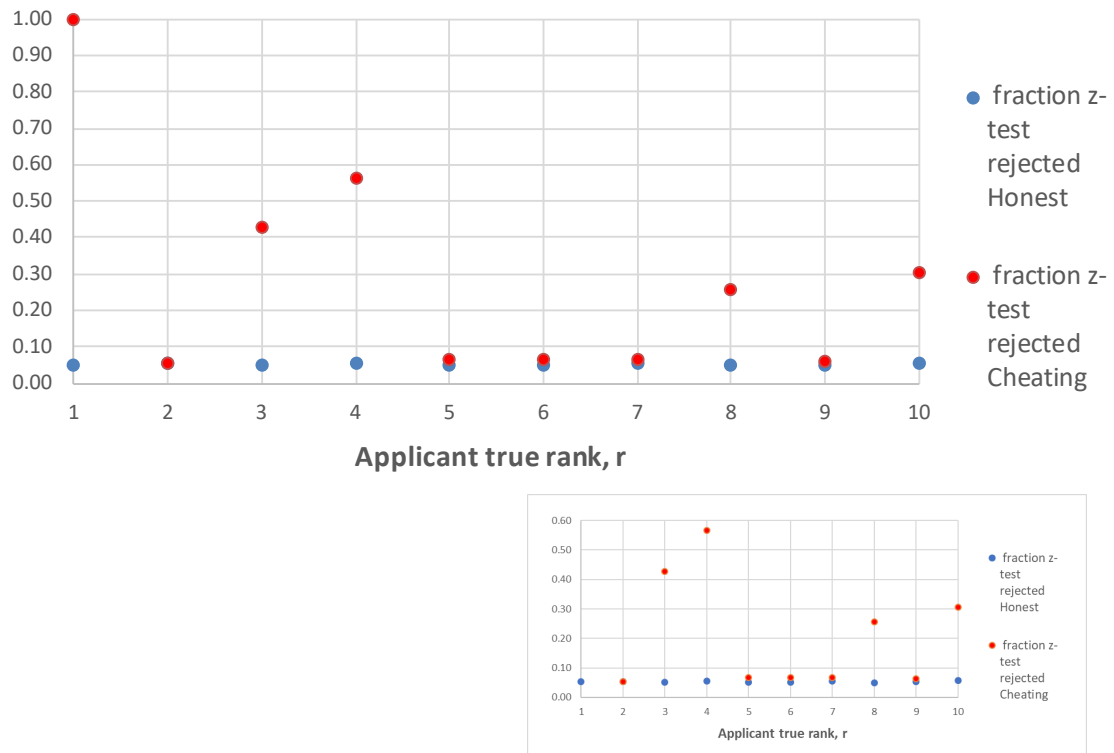
Figure 39d. Summary of reject rates for tests of hypothesis for honest-only queues and queues with CAs with ranks 1 through 10. N = 20 applicants and z -test sample size n = 1,000 . For each CA rank, points are plotted for one set of 10^4 tests of hypothesis. An independent simulation of the honest-only queue was performed with each CA simulation. Inset is scaled to show more detail for CAs 2 through 10.
