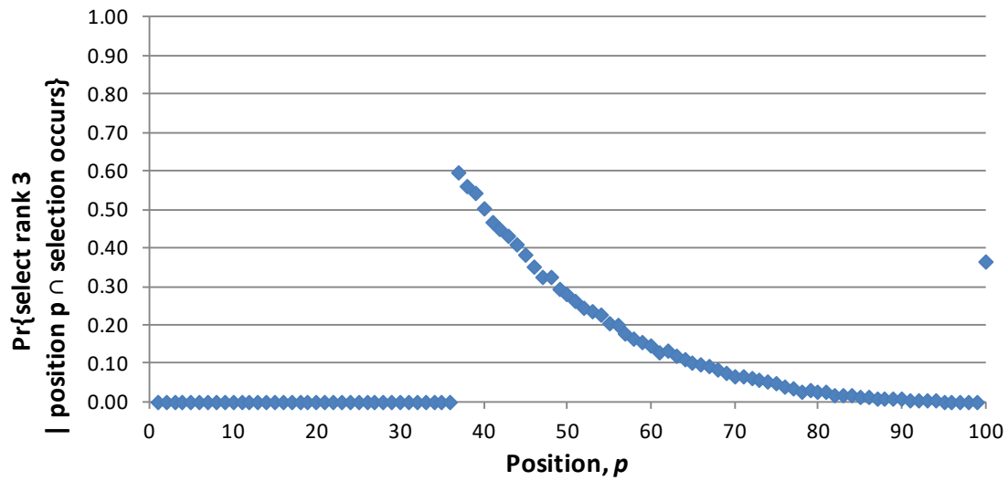
Figure 15c. For SPANS with N = 100 , probability that an applicant of rank r = 3 is selected, given the applicant is in position p and the DM makes a selection. Note that \Pr\{\text{select rank 3} \mid \text{position } p \cap \text{selection occurs}\} \geq \Pr\{\text{select rank 3} \mid \text{last position} \cap \text{selection occurs}\} for p = 37, 38, \dots 45 , and 100.
