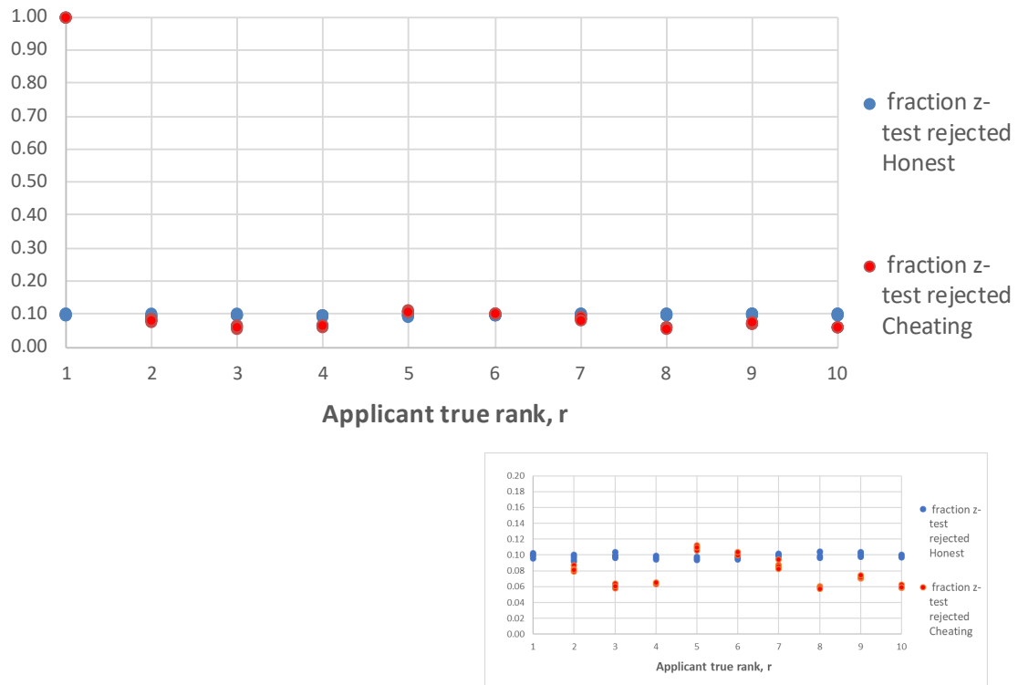
Figure 39c. Summary of reject rates for tests of hypothesis for honest-only queues and queues with CAs with ranks 1 through 10. N = 20 applicants and z-test sample size n = 100 . For each CA rank, points are plotted for five sets of tests, where each set obtained a reject rate based on 10^4 tests of hypothesis. An independent simulation of the honest-only queue was performed with each CA simulation. Inset is scaled to show more detail for CAs 2 through 10.
