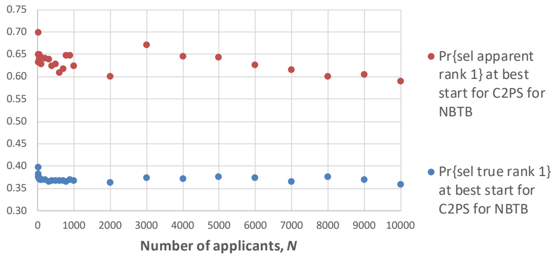
Figure 25. Probabilities of selection for true rank 1 and apparent rank 1 for C2PS for NBTB.
