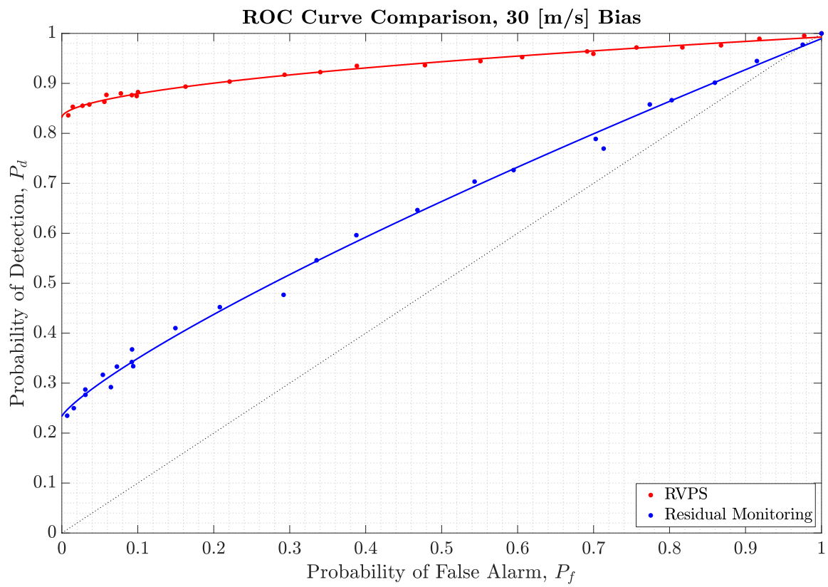
Figure 5.4: Fault detection ROC curve comparison, bias = 30 [m/s]
