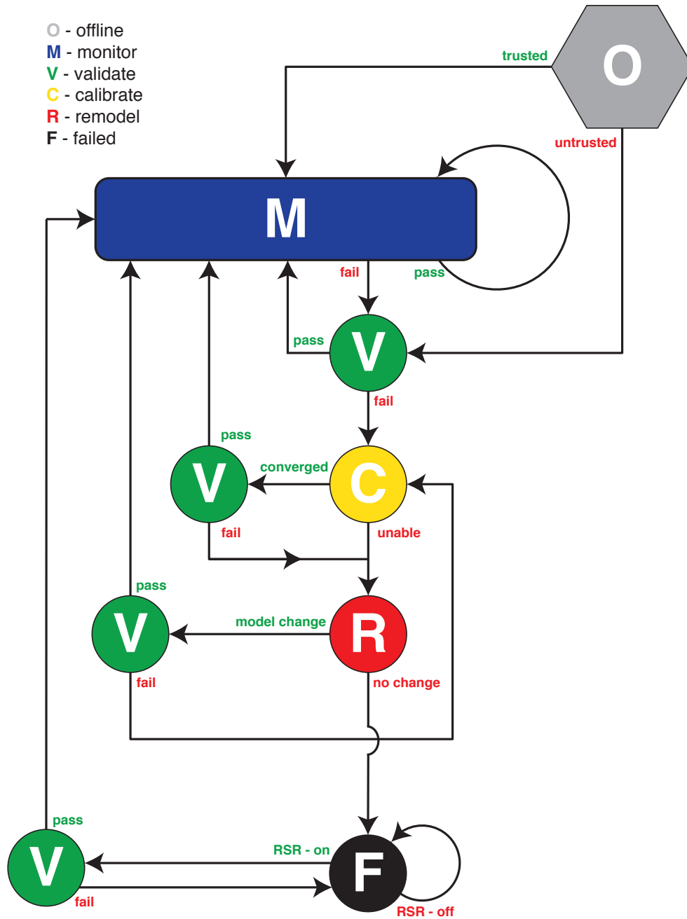
Figure 3.1: Proposed state transition diagram for ARMAS framework. New sensors (offline) begin in either validate or monitor mode. A failed monitoring test starts a calibration and remodeling loop, whose effectiveness is evaluated by the validation test. The loop continues until the validation test is passed or the sensor model selection is unchanged. Failed sensors can be periodically re-validated to recover from temporary anomalies using RSR.
