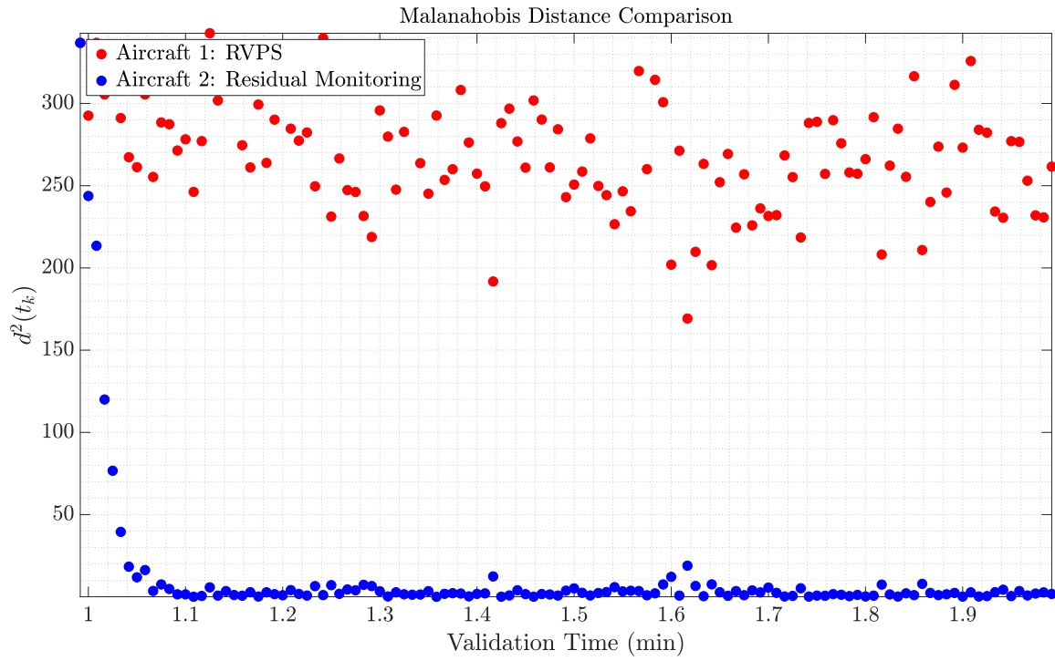
Figure 5.2: Example residual d^2 comparison, 2D velocity sensor, bias = 20 [m/s]
