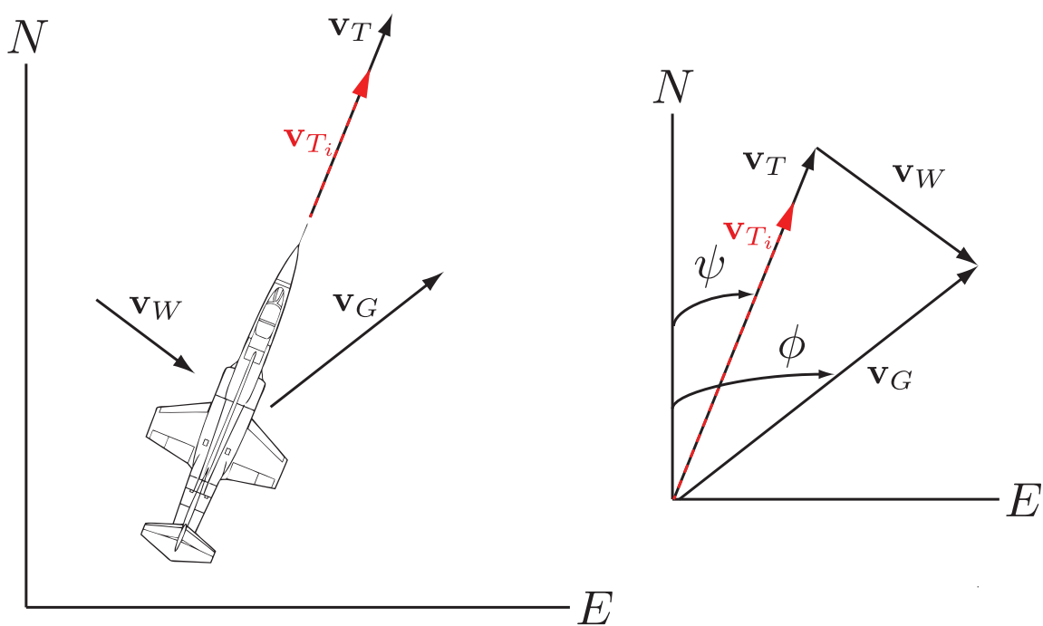
Figure 6.2: Illustration of the wind triangle.
