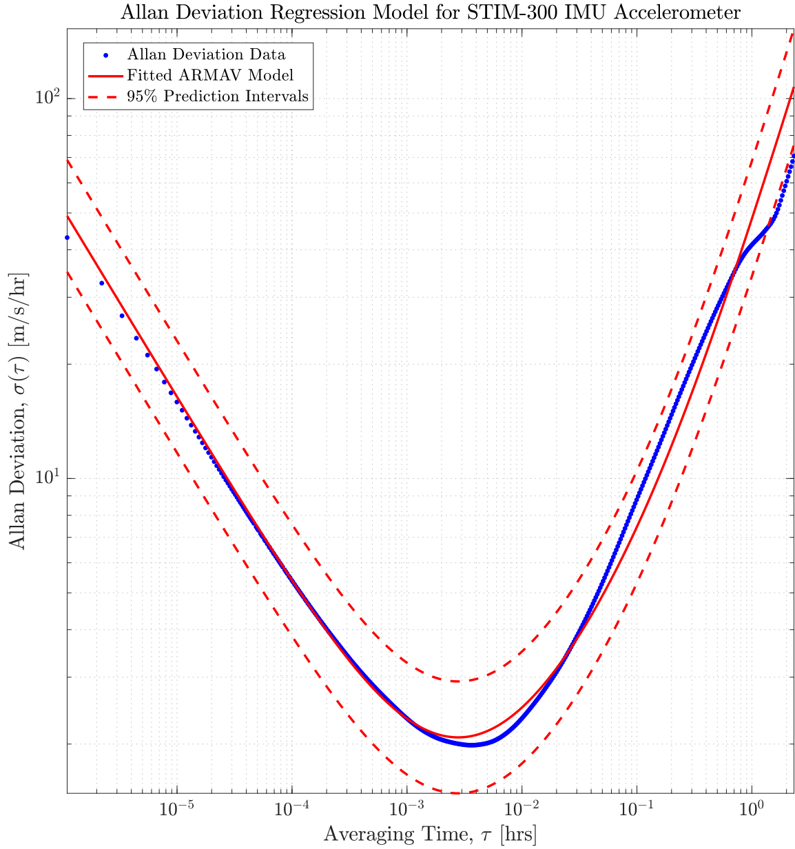
Figure 7.4: Illustration of ARMAV model on accelerometer Allan deviation measurements. As shown, ARMAV is able to accurately model the observed data with no need for human intervention, which directly enables the accurate estimation of the necessary noise strength coefficients. The resulting 95% prediction intervals cover a possible range of Allan deviation observations for each \tau .
