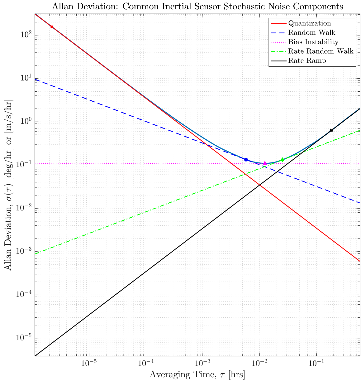
Figure 7.2: Illustration of Allan variance slope method for common stochastic noise processes.
