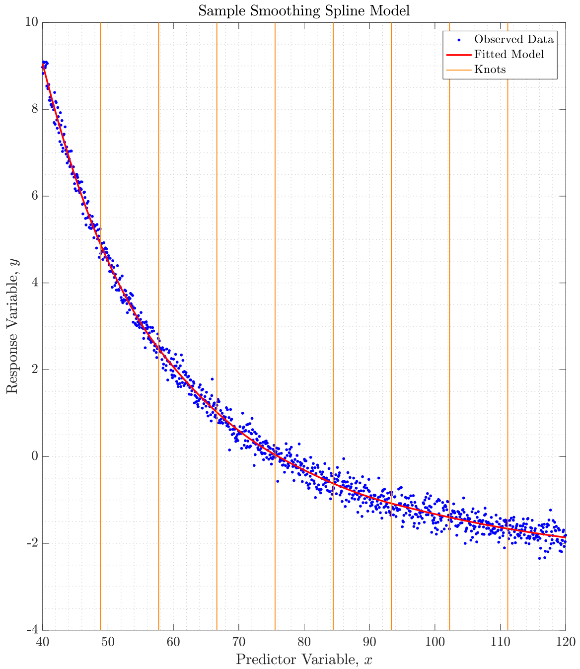
Figure 2.1: Example of a fitted smoothing spline model with eight knots selected using quantiles [89]. The second-order polynomial smoothing spline is able to model an exponential functional form with no prior knowledge.
