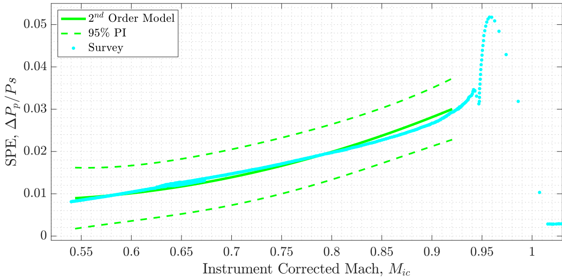
Figure 6.8: Results from Level Turn test points.
