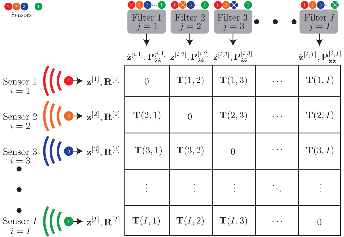
Figure 4.1: Illustration of the multi-sensor multi-filter test statistic matrix, \mathbf{T} .
