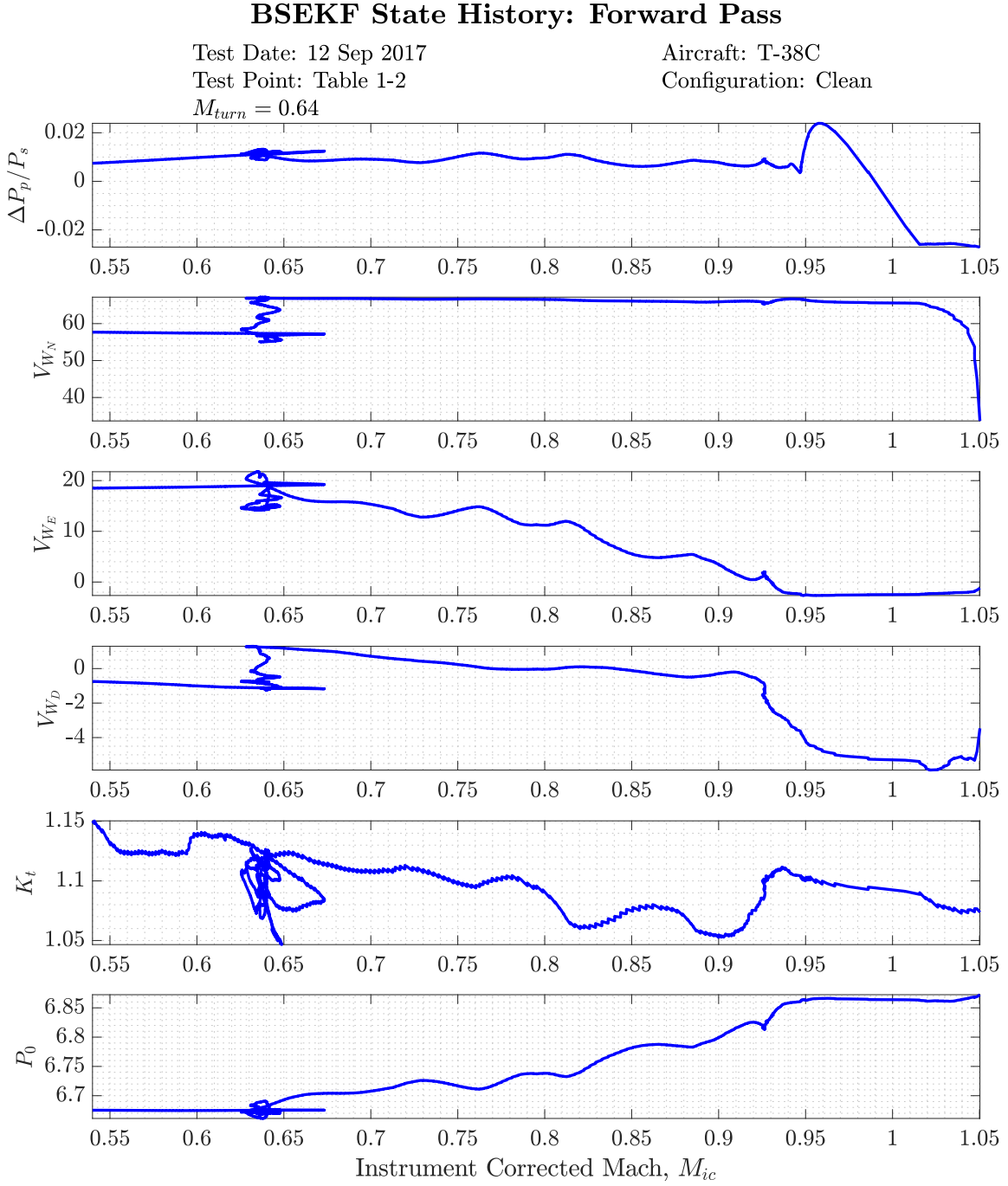
Figure 6.4: Illustration of JMOSS BSEKF output on forward pass.
