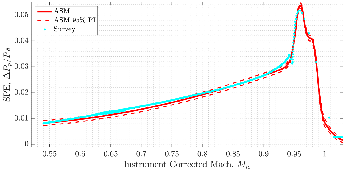
Figure 6.6: JMOSS results for a single test point.
