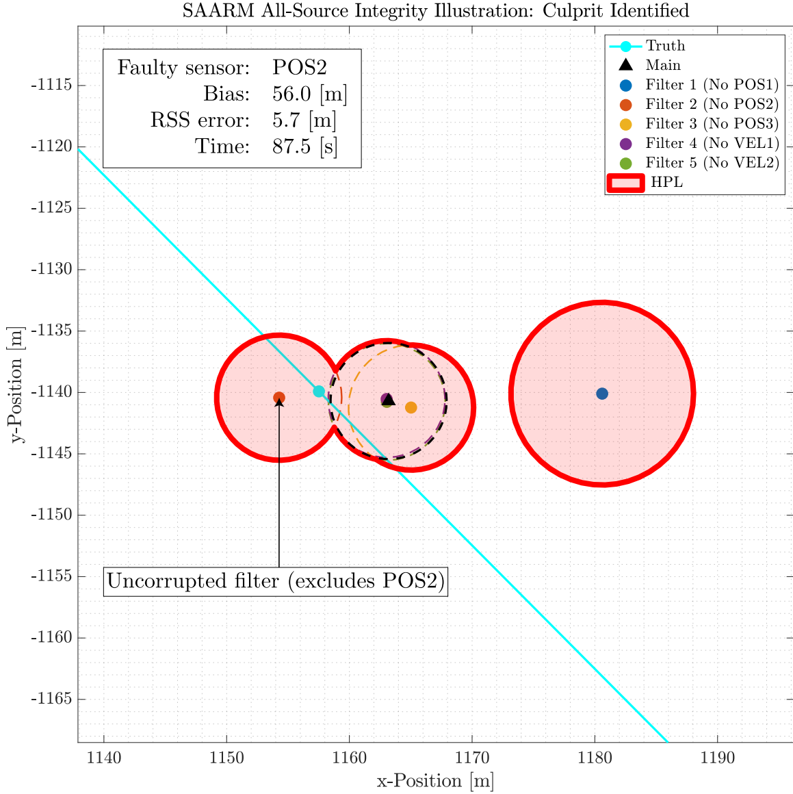
Figure 4.5: Example SAARM HPL: Culprit identified. In this example, a 56 [m] bias is affecting the POS2 sensor, a fault has been detected and the culprit has been identified (there is a single zero-entry in \mathbf{s} ), which is shown to the user as a red HPL. All filters except Filter 2 are corrupted. The HPL is comprised of the union of the 95% position error ellipses from all filters, and it is guaranteed to contain the true position at least 95% of the time since one of the filters is guaranteed to be uncorrupted. Immediately after this time step, the POS2 sensor is taken offline, and a new set of filters is re-spawned from Filter 2.
