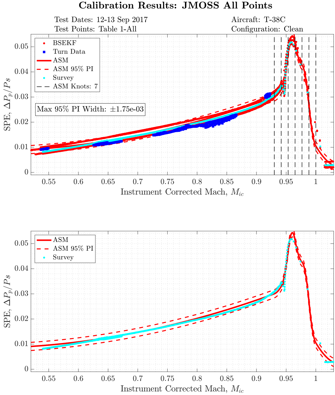
Figure 6.7: JMOSS results when combining all test points.
