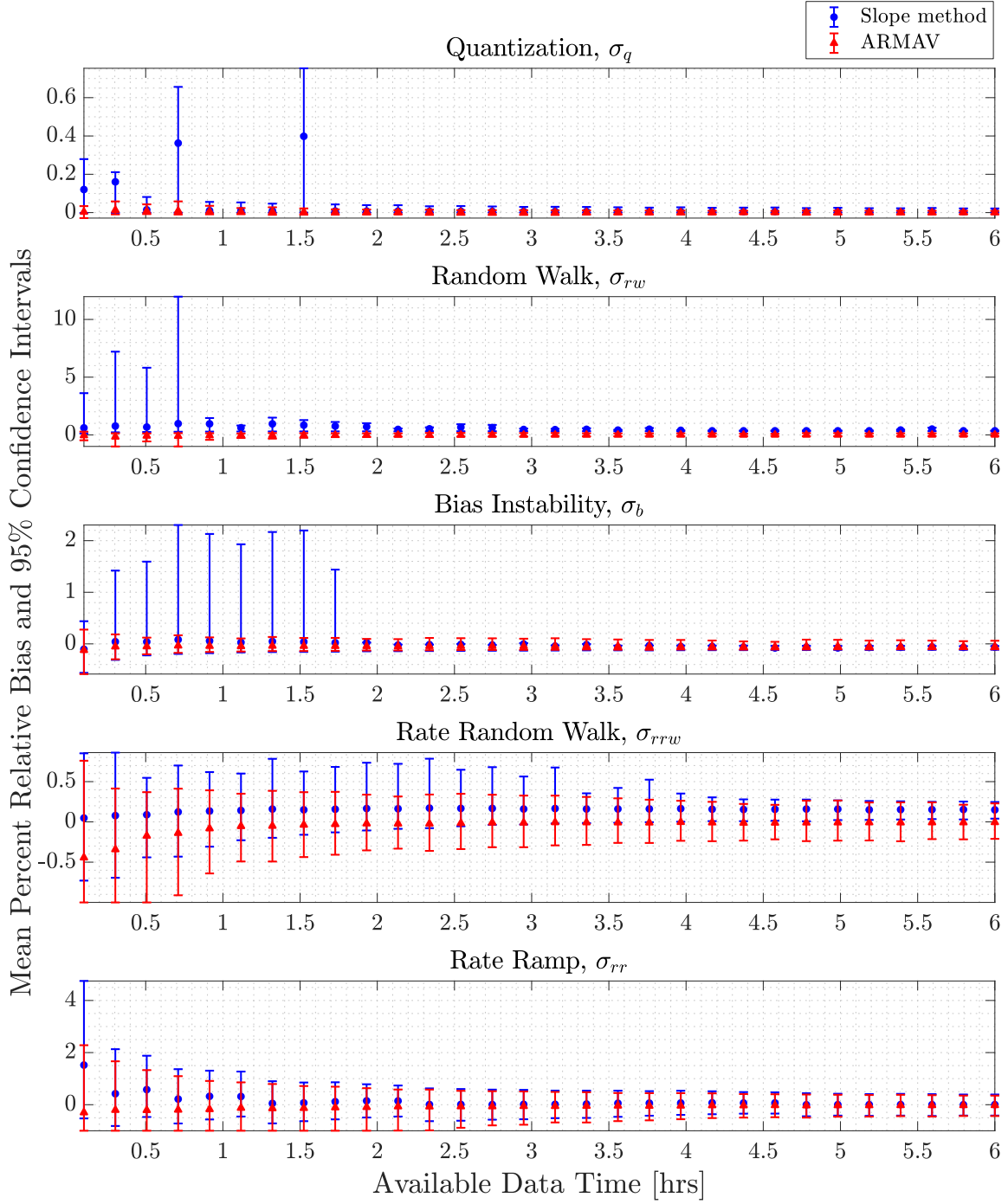
Figure 7.3: Monte-Carlo comparison between slope and ARMAV methods. The ARMAV method produced significantly more accurate, and stable results (in terms of variance) as indicated by the confidence intervals, especially as the length of available data decreased below 2 hours.
