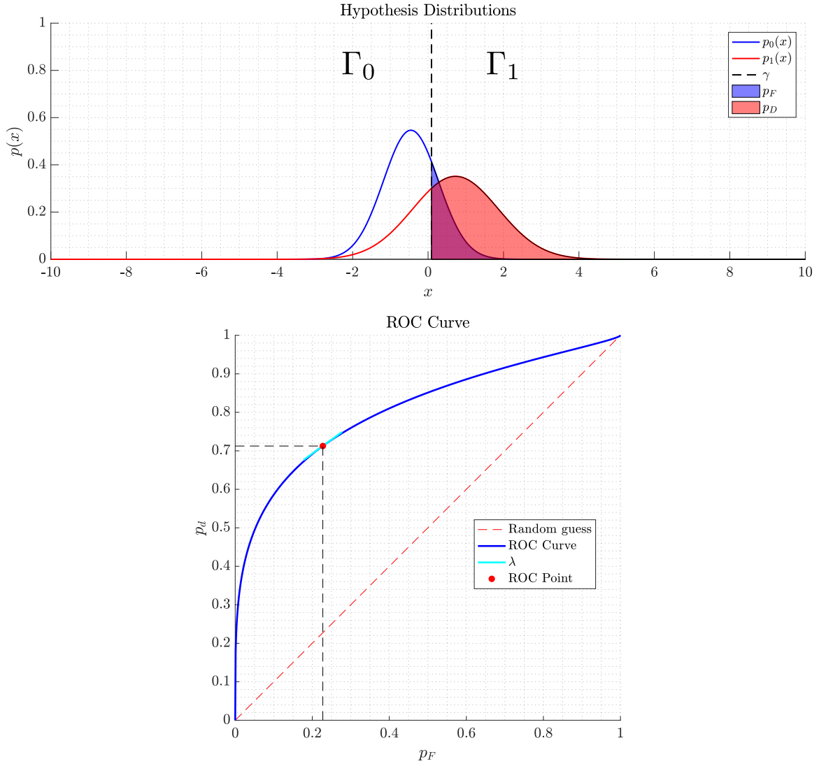
Figure 2.2: Example LRT for binary detection using univariate Gaussian distributions. The \Gamma_1 region corresponds to x > \gamma and drives p_D and p_F based on which distribution is integrated. The ROC curve on the bottom graph illustrates the possible combinations of p_D and p_F for the given problem as well as the operating point based on the chosen \gamma . The corresponding \lambda value is equal to the ROC slope at the operating point.
