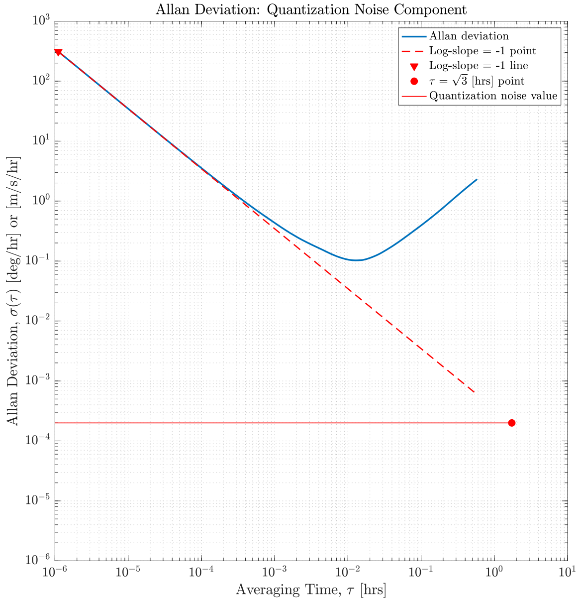
Figure 7.1: Illustration of Allan variance slope method for quantization noise.
