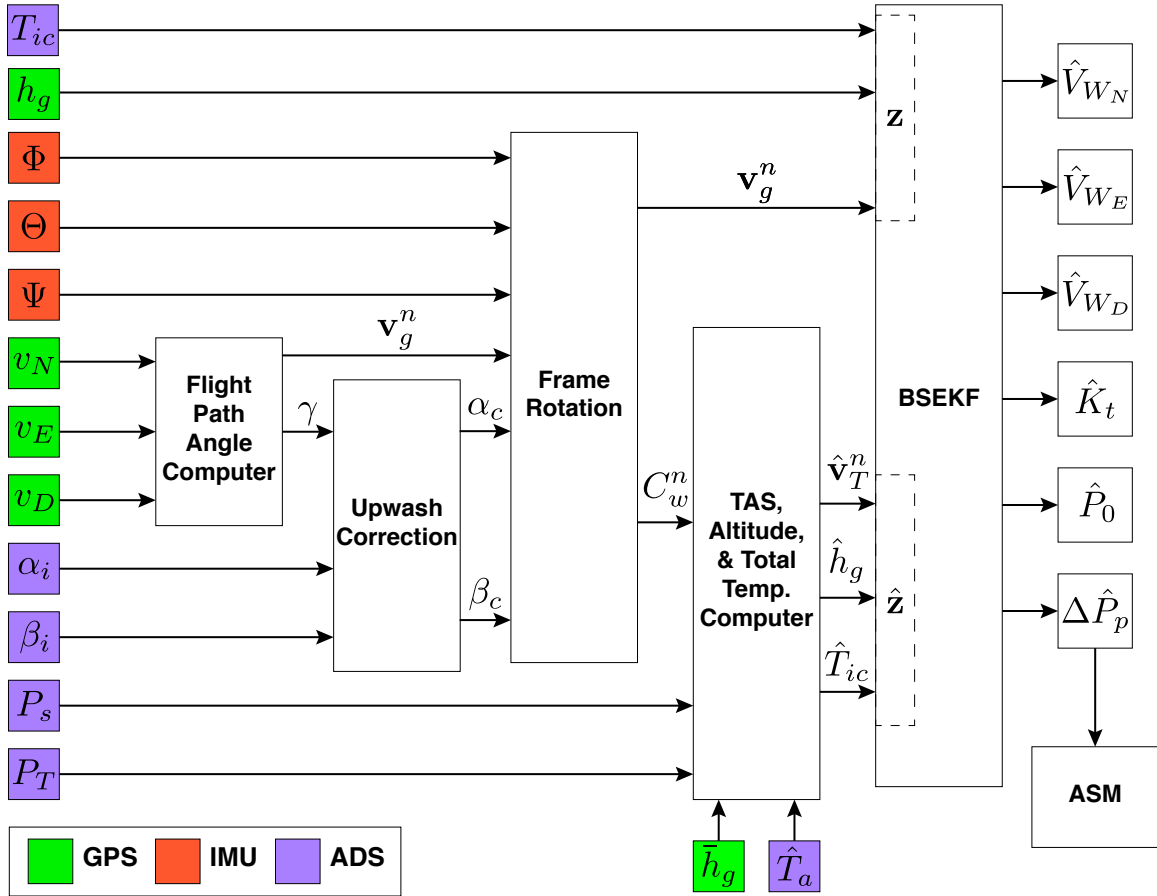
Figure 6.3: Data processing flow for JMOSS algorithm.
