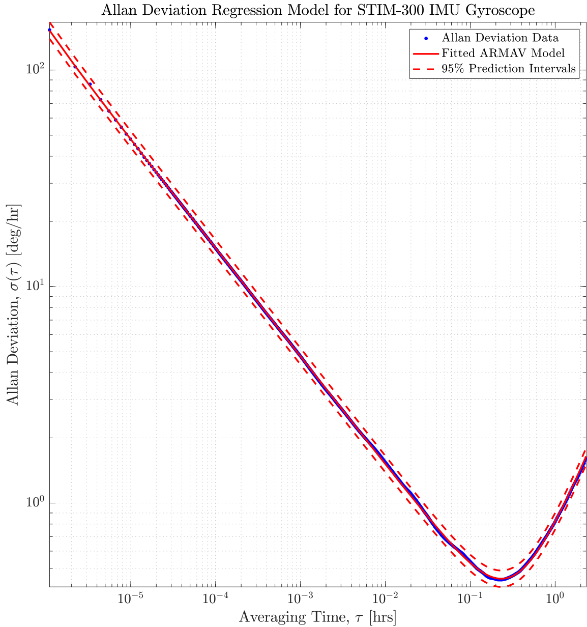
Figure 7.5: Illustration of ARMAV model on gyroscope Allan deviation measurements. As shown, ARMAV is able to accurately model the observed data with no need for human intervention, which directly enables the accurate estimation of the necessary noise strength coefficients. The resulting 95% prediction intervals cover a possible range of Allan deviation observations for each \tau .
