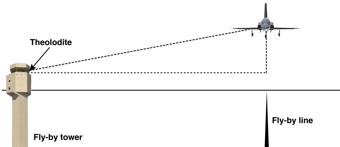
Figure 6.1: Illustration of the Tower Fly-by.
