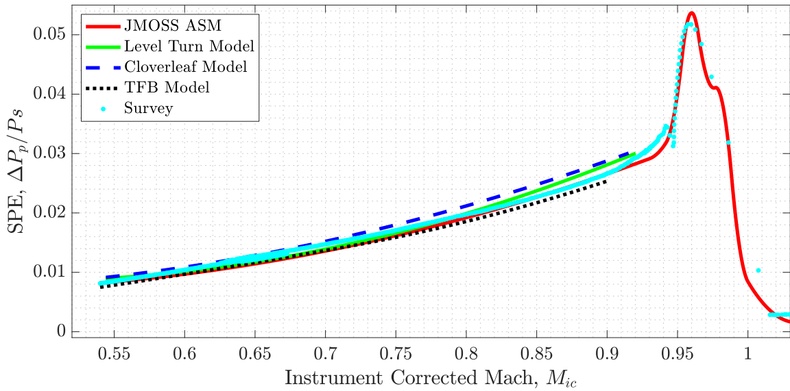
Figure 6.11: Results comparison across all methods.
