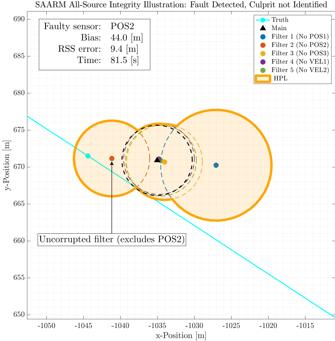
Figure 4.4: Example SAARM HPL: Unidentified culprit. In this example, a 44 [m] bias is affecting the POS2 sensor, and a fault has been detected (at least one entry in \mathbf{s} is non-zero), but no culprit has been identified (there is more than one zero entry in \mathbf{s} ), which is shown to the user as an orange HPL. All filters except Filter 2 are corrupted. The HPL is comprised of the union of the 95% position error ellipses from all filters, and it is guaranteed to contain the true position at least 95% of the time since one of the filters is guaranteed to be uncorrupted.
