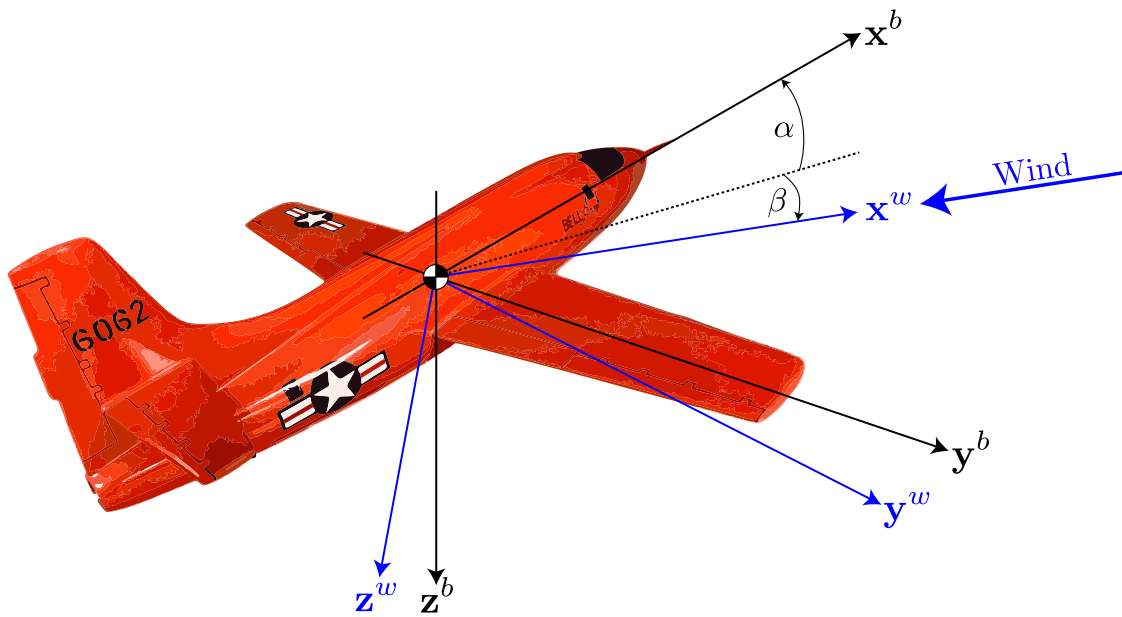
Figure 2.4: Illustration of aircraft b -frame and w -frame. Both frames are rigidly attached to the aircraft's center of mass. The b -frame and w -frame are rotated by Angle of Attack, \alpha , and Angle of Sideslip, \beta , due to the relative orientation between the aircraft body and the wind mass.
