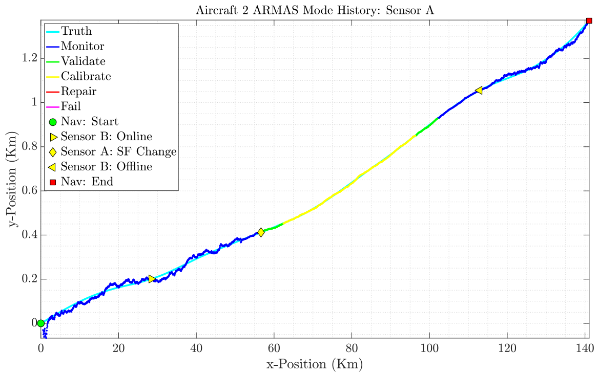
Figure 3.6: ARMAS mode history for Sensor A, Example 2.
