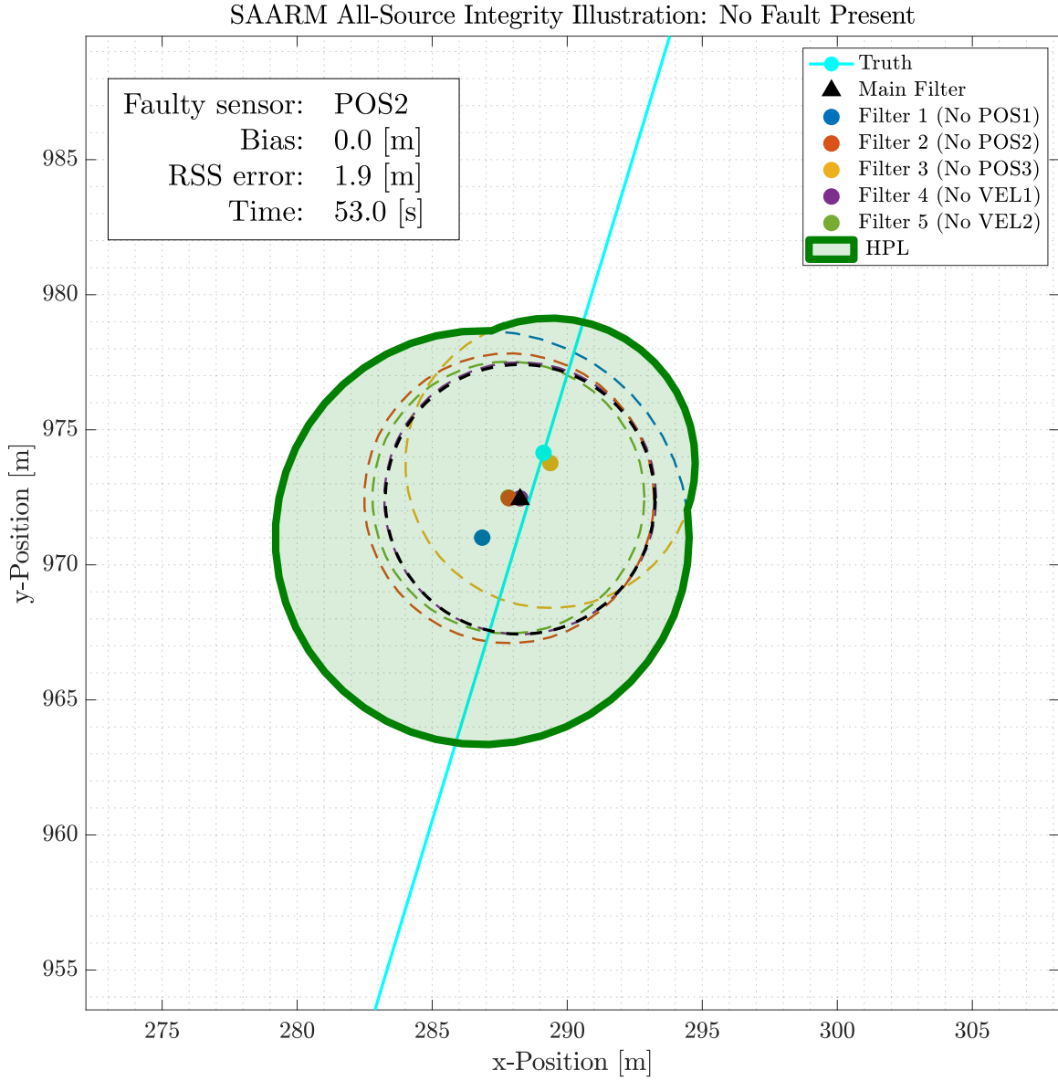
Figure 4.2: Example SAARM HPL: No fault present. In this example, there is no fault induced into any of the five sensors, and no fault has been detected (all entries in s are zero), which is shown to the user as a green HPL. All filters are uncorrupted. The HPL is comprised of the union of the 95% position error ellipses from all filters, and contains the true position at least 95% of the time.
