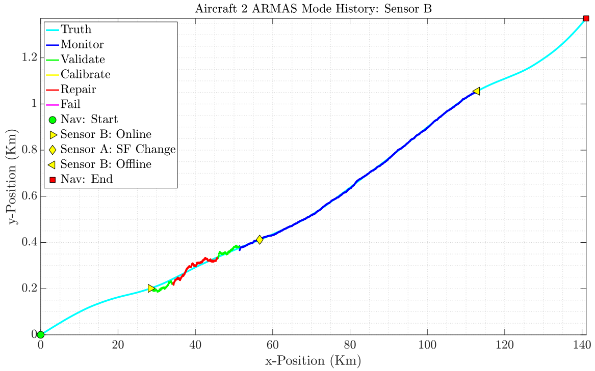
Figure 3.5: ARMAS mode history for Sensor B, Example 2.
