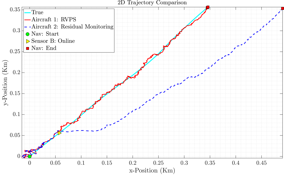
Figure 5.1: Example 2D trajectory comparison, 2D velocity sensor, bias = 20 [m/s]
