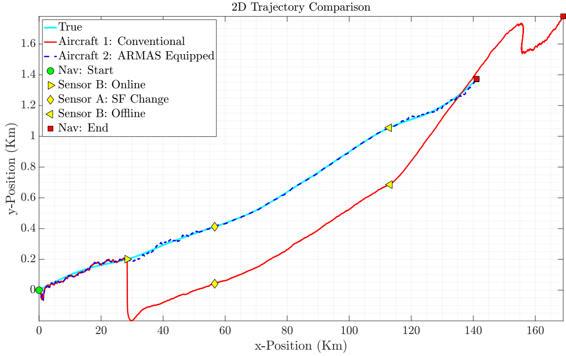
Figure 3.4: Trajectory comparison between Aircraft 1 and Aircraft 2, Example 2.
