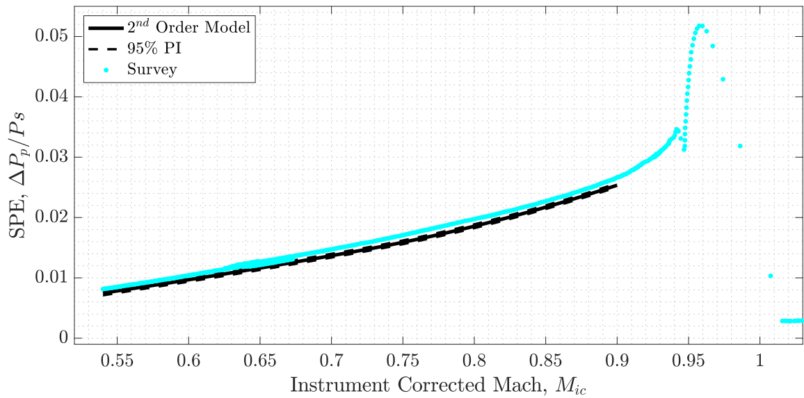
Figure 6.10: Results from Tower Fly-by test points.
