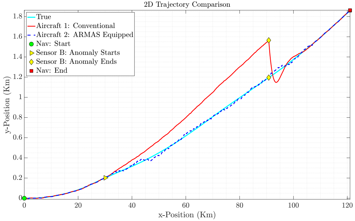
Figure 3.2: Trajectory comparison between Aircraft 1 and Aircraft 2, Example 1.
