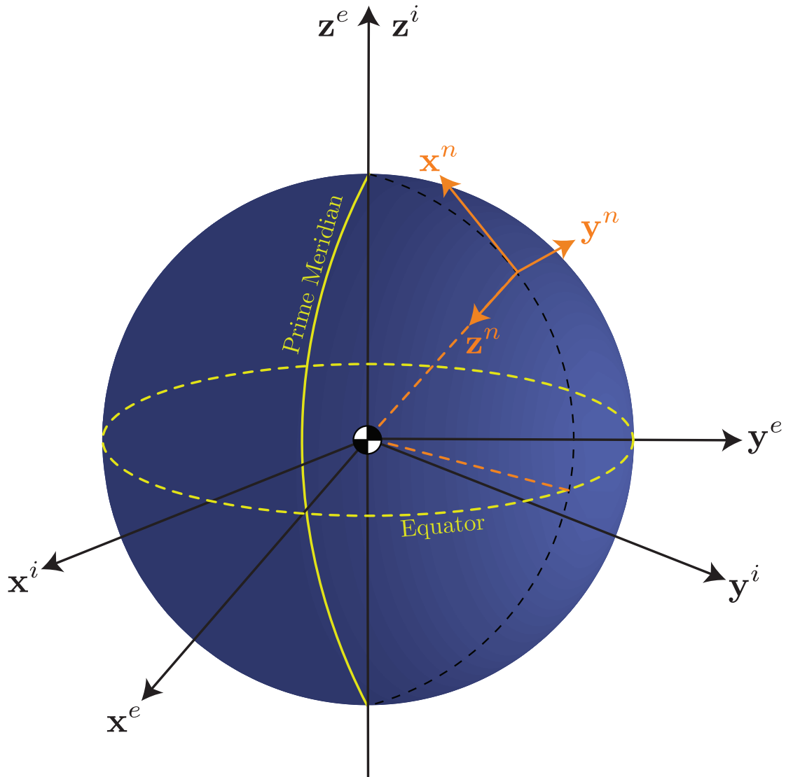
Figure 2.3: Illustration of Earth centered i -frame, e -frame, and n -frame. The e - and i -frames are rigidly attached to the Earth's center of mass, while the n -frame is attached to the surface of the Earth. The i -frame is non-rotating with respect to inertial space, while the e -frame rotates along with the Earth's rotation. The n -frame is aligned with north, east, and local gravity vectors.
