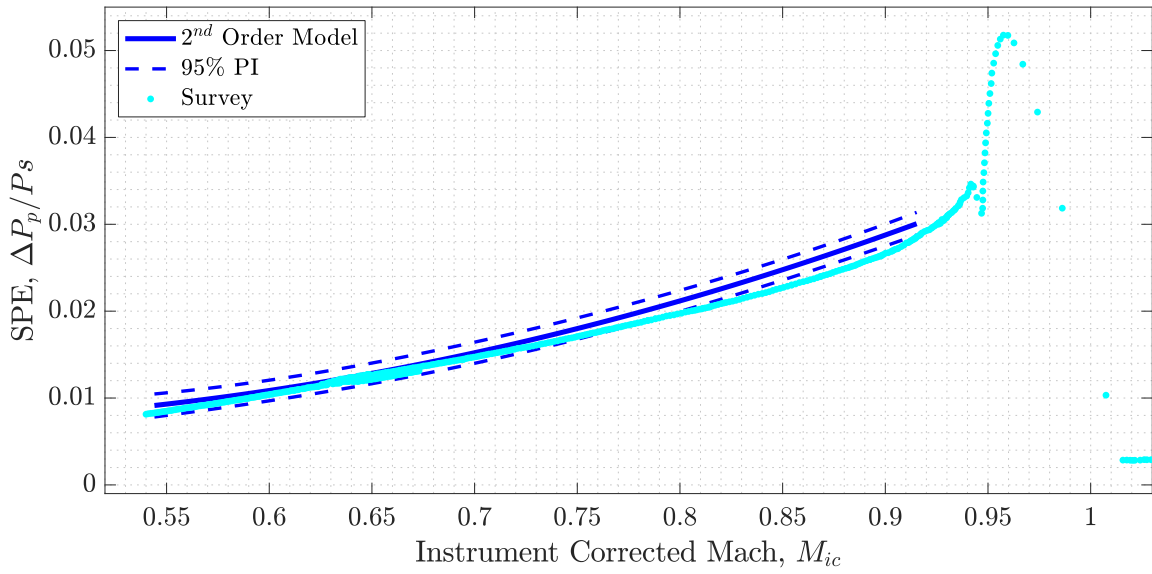
Figure 6.9: Results from Cloverleaf test points.
