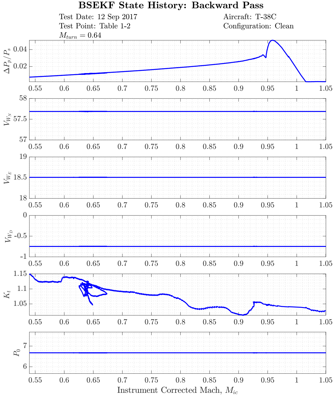
Figure 6.5: Illustration of JMOSS BSEKF output on backward pass.
