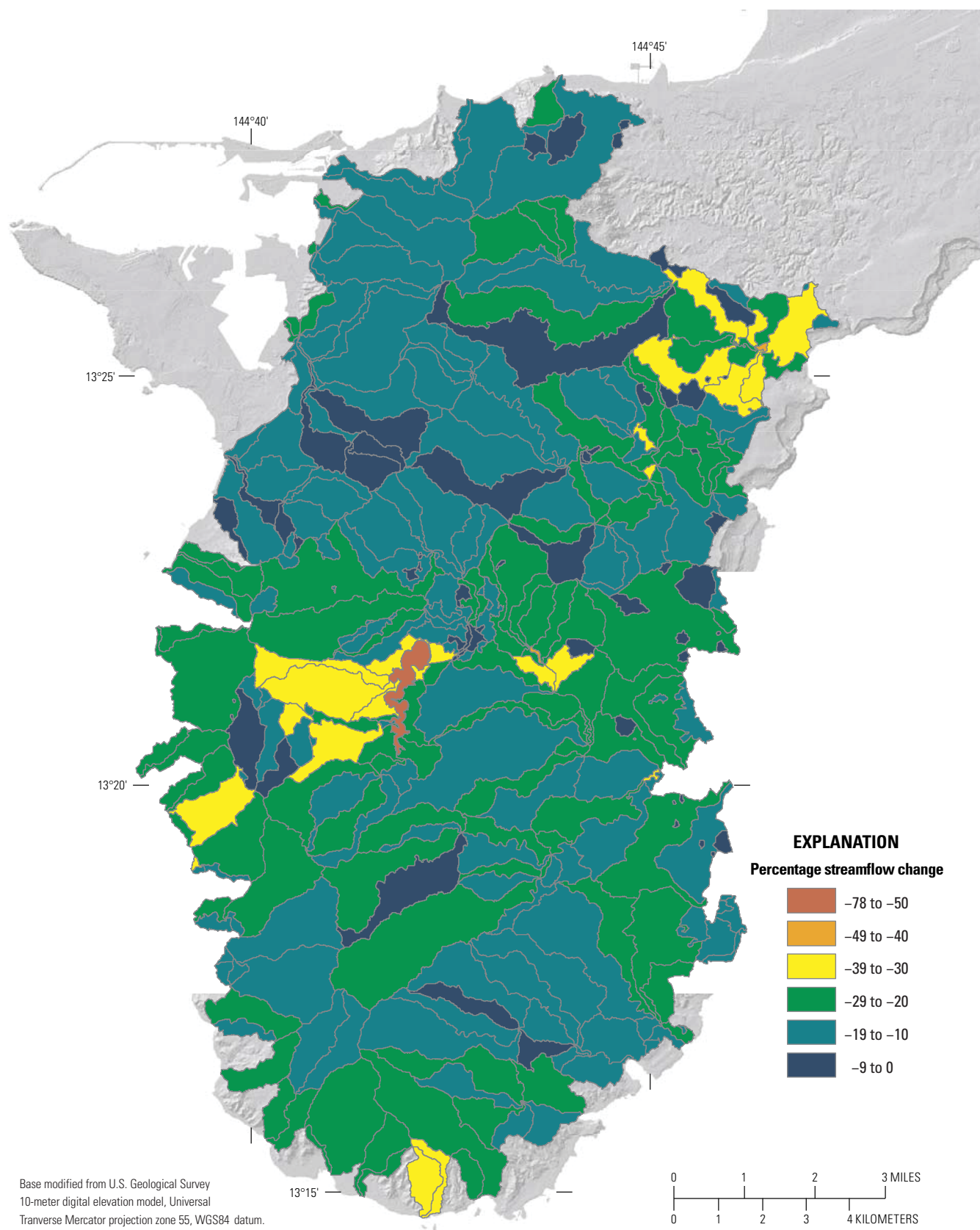
Figure 17. Map of southern Guam showing percentage streamflow change by hydrologic response unit (HRU) in the PRMS_2016 model for the scenario Representative Concentration Pathway 8.5. Fena Valley Reservoir modeled regions compare the years 1998–2009 with 2088–2099 and all other modeled regions compare the years 1990–2009 with 2080–2099.
