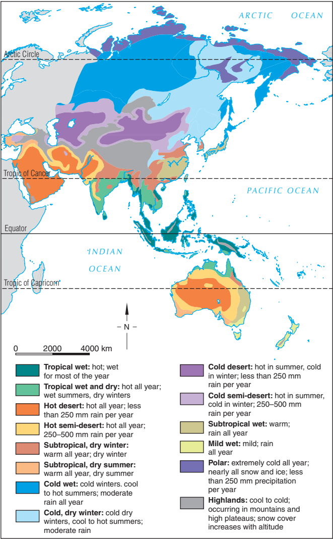
Figure 2.1 Climates of the Asia-Pacific Region Tend to Be Tropical and Wet
