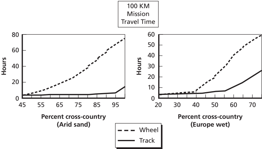
Figure 2.3 Travel Time for Different Terrain Types, Showing Increasing Delays with Wheeled Vehicles as Surface Becomes More Challenging
