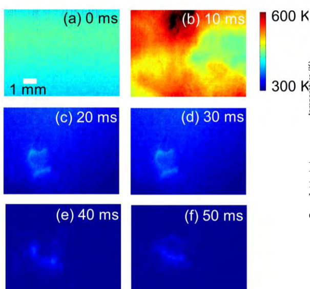
Fig. 11. Selected MWIR video images at 10 ms intervals from a 40'' impact with a polymer-encased 1 mm HMX crystal.
