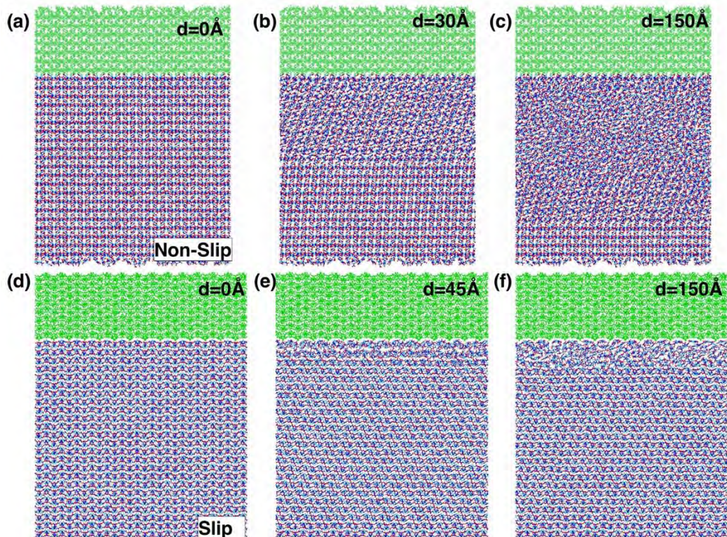
Figure 21: Effects of sliding friction on non-slip plane (100) [010] (a)-(c) and on slip plane (010) [001] (d)-(e). Here top block is shown is green color and is moved at a constant velocity of 100m/sec or 40m/sec.
