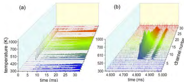
Fig. 8. Output of the linear MWIR array during a 40" drop impact with the polymer-encased 0.5 mm RDX crystal, obtained simultaneously with the video images in Fig. 5. The linear array is measuring the temperature in a strip 0.5 mm wide running through the middle of the crystal. (a) The full 32 ms record shows an instantaneous fast explosion at about 5 ms and a much slower burning lasting many tens of milliseconds. (b) Same record on an expanded scale showing the two-part explosion.
