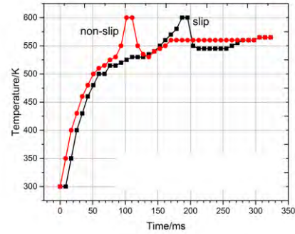
Fig. 25. Results of anisotropic rubbing of RDX crystal. When rubbed along the [001] direction, the non-slip direction makes the crystal explode much faster.
