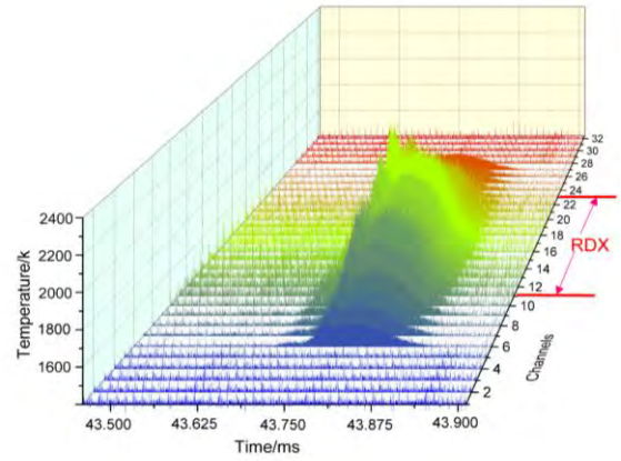
Fig. 24 Much faster thermal images of an RDX crystal exploding, obtained using the linear array.
