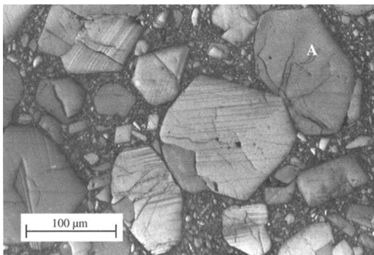
Figure 1.1 Microstructure of HMX bases polymer-bonded explosive
