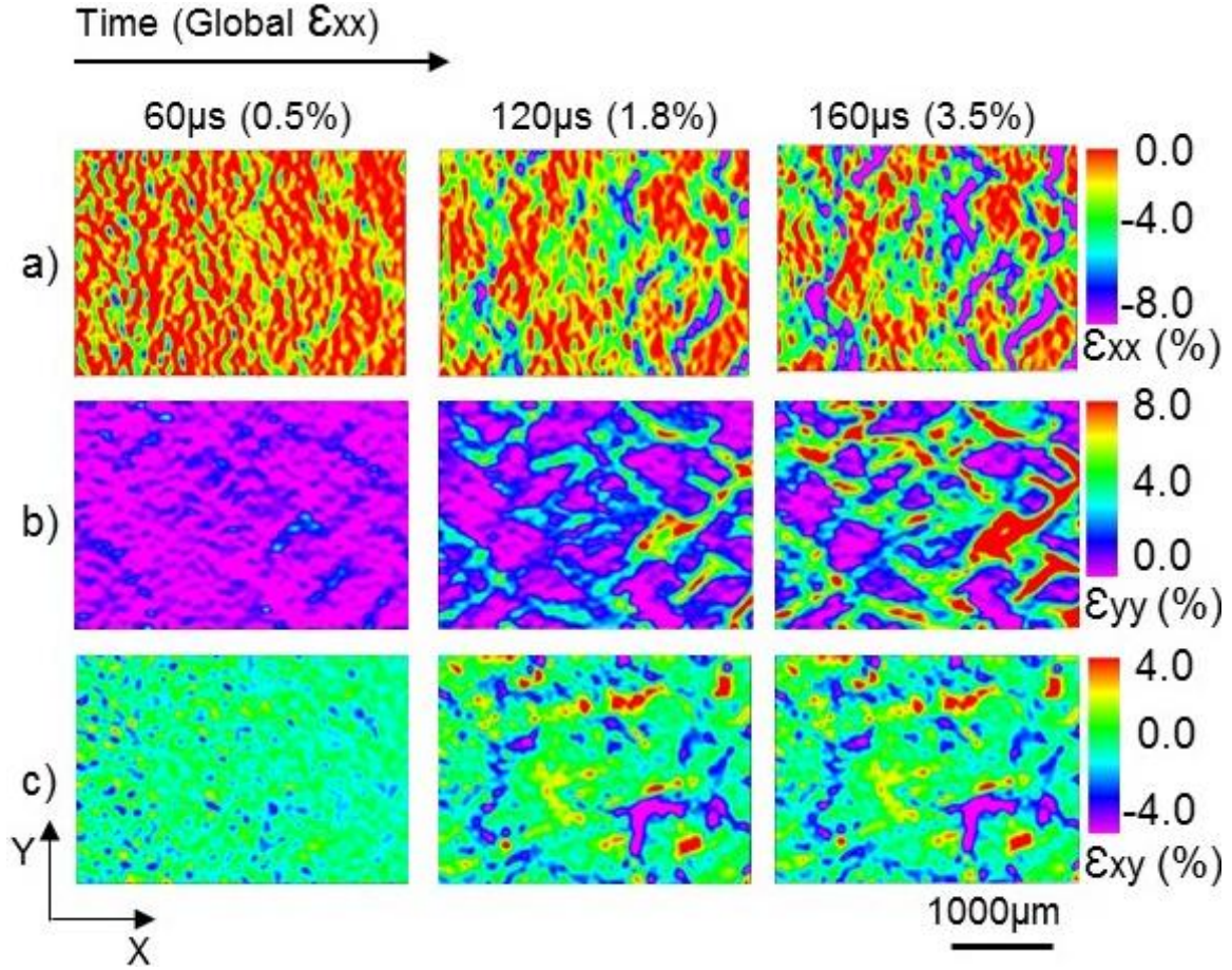
Figure 3.5 Local strain at different time (60μs, 120 μs, 160 μs) and global axial strains (0.5%, 1.8%, 3.5%), (a) local axial strain field, (b) local transverse strain field, (c) local shear strain field.
