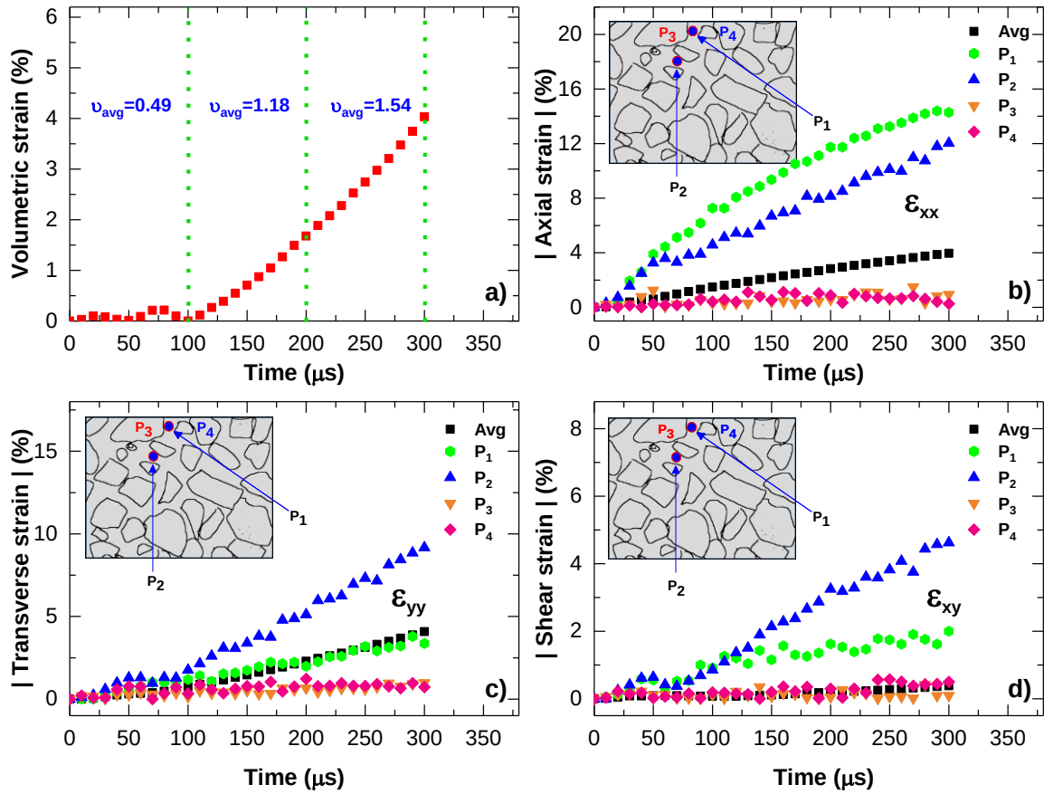
Figure 4.10 (a) Volumetric strain and average Poisson's ratio, (b) Axial strain evolution with time at points P 1 , P 2 , P 3 , and P 4 . The location the points are shows in inset figure of microstructure (c) transverse strain evolution with time at points P 1 , P 2 , P 3 , and P 4 . The location the points are shows in inset figure of microstructure, (d) shear strain evolution with time at points P 1 , P 2 , P 3 , and P 4 . The location the points are shows in inset figure of microstructure.
