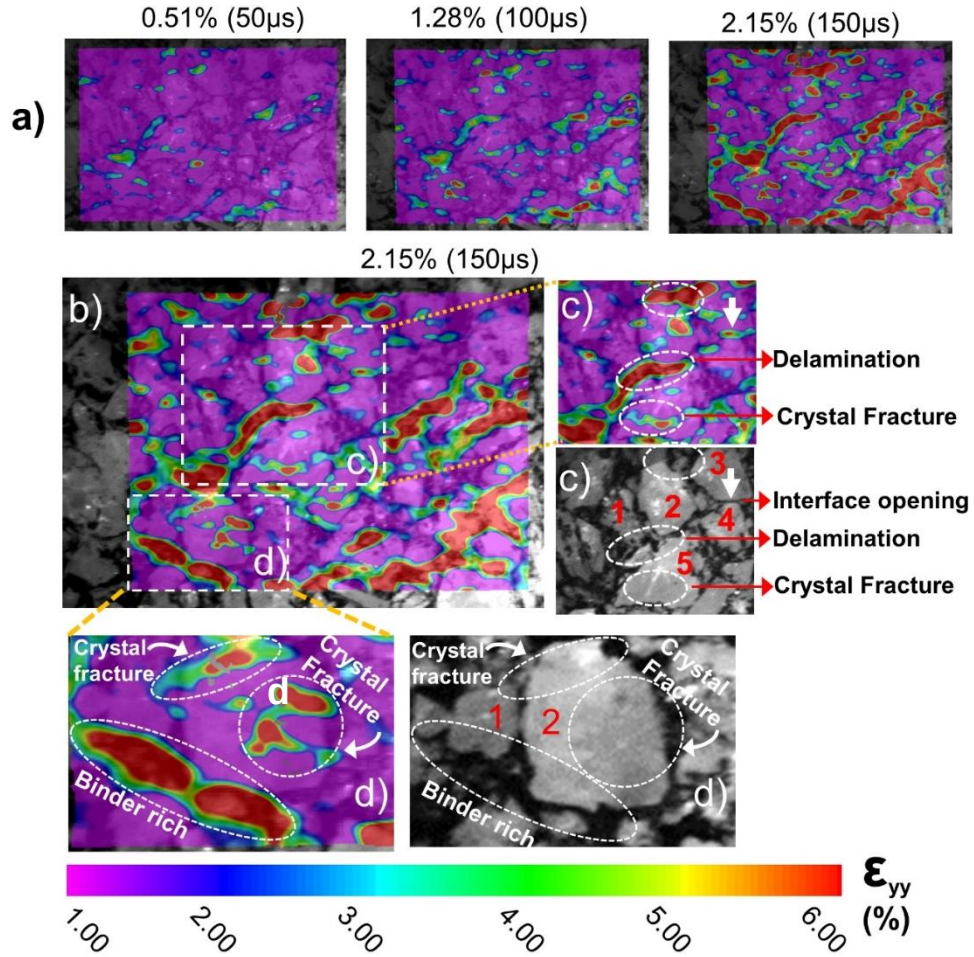
Figure 4.11 (a) Transverse strain evolution (50, 100 and 150 \mu\text{s} ), (b) Magnified view of the transverse strain field at t=150 \mu\text{s} , (c) The strain field and the microstructure of the highlighted area shows the crystal fracture and debonding, (d) strain field and microstructure of the highlighted area shows strain localization at the binder rich area and crystal fracture
