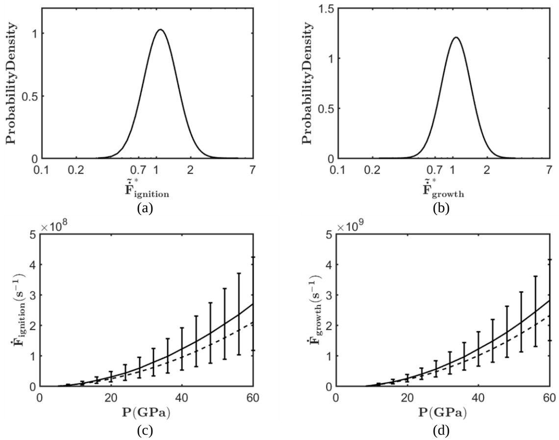
Figure 11. Probability density functions (a) \tilde{F}_{\text{ignition}}^* and (b) \tilde{F}_{\text{growth}}^* computed using Eqn. (9). Figure (c) shows the surrogates \tilde{F}_{\text{ignition}}(P_s; \mu_\pi) (in dotted lines) and \tilde{F}_{\text{ignition}}(P_s) (in solid lines). Figure (d) shows the surrogates \tilde{F}_{\text{growth}}(P_s; \mu_\pi) (in dotted lines) and \tilde{F}_{\text{growth}}(P_s) (in solid lines). The error bars in (c) and (d) represent the 90% confidence intervals with equal tail sets for \tilde{F}_{\text{ignition}}(P_s) and \tilde{F}_{\text{growth}}(P_s) .
