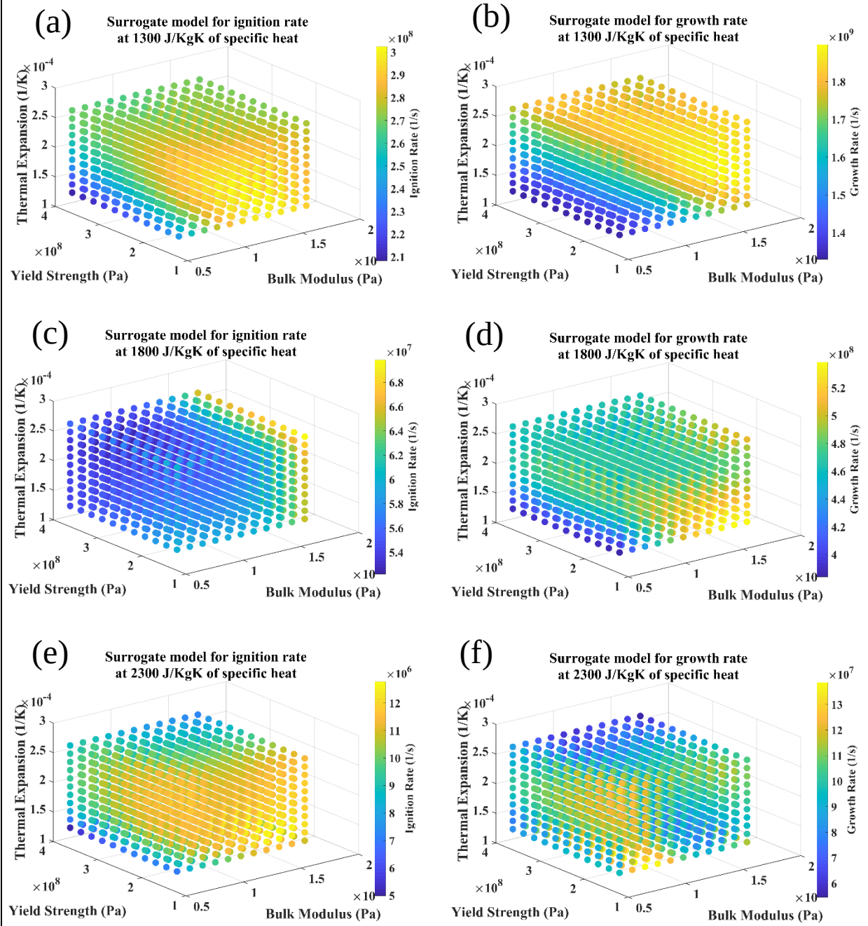
Figure 4. Surrogate models for \dot{F}_{ignition} and \dot{F}_{growth} constructed using the DKG method, as functions of C_p , Y_0 , BM and \alpha . Each plot shows the ignition (a,c,e) and growth (b,d,f) rates in color map bar as seen to the right. X,Y,Z axes denote thermal expansion, yield strength, and bulk modulus respectively while the specific heat are selected with minimum (a)(b), mean (c)(d), and maximum values (e),(f). All the points are uniformly distributed to observe the values.
