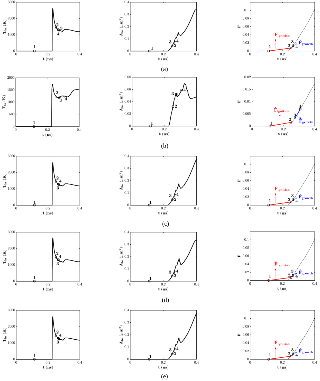
Figure 10: Evolution of the hot-spot temperature ( T_{hs} ) and area ( A_{hs} ), and the meso-scale product formation rate, F at different stages of the collapse of a void of diameter D_{void} = 0.5 \mu m for P_s = 22 GPa . The plots are for [C_p, K_T, \sigma_Y, \alpha] = [1800 J/KgK, 10.8545 GPa, 0.249 GPa, 20.05 \times 10^{-5} / K] , [2300 J/KgK, 10.8545 GPa, 0.249 GPa, 20.05 \times 10^{-5} / K] , [1800 J/KgK, 16.4 GPa, 0.249 GPa, 20.05 \times 10^{-5} / K] , [1800 J/KgK, 10.8545 GPa, 0.37 GPa, 20.05 \times 10^{-5} / K] & [1800 J/KgK, 10.8545 GPa, 0.249 GPa, 27 \times 10^{-5} / K] in (a) through (e). Instances 1 and 2 denote the start and end of the ignition phase, while instances (3) and (4) denote the start and end of the growth phase in cases (a) through (e).
