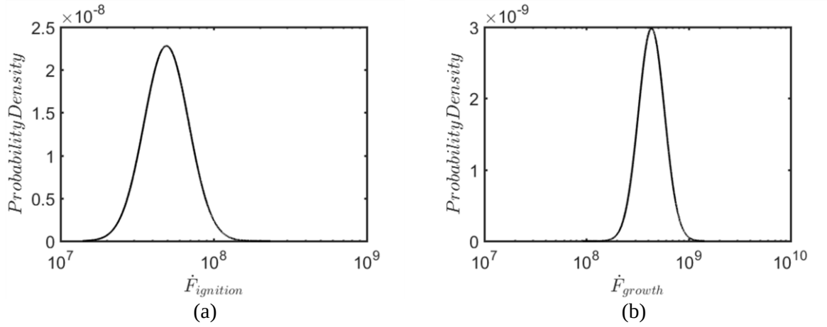
Figure 7. Probability density functions for (a) \dot{F}_{ignition} and (b) \dot{F}_{growth} computed at P_s = 22 \text{ GPa} for the collapse of a single isolated cylindrical void of diameter D_{void} = 0.5 \mu m . The pdfs are constructed by sampling the surrogate for \dot{F}_{ignition} and \dot{F}_{growth} at 1 million sampling points. The pdfs follow a log-normal distribution with mean and variances \mu_{\dot{F}_{ignition}}, \sigma_{\dot{F}_{ignition}}^2 for \dot{F}_{ignition} and \mu_{\dot{F}_{growth}}, \sigma_{\dot{F}_{growth}}^2 for \dot{F}_{growth} .
