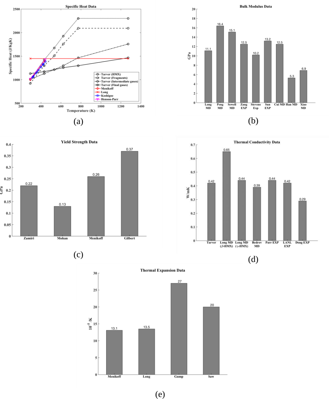
Figure 2 (a) Distribution of C_p for HMX based on the references [9, 12, 16, 19, 22]. (b) K_T distribution for HMX based on the references [1-9]. MD denotes data estimated by Molecular Dynamics computations while EXP denotes data estimated from experiments. (c) \sigma_Y distribution for HMX based on the references [10-13]. (d) k distribution of HMX based on the references [16-21]. MD denotes data estimated by Molecular Dynamics computations while EXP denotes data estimated from experiments. (e) \alpha distribution for HMX based on the references [9, 12, 14, 15].
