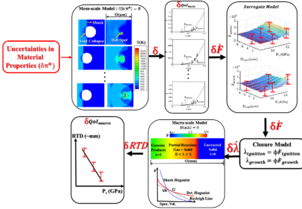
Figure 1. Schematic representation of uncertainty propagation across scales in the MES-IG model. The MES-IG model performs ensembles of high-fidelity meso-scale reactive void-collapse computations to compute two meso-scale product formations rates, \dot{F}_{ignition} and \dot{F}_{growth} . These are then used as inputs to a Kriging method to constructs surrogates of the form \dot{F}_{ignition}(P_s, D_{void}) and \dot{F}_{growth}(P_s, D_{void}) . The surrogates are used to compute the macro-scale reaction progress variables, \dot{\lambda}_{ignition} and \dot{\lambda}_{growth} , which are used close a homogenized macro-scale computational model. Macro-scale computations are used to simulate SDT and compute the run-to-detonation distances (RTD) for different shock pressures. The uncertainties (symbolically denoted by \delta ) in material properties are propagated through the meso-scale computations, resulting in stochastic surrogate models, \delta\dot{F}_{ignition}(P_s, D_{void}) and \delta\dot{F}_{growth}(P_s, D_{void}) . These result in stochastic closure models, \delta\dot{\lambda}_{ignition} and \delta\dot{\lambda}_{growth} for the reaction progress variables, which are fed as inputs to the macro-scale computations. Subsequently, this results in uncertainties in the run-to-detonation distances for the energetic material and are shown as error-bars in the pop-plots.
