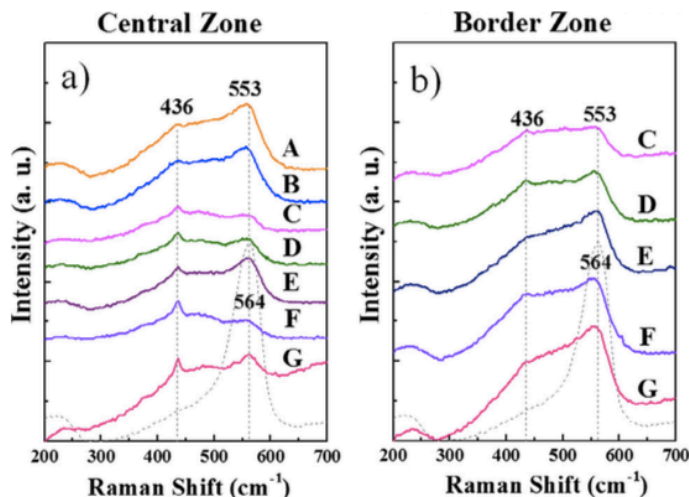
Figure 4. Raman spectra of (a) central zone and (b) border zone of A to G tracks. [3]
