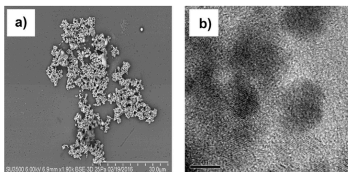
Figure 6. Morphology of synthesized ZnO NPs. (a) SEM image of the ZnO NPs deposited on a glass slide. (b) HRTEM image of ZnO NPs clusters conformed of spheroidal nanoparticles of around 5–8 nm size. [4]
