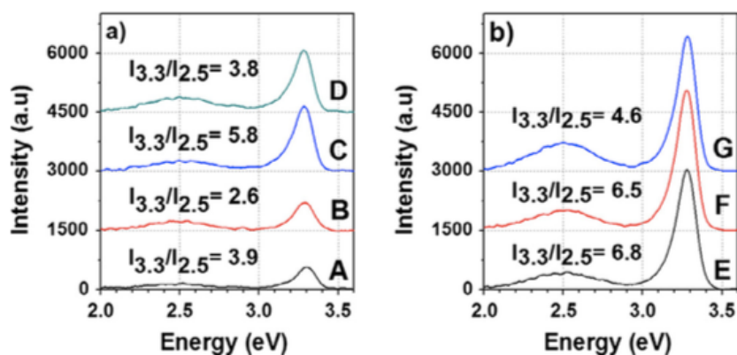
Figure 5. CL spectra of A to G tracks and their respective relative intensity ratio ( I_{3.3}/I_{2.5} ). [3]
