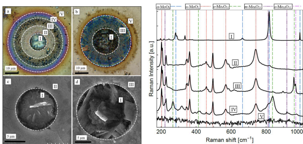
Figure 2. Left: Micrographs of irradiated molybdenum thin films ( 0.58 \text{mJ}/\text{cm}^2 , 10 s) in atmospheric air (a) and 16 psig \text{O}_2 (b). c-d: SEM images from samples depicted in a-b, respectively. Different modified regions can be observed (labeled as I, II, III IV and V). The images suggest a crater-like morphology and crystallites in the inner region. Right: Representative Raman spectra for the different regions shown in Fig. 2. Some of the characteristic peaks of molybdenum oxides have been highlighted. [2]
