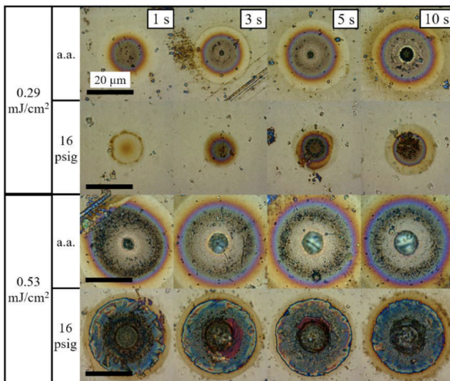
Figure 1. Optical micrographs of molybdenum thin films irradiated for 1, 3, 5 and 10 seconds. Two sets of fluences ( 0.29 and 0.53 \text{mJ}/\text{cm}^2 ) and two atmosphere conditions, ambient air (a.a.) and pressurized oxygen at 16 psig are depicted. The scale bar corresponds to 20\text{ }\mu\text{m} . [2]
