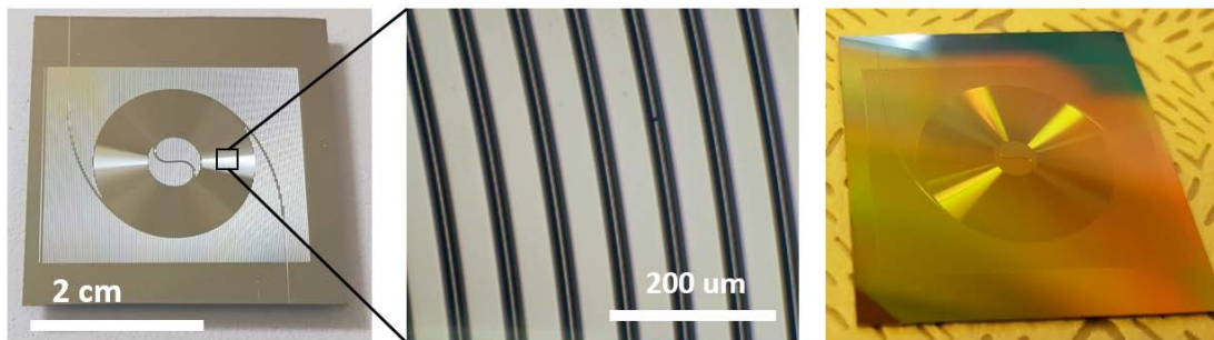
Figure 11. Low loss waveguide of hybrid material structure. (Left) Continuous waveguide having SiO 2 wedge cross-section was fabricated on a silicon chip as a bottom platform structure. (Middle) Microscope image of the waveguide (Right) Chalcogenide glass film was deposited on the top of the platform structure.
