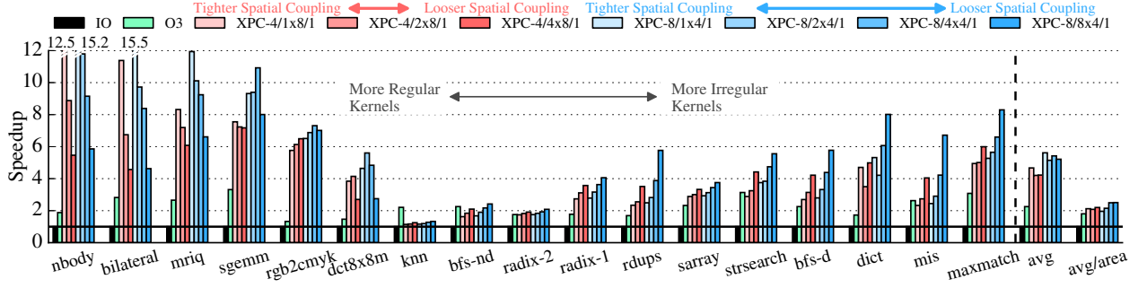
Figure 10: Performance of Single-Core XPC Engine with Variable Spatial Task-Coupling – All XPC engines have 32 \mu threads and all results are normalized against the performance of the baseline scalar in-order core for each kernel.
