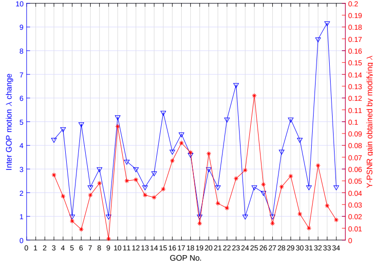
Fig. 36. Change of \lambda and Y-PSNR gain obtained by adaptation algorithm in processing Foreman
