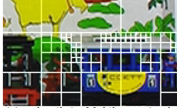
Fig. 9. quadtree based block division details in Mobile , moving boundaries tend to be compensated by smaller blocks
