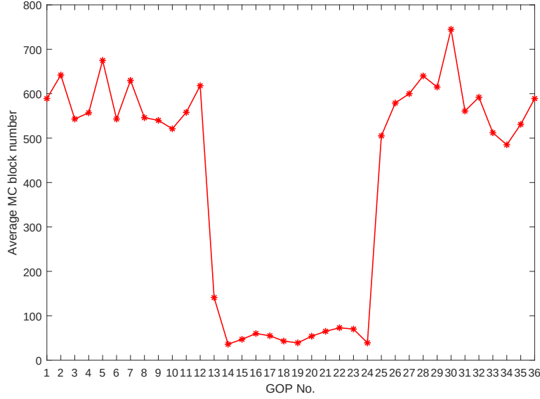
Fig. 40. Average motion-compensation block number in each GOP of the concatenated test clip.
