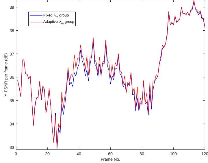
Fig. 37. Y-PSNR results of frame 1 – 120 of Tennis , obtained by coders with/without motion \lambda adaptation mechanism
