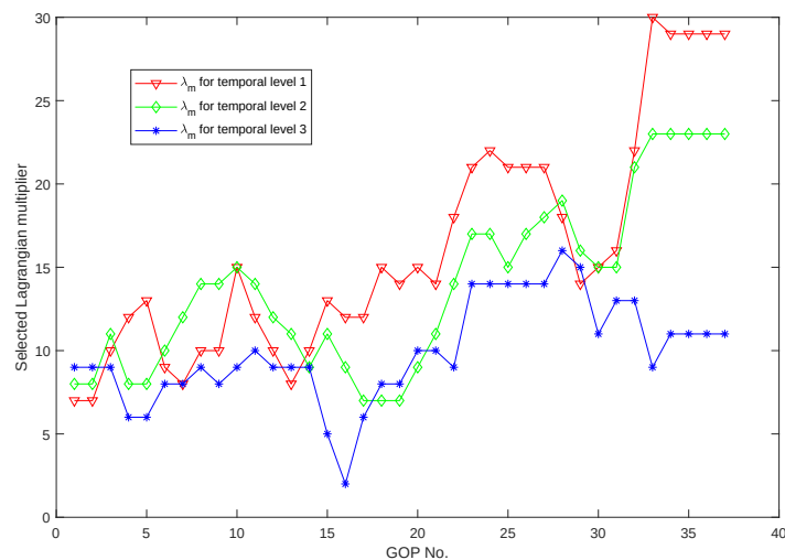
Fig. 34. Best motion Lagrange multipliers for different GOPs/temporal levels
