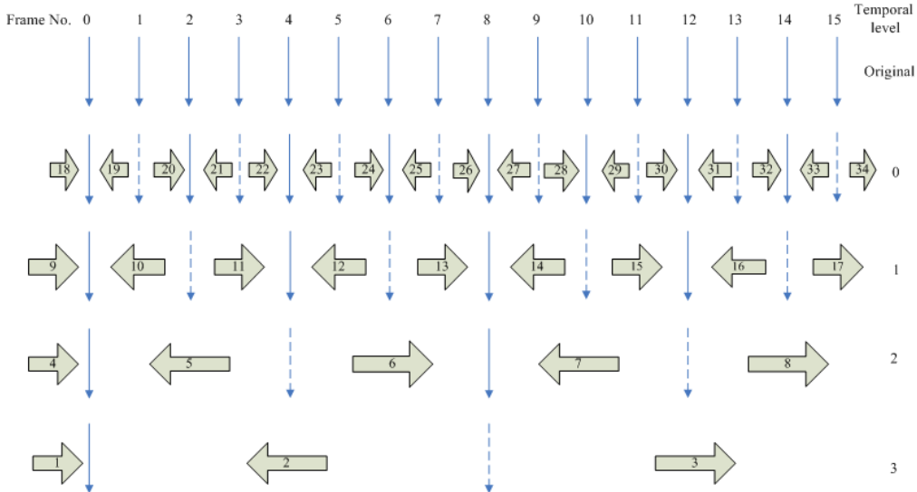
Fig. 1. Temporal decomposition structure of enhanced MC-EZBC with a GOP size of 16
