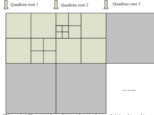
Fig. 2. Example of quadtree based block splitting
