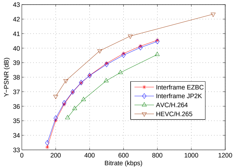
Fig. 19. Y-PSNR results of Flower Vase , obtained by different coders
