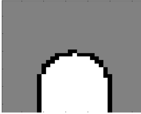
Fig. 25. Canny edge detection result of the 32 \times 32 block in Tennis , foreground (white), background (gray) and edge pixels are respectively marked
