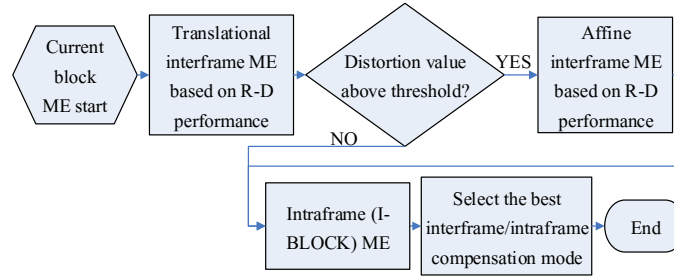
Fig. 14. Diagram of motion estimation (ME) algorithm for the new coder
