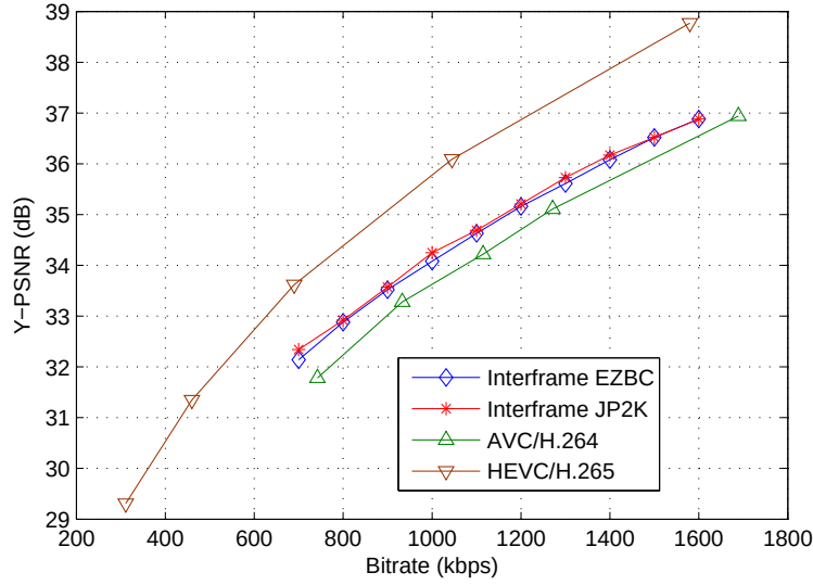
Fig. 18. Y-PSNR results of Flower , obtained by different coders
