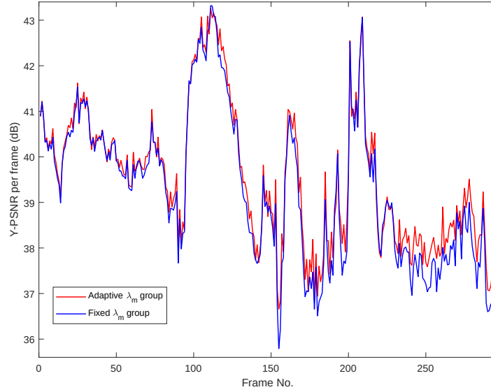
Fig. 33. Y-PSNR results of frame 1 – 296 of Foreman , obtained by coders with/without motion \lambda adaptation mechanism
