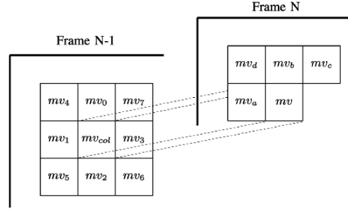
Fig. 3. Example of MV Predictor Candidates in [11]
