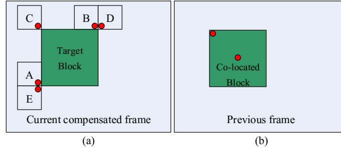
Fig. 10. Translational MV prediction candidates from (a) spatial (b) temporal neighbor positions
