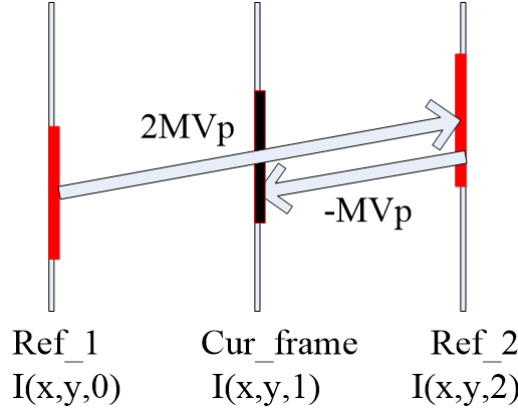
Fig. 21. Three-frame model for obtaining two-component MVs
