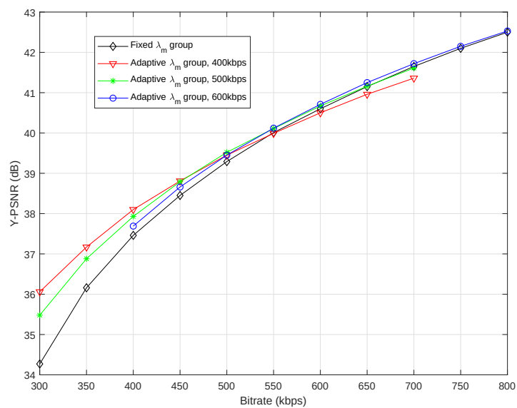
Fig. 35. Overall Y-PSNR curves of Foreman , obtained by different codecs.
