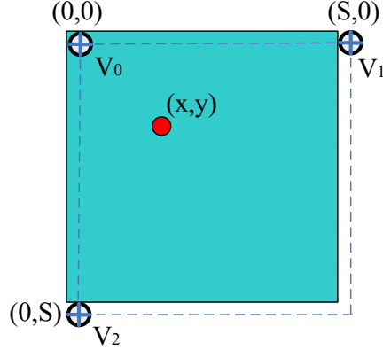
Fig. 7. Affine motion block with three control points
