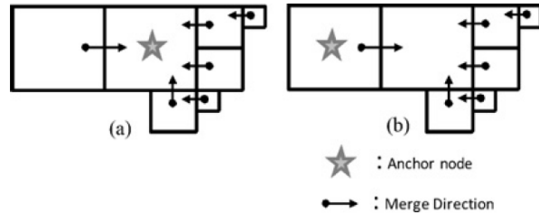
Fig. 4. Example of Leaf-Merging in [25]
