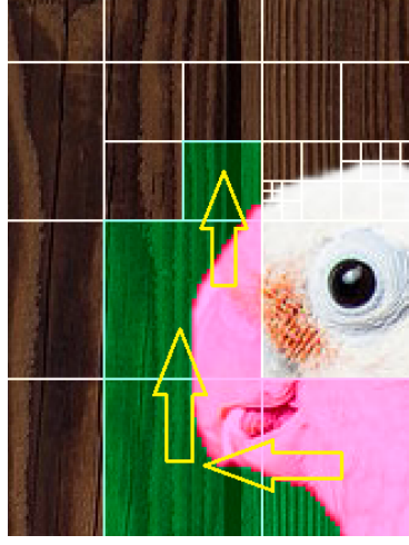
Fig. 39. Mutual merging of two-component motion blocks
