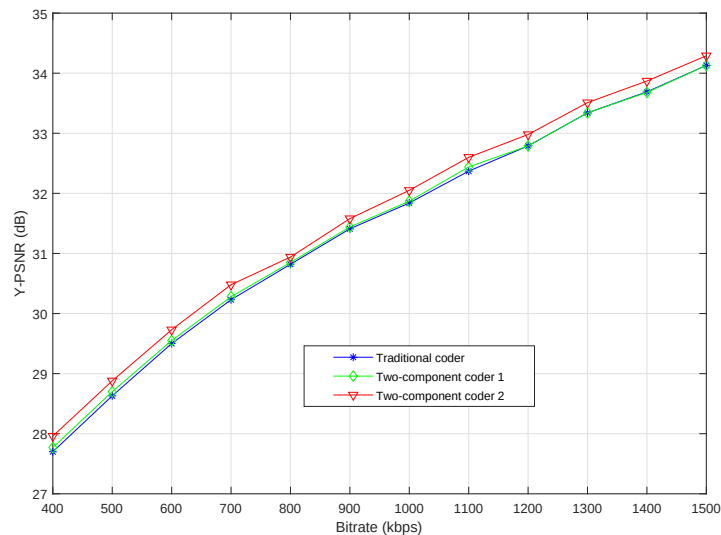
Fig. 30. Y-PSNR curves for 400-1500 kbps bitrate range
