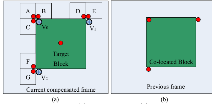
Fig. 12. Affine predictor system from (a) current frame. (b) previous motion-compensated frame
