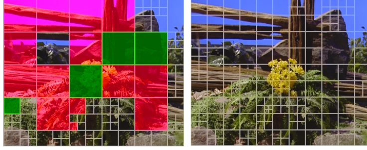
Fig. 16. Change of block division by introducing affine modes (left) compared with translational-only case (right), where affine merge blocks (green) and other affine blocks (red) were highlighted
