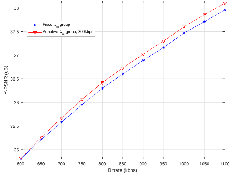
Fig. 38. Overall Y-PSNR curves of Tennis , obtained by codecs with/without \lambda adaptation
