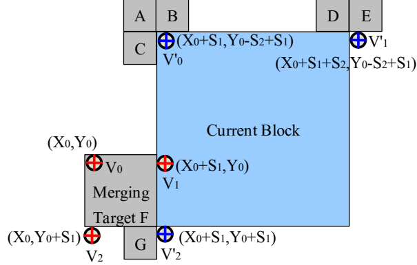
Fig. 13. Motion-estimation process for the new coder
