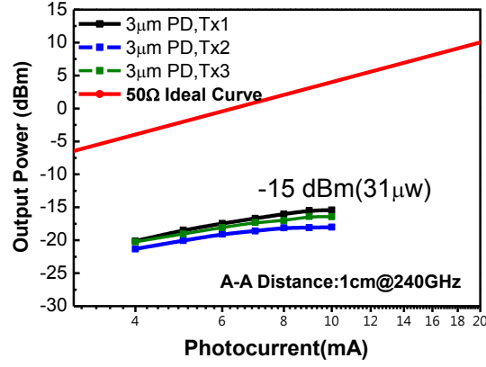
Figure 8. The detected power at the receiving-end at 0.24 THz versus output photocurrent from our photonic transmitters. Tx 1 to Tx 3 represent the three different photonic transmitters with the same packaging, same active PD inside, and under the same test setup.
