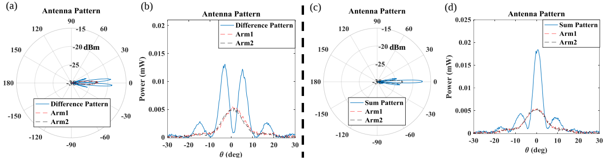
Fig. 11. Far-field antenna pattern measurement. (a,b) Far-field (3 m) broadband antenna array pattern with Tx1 and Tx2 out of phase. Polar plot with log scale in (a) and Cartesian plot with linear scale in (b). (c,d) Far-field (3 m) broadband antenna array pattern with Tx1 and Tx2 in phase. Polar plot with log scale in (c) and Cartesian plot with linear scale in (d). The measured powers at \theta = 0 are 0.65 \mu W and 22.1 \mu W for out-of-phase and in-phase transmission, respectively; the power at \theta = 0 with only a single transmitter enabled is 5.81 \mu W .
