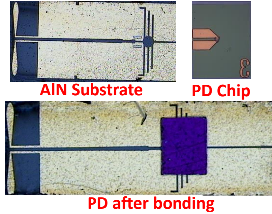
Figure 3. Top-view of the fabricated photonic transmitter chip: (a) before; and (b) after flip-chip bonding.
