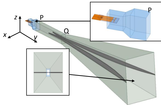
Figure 2. CAD layout of the entire waveguide-coupled photonic transmitter module, including a dual ridge horn antenna.
