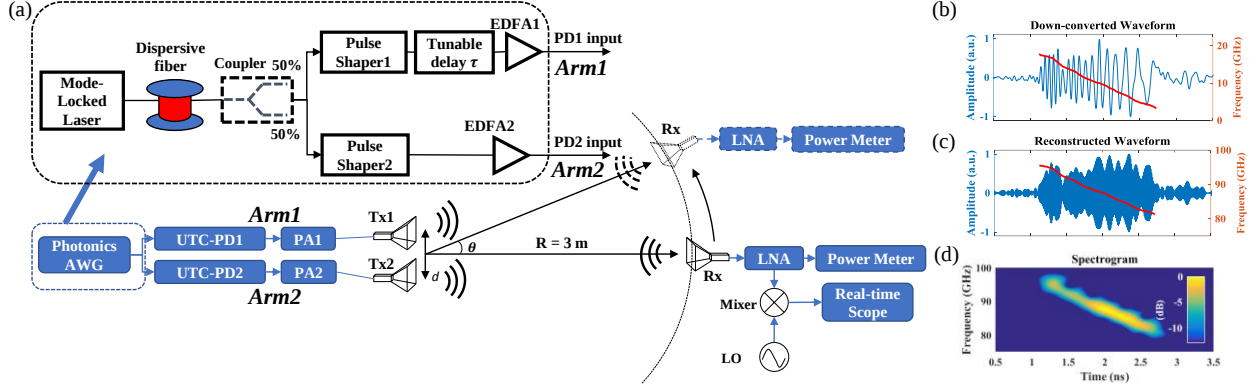
Fig. 9. Experimental arrangement and wireless W-band waveform transmission with ultrabroad bandwidth. (a) Setup schematic. EDFA, erbium doped fiber amplifier; PD, photodiode; AWG, arbitrary waveform generation; UTC-PD, uni-traveling carrier photodiode based waveguide-coupled photomixer; PA, power amplifier; Tx, transmitter; Rx, receiver; LNA, low noise amplifier; LO, local oscillator; d = 2 cm, R = 3 m. (b) W-band chirp signal from a single transmitter and its instantaneous center frequency, measured at the receiver end after down-conversion, showing 15 GHz bandwidth. Transmitted chirp, 80 – 95 GHz. LO frequency, 78 GHz. (c) Reconstructed received W-band chirp signal and its instantaneous center frequency. (d) Spectrogram of (c).
