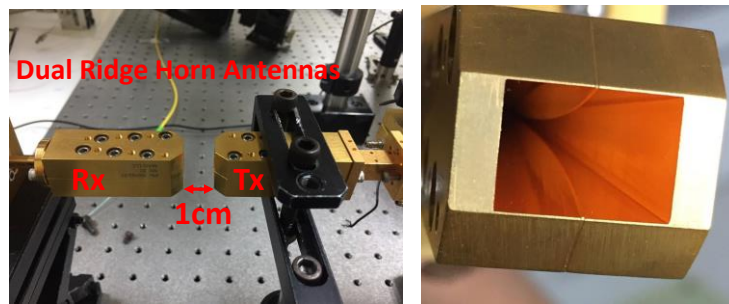
Figure 4. Photo of the wireless transmission setup and the fabricated dual ridge horn antenna.
