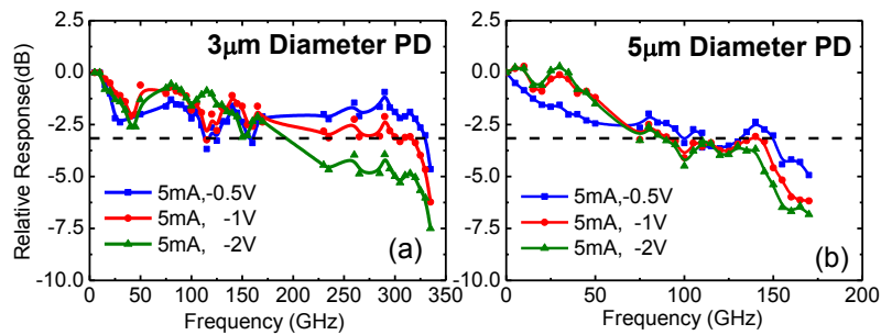
Figure 5. (a) The measured O-E frequency responses of our active PD with: (a) 3; and (b) 5 \mu\text{m} active diameters
