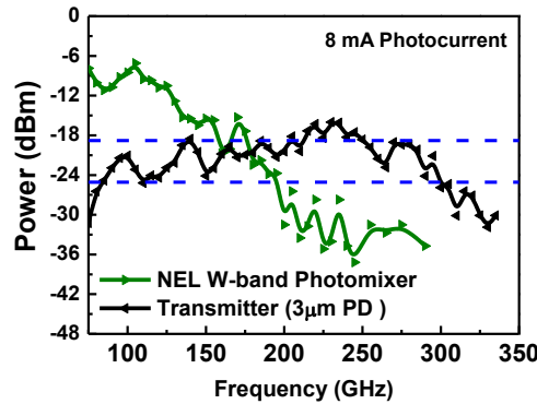
Figure 7. The measured O-E frequency responses for our wireless transmission channel (photonic transmitter with receiving antenna) design obtained using our home-made transmitter (black trace) and the commercial one (green trace).
