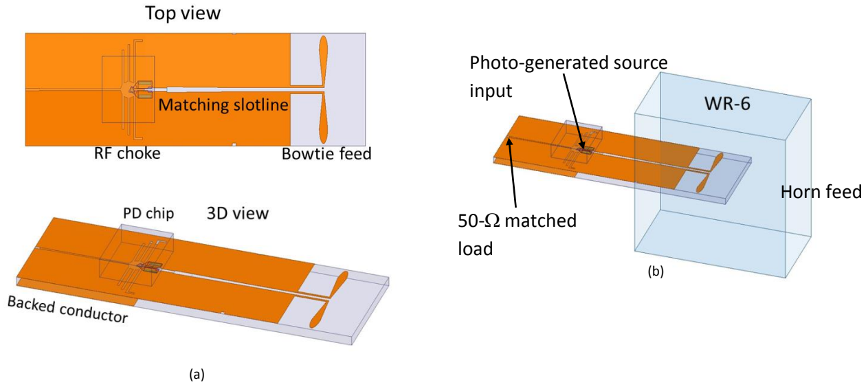
Figure 1. (a) CAD layout of the transmitter chip in our proposed waveguide-coupled photonic transmitter; (b) CAD layout of the feed configuration for the WR-6 waveguide.
