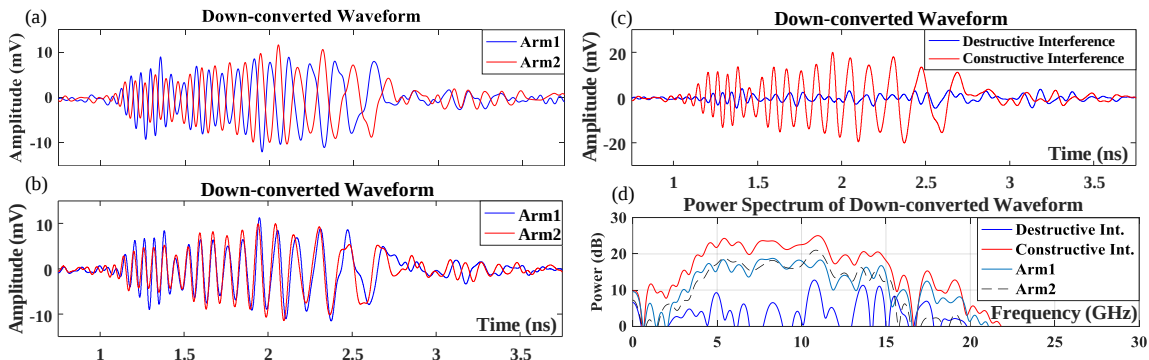
Fig. 10. Far-field antenna array measurement in the time domain. (a): Down-converted waveform at Rx when Tx1 on Tx2 off (blue), Tx1 off Tx2 on (red). Feeding waveforms for Tx1 and Tx2 are out of phase. (b): Similar to (a) but feeding waveform for Tx1 and Tx2 are in phase. (c): Down-converted sum (red) and difference (blue) interference waveforms at Rx when both Tx are switched on. (d) Spectrum analysis of received signal. Red
