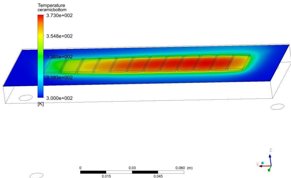
Figure 2. Temperature profile on the ceramic layer adjacent to the coolant. Inlet tube is on the left, outlet on the right
