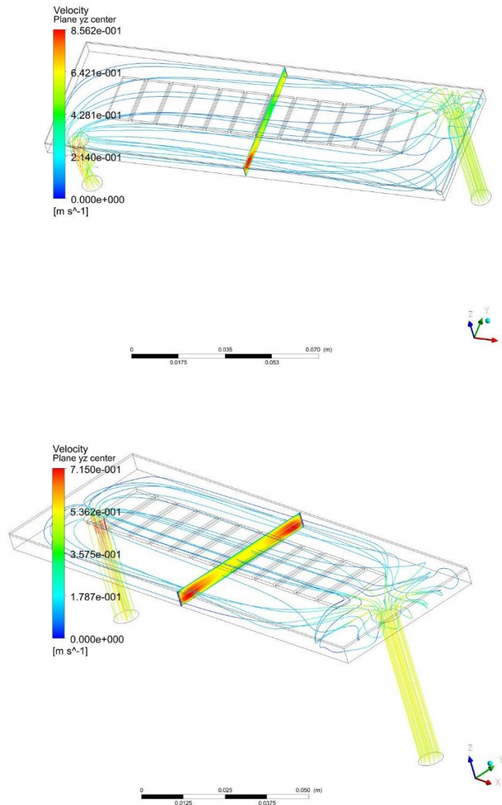
Figure 3 a&b. Streamlines of 5 mm thick channel with inlet and outlet in a) original locations and b) in line with the diodes. YZ plane in the center is colored by velocity, again showing high velocity is not under the diodes.
