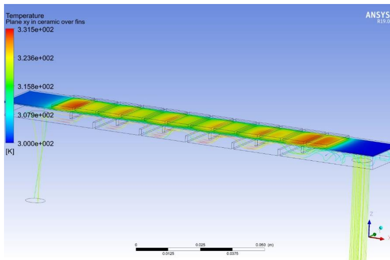
Figure 5. Temperature profile with width reduced and upper and lower fins.
