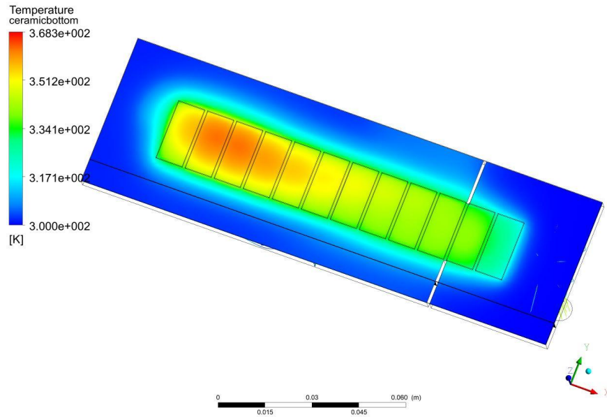
Figure 4. Temperature profile with two baffles. Baffles can be seen between the 2 nd and 3 rd diode from the right.
