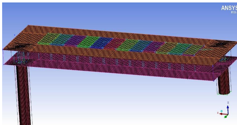
Figure 1. Computational mesh. 12 diode mounting blocks are visible on the top. The longer tube to the left is the water inlet and the water outlet is on the right.
