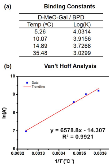
Figure 5. (a) Binding constants between BPD and MeO-α-Gal at various temperatures determined by 1 H NMR titrations in D 2 O. (b) van't Hoff plot for the binding between BPD and MeO-α-Gal.
