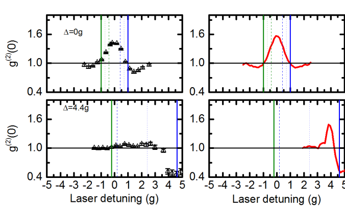
Figure JV8: g^{(2)}(0) as function of the laser detuning for two different QD-cavity detunings: (left) experiment and (right) simulation. With detuning the depth of the anti-bunching is more pronounced. The positions of the first upper and lower polariton branch are indicated by blue and green lines, respectively. The energies for subsequent climbs from first to second rung are indicated by dashed lines and the energies of a two-photon excitation of the second rung by dashed lines
