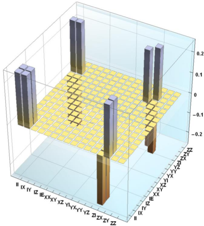
Figure showing the simulated process matrix for a CNOT gate between two ensemble qubits. From [8].
