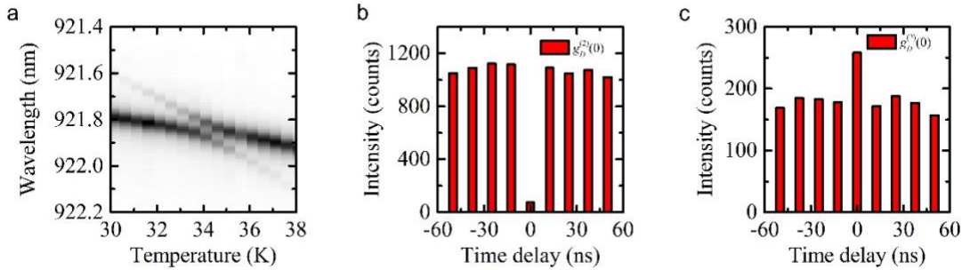
Figure JV10: a Anticrossing of a strongly coupled system in a cross-polarized reflectivity measurement. Hanbury Brown-Twiss measurement yielding a second-order coherence value of b g^{(2)}(0) = 0.063 \pm 0.010 in the photon-blockade regime and c g^{(2)}(0) = 1.490 \pm 0.034 in the photon-induced tunneling regime.
