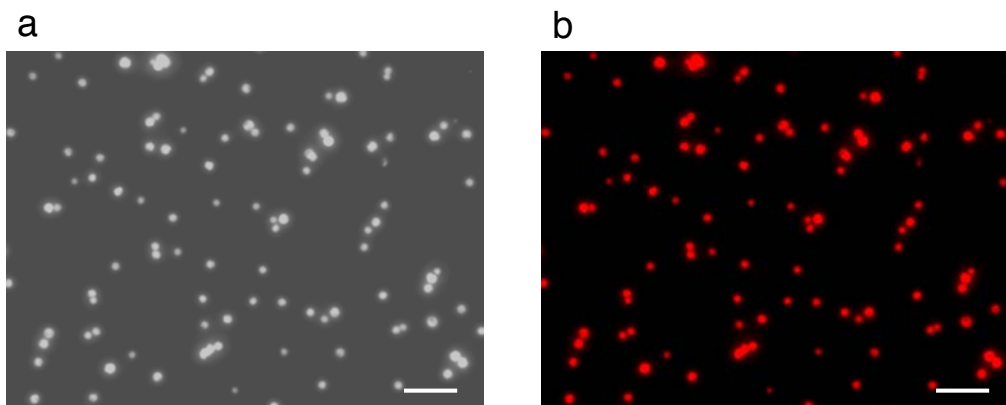
Figure SI 3. Microscopy image of MPs incubated in PBS 1x, pH= 7.4 (a) the dark field image and (b) the rhodamine fluorescence channel image evaluate that the size of MPs ca. is 2.12 \pm 0.41 \mu m . The data are collected from 3 different Images. The red color is corresponding to conjugated rhodamine dye on the Ac-Dex polymer. The scale bare in the images is 10 \mu m .
