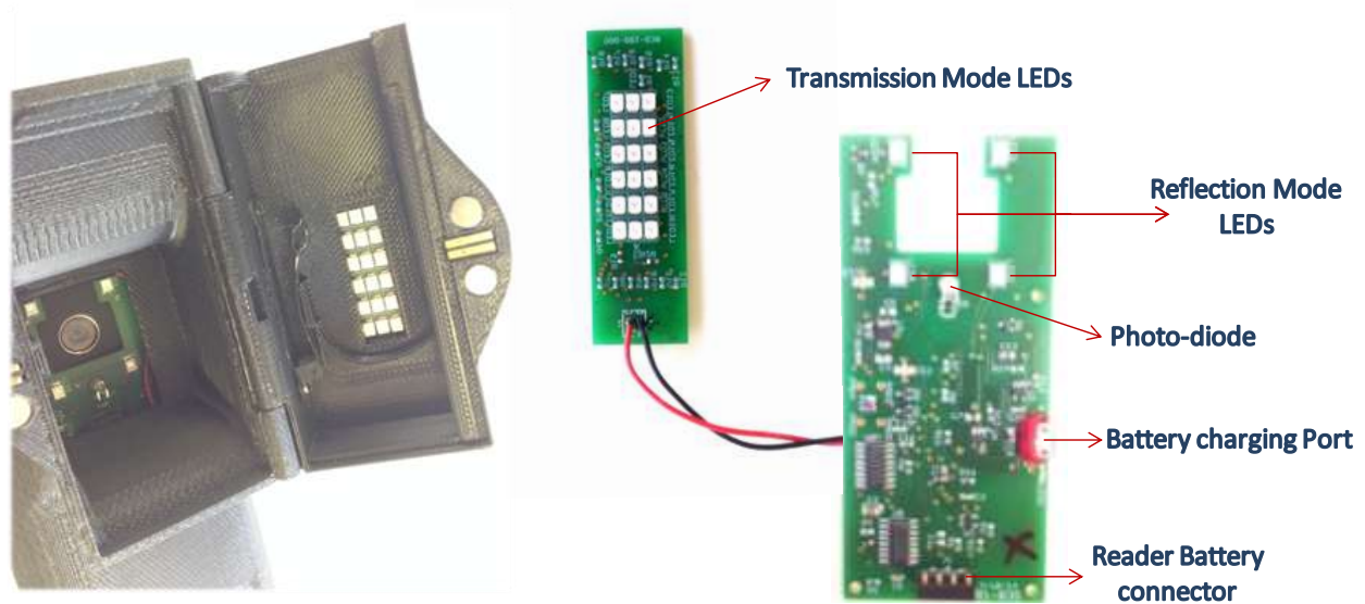
Figure 3 All readers are now capable of operating in both reflection and transmission modes and users can configure their own readers to selectively work on a specific mode based on the assay specifications and design.
