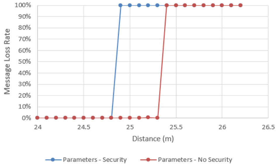
Figure 20. Message loss rate with security turned on and off using the Parameters profile
