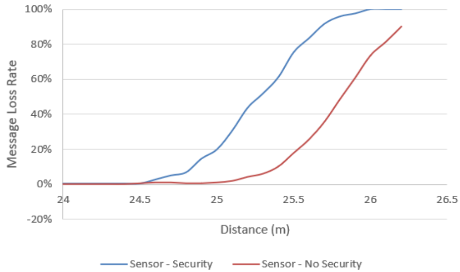
Figure 18. Message loss rate with security turned on and off using the Sensor profile
