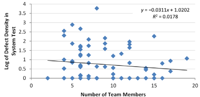
Defect Density vs Team size
