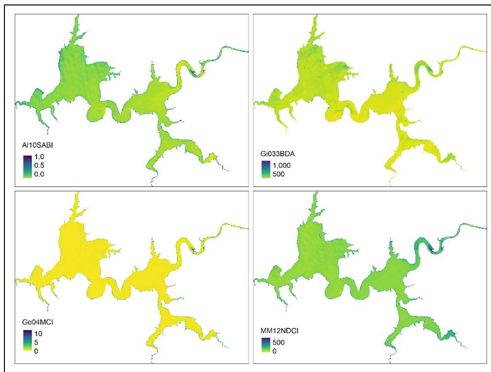
Figure 3. Four Sentinel-2 algorithms produced by the wq_calc function in the waterquality package. Note that measurements of each algorithm are relative index values and do not represent absolute water quality parameter values.
