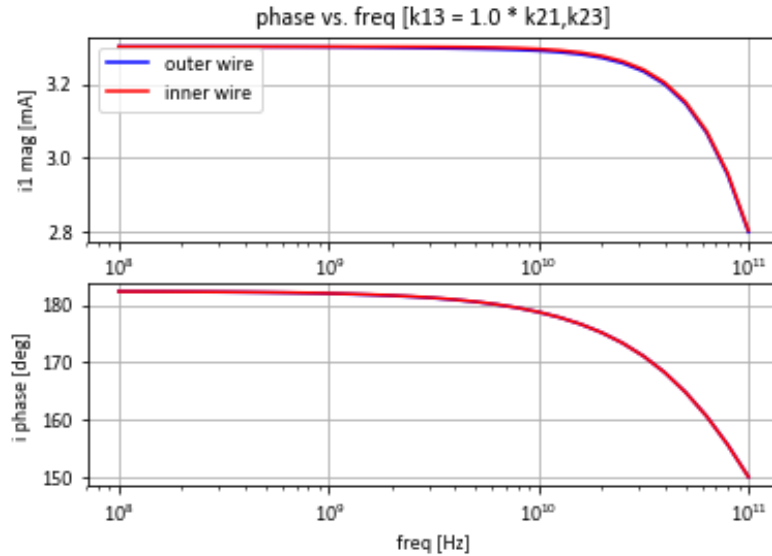
Figure 44. All wire-wire Coupling is Identical
