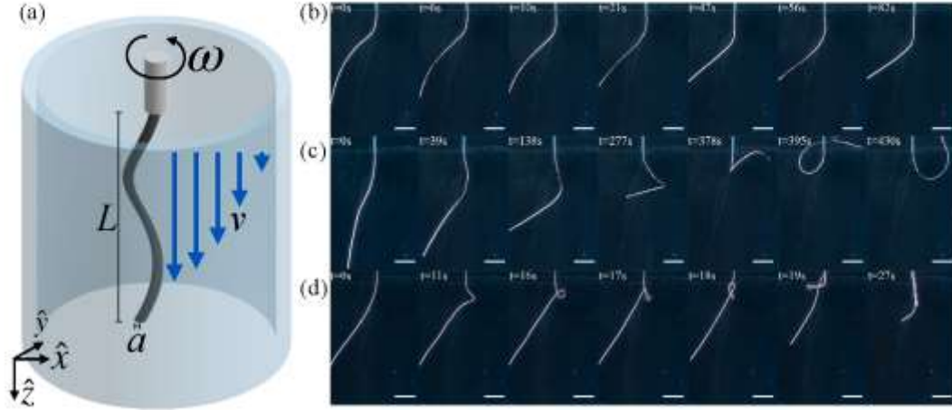
FIG. 1. (a) Diagram of the experimental setup. A flexible filament of length l and radius a is freely suspended in a viscous fluid and rotated at the top with an angular velocity \omega . A pump provides downward flow with a velocity v to tension the filament. (b)-(d) Time series of 380 \mu\text{m} diameter filaments with v = 0 , demonstrating: (b) stable twirling motion with L = 8 cm and \omega = 12 rad/s, (c) unstable whirling leading to overwhirling motion with L = 8 cm and \omega = 26 rad/s, and (d) plectoneme formation with L = 11 cm and \omega = 61 rad/s. Scale bars are all 2 cm.
