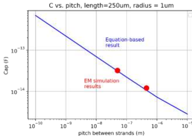
Figure 48. Capacitance between two parallel wires as a function of center-center distance between wires calculated two ways: (1) using the above equation and (2) using the finite element simulation software COMSOL
