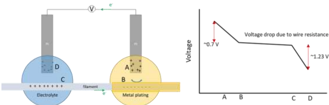
Figure 16. Basic set up of an indirect bipolar electrodeposition (BPE) of gold onto the PMIA filament. The platinum wires are connected to power and a current is driven through. Oxidation/reduction reactions drive ionic current in solution allowing for the PMIA metal-seeded fiber to also under-go redox reactions leading to gold metal plating ( V=0.7 V), while hydrolysis occurs in the salt solution ( V=1.23 V). Current flows through the filament closing the circuit.
