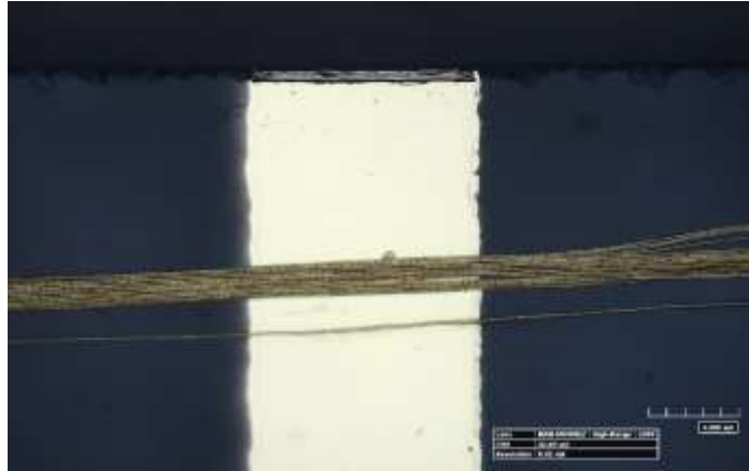
Figure 27: An untwisted bundle after transfer to a borofloat glass electrical measurement substrate. The bright yellow region is a Cr/Au bonding pad
