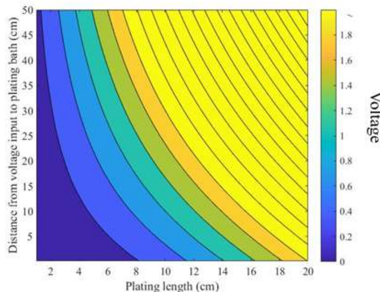
Figure 56. Voltage drop along filament for varying plating length and distance from voltage input, for 4ASF current density .
