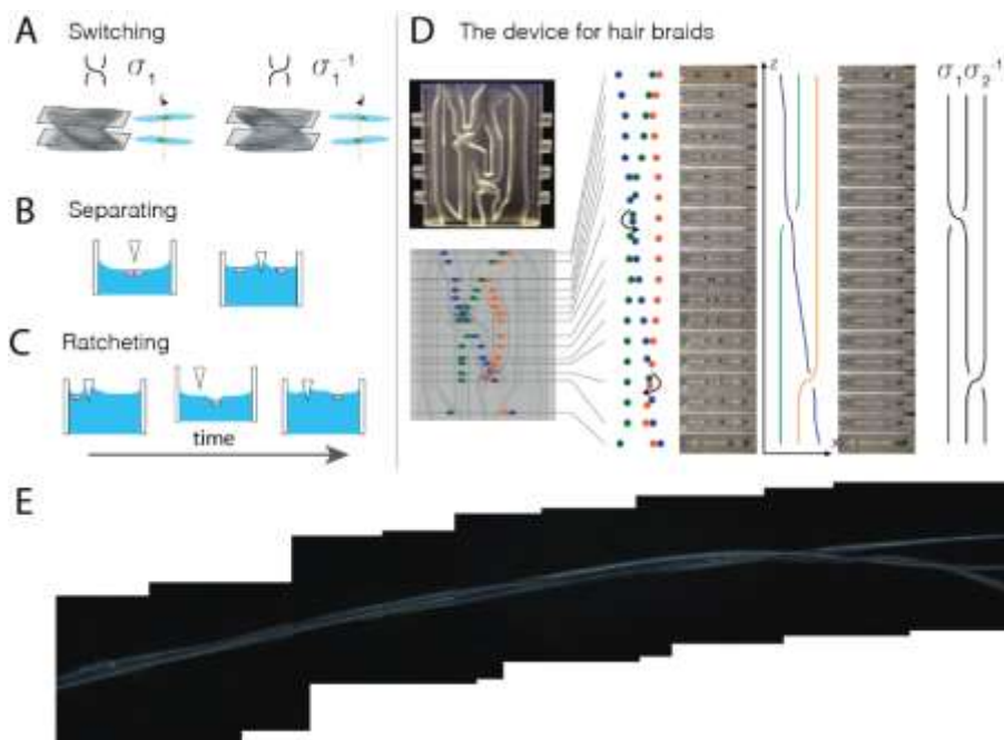
Figure 62. A 3-strand braid is achieved by integrating three operations into one device. (A) The switch, in which two floats change positions, leading to wires crossing each other. Each cross-section of a switching section is an oval whose long axis rotates 180^\circ along the z-axis.
