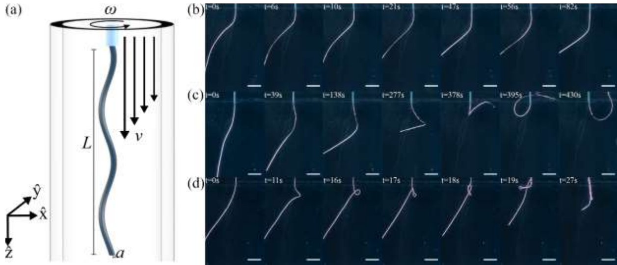
Figure 60: (a) Diagram of the experimental setup. A flexible filament of length l and radius a is freely suspended in a viscous fluid and rotated at the top with an angular velocity \omega . A pump provides downward flow with a velocity v to tension the filament. (b)-(d) Time series of 380 \mu\text{m} diameter filaments with v = 0 , demonstrating: (b) stable twirling motion with L = 8 cm and \omega = 12 rad/s, (c) unstable whirling leading to overwhirling motion with L = 8 cm and \omega = 26 rad/s, and (d) plectoneme formation with L = 11 cm and \omega = 61 rad/s. Scale bars are all 2 cm.
