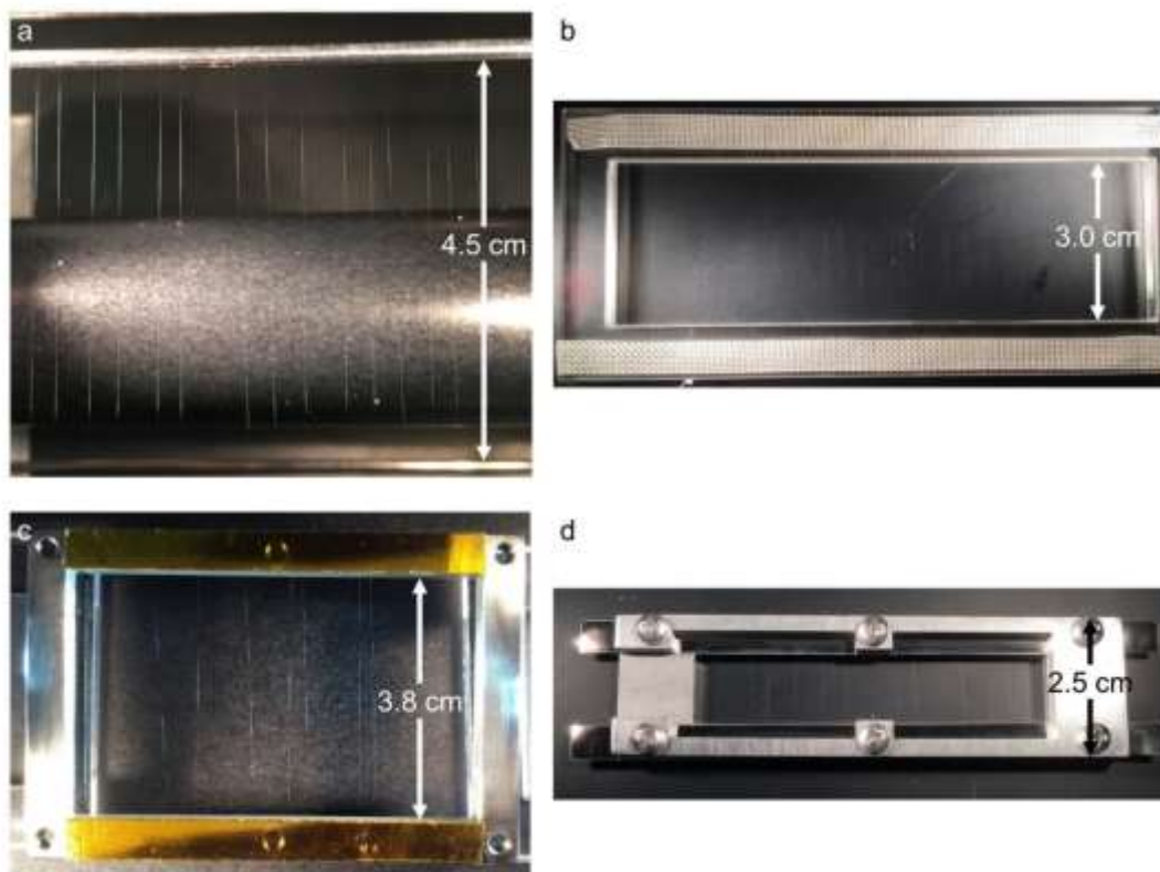
Figure 7. Photographs of electrospun nanofibers. (a) Photograph of aligned fibers on part of the rotating spoked-drum collector. (b) Photograph of aligned fibers on a transfer holder. (c) Photograph of our widest holder with some single fibers attached by double-sided tape that is suitable for PVD. (d) Photograph of Co coated fibers with CVD. Bright illumination from the side results in scattered light from the submicron fibers, making them visible to the naked eye.
