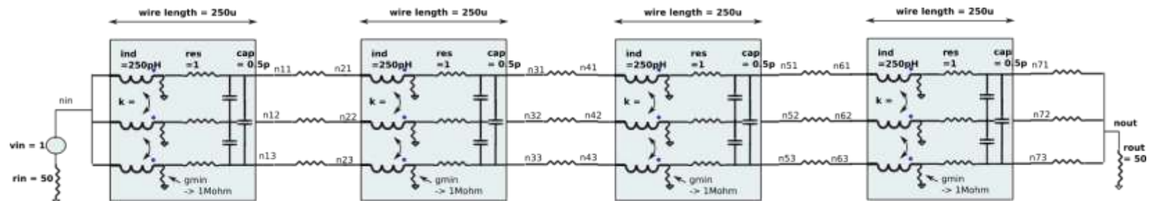
Figure 39. Example Series Connection of Circuit-Element Sections
