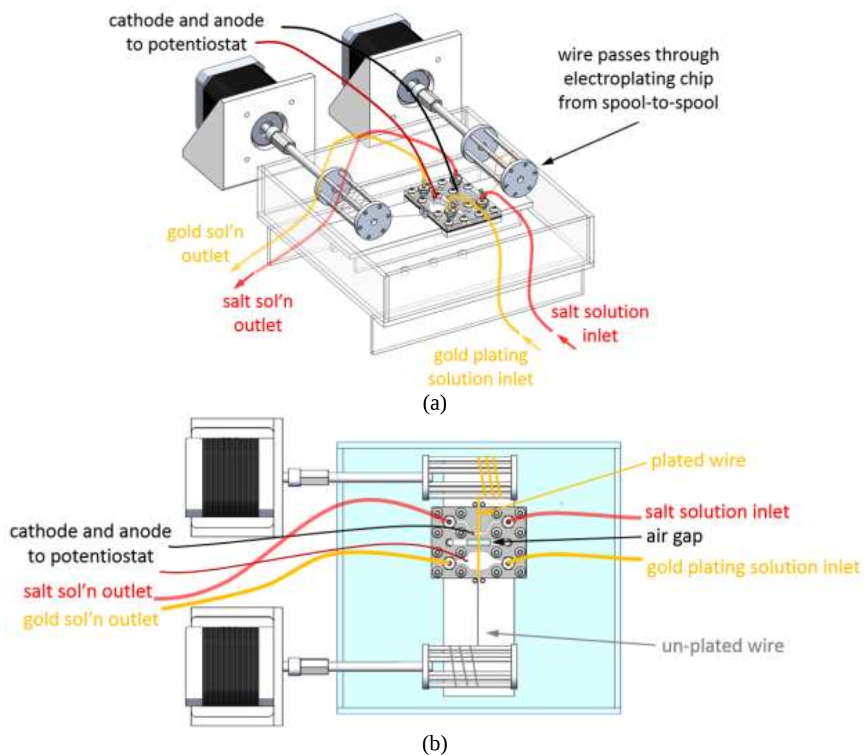
Figure 21. (a) Design of the reel-to-reel electroplating system. (b) Top view of the system.
