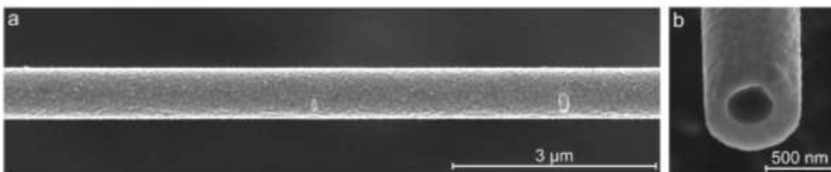
Figure 10. Conformal physical vapor deposition on nanofiber scaffolds. (a) Fiber sputter-coated with Ag from both sides and (b) its cross-section
