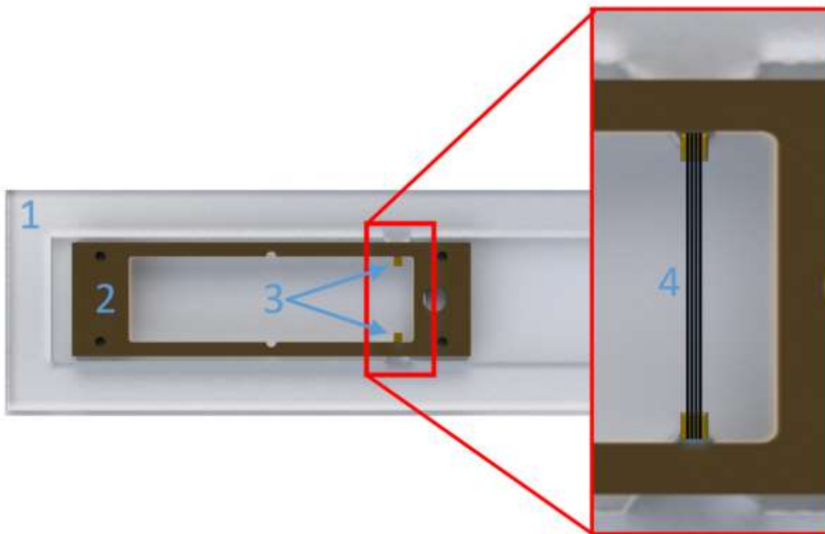
Figure 26: The setup for capturing untwisted nanofibers is shown. Number 1 represents the fixture, 2 the frame of wires, 3 the kapton tape, and 4 the nanofibers that have been captured previously.
