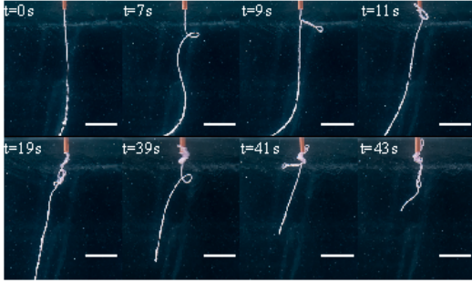
FIG. 3. Time series showing successive formation of three plectonemes in a filament with L = 10 cm, \alpha = 178 \mu m, and \omega = 57 rads/s.
