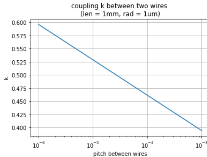
Figure 42. Mutual Inductance(k factor) vs. Separation (log meters)
