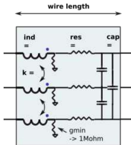
Figure 37. Three-strand circuit-element model of a short section of three straight, parallel wires. A model of a realistic bundle would be represented by multiple sections connected in series. Twisting or braiding can be represented by varying the circuit parameters appropriately in different sections.
