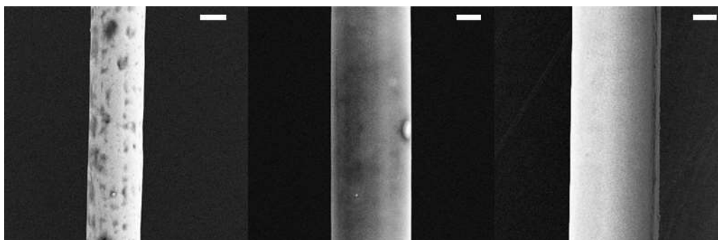
Figure 17. 1 mil copper wire plated in gold using CBPE set up. Over time the thickness plates from 2 microns to 14 and finally to 20 micron thick gold over 45 minutes, demonstrating a scalable process. Scale bar is 10 microns.
