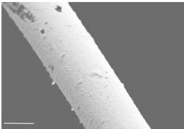
Figure 22. Gold plated copper wire section form 85 cm run. Scale bar is 10 microns.
