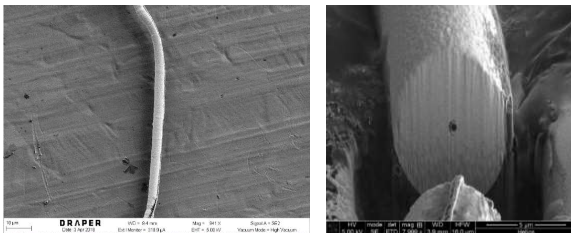
Figure 15. SEM images of PMIA nanofiber electroplated using a current density of 8 mA/cm 2 to achieve a ~5 µm-diameter wire
