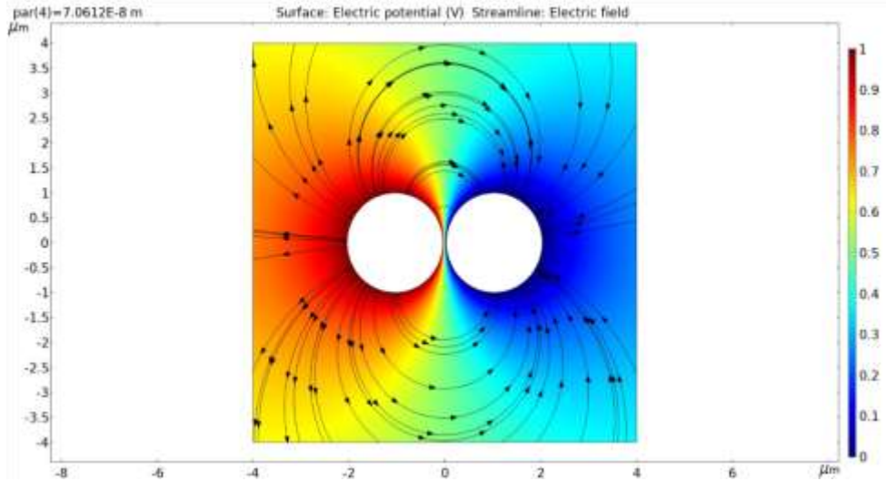
Figure 47. Electric fields and surface potential between wires in a finite element simulation of two parallel wires.
