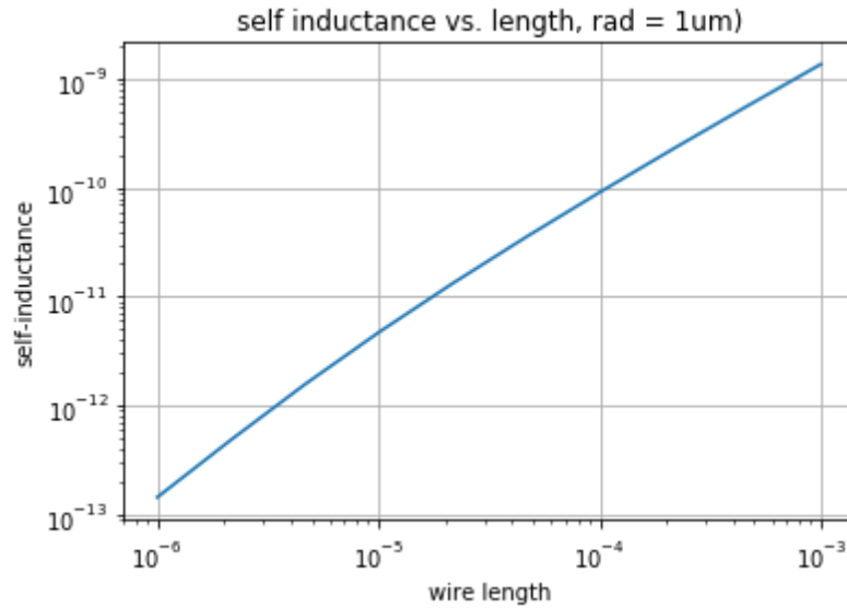
Figure 40. Analytic Self Inductance(nH) vs. Length(log meters)
