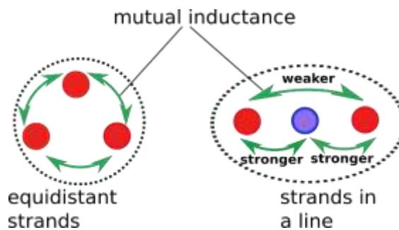
Figure 43. Outer to Outer Coupling 1/2 of Inner to Outer Coupling
