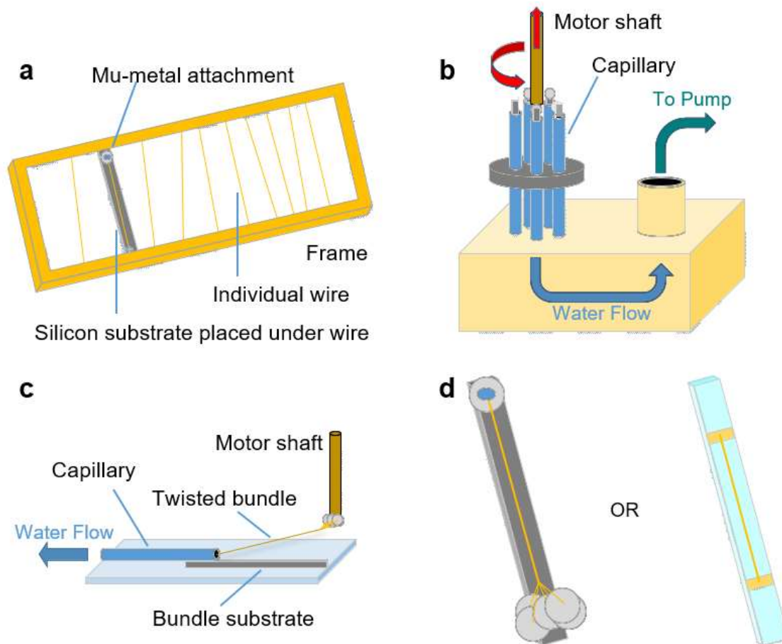
Figure 25. Twisting nano-litz bundles from individual nanowires. a, Placing an individual metal-coated PMIA nanofiber wire onto a silicon substrate, affixing with water-soluble adhesive, and attaching a disc of mu-metal to one end. b, Wires mounted on substrates are inserted into separate capillary tubes, and the entire apparatus is submerged in water. A pump draws water through the capillaries, releasing the water-soluble adhesive. The oversized mu-metal discs prevent the wires from being sucked into the apparatus, while flow tensions the wires within the capillaries. A motor shaft with magnetic tip placed in the center of the capillary array attracts the mu-metal discs, providing reversible attachment of wires to the motor shaft. To twist a bundle, the motor turns while the shaft is withdrawn from the fixture. c, After twisting, the free end of the twisted bundle is drawn into the capillary of a second fixture to provide tension while the bundle is placed on a new substrate. d, If the bundle will be twisted into a twist-of-twists, a new mu-metal disc can be attached to the bundle and the previous discs removed. If the bundle is to be electrically measured, it can be placed directly onto an electrical test substrate and bonded.
