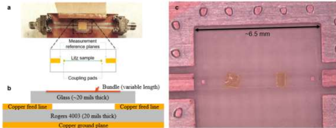
Figure 33. Resonant-cavity measurement fixture. a, Optical image of a measurement channel on the test fixture.
