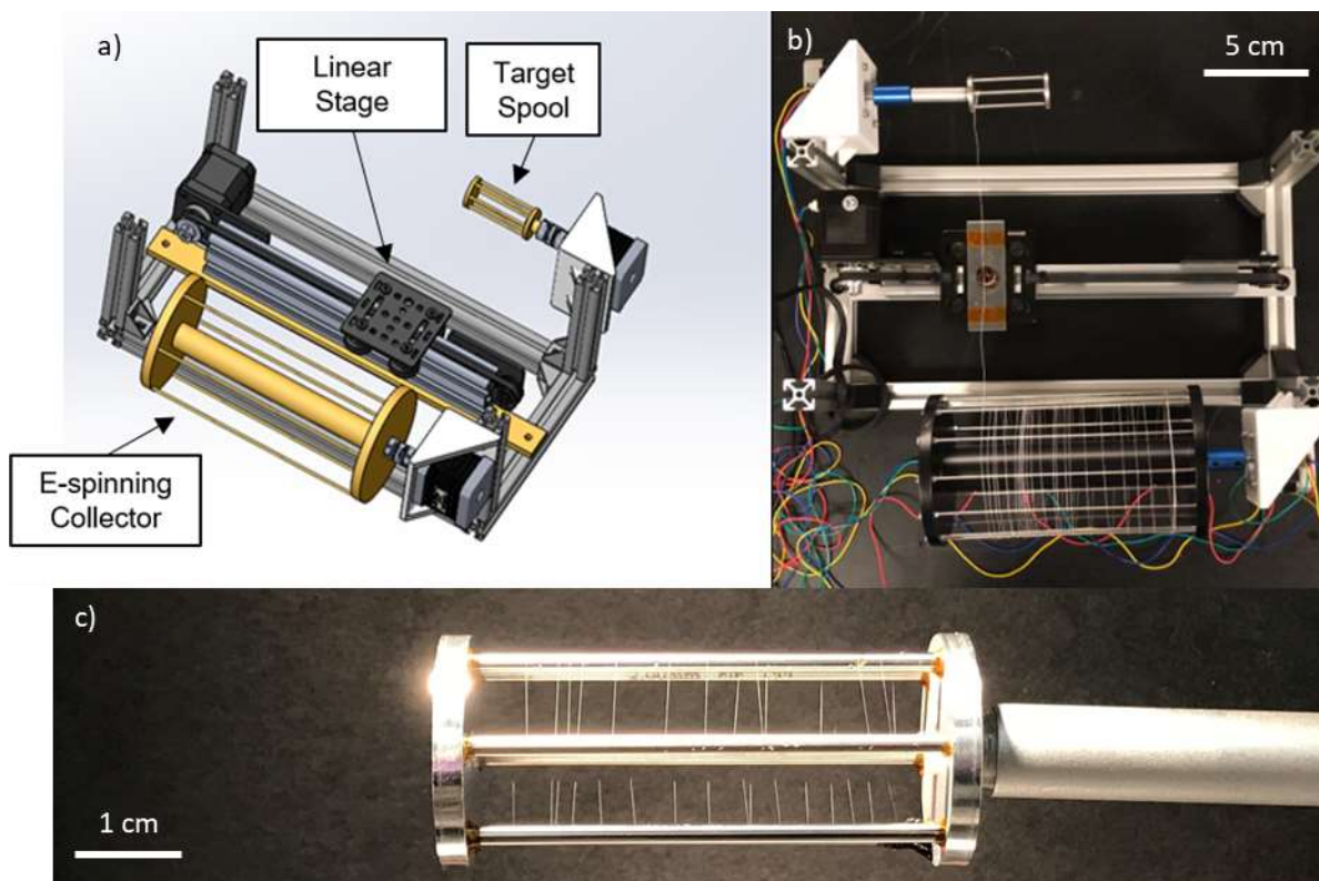
Figure 12. Motorized reel-to-reel nanofiber processing. a) CAD model of spool-to-spool transfer system and b) actual transfer apparatus. C) Successful transfer of 1.2 m of PMIA nanofiber onto a spool
