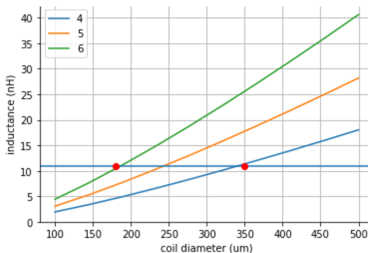
Figure 53. Inductance versus coil diameter for coils with 4, 5, and 6 turns
