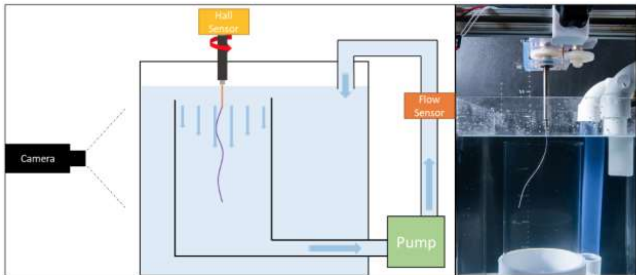
Figure 28. Experimental apparatus for twisting a filament immersed in a recirculating fluid bath. Left, Schematic diagram of apparatus. Right, Image of filament and tank
