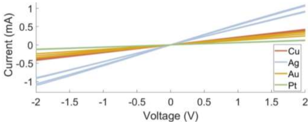
Figure 55. Current versus voltage measurements of PMIA nanofibers coated with various metals
