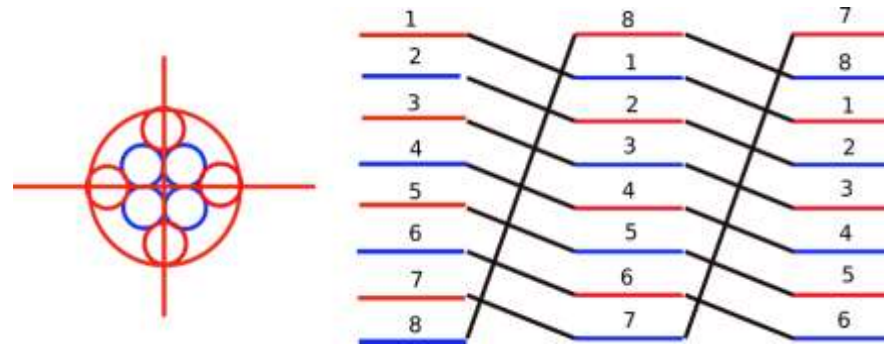
Figure 38. Series Cross-Connection of sections for modeling Litz Effect
