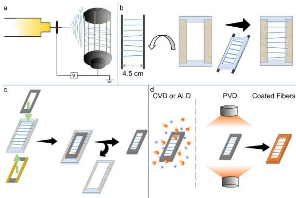
Figure 6. Electrospinning and fiber transfer. (a) Diagram of the electrospinning experiment. (b) Schematic of fiber transfer steps from the spoked drum onto a holder with double-sided tape. The final holder can be used directly for sputter coating or as an intermediate holder to transfer for CVD/ALD holders. (c) Transfer of fibers onto metal holder for deposition experiments. The top frame can be attached using screws, avoiding any tape that might interfere with CVD or ALD experiments. (d) Scheme of metal coating onto polymer nanofibers with different methods.
