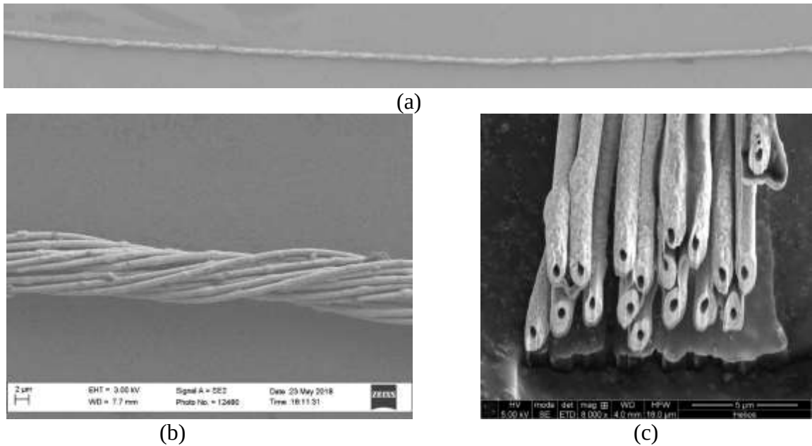
Figure 58. Bundle of 23 uninsulated nanowires. (a) Scanning electron microscope image, (b) detail, and (c) FIB cross-section.
