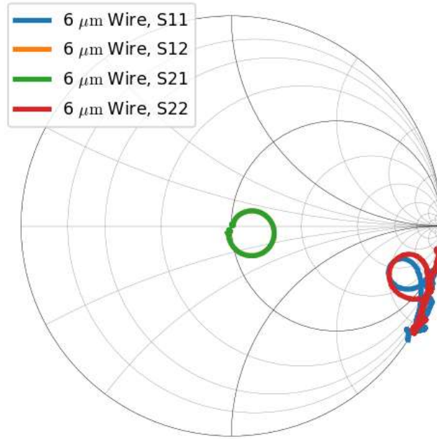
Figure 34. Example Smith plot of a ~6 \mu\text{m} diameter control wire measured in the resonant transmission fixture
