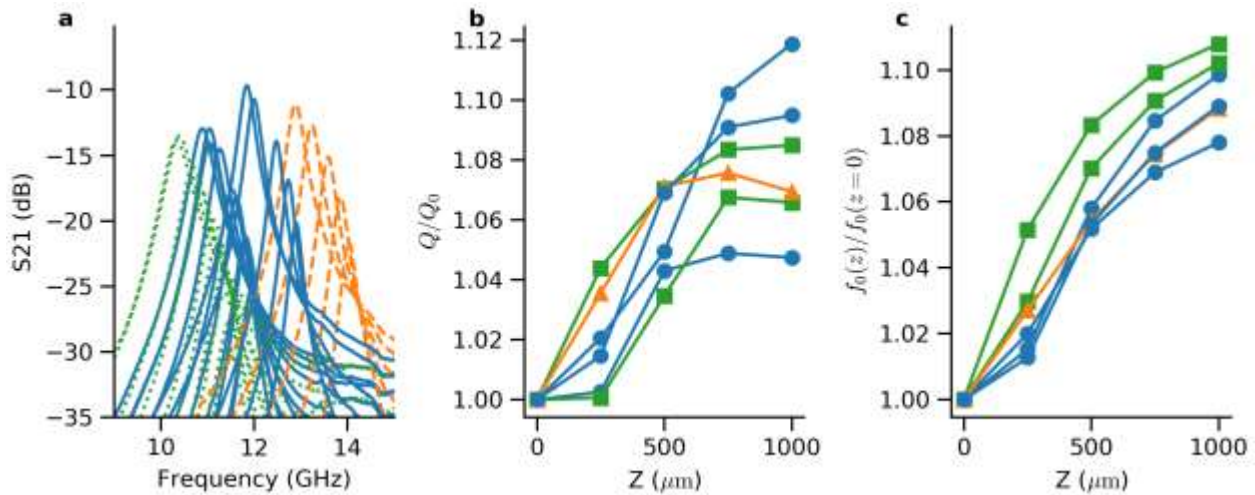
Figure 51. Dependence of sample Q on distance above test fixture, Z .
