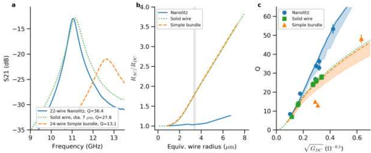
Figure 50. Experimental measurements of nano-litz performance benefit at GHz frequencies for sputtered gold wires. (a), Measured transmission scattering parameter S_{21} plotted for three representative samples. Unloaded Q extracted for each sample is indicated. (b), Calculated resistance ratio R_{AC}/R_{DC} versus wire radius at 11 GHz for each type of sample. For wire bundles, radius used is of an equivalent wire with equal metal cross-sectional area. The curves for solid wire and non-litz bundle are indistinguishable. (c), Unloaded Q vs G_{DC}^{1/2} . Points, extracted unloaded Q factors from experimental data. Lines, predicted values using the analysis in (b). For nano-litz and simple bundles, shaded regions indicate the range of Q expected from sub-optimal fill factor.
