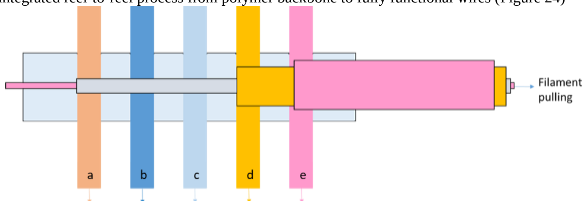
Figure 24. Schematic diagram illustrating a multi-stream approach to creating an insulated electroplated wire using an electroless strike on a polymer filament followed by electroplated metal and a final insulating polymer coating. The streams listed are (a) electroless metal, (b) saline, (c) rinse, (d) metal electroplating, and (e) polymer solutions.
