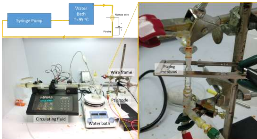
Figure 14. Electroplating bath set up. A syringe pump circulates electroplating solution as it passes through a water bath to raise the temperature and provide more conformal plating. The wires are plated where there is an exposed meniscus of electrolyte providing isolation and mechanical support for the wire as it is plated.
