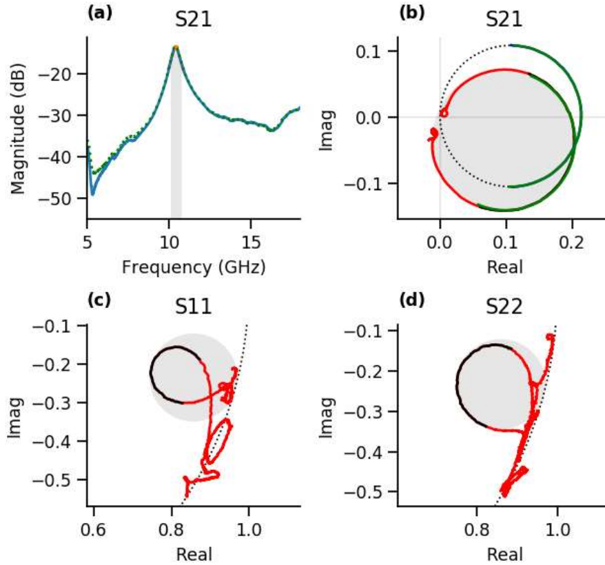
Figure 35. Example Q-factor extraction procedure from the same sample shown in Figure 34. (a), Transmission (S21) magnitude versus frequency. Gray band indicates region within 3 dB of peak that is used for fitting bilinear function for Q-factor extraction. (b-d), Real versus imaginary components of transmission (S21) and reflection from either port (S11 and S22).
