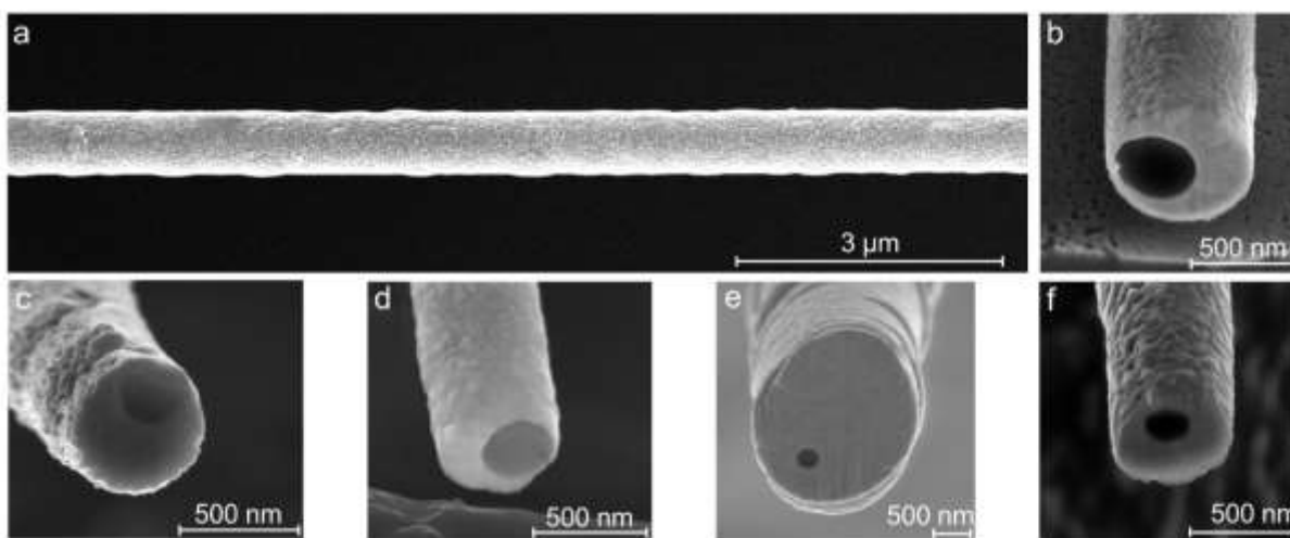
Figure 9. Non-conformal physical vapor deposition on nanofiber scaffolds. (a) Platinum sputter coated fiber and (b) its cross-section. (c) Cross-section of a fiber sputter coated with titanium from one side only. Cross-sections of (d) gold, (e) copper, and (f) cobalt coated fibers sputtered from both sides
