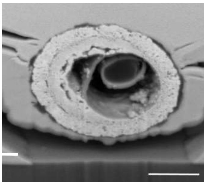
Figure 23. Gold-plated PMIA wire. Scale bar, 500 nm. The PMIA core used for this investigation had multiple concentric layers resulting from presence of \text{CaCl}_2 , as described in Section 3.1.3.
