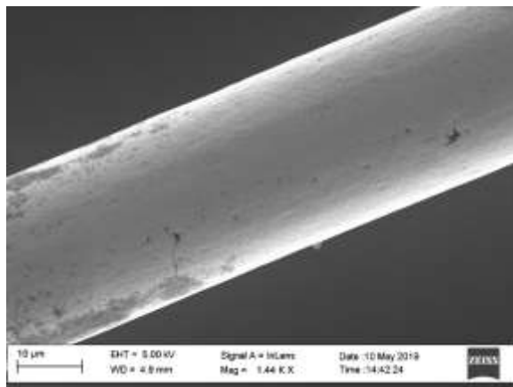
Figure 19. Segment of copper wire coated in gold using the reel-to-reel CBPE set up.
