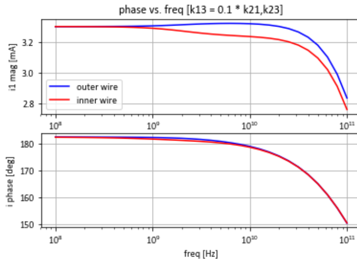
Figure 45. Wires in a plane: Outer-to-outer coupling is 1/2 of inner-to-outer coupling
