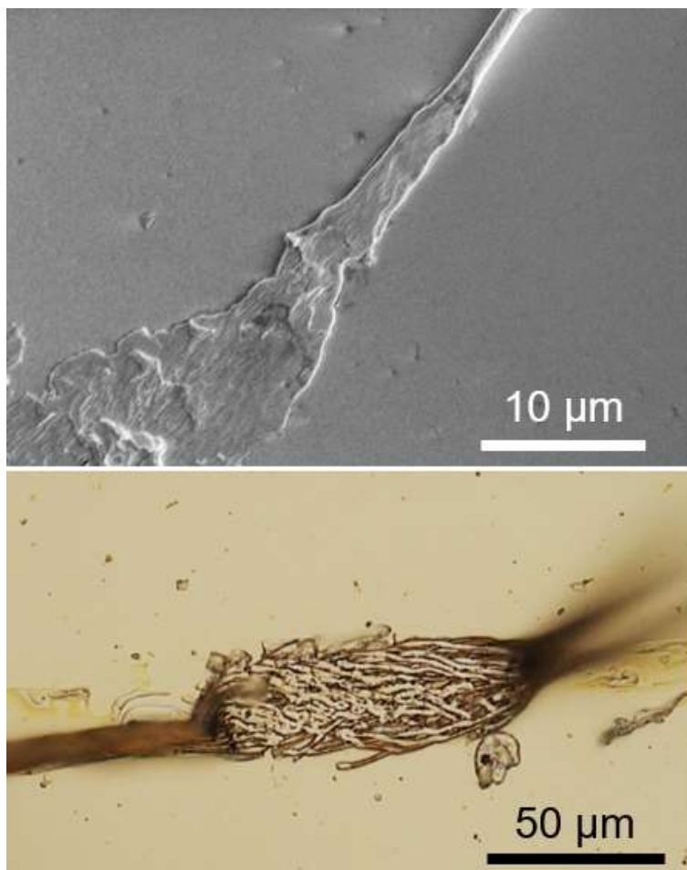
Figure 30. Wire bonding individual metal-coated PMIA nanofibers (top) and nano-litz bundles of ALD-insulated wires (bottom)
