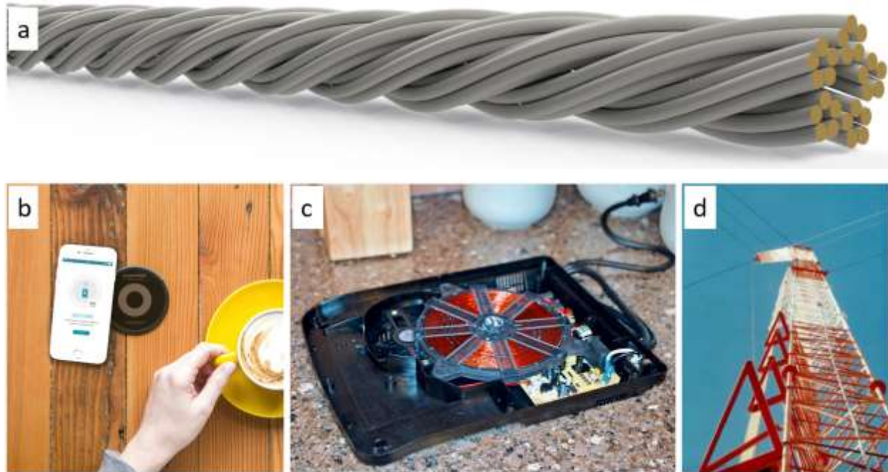
Figure 3. Litz wire and its uses. a, Schematic illustration of a hierarchically-twisted litz bundle of five bundles of five strands each (for 25 total wires). b-d, Example uses of litz wire at sub-MHz frequencies: b, Qi wireless charging mat. c, Induction stove. d, NIST WWVB timing signal transmitting tower.
