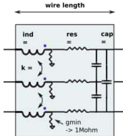
Figure 46. Coupling Capacitance model
