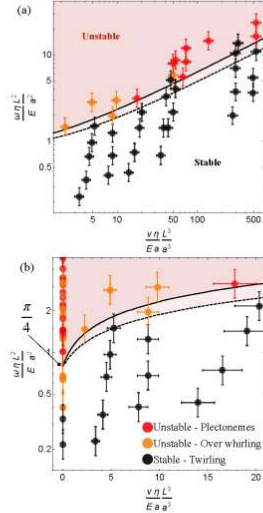
FIG. 2. Phase diagrams of instability with log-log (a) and log-linear (b) scaling. The solid and dashed lines show Eq. (7) with \alpha = 8 for (L/a) = 100 and (L/a) = 1,000 , respectively. The region above each line is predicted to be unstable to helical buckling for the given (L/a) . Error bars show one standard deviation attributed to experimental conditions. Parameters from individual data points are given in the S.I.
