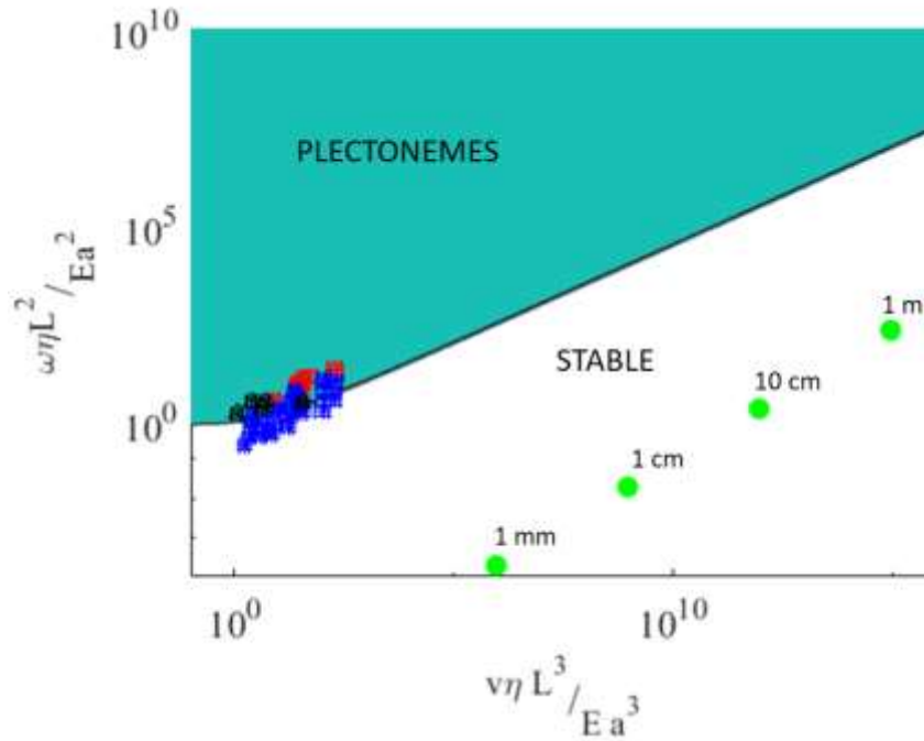
Figure 61. Macro-scale modeling and analytical results show that the approach used for twisting Nomex wires into nanolitz should scale from the milli- and centimeter-length-scales to meter without inducing buckling instabilities.
