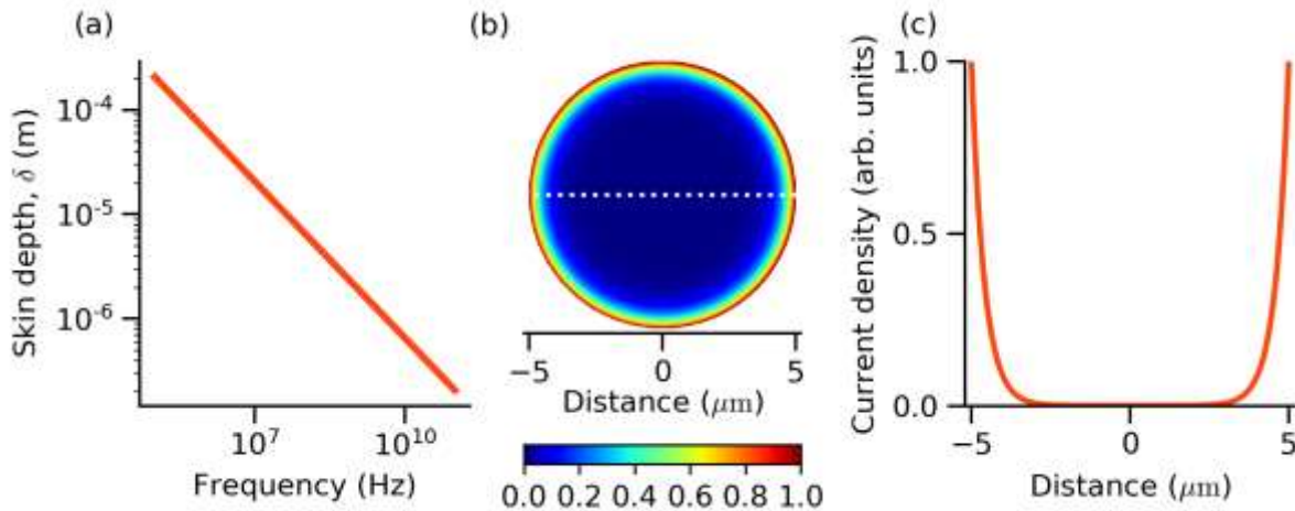
Figure 2. Skin depth and skin effect. (a), Skin depth versus frequency for bulk copper ( \rho=1.68\text{E-}8 \Omega\text{-m} ). (b) and (c), Finite element simulation of current distribution in a 58 AWG copper wire at 28 GHz. (b), Cross-sectional plot of normalized current density. (c), Current density versus radial position along the dotted section line in (b)
