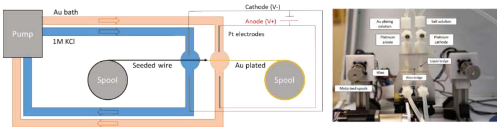
Figure 18. Reel to reel CBPE electroplating using fluid droplets. Two platinum covered titanium rods are used as both the anode and cathode in two separate streams of conductive saline and gold plating solution which are bridged by the wire.
