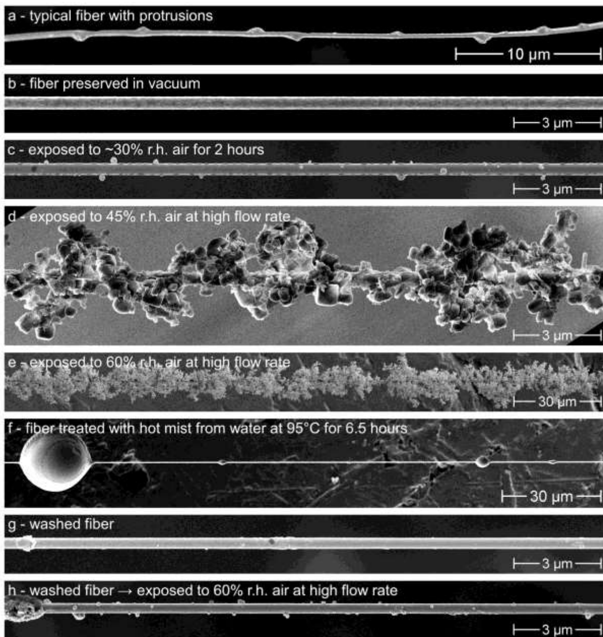
Figure 8. Humidity-dependent morphology evolution: (a) SEM image of a bumpy Pt/Pd alloy (80/20) coated PMIA fiber. (b) Fiber kept in vacuum for 2 hours before imaging. (c) Fiber exposed to ambient air at ~30% RH for 2 hours. (d) Fiber annealed with a high flow rate 45% RH air at room temperature. (e) Fiber annealed with a high flow rate 60% RH air at room temperature. (f) Fiber annealed over a beaker of hot water for 6.5 hours. (g) Fiber where \text{CaCl}_2 is mostly removed by treatment with an ultrasonic humidifier for 6 hours. (h) After \text{CaCl}_2 was removed with the previous treatment, fibers were exposed to a high flow rate of 60% RH air as in part d, but they did not roughen nearly as much. (All fibers were coated with a thin layer of Pt/Pd alloy (80/20) to assist with imaging.)
