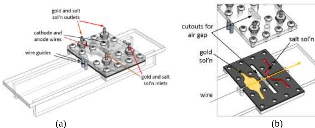
Figure 20. (a) Mesofluidic chip for contactless electroplating onto a continuously-moving nanofiber scaffold (b) Exploded drawing of chip detail view.
