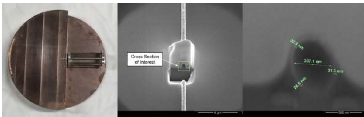
Figure 13. Apparatus for continuously rotating a spool during sputter deposition. Left, Optical image of apparatus (6" diameter). Center and Right, FIB cross-section of completed sputtering, showing the ~300 nm diameter PMIA nanofiber coated with ~30 nm of metal
