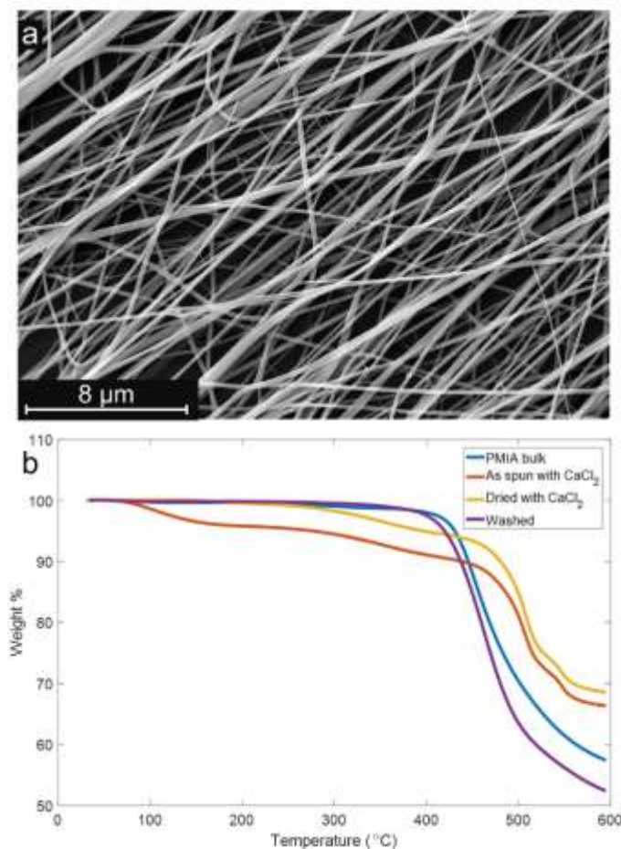
Figure 54. Thermal stability of electrospun PMIA nanofibers. (a) SEM image of a mat of PMIA fibers. (b) TGA results for PMIA bulk starting material, electrospun fibers containing hydrated CaCl 2 , CaCl 2 -containing fibers that were dried inside the TGA instrument, and fibers that were washed by immersion in water. (A 12 wt. % PMIA and 8 wt. % CaCl 2 in DMAc was used to generate the thick mat used in TGA.)
