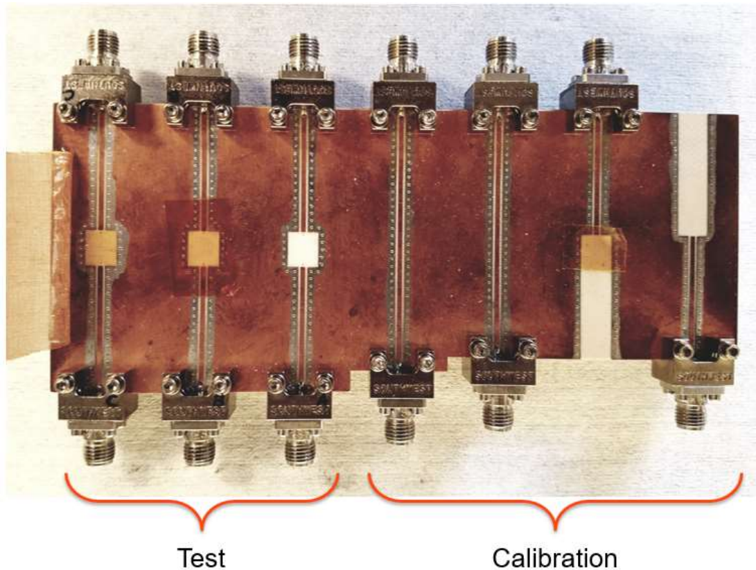
Figure 31. Optical image of resonant cavity measurement fixture
