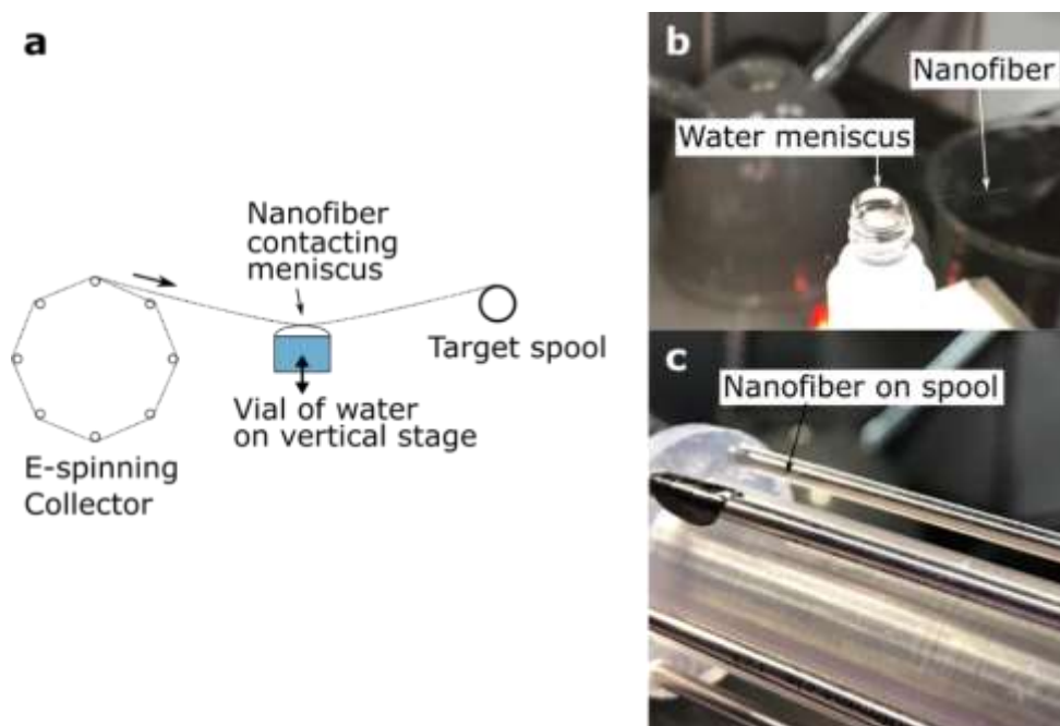
Figure 11. Controlling tension during spooling of PMIA nanofiber. a, Schematic illustration of our tensioning process utilizing hydrophilic interactions between the nanofiber and a water meniscus to provide controllable sub-micronewton forces to tension the nanofiber during spooling. b, Image of PMIA nanofiber in contact with water meniscus during spooling. c, Image of PMIA nanofiber wound around target spool.
